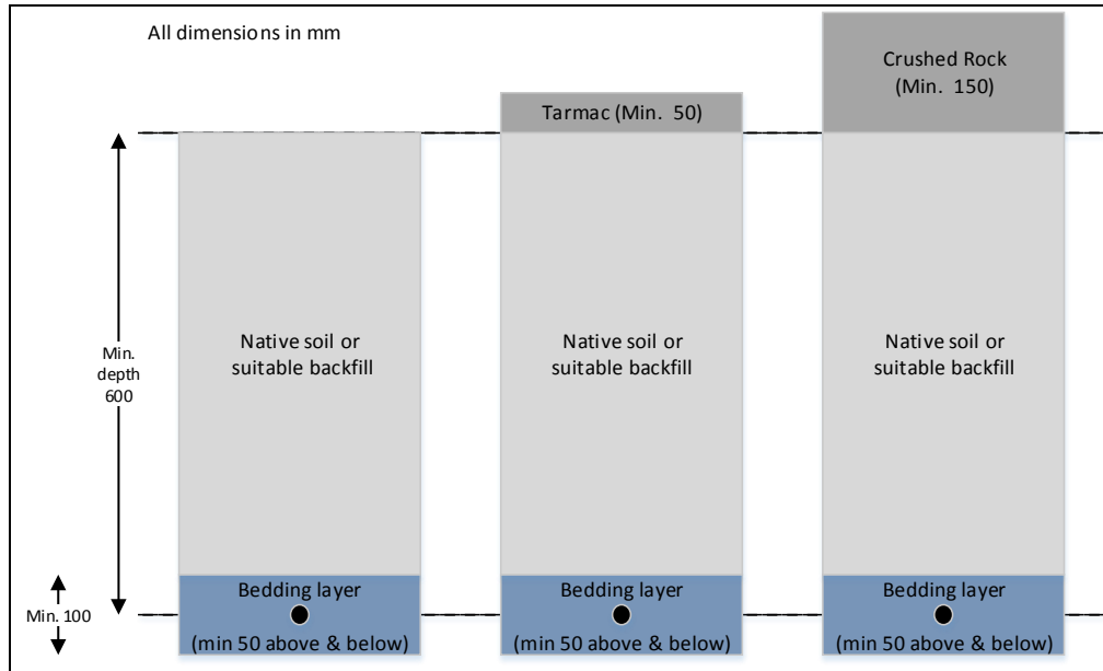
Figure 1: Electrode depth
