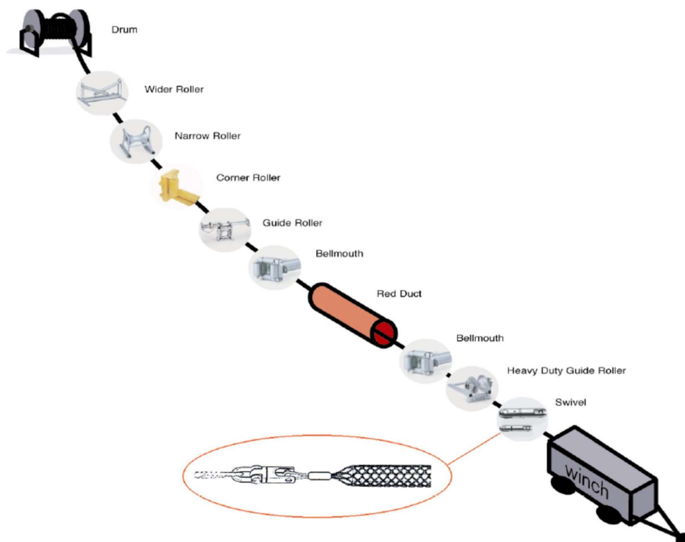
Figure 4 - Set up for Cable Pulling
