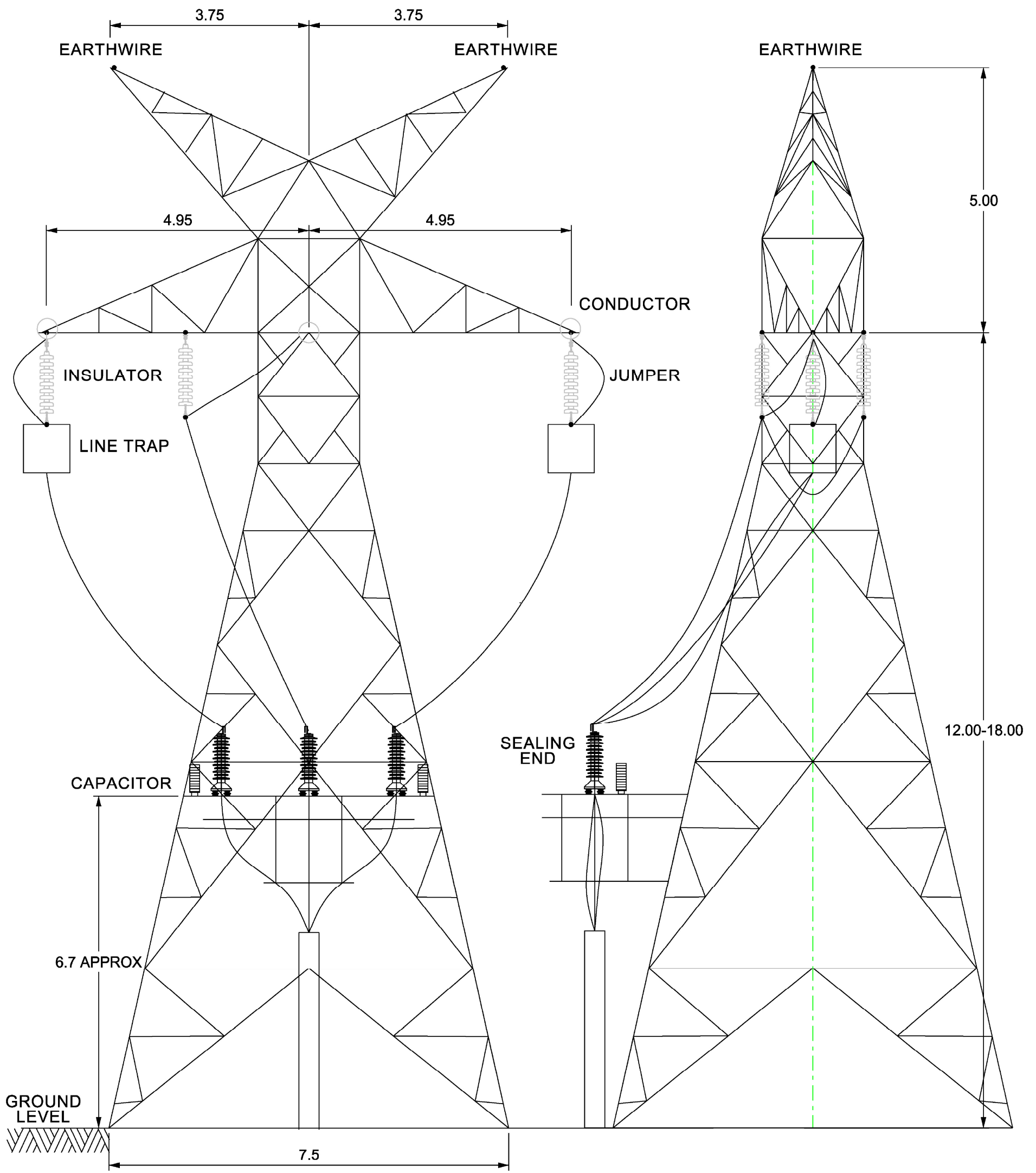
TRANSVERSE VIEW
