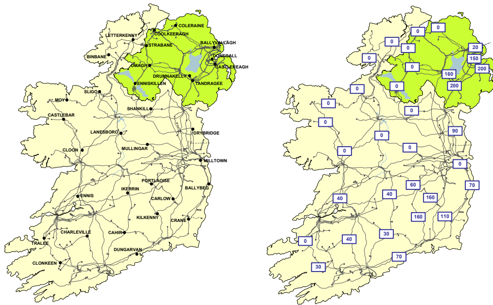
Figure 7-2: Generation opportunity at 110 kV stations in 2025
