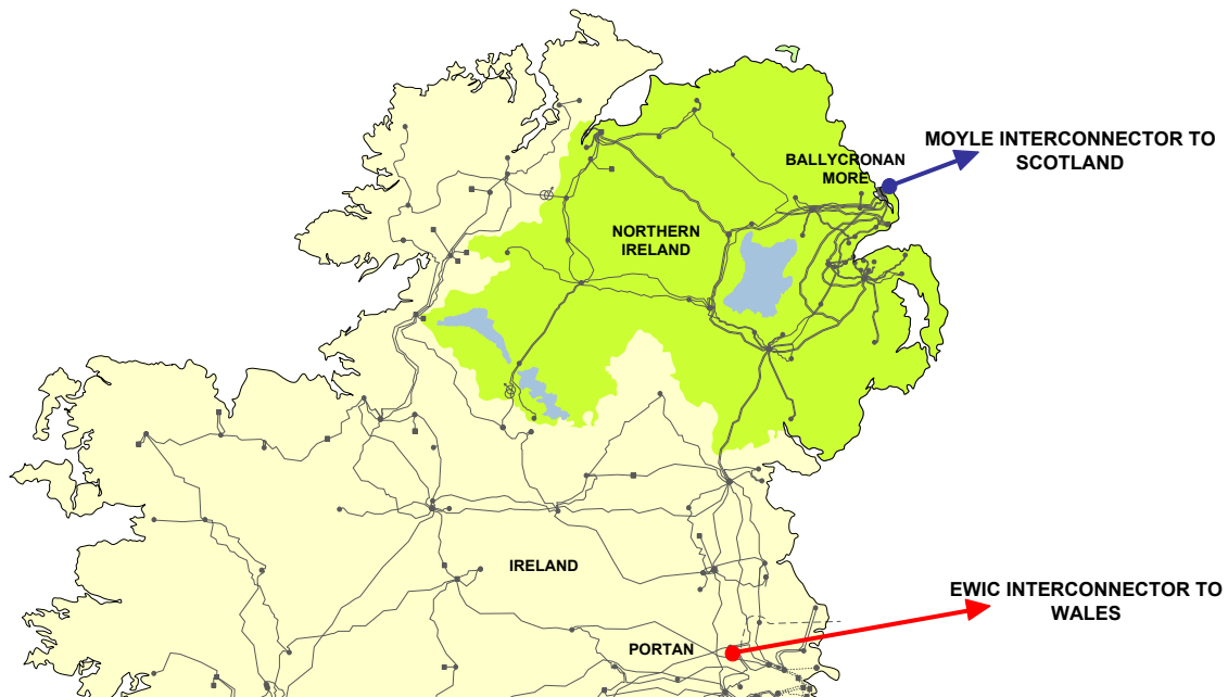
Figure 2-2 Existing Interconnectors
