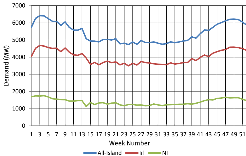
Figure 3-3 Weekly Demand Peak Values for Year 2015
