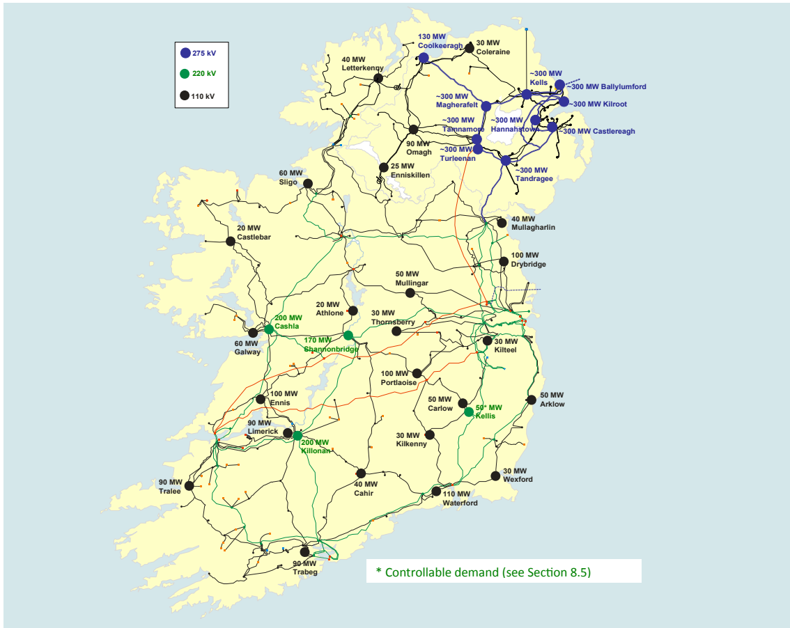
Figure 8-1 Capability for Additional Demand at 275 kV, 220 kV and 110 kV Stations (given to the nearest 10MW)
