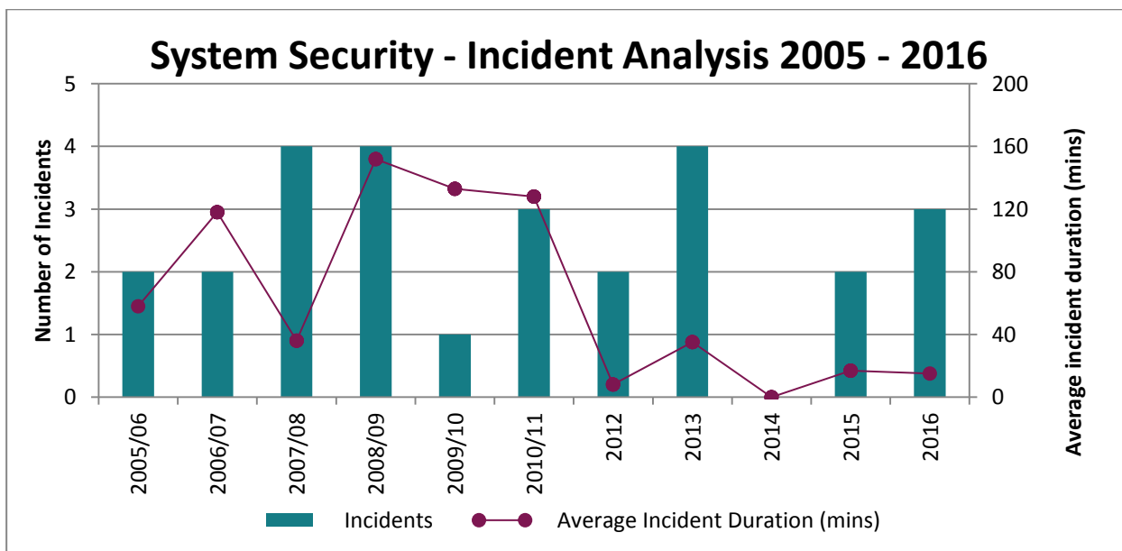
Figure 29: Historic System Security 2005-2016
