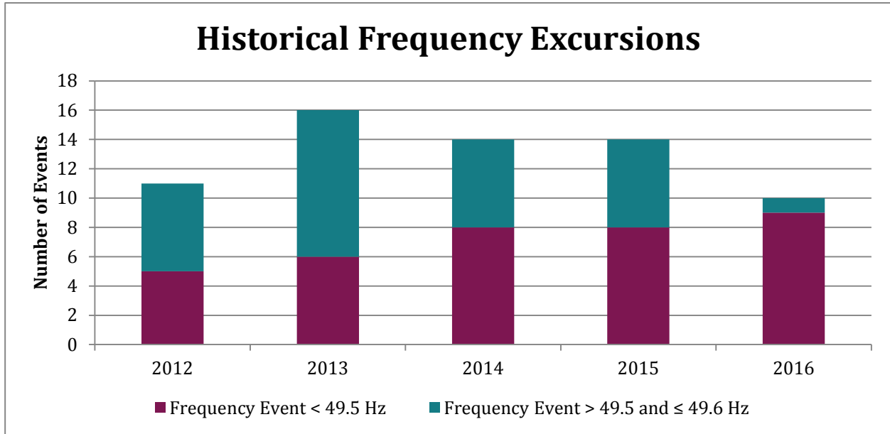
Figure 31: Historic Frequency Excursions 2012-2016
