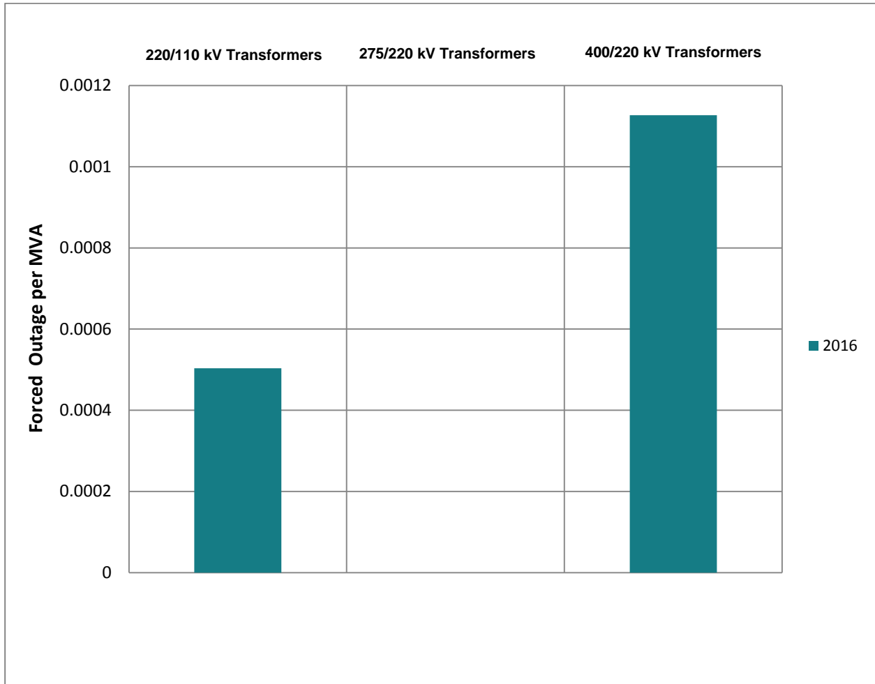
Figure 17: Transformer Forced Outages in 2016
