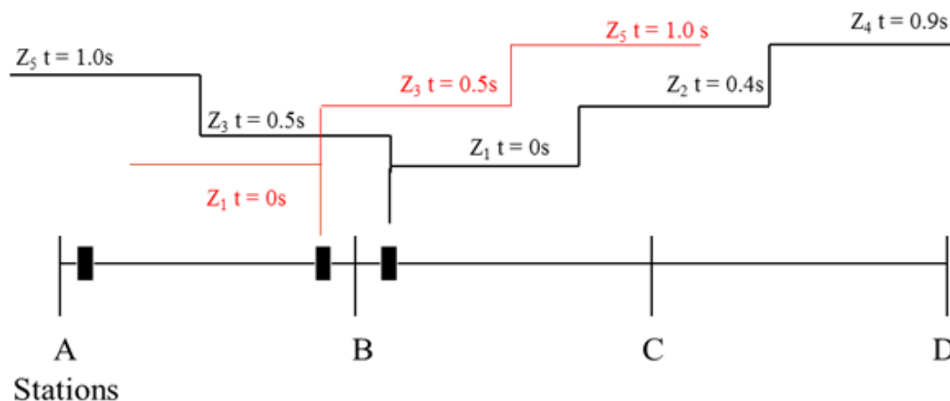
Figure 32: Zones of Protection
