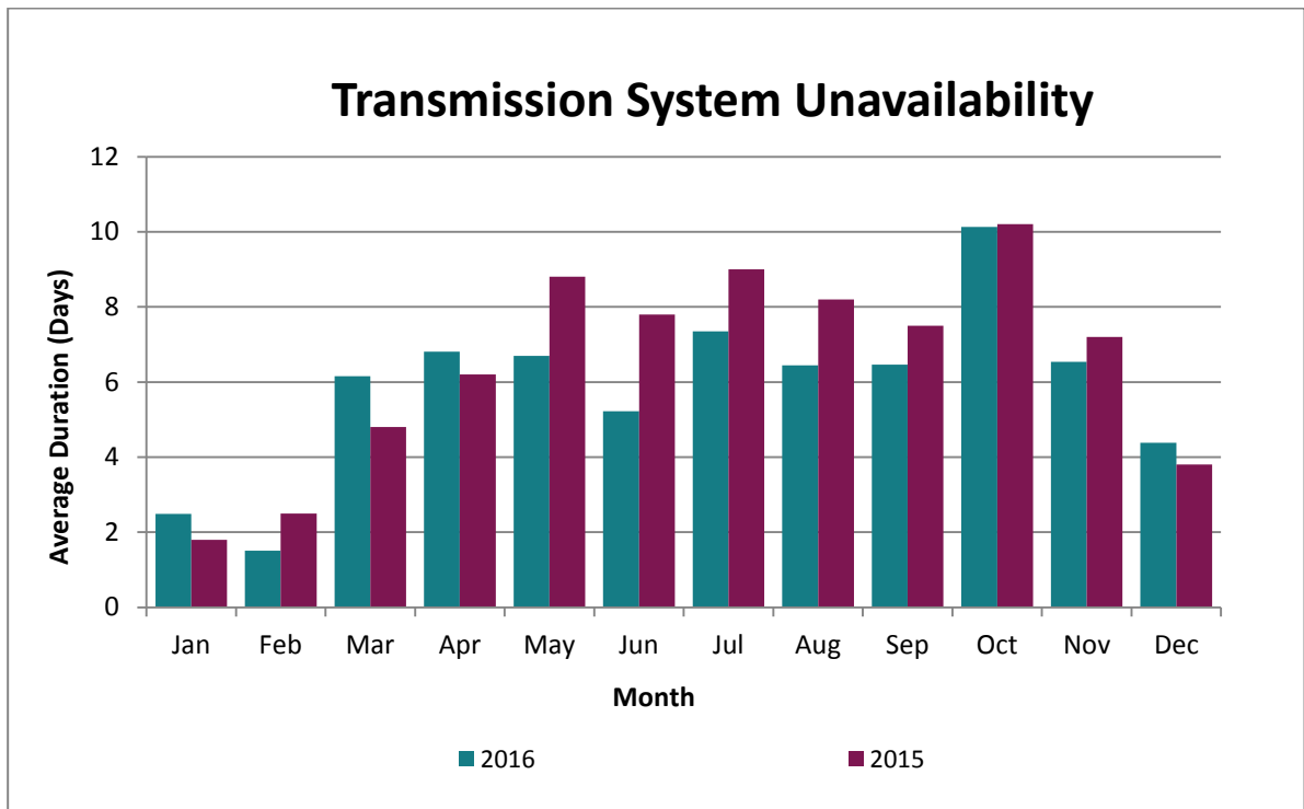
Figure 15: Average duration of outages 2015 & 2016
