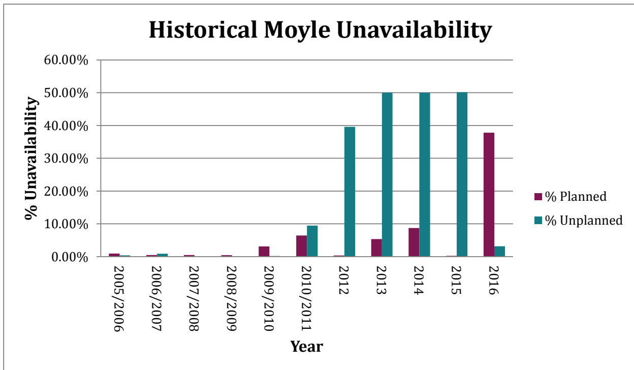
Figure 23: Historic Moyle Interconnector Unavailability 2005-2016
