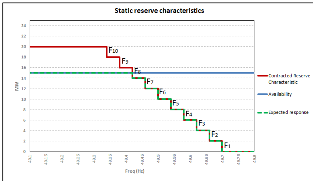
Figure 5: Required Response Characteristic (Truncated response)
