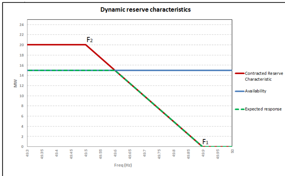
Figure 3: Required Response Characteristic
