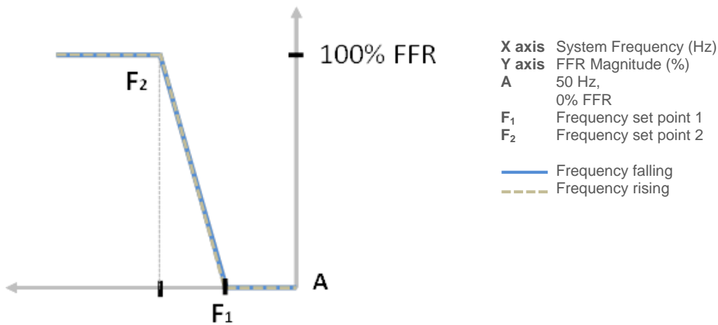
Figure 2: FFR Dynamic Capability Frequency Response Curve.
