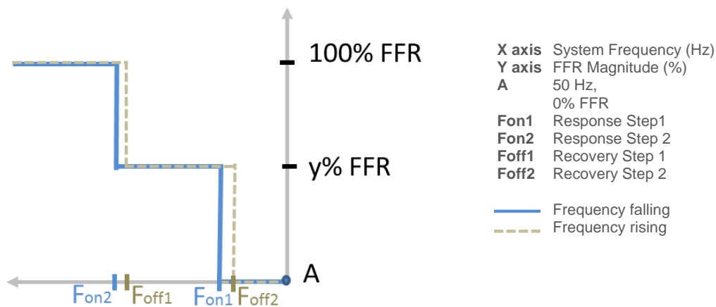
Figure 34: FFR Static Capability Frequency Response Curve
