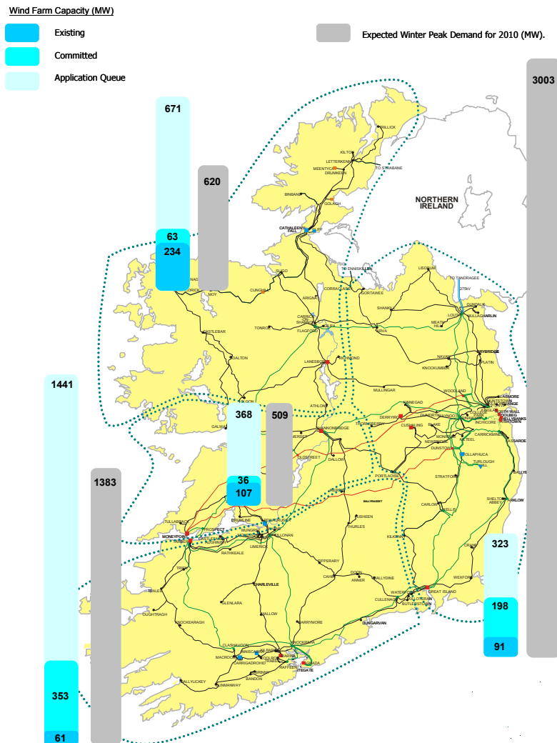
Figure 5-2: Map indicating the geographical profile of wind generation applications
