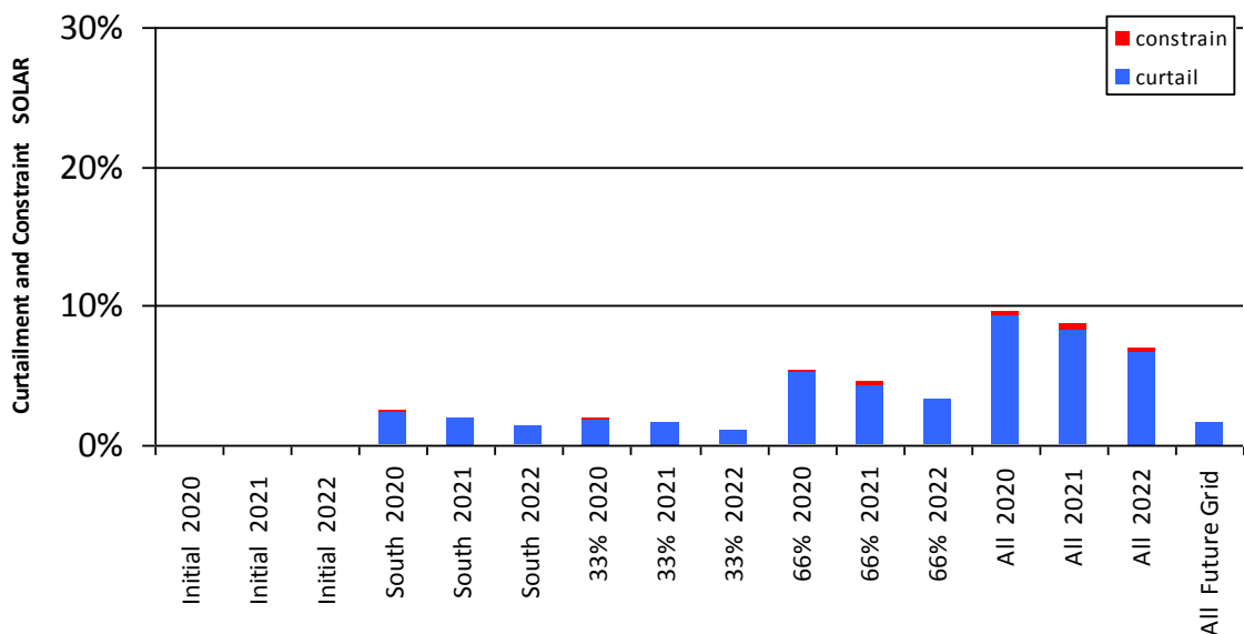
Figure 0-11 Curtailment and Constraint for Midleton
