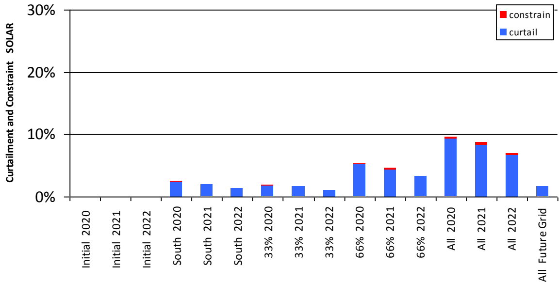
Figure 0-7 Curtailment and Constraint for Cow Cross
