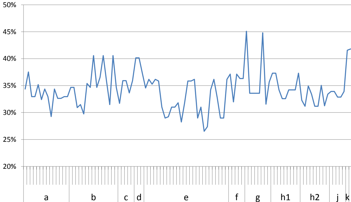
Figure 0-3 Capacity Factor by Node, grouped by Area, for Existing Wind
