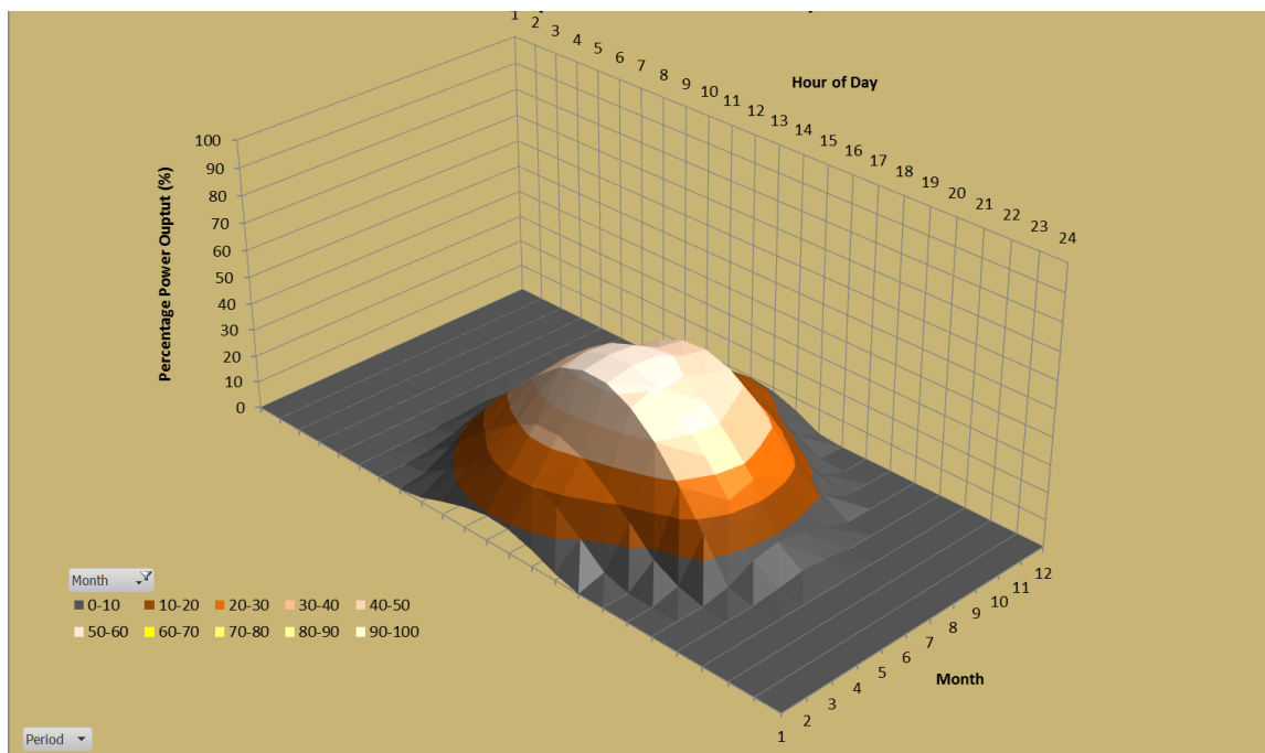
Figure 0-1 Solar Energy Profile (monthly average – hour of day)
