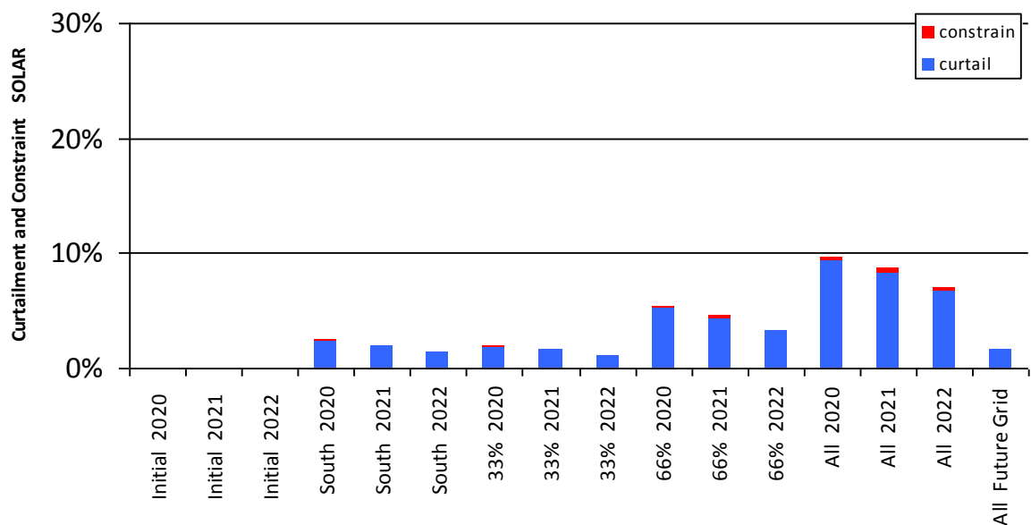
Figure 0-13 Curtailment and Constraint for Trabeg
