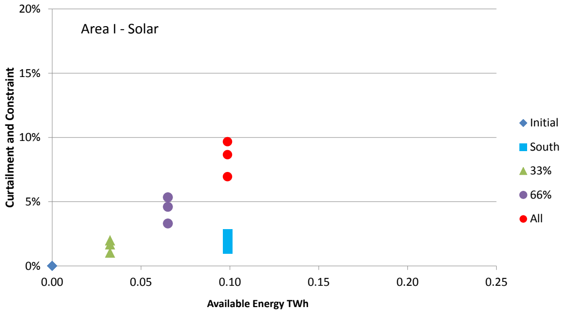
Figure 5-2 Average Curtailment and Constraint Area I Solar
