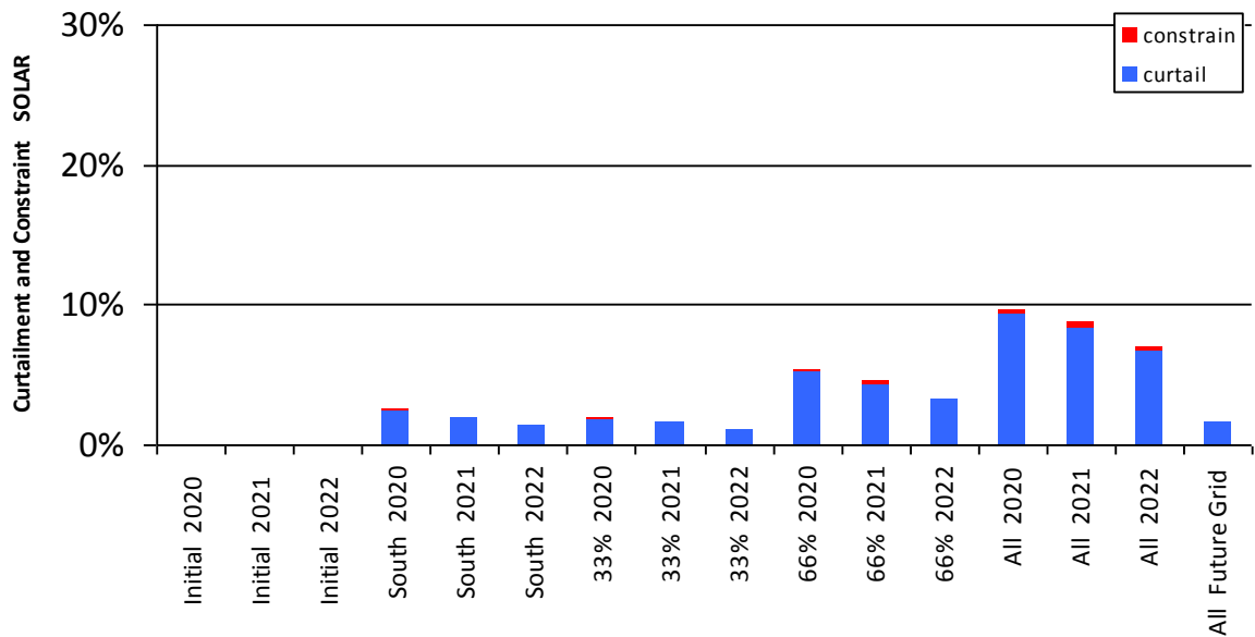
Figure 0-5 Curtailment and Constraint for Coolroe
