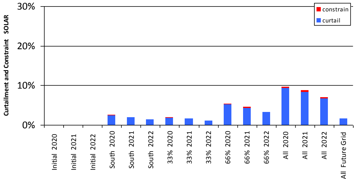
Figure 0-3 Curtailment and Constraint for Barnahely
