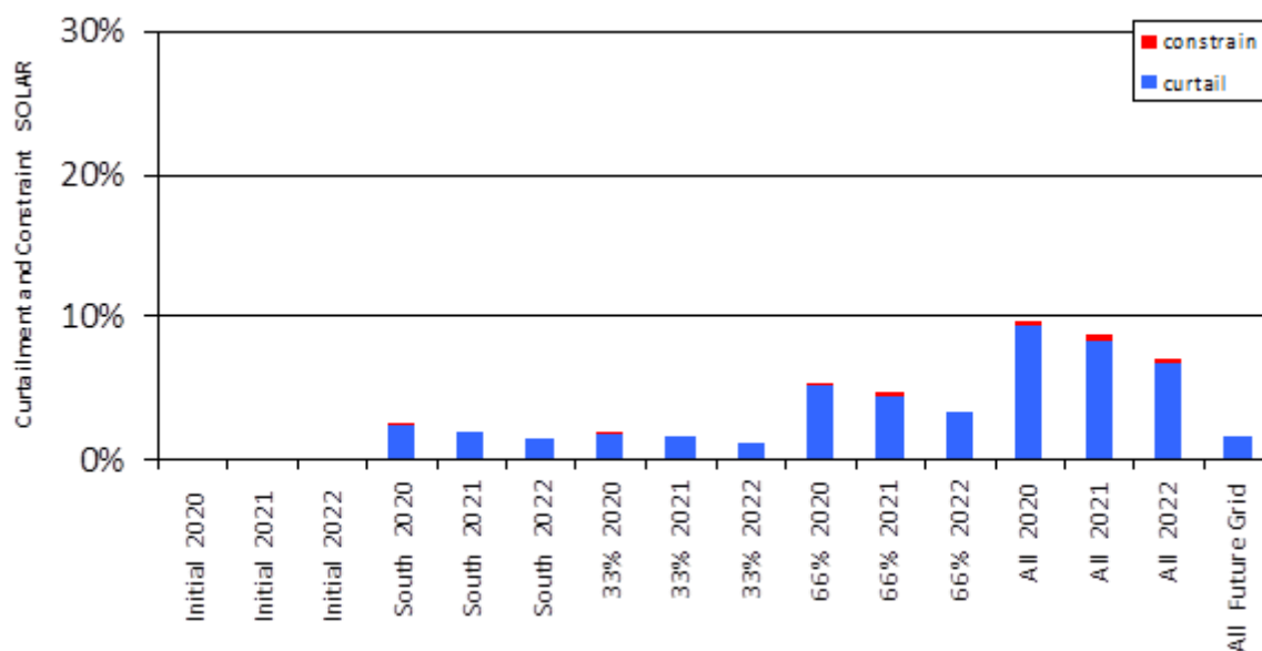
Figure 5-2 Average Curtailment and Constraint in Area I (solar only)
