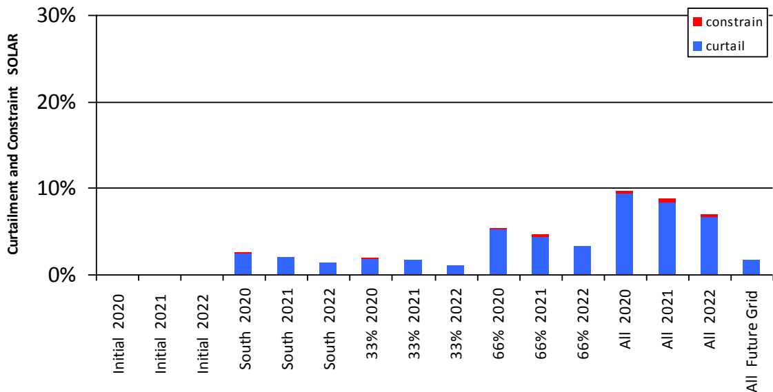
Figure 0-9 Curtailment and Constraint for Kilbarray
