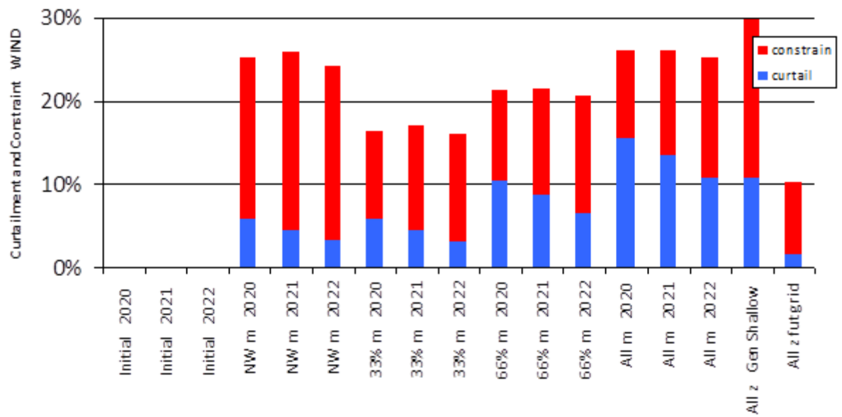
Figure 0-20 Curtailment and Constraint for Letterkenny Wind
