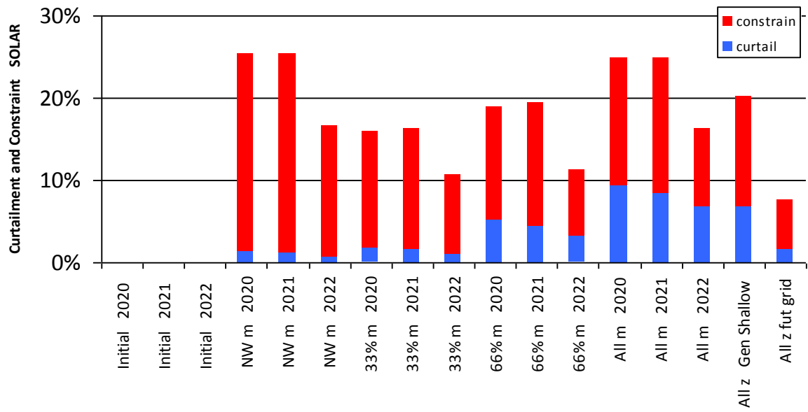
Figure 0-11 Curtailment and Constraint for Corderry Solar
