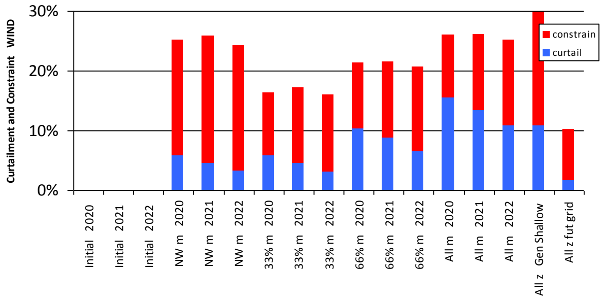
Figure 0-7 Curtailment and Constraint for Carrickaduff and Carrickalangan Wind
