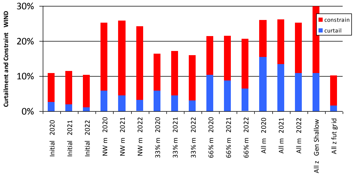
Figure 0-3 Curtailment and Constraint for Ardnagappary Wind
