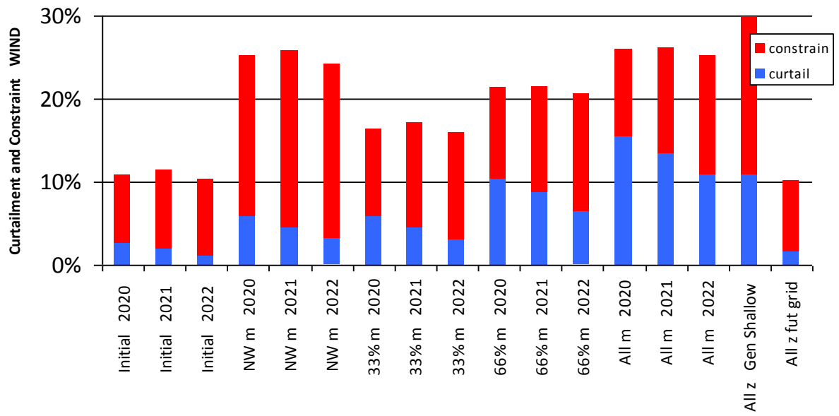
Figure 0-26 Curtailment and Constraint for Sorne Hill Wind
