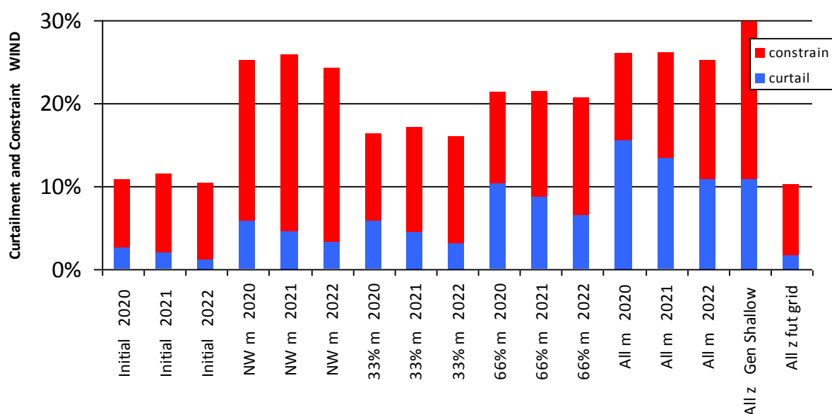
Figure 5-3 Results WIND – subgroup Area A with Sligo and (for most studies) Area C north
