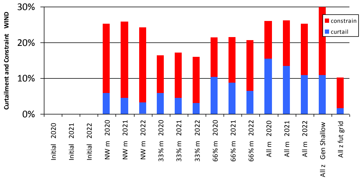
Figure 0-18 Curtailment and Constraint for Leanalea Wind
