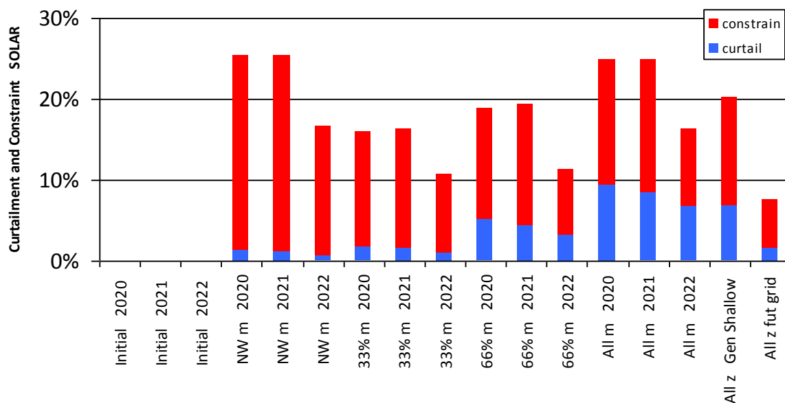
Figure 5-2 Results SOLAR – subgroup ABC Solar north
