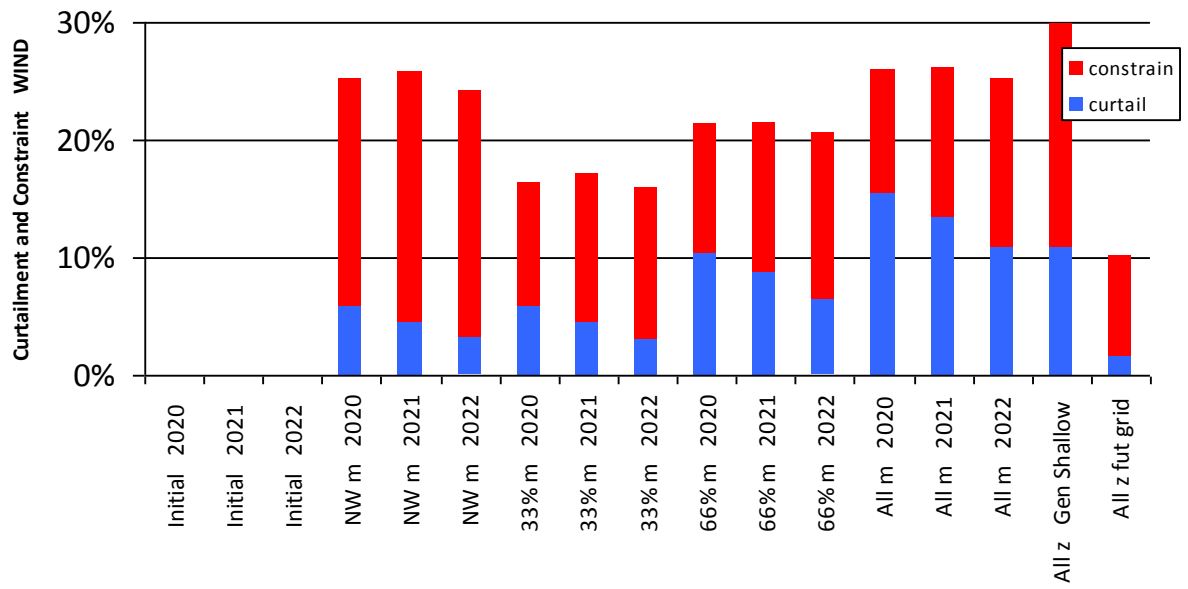
Figure 0-28 Curtailment and Constraint for Tievebrack Wind
