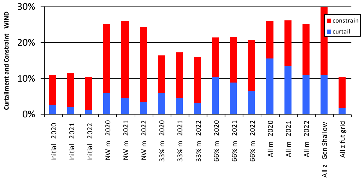
Figure 0-9 Curtailment and Constraint for Cathaleen's Fall Wind
