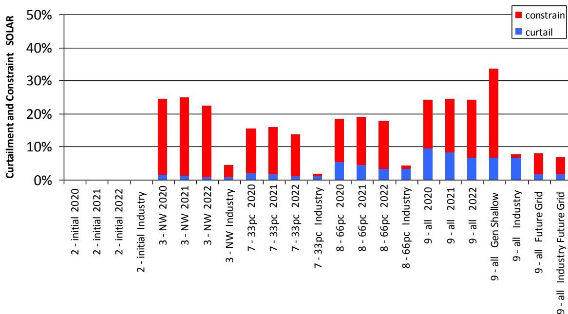
Figure 5-3 Results SOLAR – subgroup ABC Solar north
