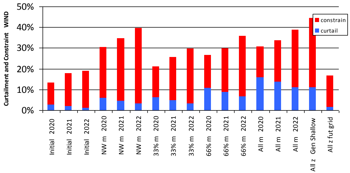
Figure 0-12 Curtailment and Constraint for Dalton Wind
