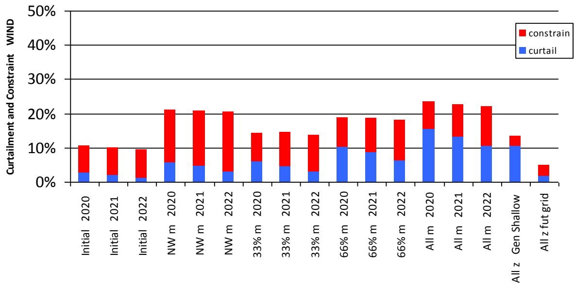
Figure 0-16 Curtailment and Constraint for Knockranny Wind
