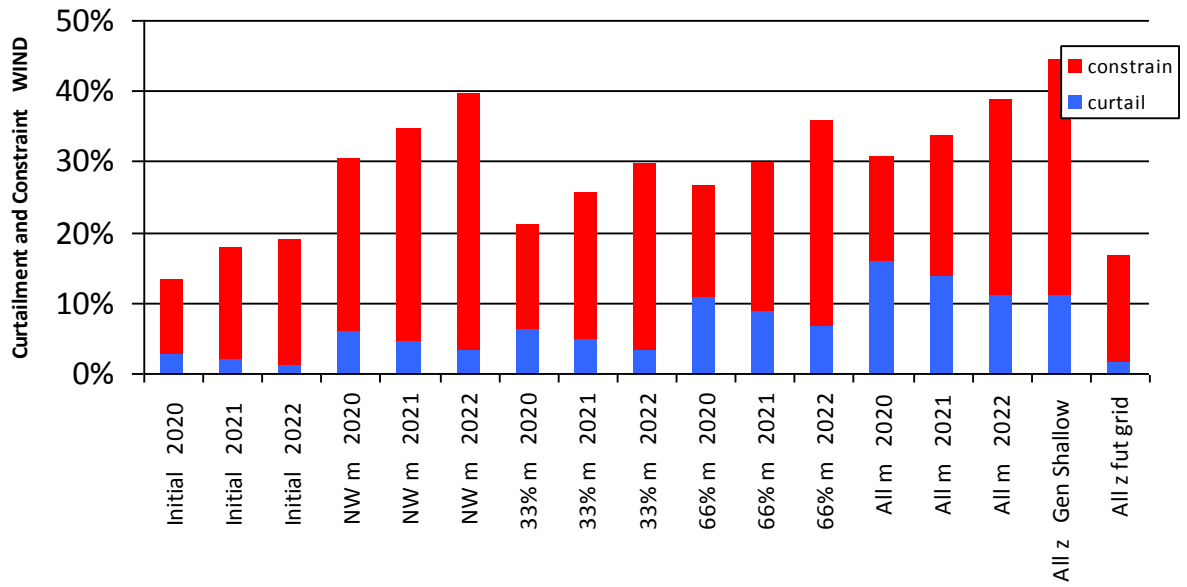
Figure 0-5 Curtailment and Constraint for Castlebar Wind
