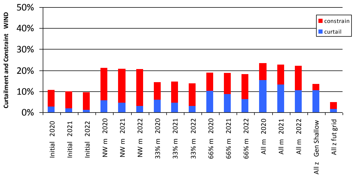
Figure 5-6 Results WIND– subgroup Area B Galway
