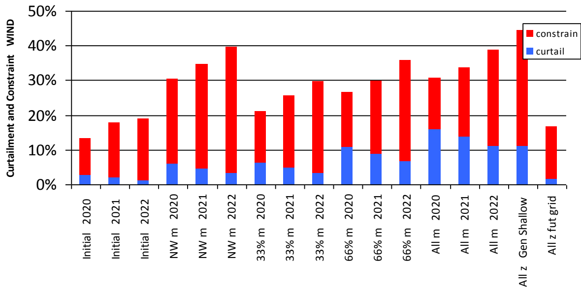
Figure 0-27 Curtailment and Constraint for Tawnaghmore Wind
