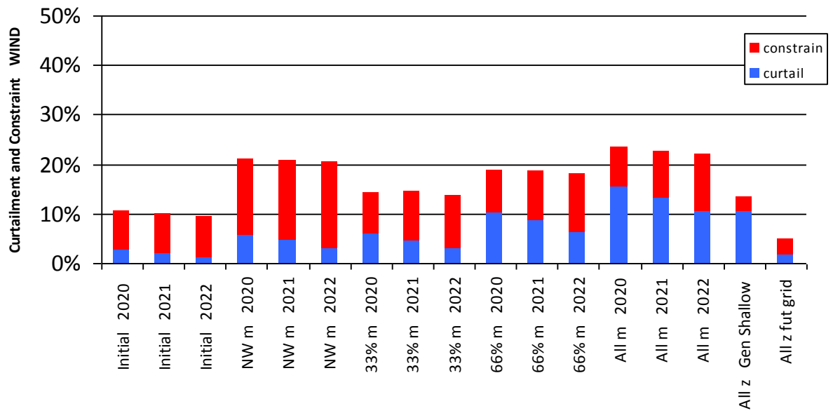
Figure 0-29 Curtailment and Constraint for Uggool Wind
