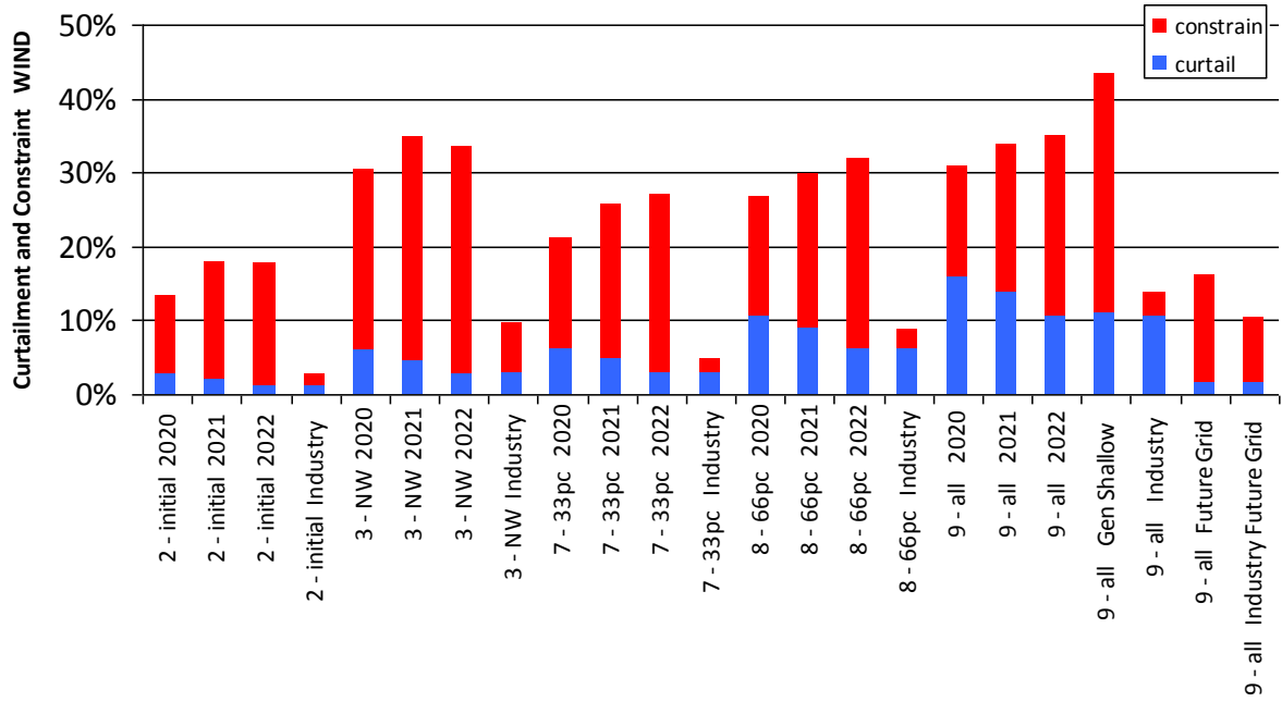
Figure 5-6 Results WIND- subgroup Area B Mayo
