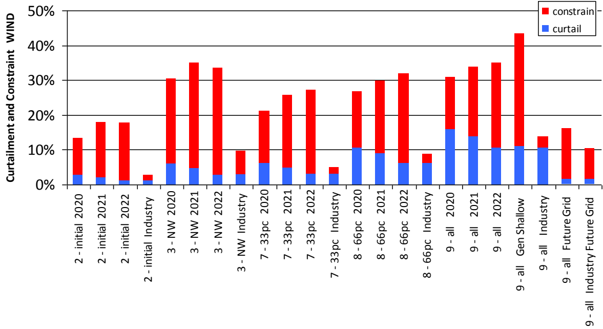
Figure 0-13 Curtailment and Constraint for Dalton Wind
