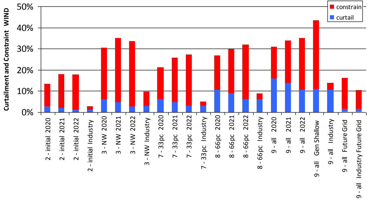
Figure 0-22 Curtailment and Constraint for Moy Wind
