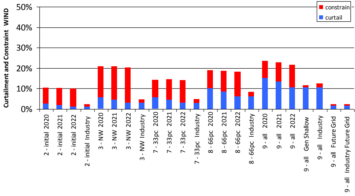
Figure 0-24 Curtailment and Constraint for Salthill Wind
