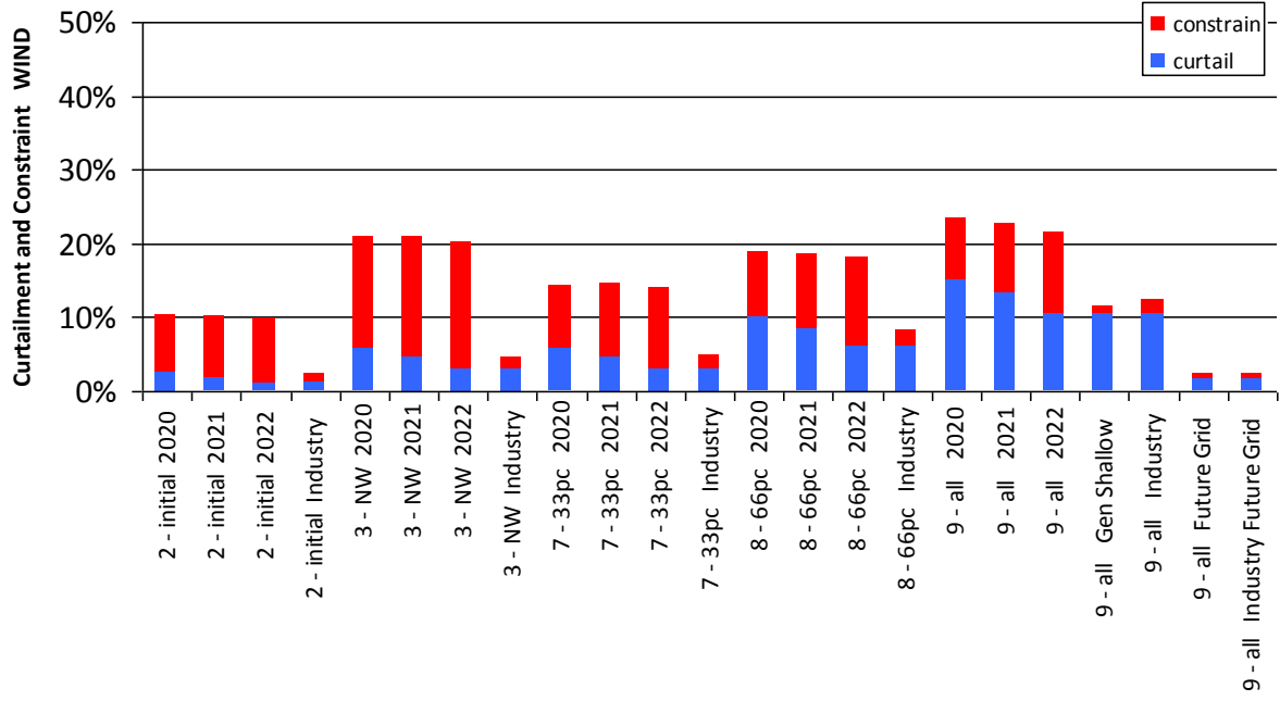
Figure 0-32 Curtailment and Constraint for Uggool Wind
