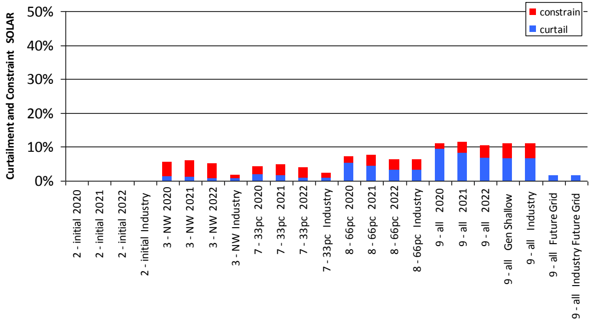
Figure 0-26 Curtailment and Constraint for Shantallow Solar
