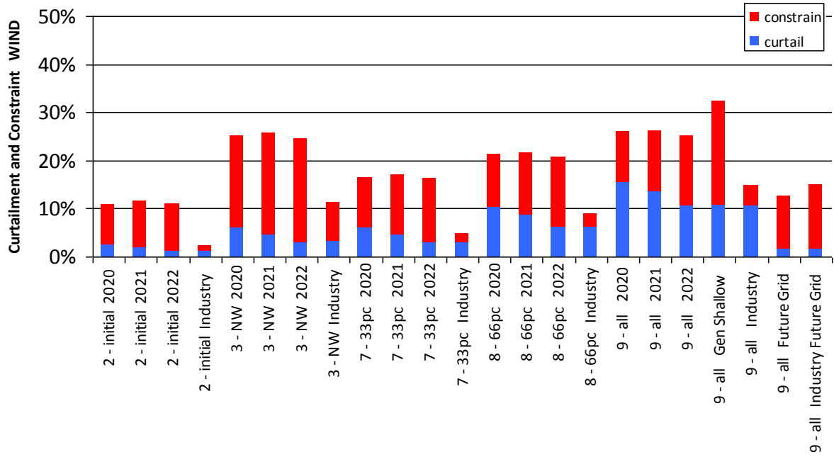
Figure 0-28 Curtailment and Constraint for Sligo Wind
