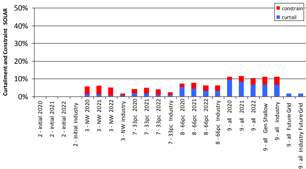
Figure 5-4 Results SOLAR – subgroup ABC South
