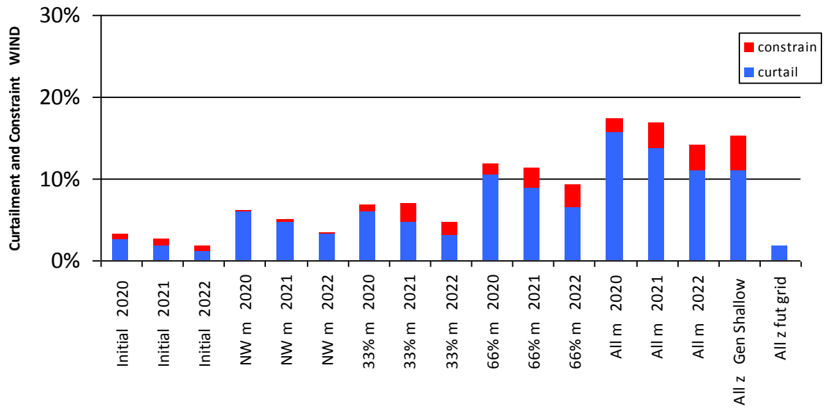
Figure 0-8 Curtailment and Constraint for Dallow Wind
