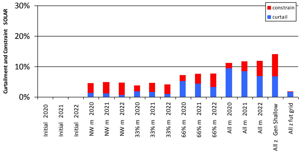
Figure 0-10 Curtailment and Constraint for Lanesboro Solar
