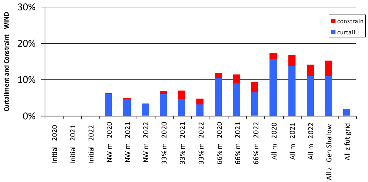
Figure 0-13 Curtailment and Constraint for Lumcloon Wind
