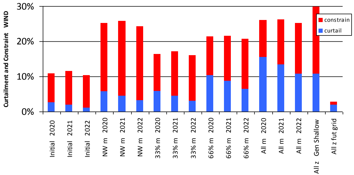
Figure 5-2 Results WIND – subgroup A and C north
