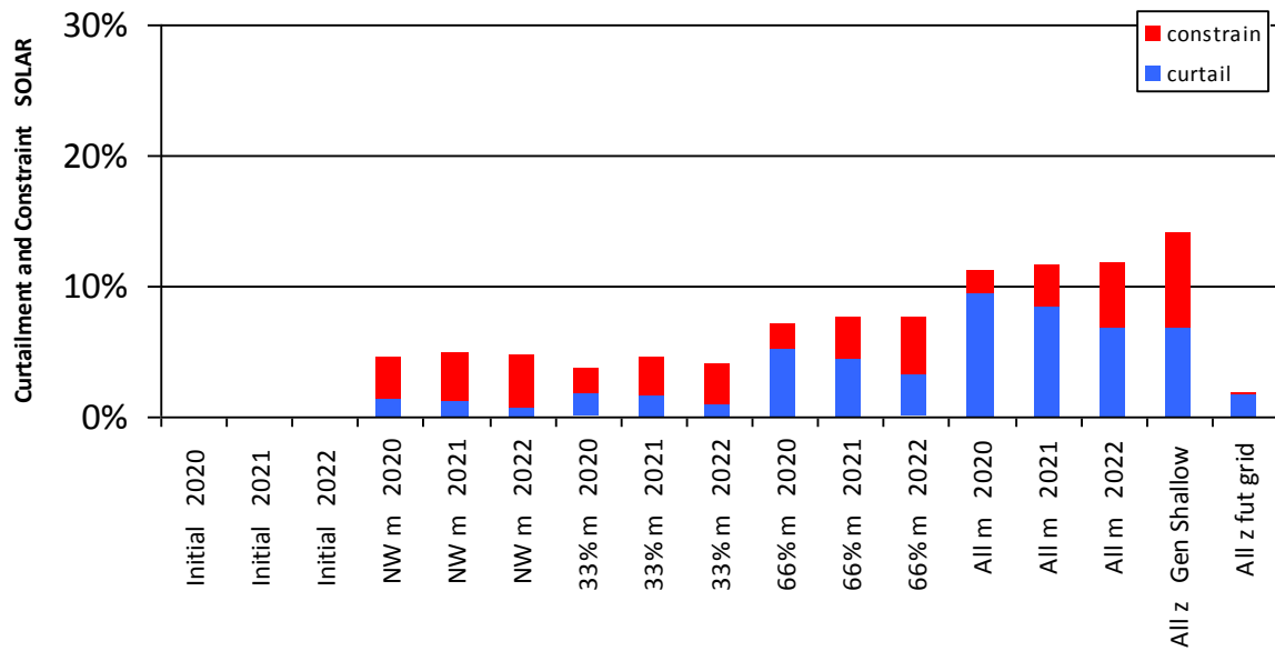
Figure 0-3 Curtailment and Constraint for Athlone Solar
