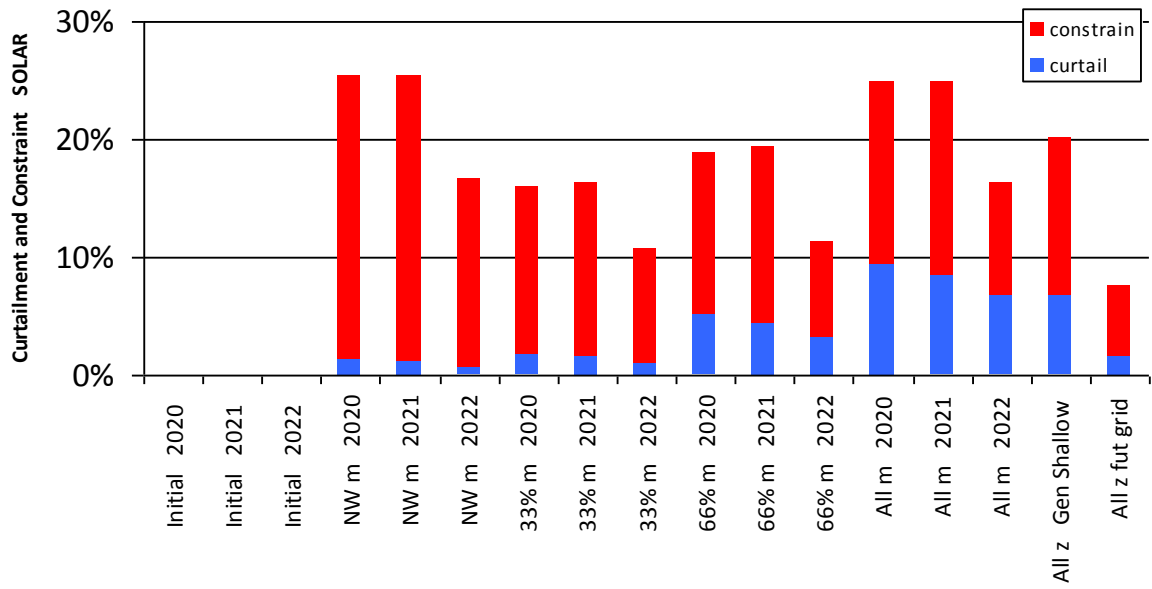
Figure 5-4 Results SOLAR – subgroup C north
