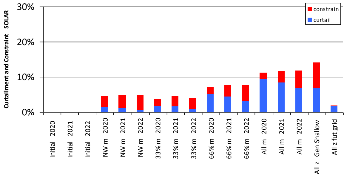
Figure 0-19 Curtailment and Constraint for Richmond Solar
