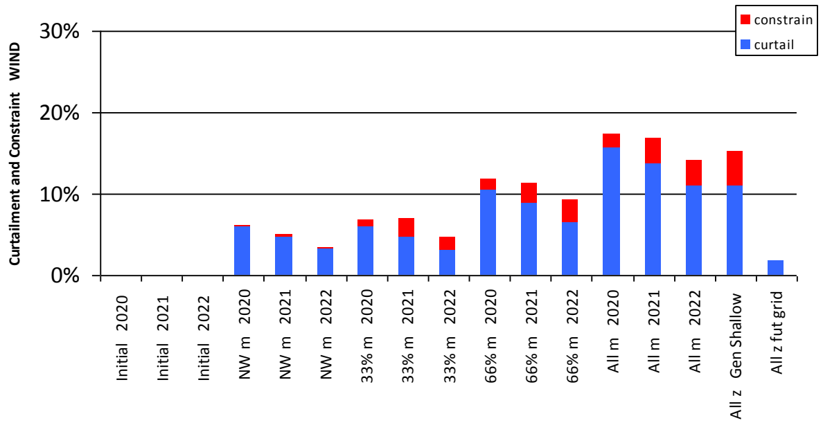
Figure 0-26 Curtailment and Constraint for Somerset Wind
