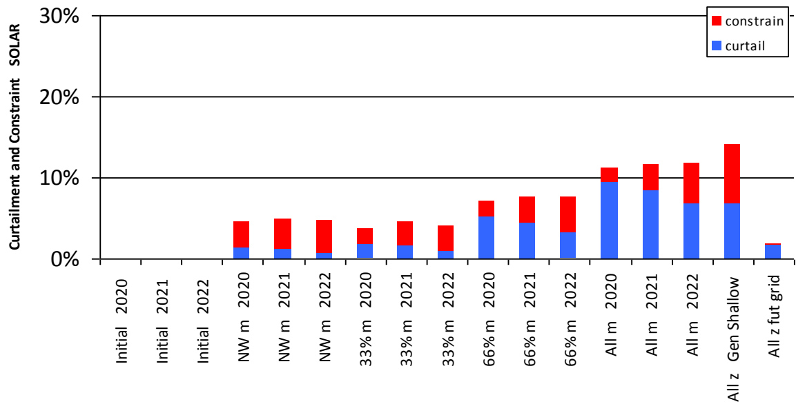
Figure 0-25 Curtailment and Constraint for Somerset Solar
