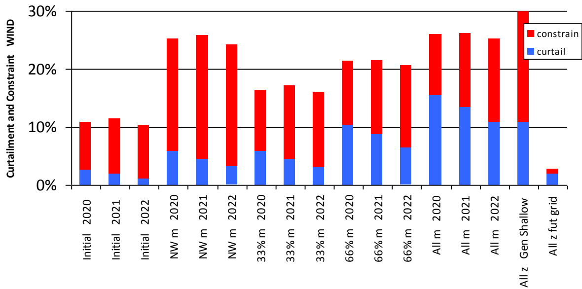
Figure 0-23 Curtailment and Constraint for Sliabh Bawn Wind
