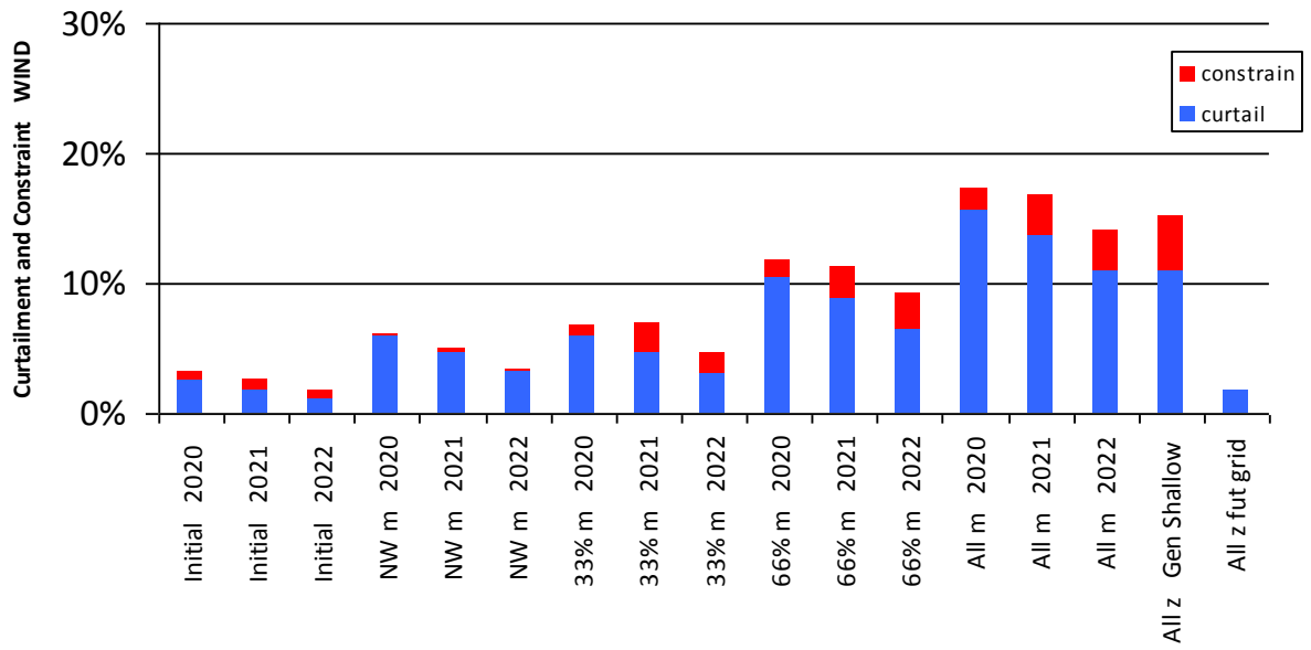
Figure 5-3 Results WIND – subgroup C south
