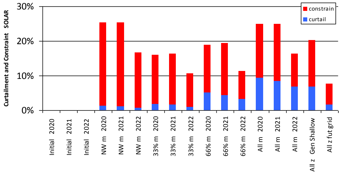
Figure 0-5 Curtailment and Constraint for Carrick on Shannon Solar
