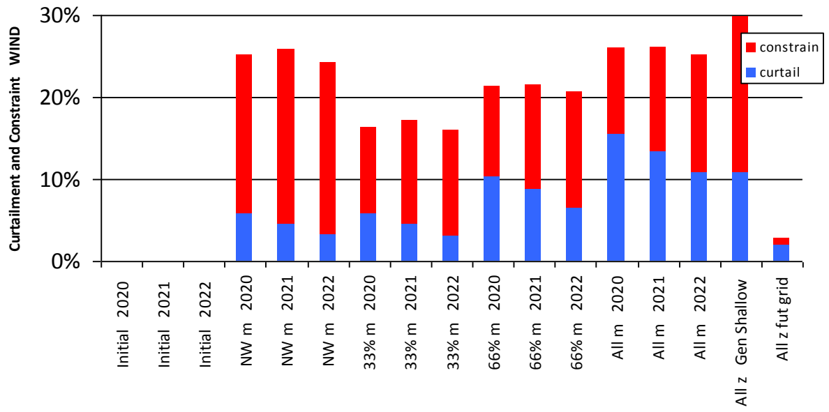
Figure 0-11 Curtailment and Constraint for Lanesboro Wind
