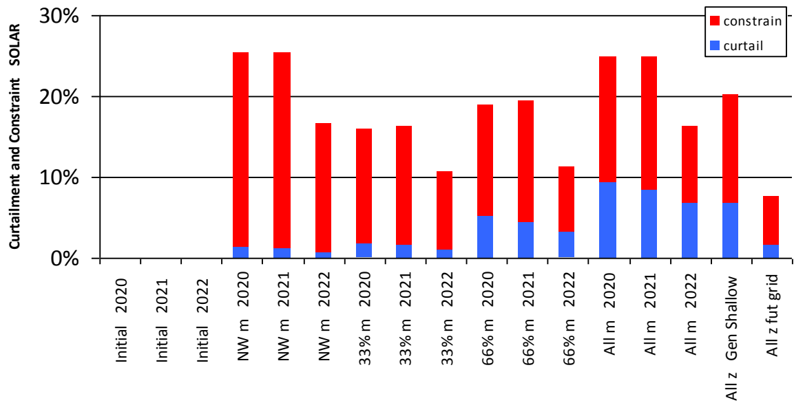
Figure 0-15 Curtailment and Constraint for Mount Dillon Solar
