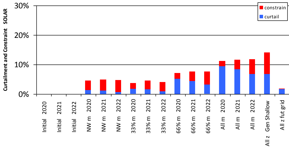
Figure 0-7 Curtailment and Constraint for Dallow Solar
