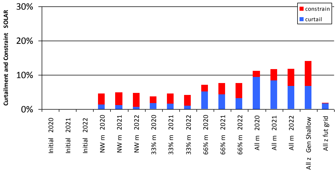
Figure 5-5 Results SOLAR – subgroup C south
