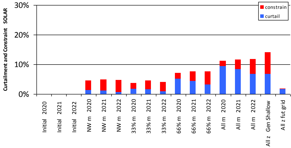
Figure 0-21 Curtailment and Constraint for Shannonbridge solar
