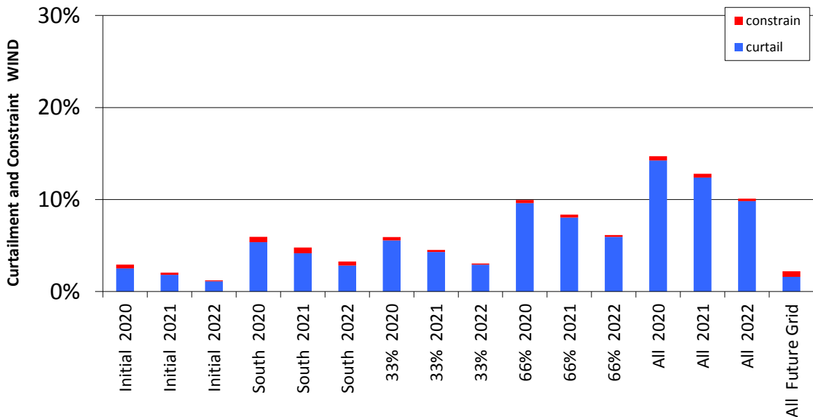
Figure 0-41 Curtailment and Constraint for Knockearagh Wind
