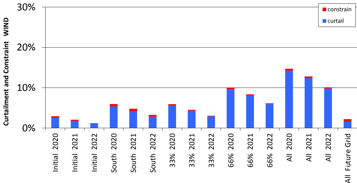
Figure 0-60 Curtailment and Constraint for Tralee Wind
