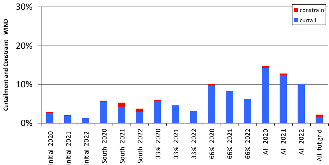
Figure 0-32 Curtailment and Constraint for Glenlara Wind
