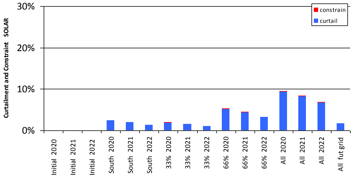
Figure 0-5 Curtailment and Constraint for Aughinish Solar
