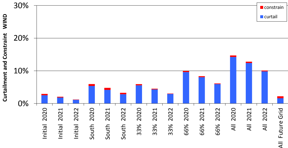
Figure 0-47 Curtailment and Constraint for Moneypoint Wind
