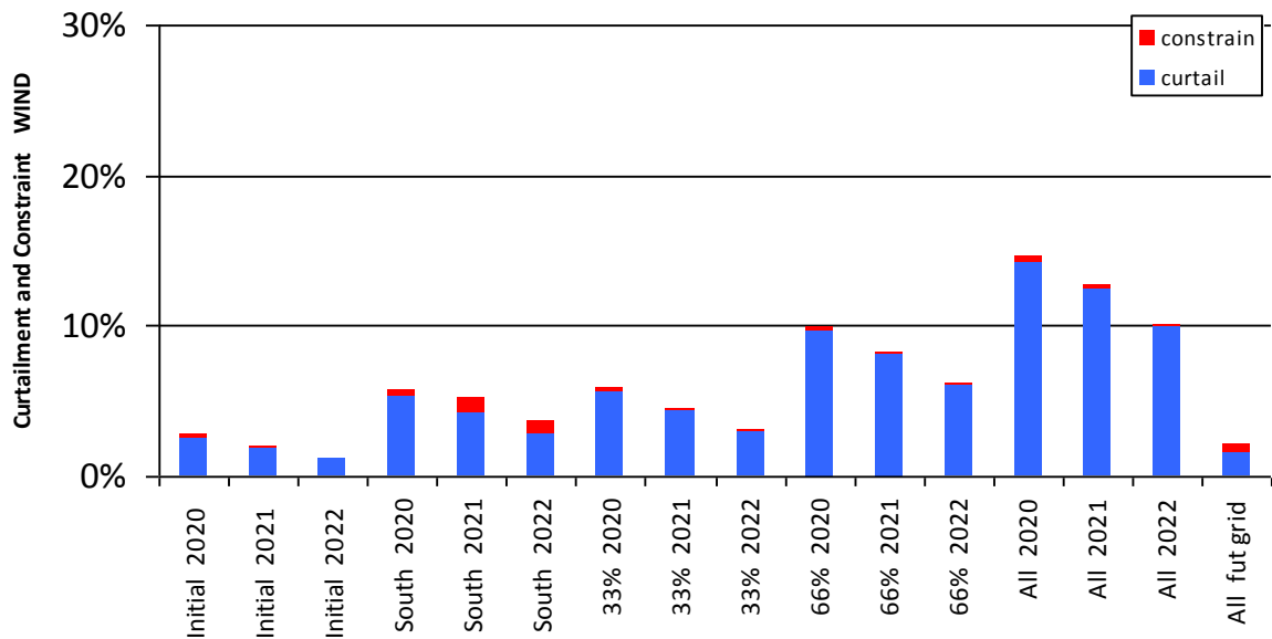
Figure 0-7 Curtailment and Constraint for Boggeragh Wind
