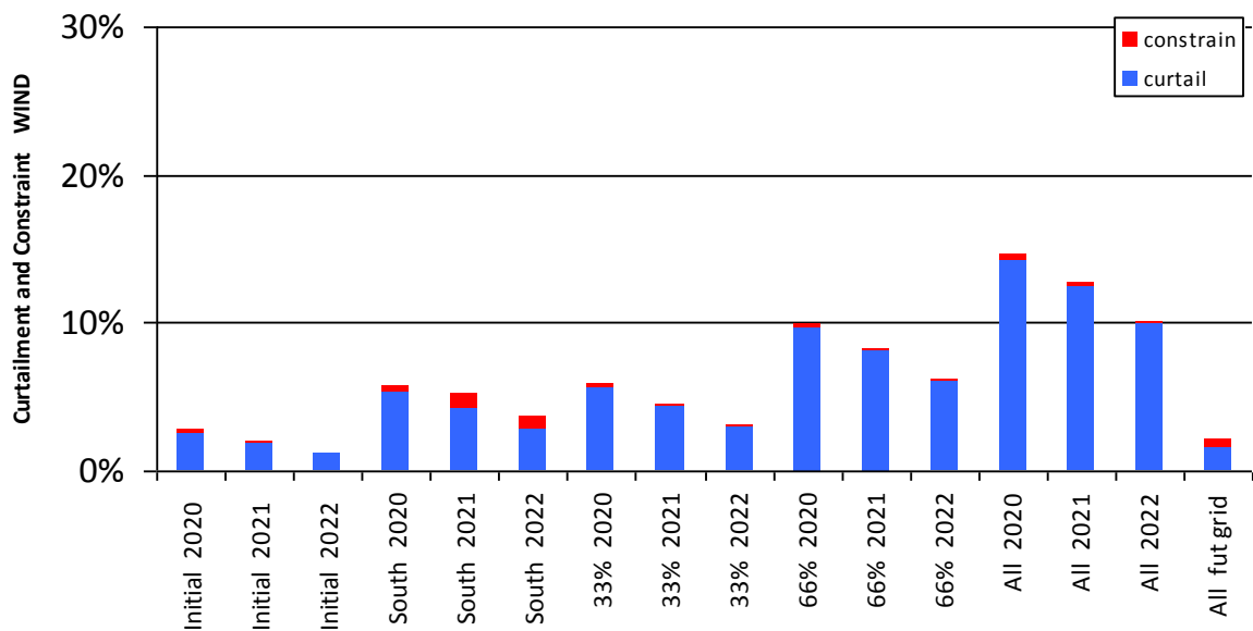
Figure 0-17 Curtailment and Constraint for Coomagearlahy Wind
