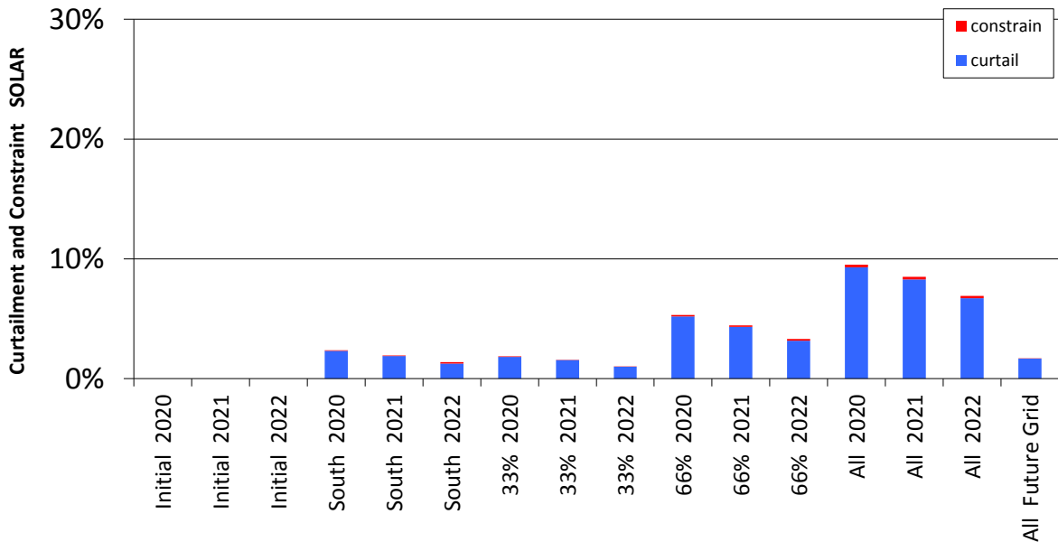
Figure 0-62 Curtailment and Constraint for Trien Solar
