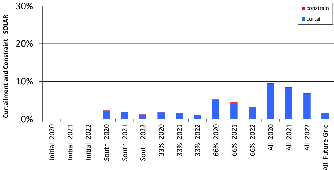
Figure 0-45 Curtailment and Constraint for Mallow Solar
