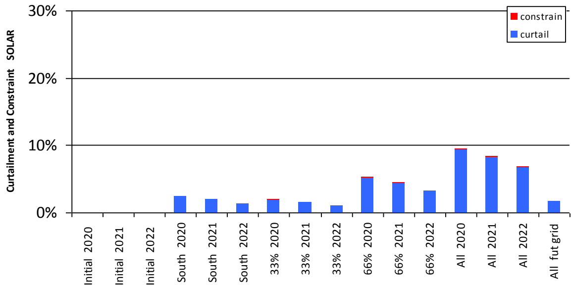
Figure 0-31 Curtailment and Constraint for Glenlara Solar
