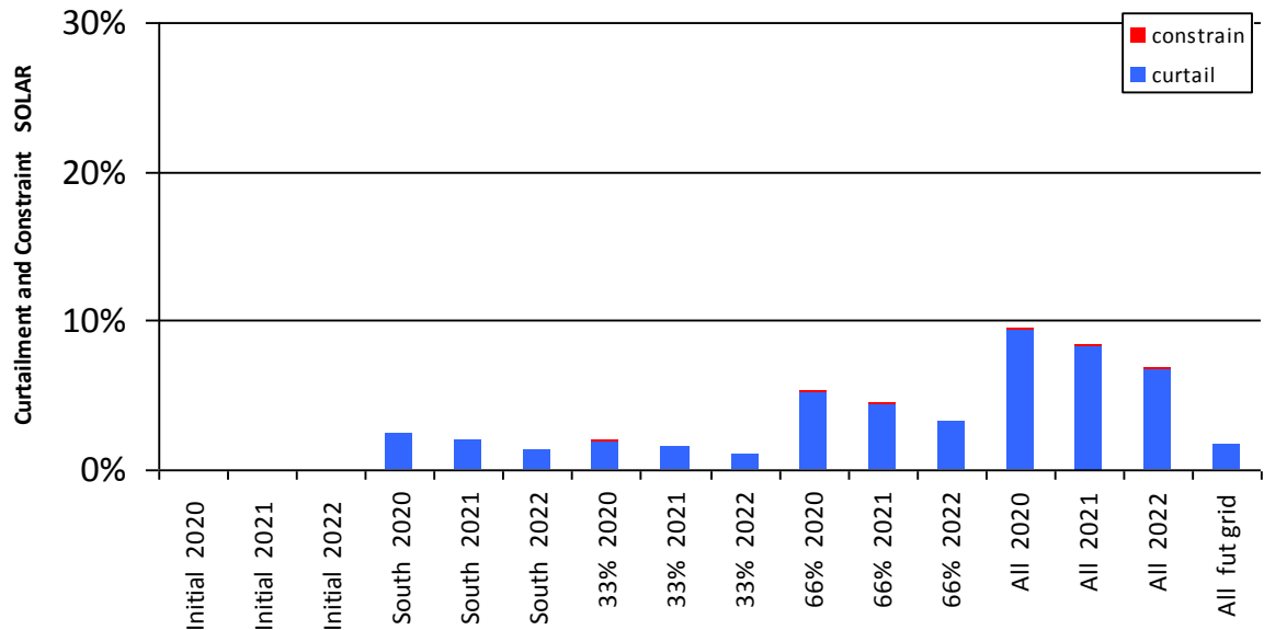
Figure 0-9 Curtailment and Constraint for Charleville Solar
