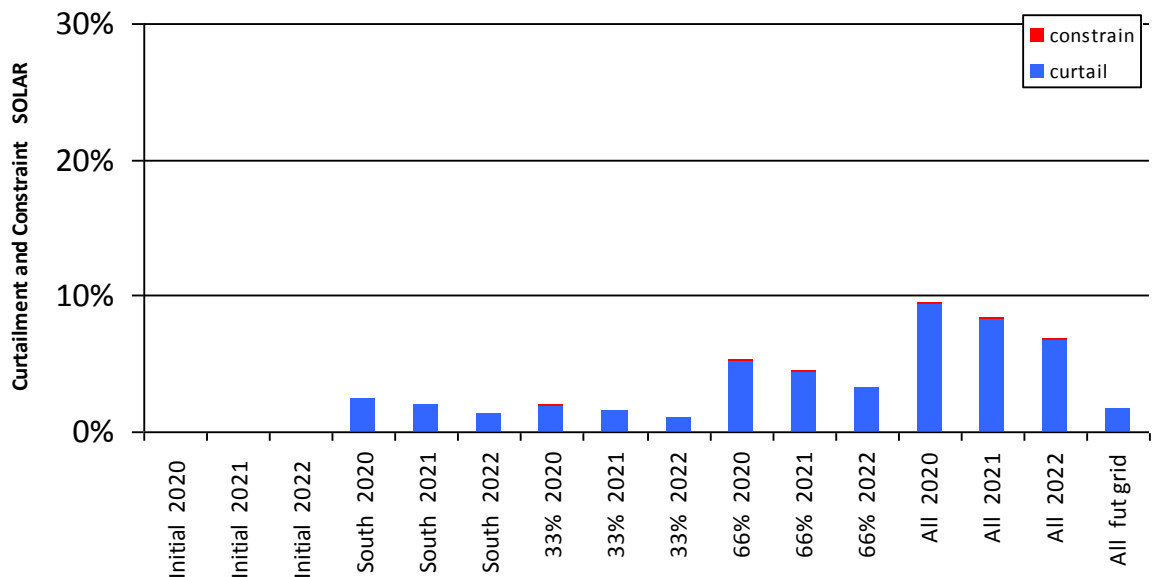
Figure 0-25 Curtailment and Constraint for Drombeg Solar
