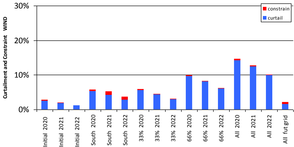
Figure 0-10 Curtailment and Constraint for Charleville Wind
