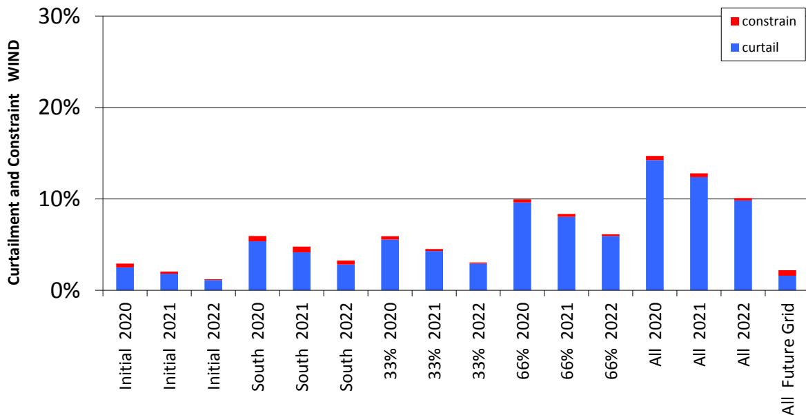
Figure 0-53 Curtailment and Constraint for Rathkeale Wind
