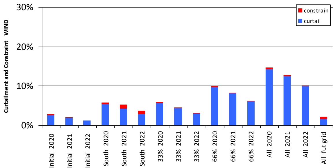
Figure 0-34 Curtailment and Constraint for Glenlara 220 Wind
