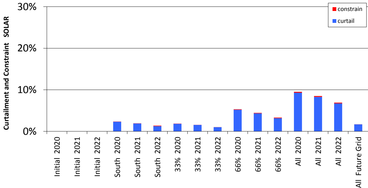
Figure 0-57 Curtailment and Constraint for Toorard Solar
