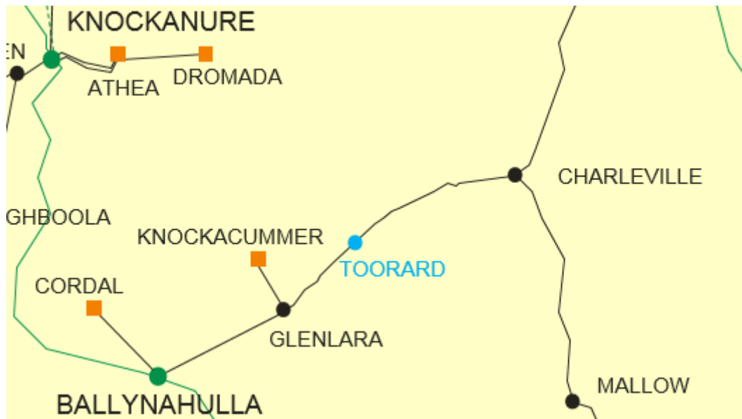
Figure 0-33 Location of Glenlara 220 Node
