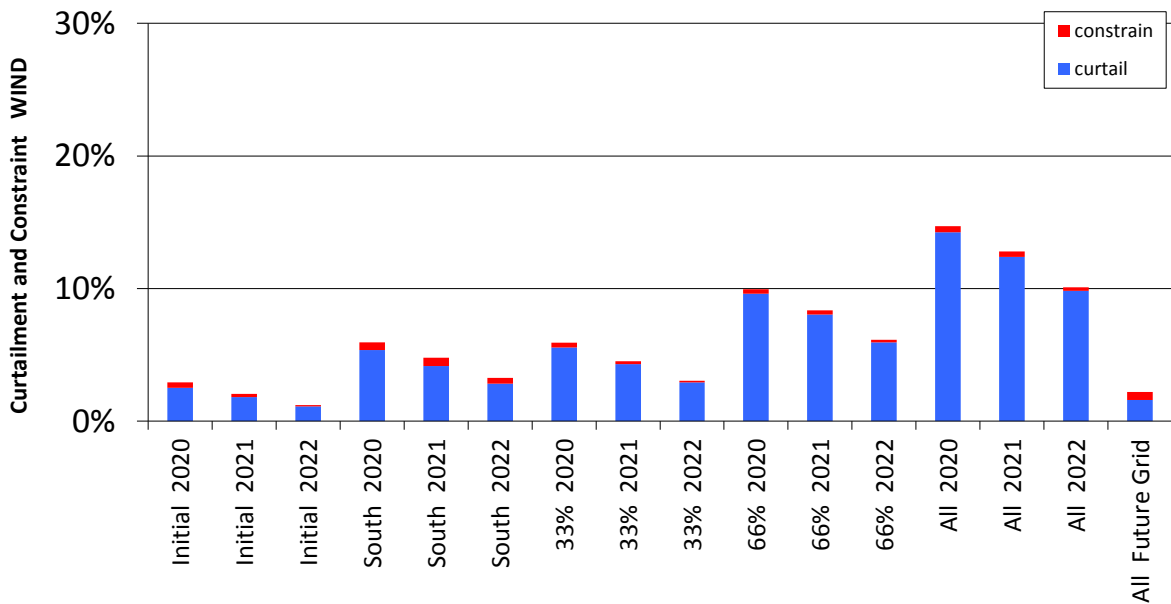
Figure 0-50 Curtailment and Constraint for Oughtragh Wind
