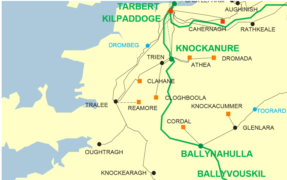
Figure 0-64 Location of Trien 220 kV Node
