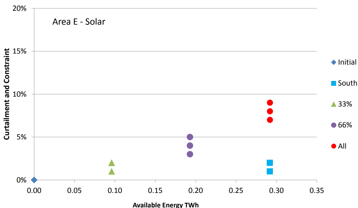
Figure 5-3 Average Curtailment and Constraint Area E Solar
