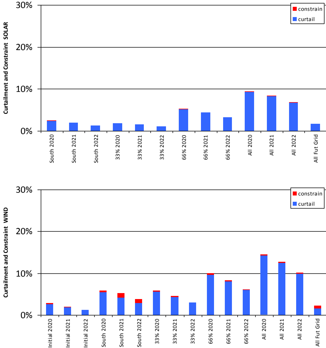
Figure 5-5 Average Curtailment and Constraint in Area E
