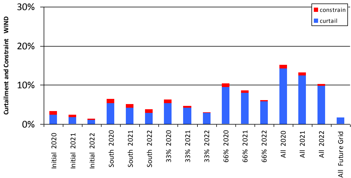
Figure 0-11 Curtailment and Constraint for Cauteen
