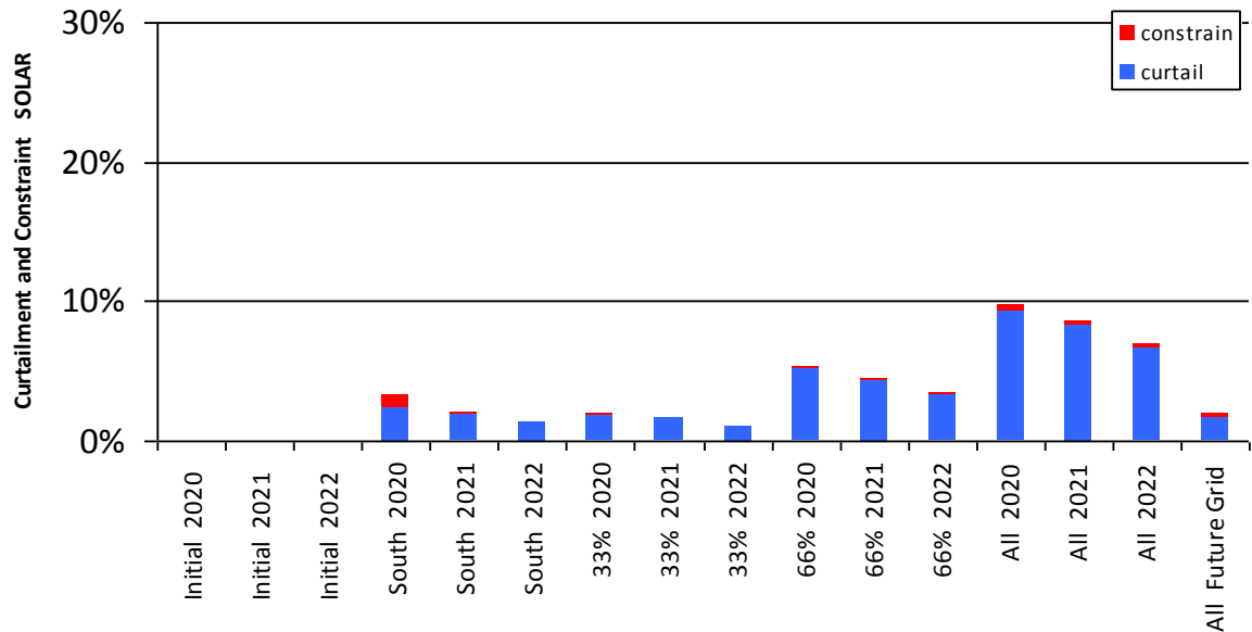
Figure 0-6 Curtailment and Constraint for Barrymore Solar
