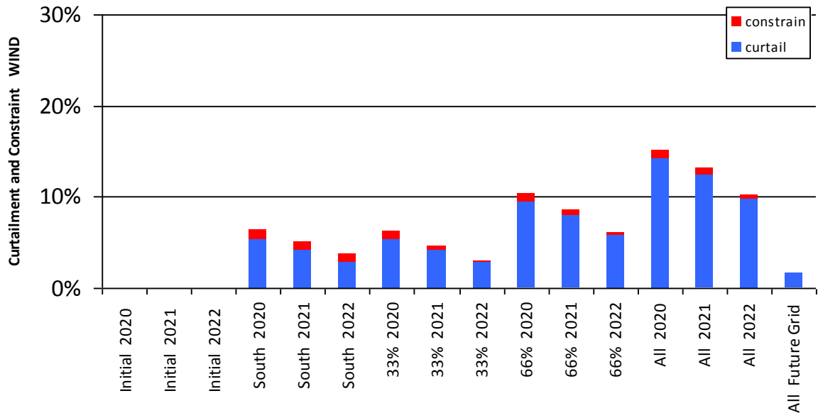
Figure 0-14 Curtailment and Constraint for Doon Wind
