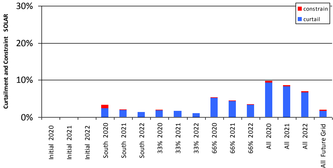
Figure 0-13 Curtailment and Constraint for Doon Solar
