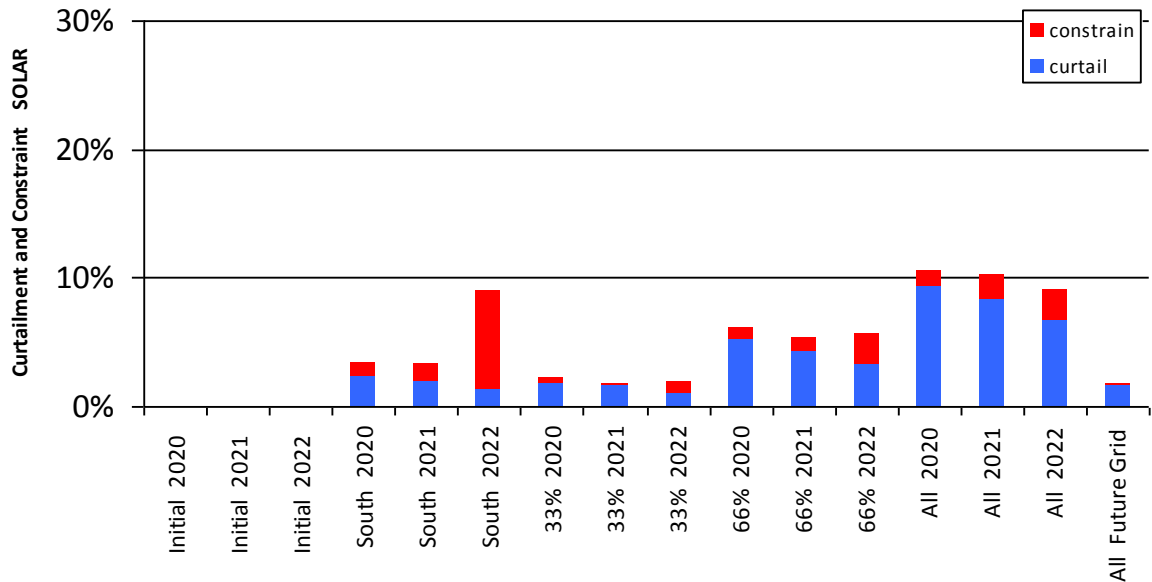
Figure 0-27 Curtailment and Constraint for Nenagh Solar
