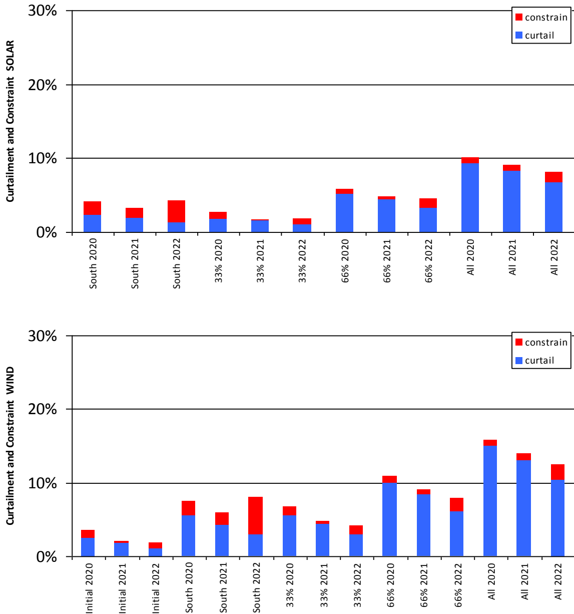
Figure 5-4 Average Curtailment and Constraint in Area H1
