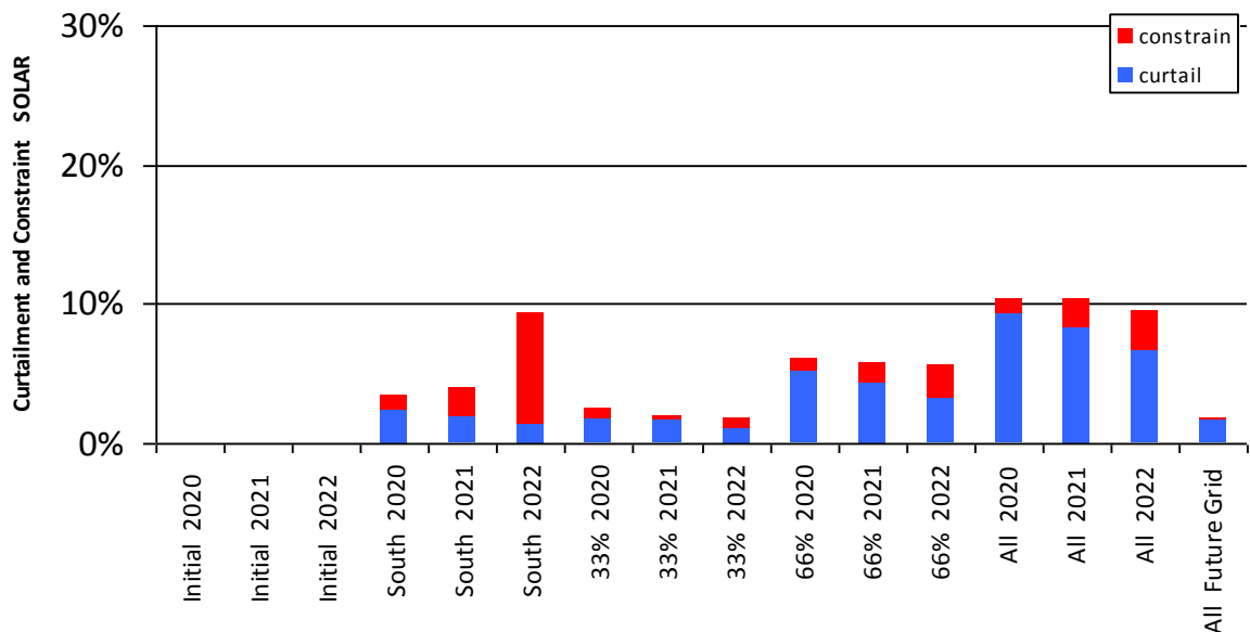
Figure 0-2 Curtailment and Constraint for Ahane Solar
