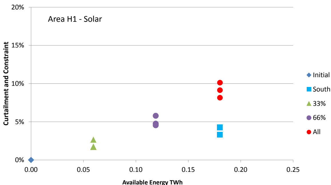
Figure 5-2 Average Curtailment and Constraint Area H1 Solar
