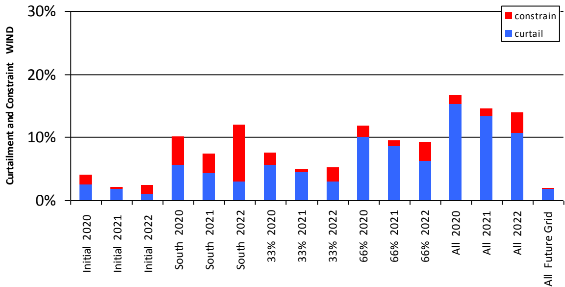
Figure 0-17 Curtailment and Constraint for Ikerrin Wind
