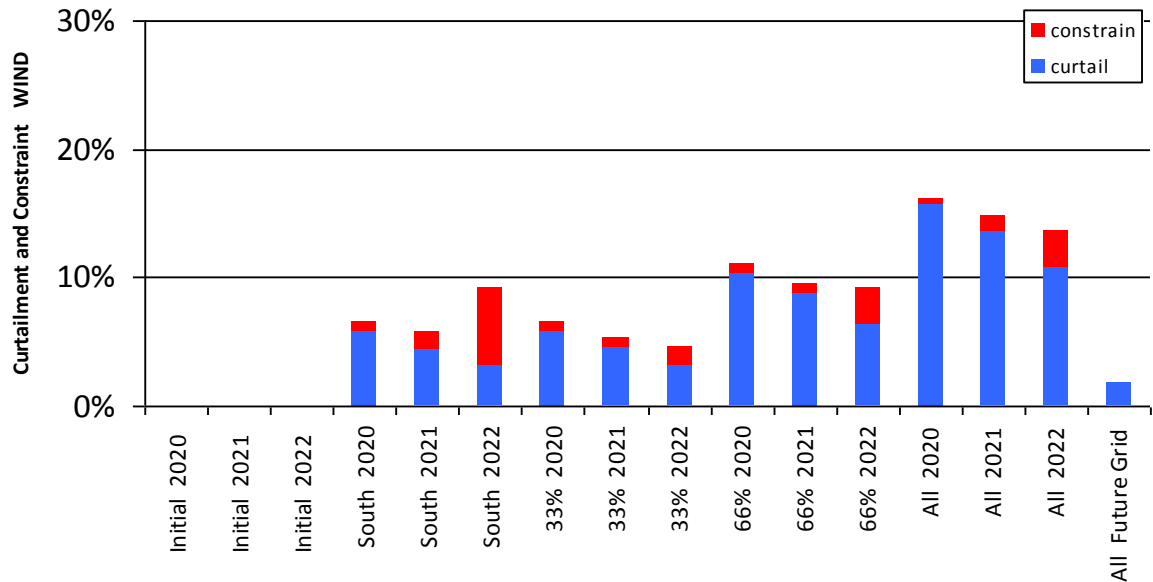
Figure 0-28 Curtailment and Constraint for Nenagh Wind
