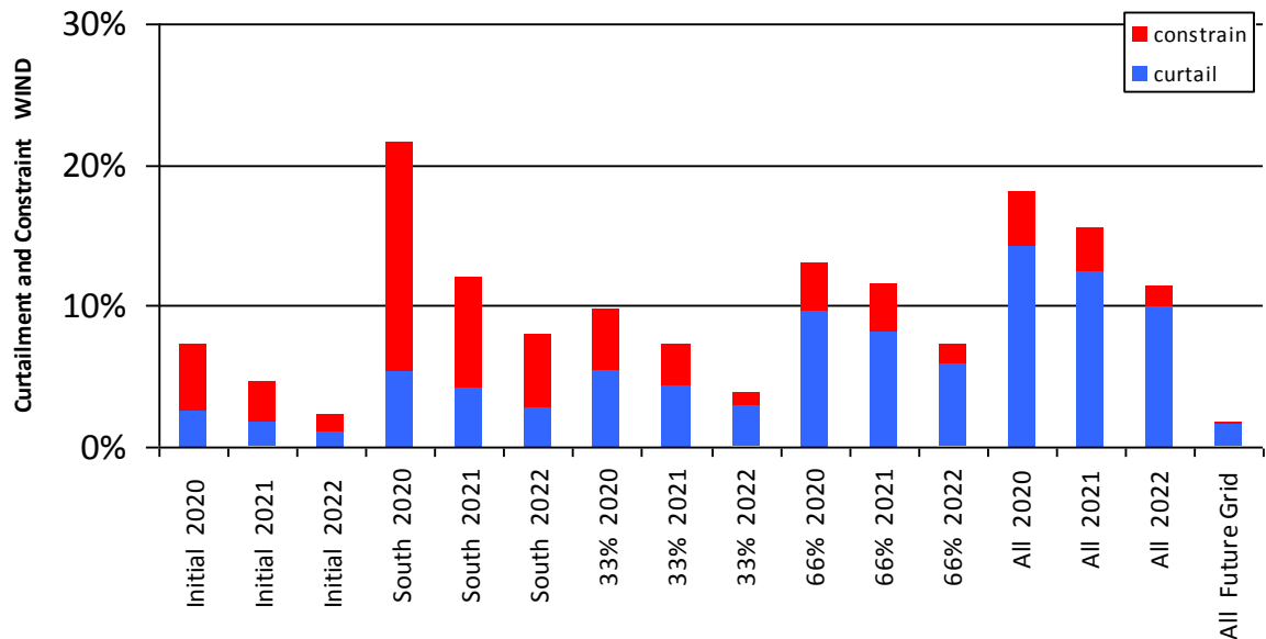
Figure 0-9 Curtailment and Constraint for Ballywater
