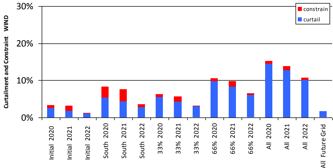
Figure 0-18 Curtailment and Constraint for Castledockrell
