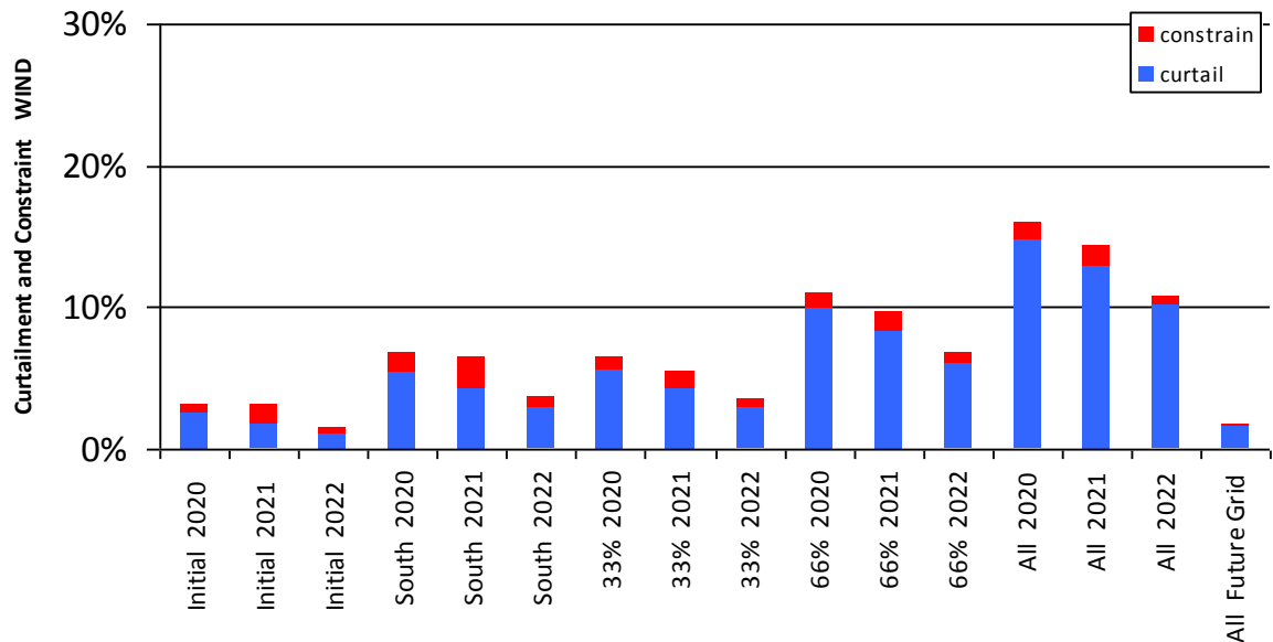
Figure 0-16 Curtailment and Constraint for Carlow Wind
