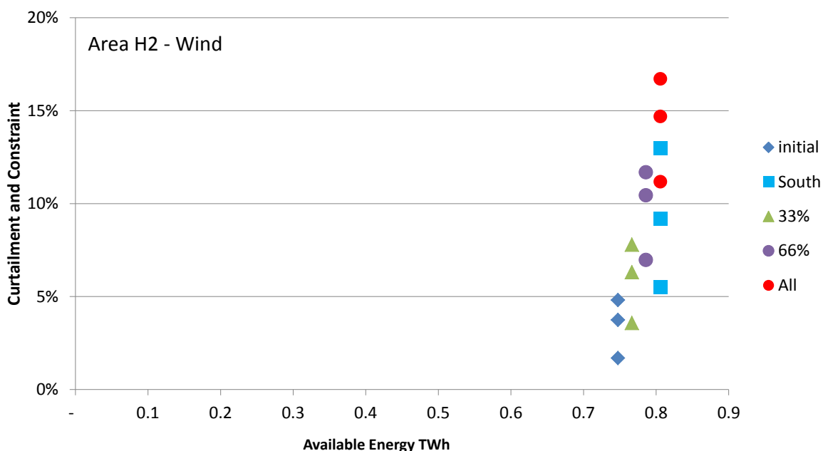
Figure 5-2 Average Curtailment and Constraint Area H2 Wind
