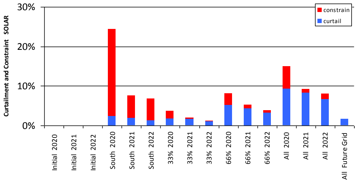
Figure 0-2 Curtailment and Constraint for Arklow Solar
