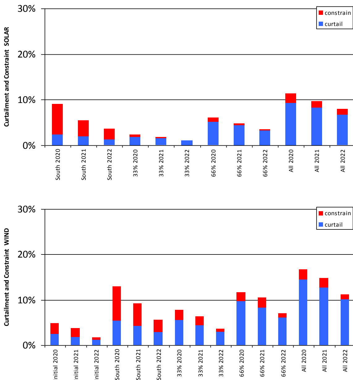
Figure 5-4 Average Curtailment and Constraint in Area H2
