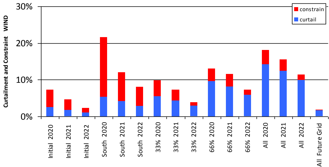
Figure 0-3 Curtailment and Constraint for Arklow Wind
