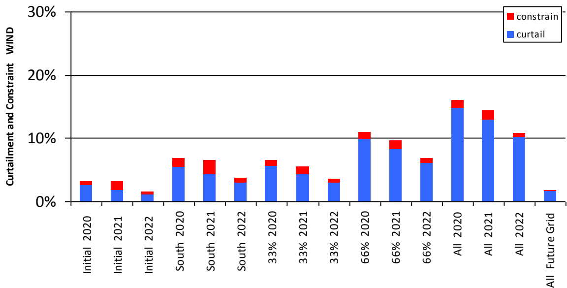
Figure 0-37 Curtailment and Constraint for Waterford Wind
