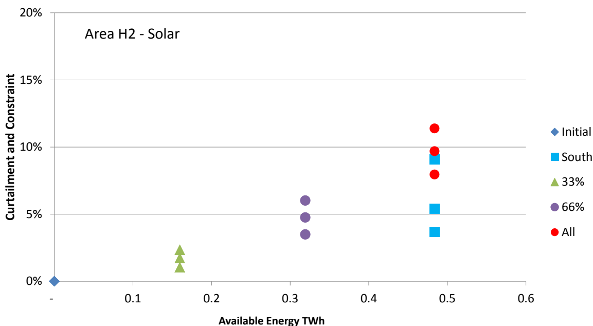
Figure 5-3 Average Curtailment and Constraint Area H2 Solar
