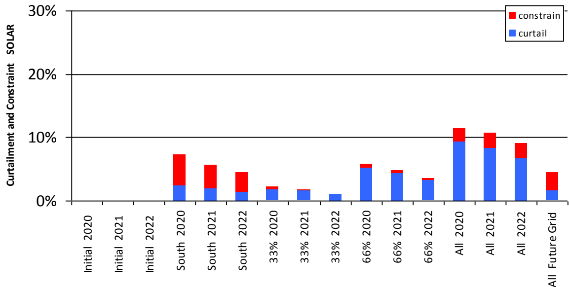
Figure 0-30 Curtailment and Constraint for Rosspile
