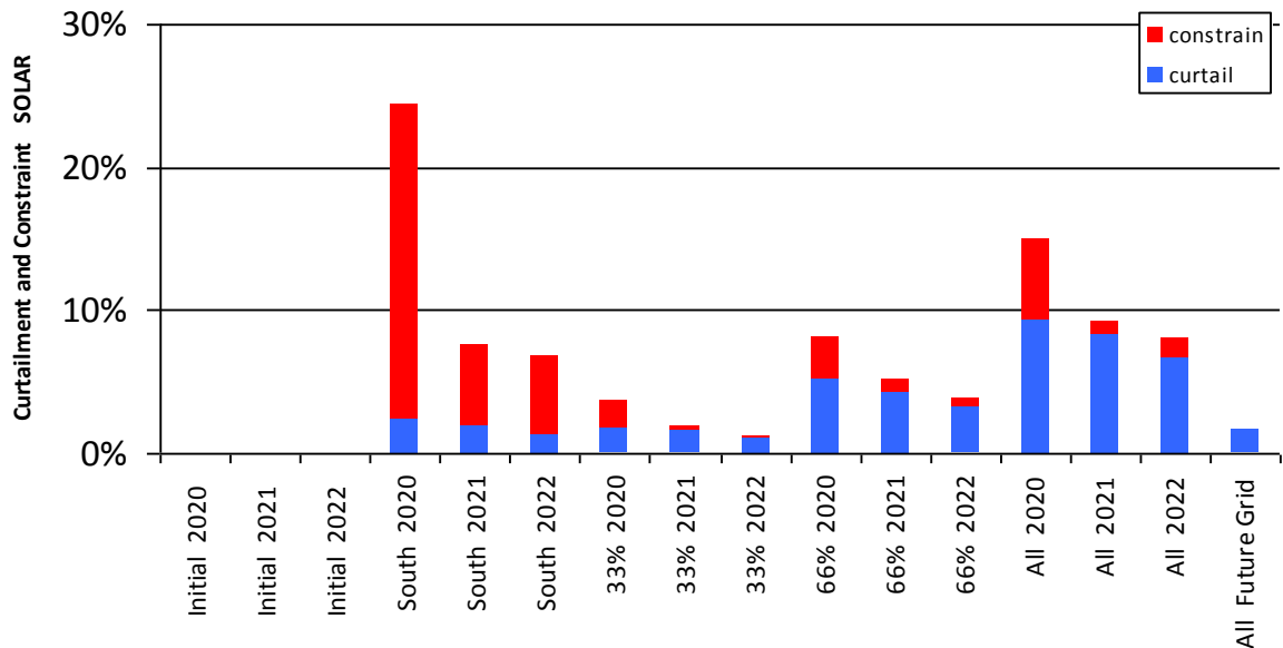
Figure 0-11 Curtailment and Constraint for Banoge
