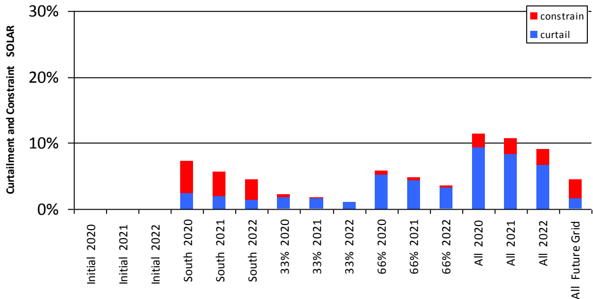
Figure 0-39 Curtailment and Constraint for Wexford Solar
