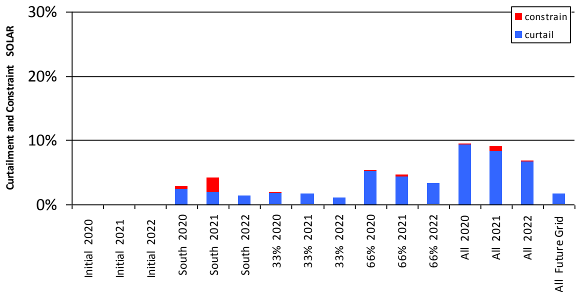
Figure 0-28 Curtailment and Constraint for Kilkenny
