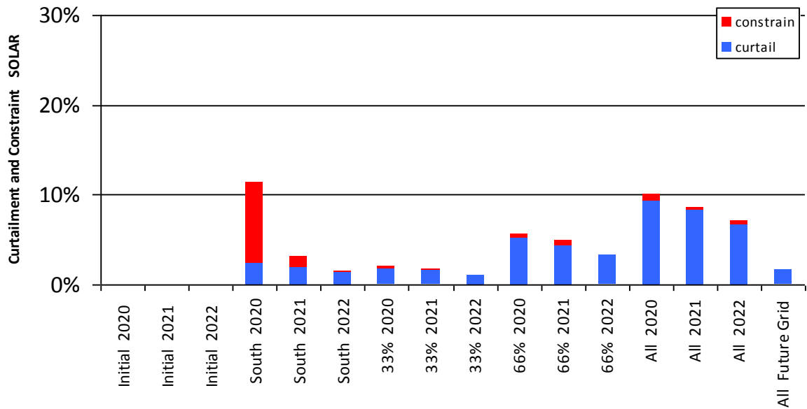
Figure 0-23 Curtailment and Constraint for Crory Solar
