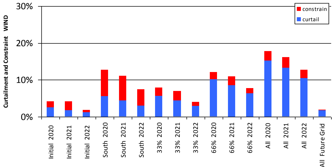
Figure 0-40 Curtailment and Constraint for Wexford Wind
