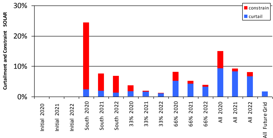
Figure 0-20 Curtailment and Constraint for Crane Solar
