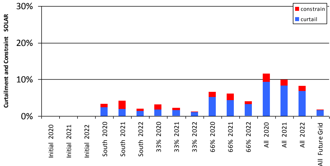
Figure 0-5 Curtailment and Constraint for Ballybeg
