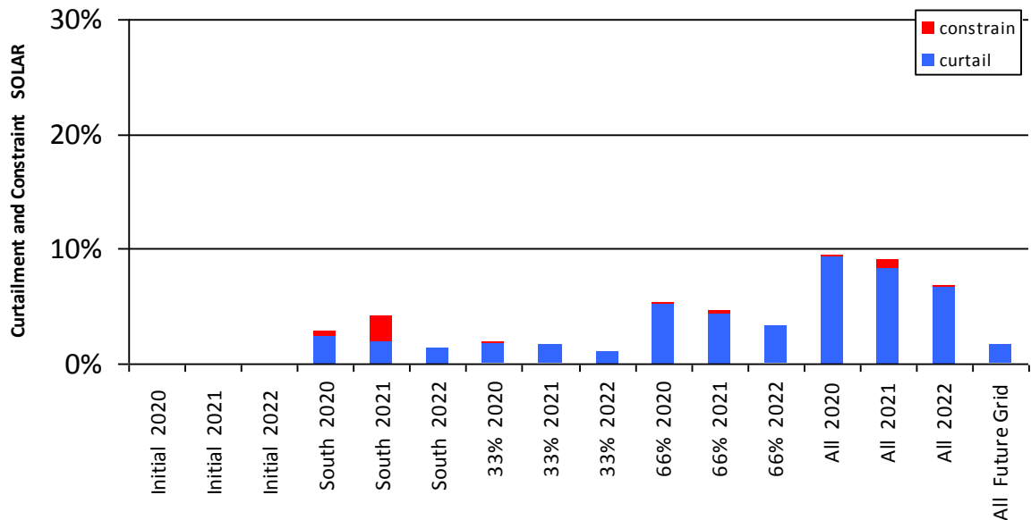
Figure 0-15 Curtailment and Constraint for Carlow Solar
