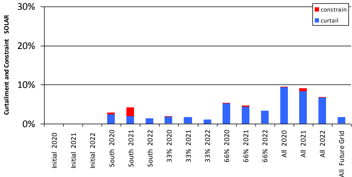
Figure 0-13 Curtailment and Constraint for Bullockhill
