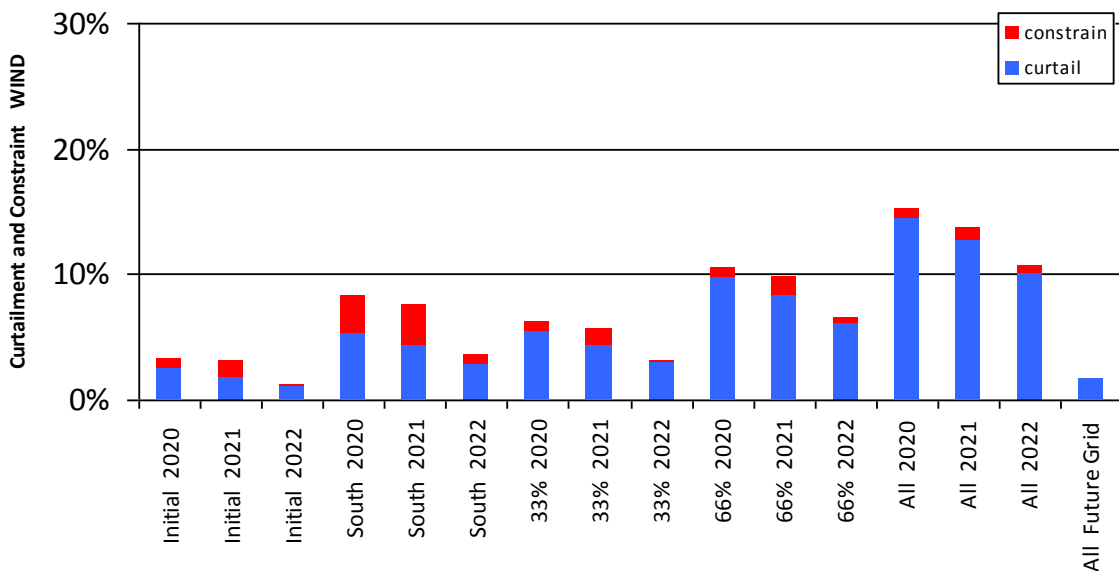
Figure 0-24 Curtailment and Constraint for Crory Wind
