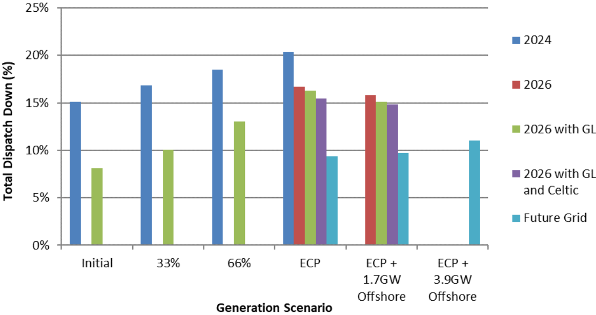
Figure C - 27 Total Dispatch Down for Wind Priority
