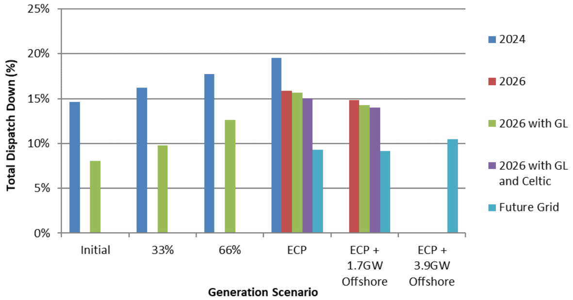
Figure C - 23 Total Dispatch Down for Wind Priority
