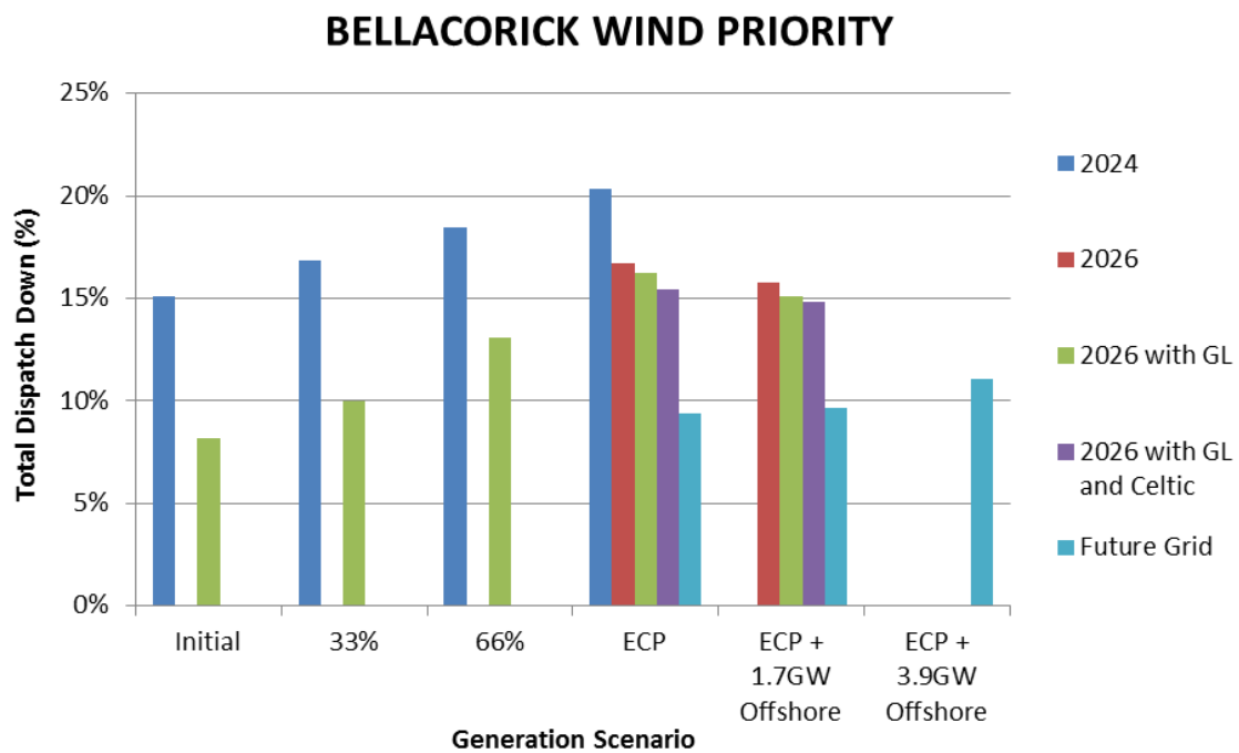
Figure C - 4 Total Dispatch Down for Wind Priority
