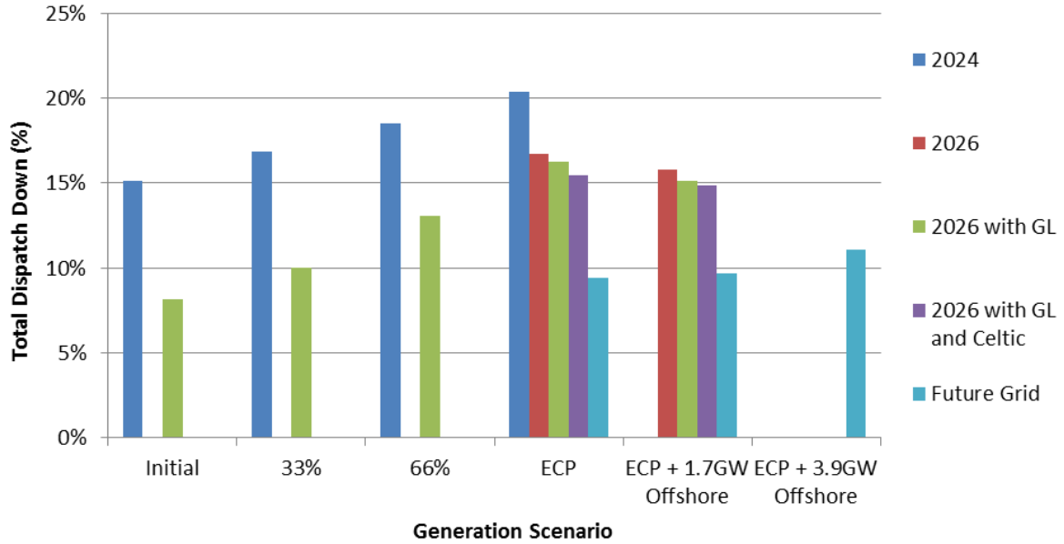
Figure 6-4 Results Wind Priority Area B
