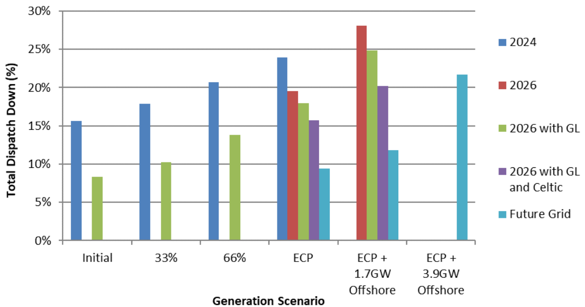
Figure C - 22 Total Dispatch Down for Wind Not Priority
