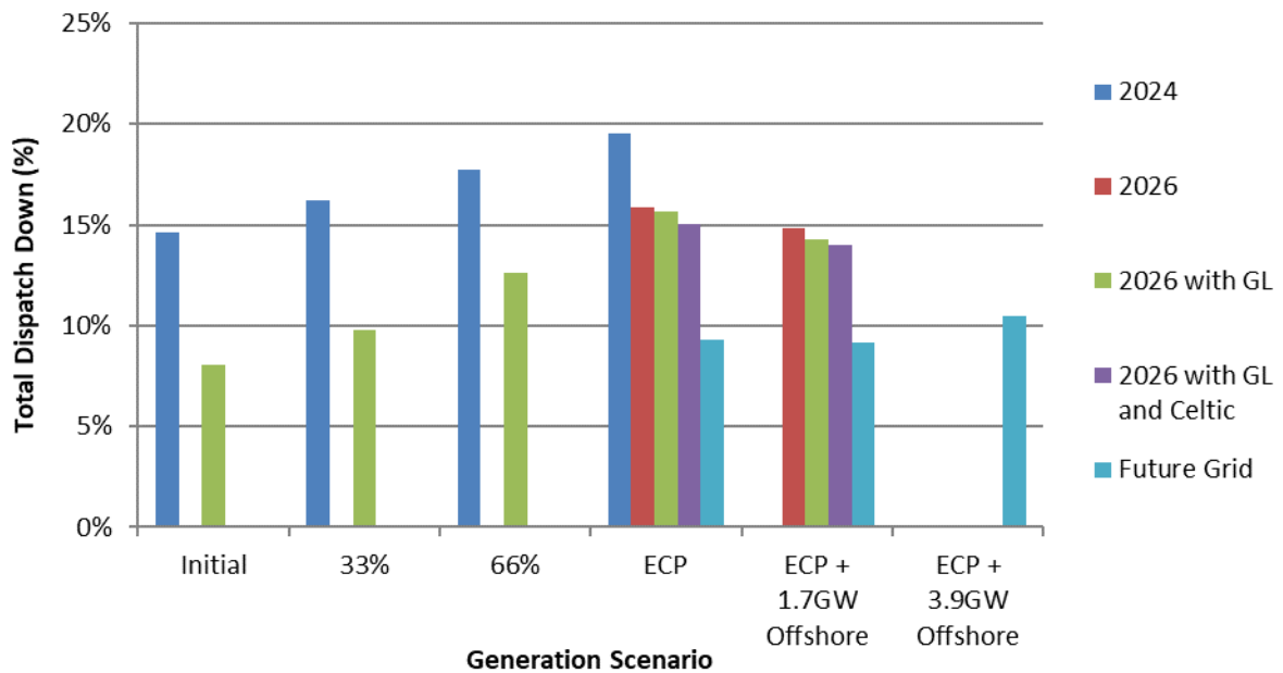
Figure C - 36 Total Dispatch Down for Wind Priority
