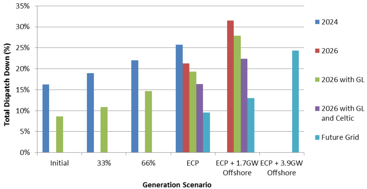
Figure 6-3 Results Wind Not Priority Area B
