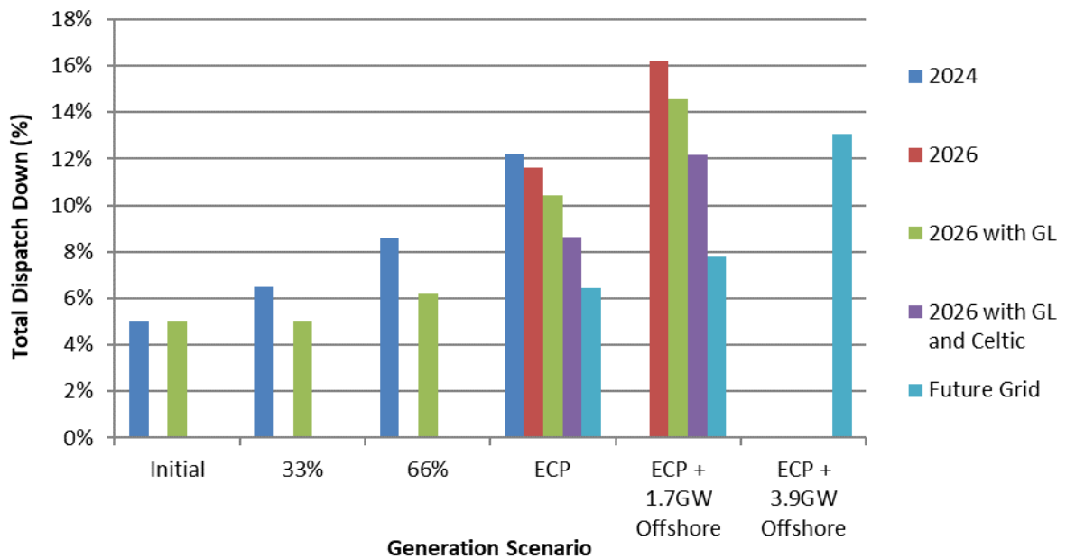
Figure C - 29 Total Dispatch Down for Solar Not Priority
