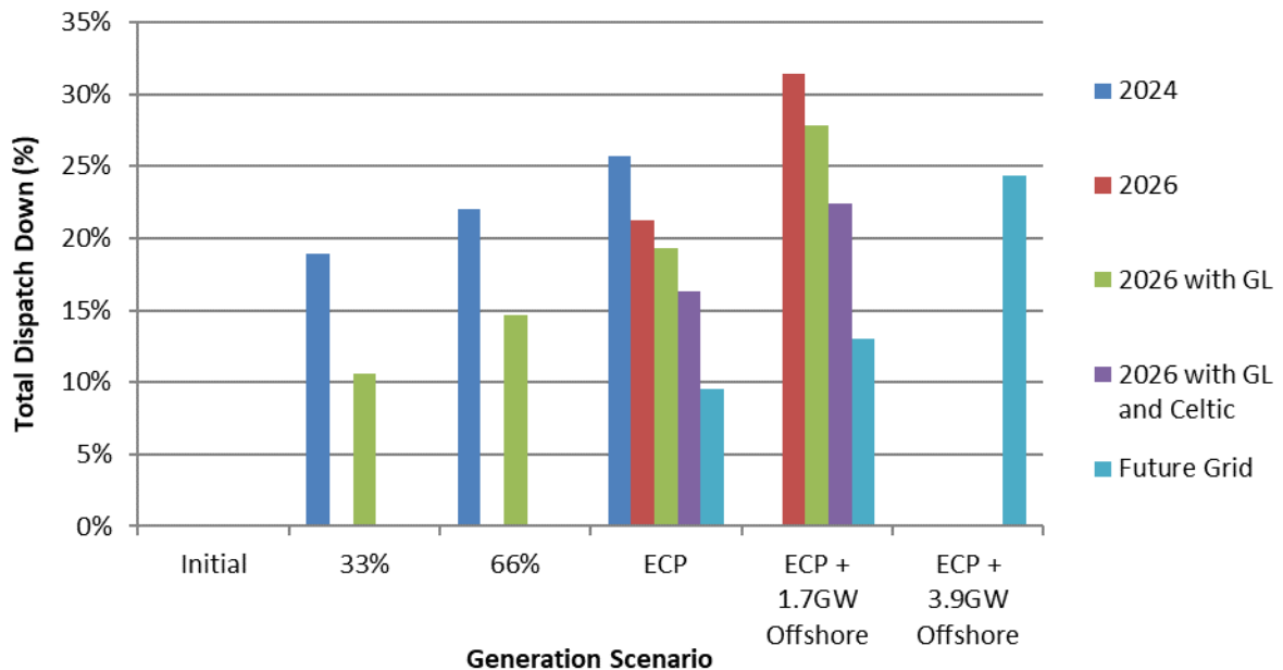
Figure C - 31 Total Dispatch Down for Wind Not Priority
