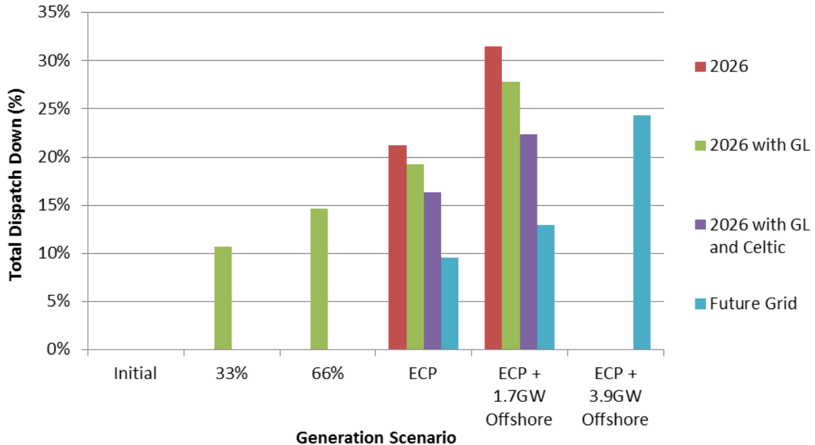
Figure C - 18 Total Dispatch Down for Wind Not Priority
