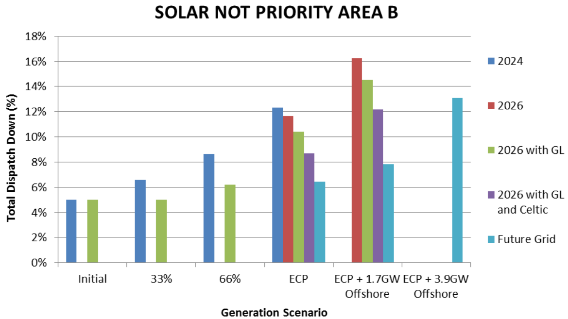
Figure 6-2 Results Solar Not Priority Area B
