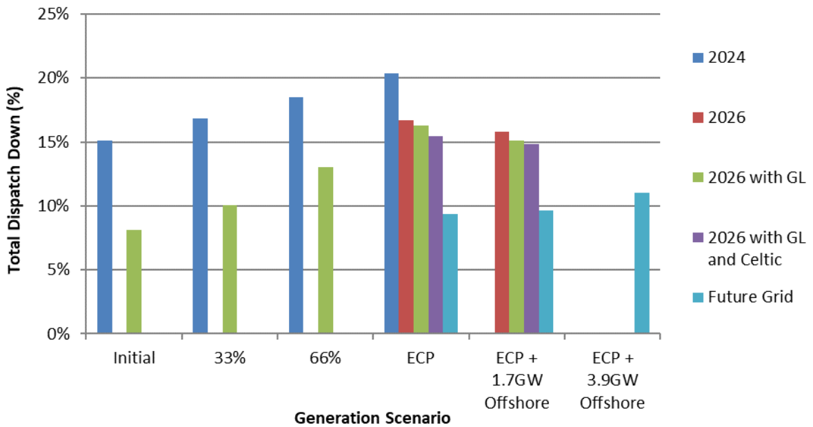
Figure C-13 Total Dispatch Down for Wind Priority
