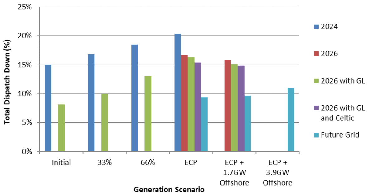
Figure C-25 Total Dispatch Down for Wind Priority
