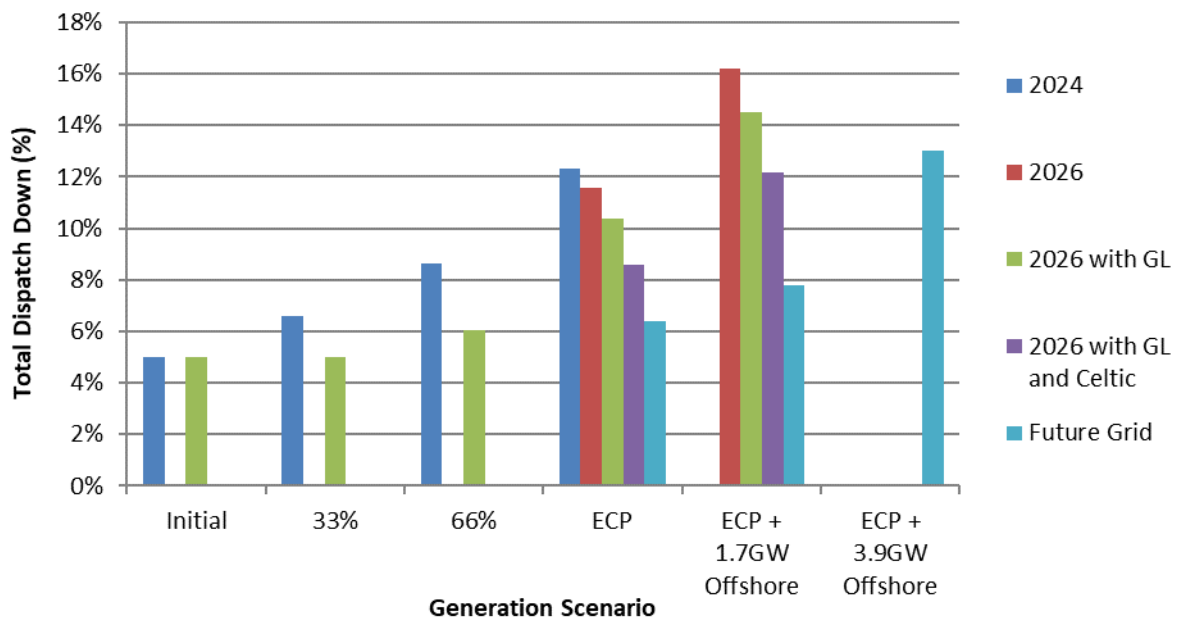
Figure C - 15 Total Dispatch Down for Solar Not Priority
