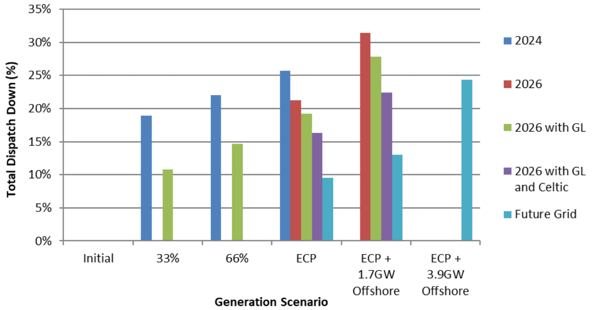
Figure C - 11 Total Dispatch Down for Wind Not Priority
