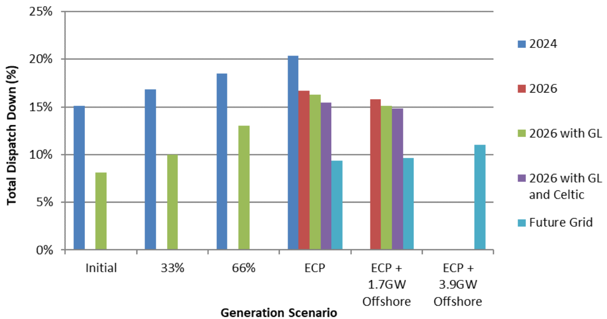
Figure C - 20 Total Dispatch Down for Wind Priority
