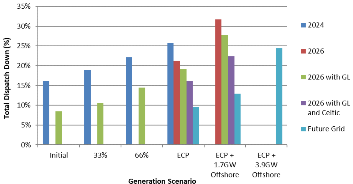
Figure C-9 Total Dispatch Down for Wind Not Priority
