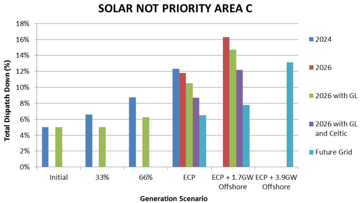
Figure 6-2 Results Solar Not Priority Area C
