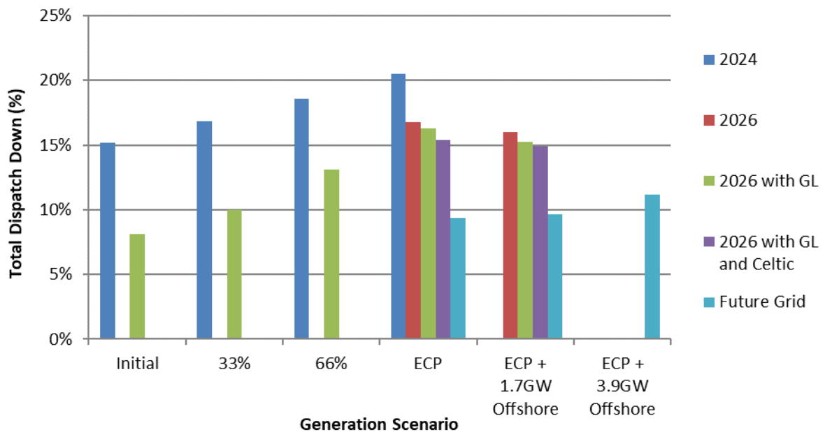
Figure C-7 Total Dispatch Down for Wind Priority
