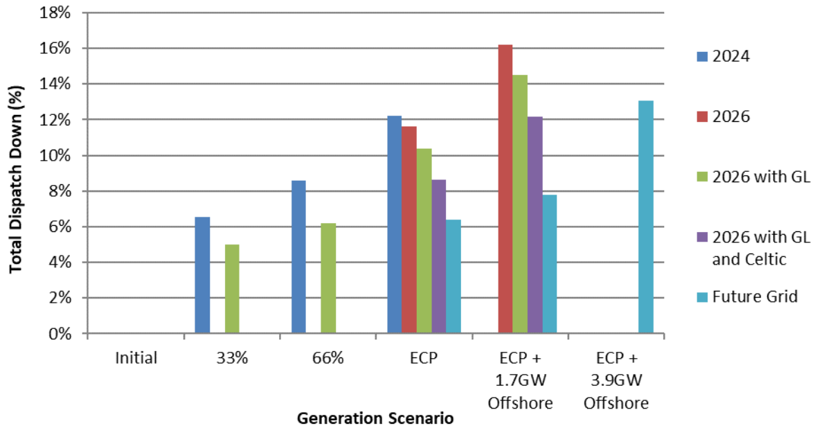
Figure C-14 Total Dispatch Down for Solar Not Priority
