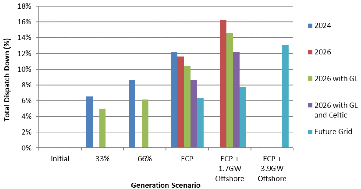
Figure C-11 Total Dispatch Down for Solar Not Priority
