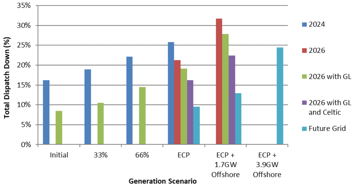
Figure C-12 Total Dispatch Down for Wind Not Priority
