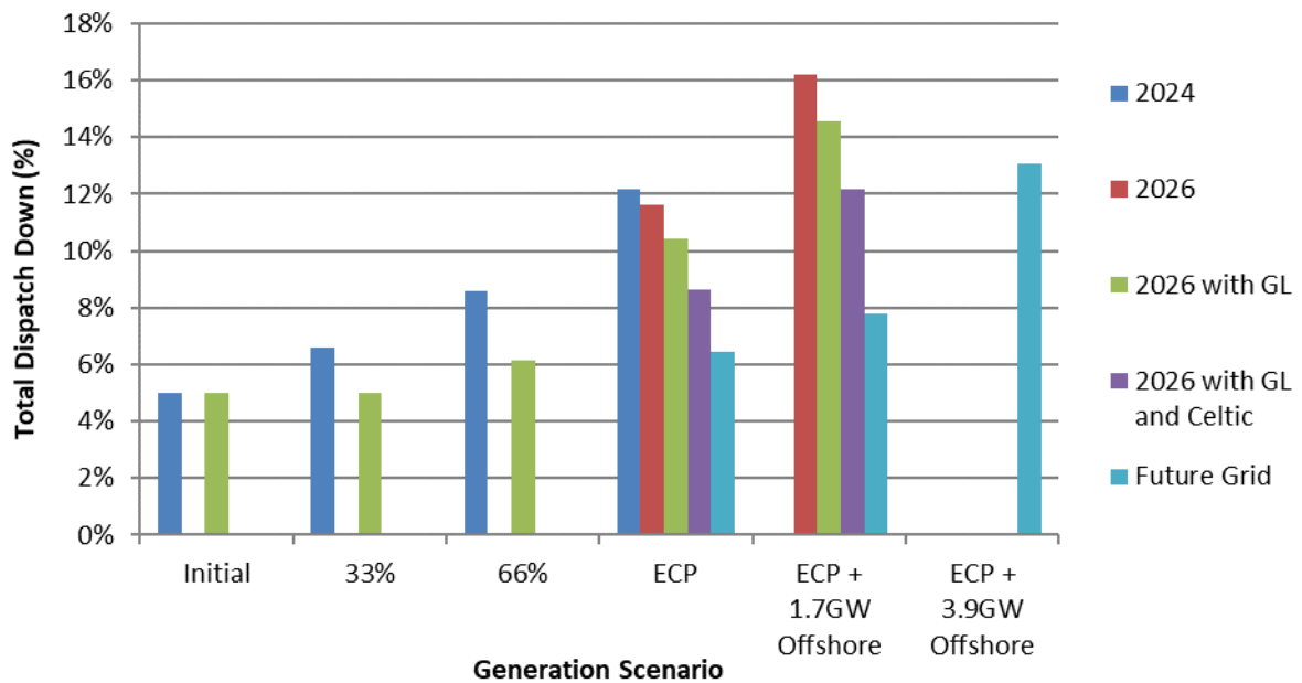
Figure C-17 Total Dispatch Down for Solar Not Priority
