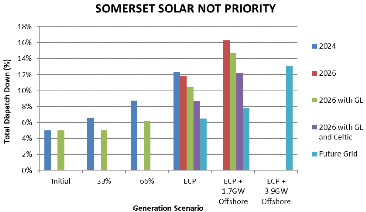
Figure C-25 Total Dispatch Down for Solar Not Priority
