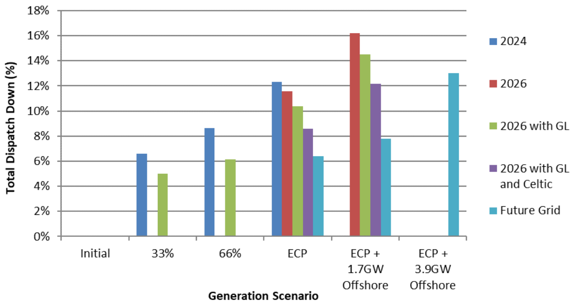
Figure C-3 Total Dispatch Down for Solar Not Priority
