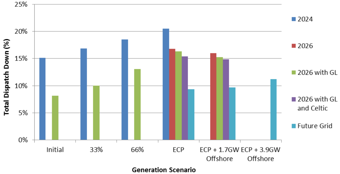
Figure 6-4 Results Wind Priority Area C
