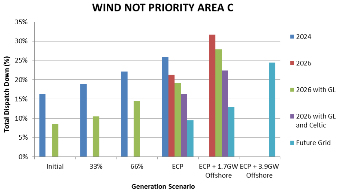
Figure 6-3 Results Wind Not Priority Area C
