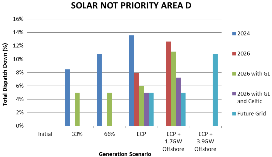
Figure 6-2 Results Solar Not Priority Area D
