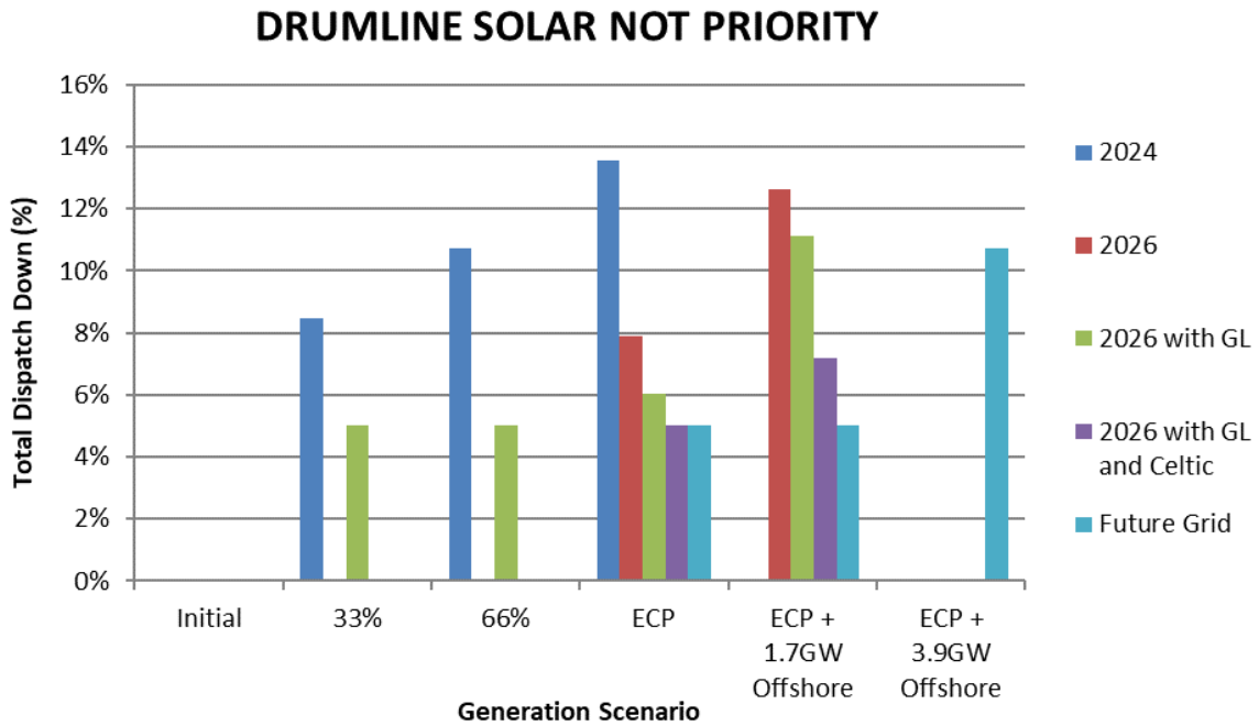
Figure C-11 Total Dispatch Down for Drumline Solar Not Priority
