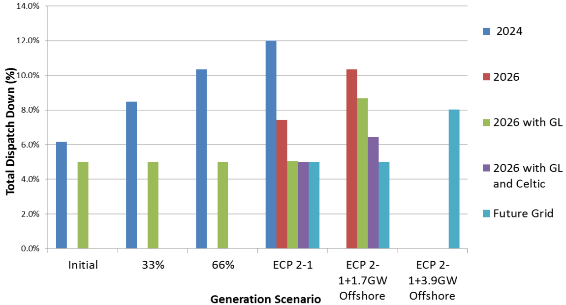
Figure 6-4 Results Wind Priority Area D
