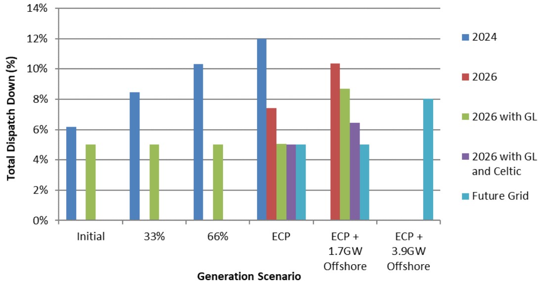
Figure C-4 Total Dispatch Down for Ardnacrusha Wind Priority
