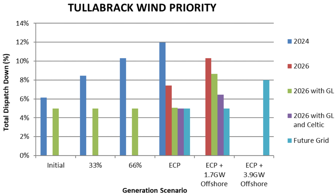
Figure C-15 Total Dispatch Down for Tullabrack Wind Priority
