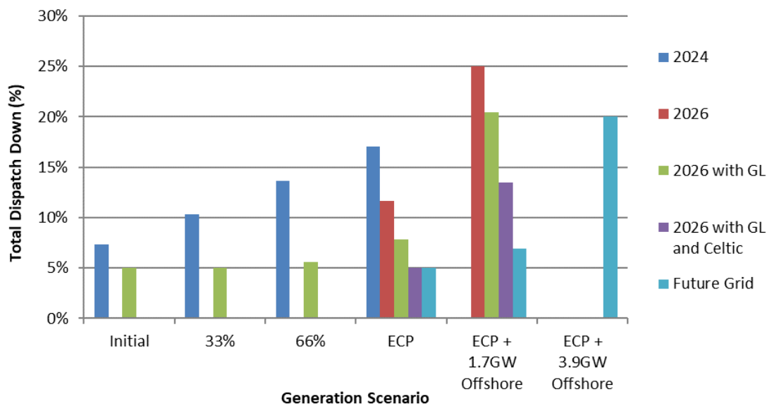
Figure C-6 Total Dispatch Down for Booltiagh Wind Not Priority
