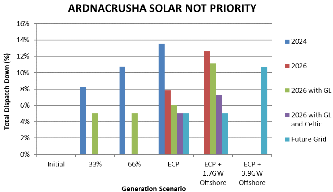
Figure C-3 Total Dispatch Down for Ardnacrusha Solar Not Priority
