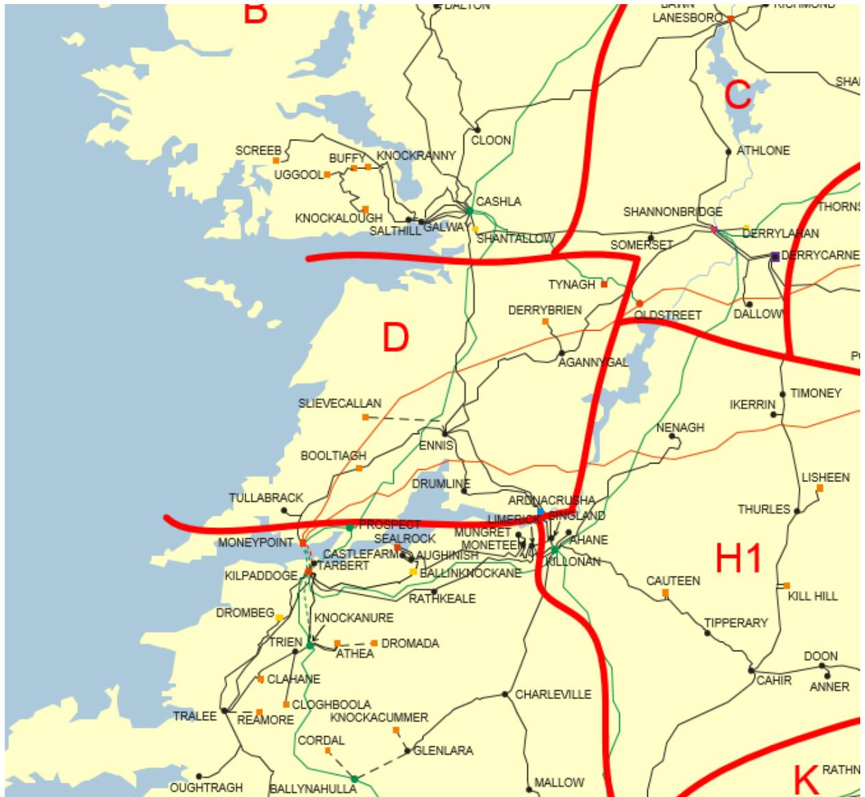
Figure 6-1 Network Map for Area D
