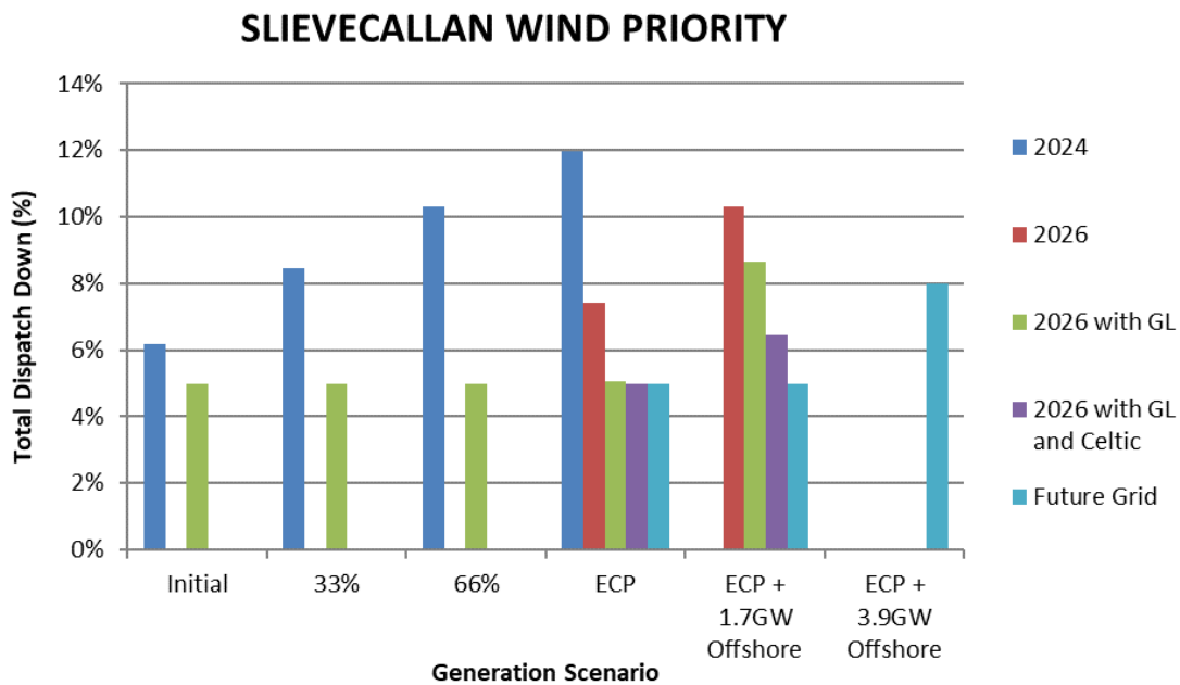
Figure C-13 Total Dispatch Down for Slievecallan Wind Priority
