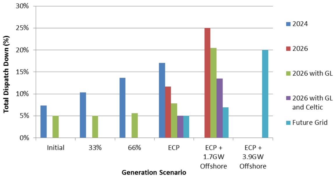
Figure 6-3 Results Wind Not Priority Area D
