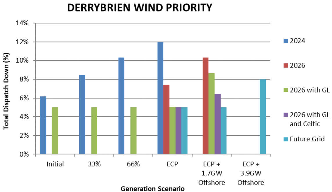
Figure C-9 Total Dispatch Down for Derrybrien Wind Priority
