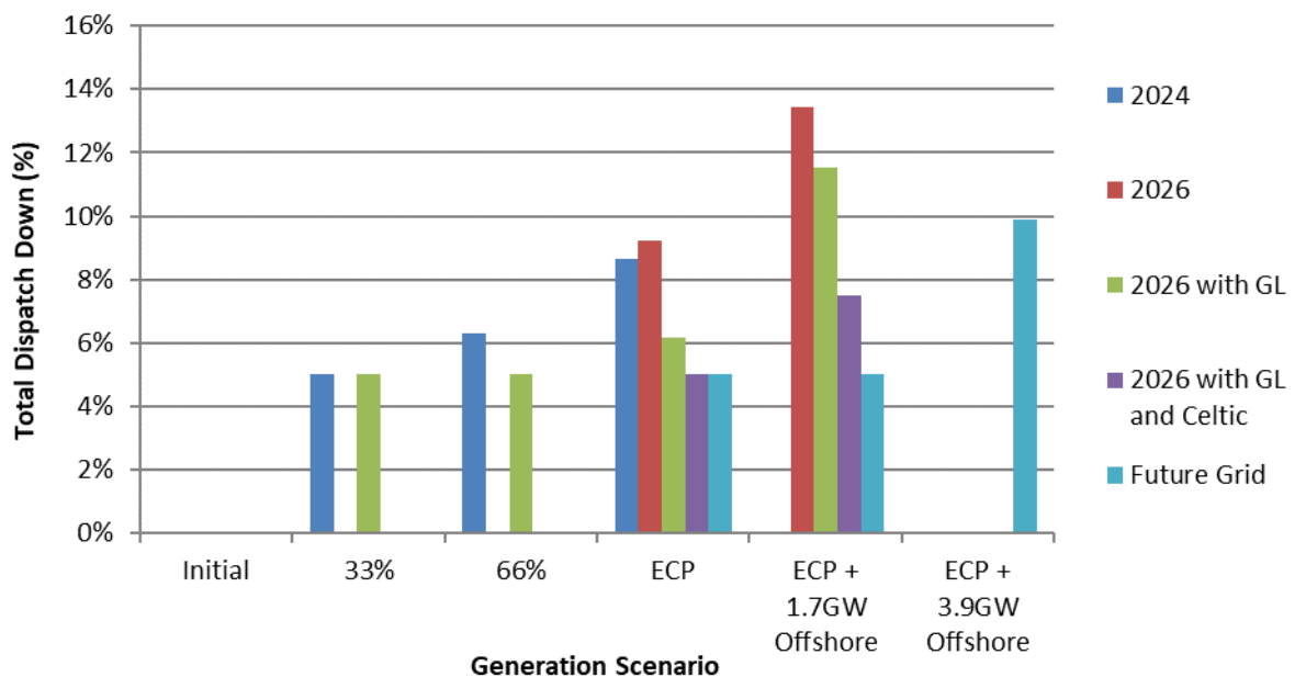
Figure C-21 Total Dispatch Down for Solar Not Priority
