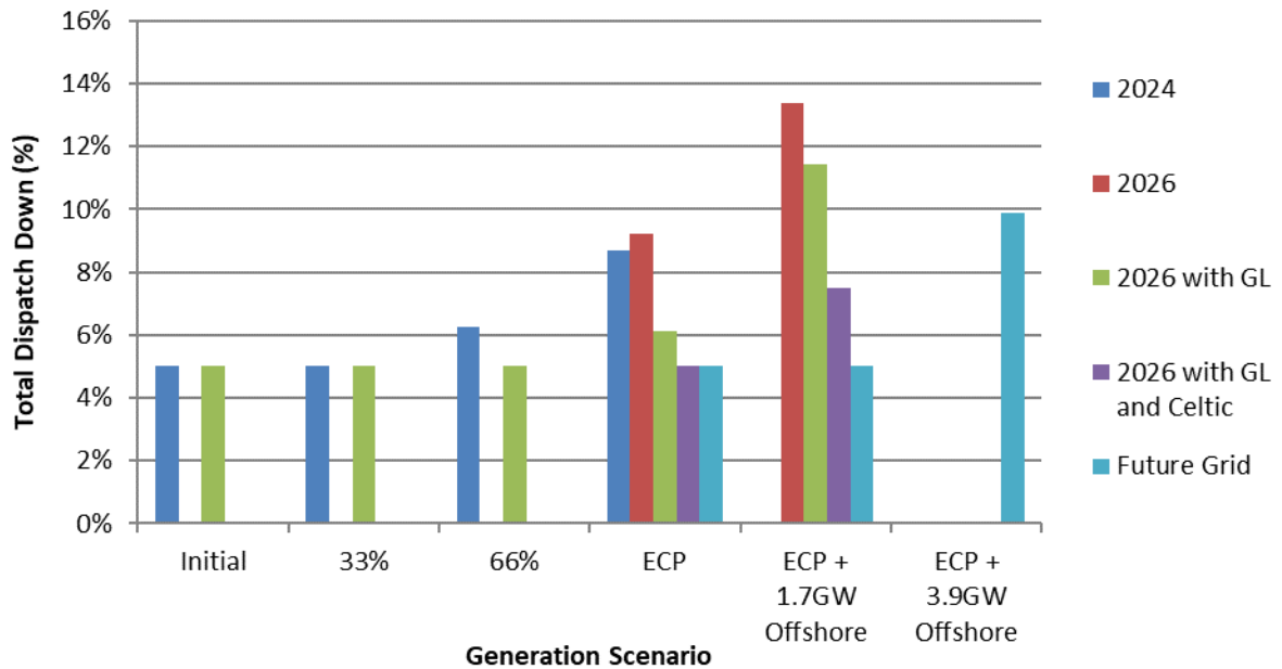
Figure C-5 Total Dispatch Down for Solar Not Priority
