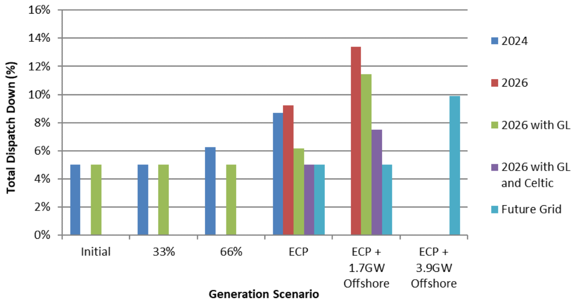
Figure C-16 Total Dispatch Down for Solar Not Priority
