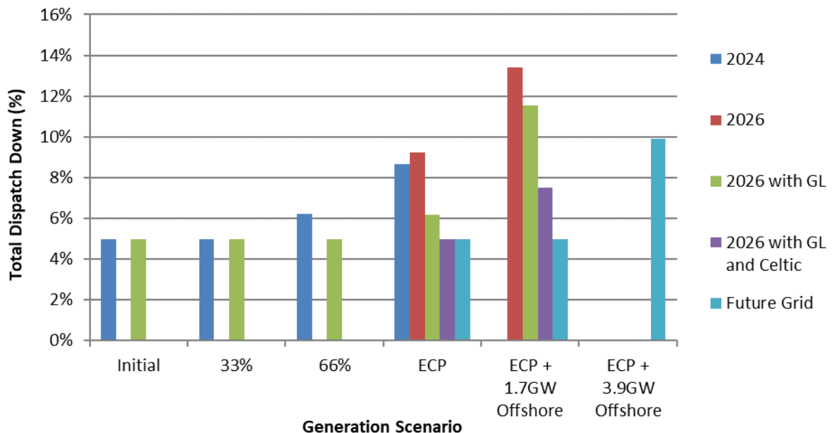
Figure C-64 Total Dispatch Down for Solar Not Priority
