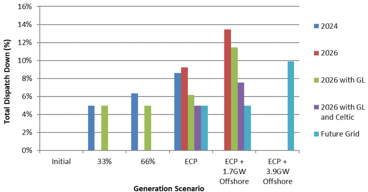
Figure C-49 Total Dispatch Down for Solar Not Priority
