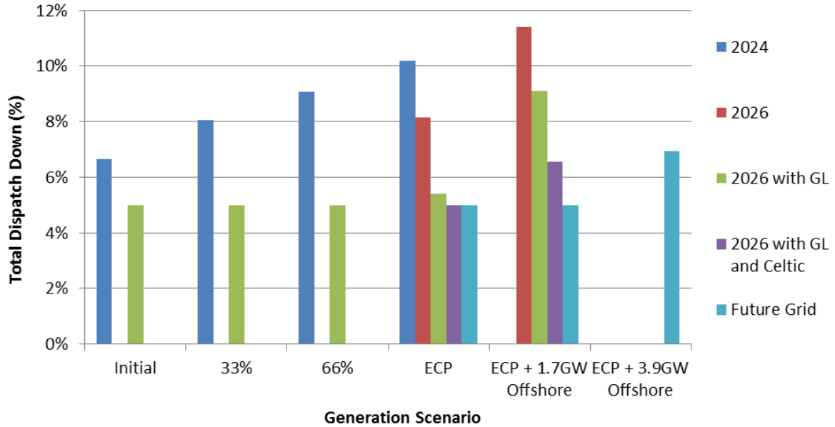
Figure 6-4 Results Wind Priority in Area E
