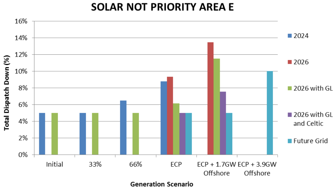
Figure 6-2 Results Solar Not Priority Area E
