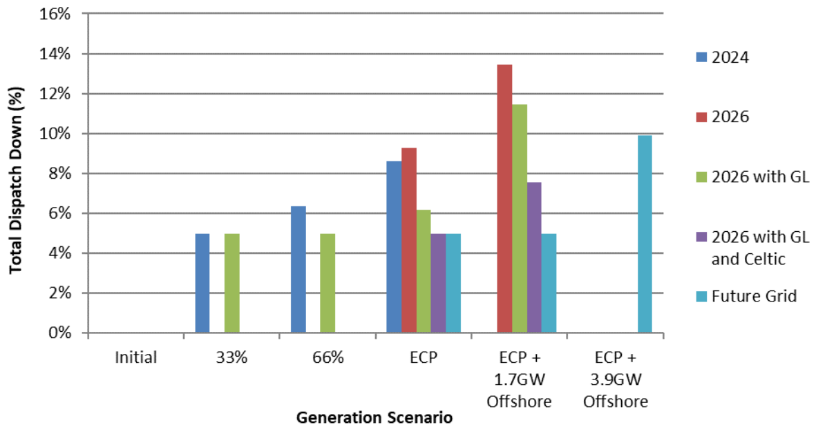
Figure C-46 Total Dispatch Down for Solar Not Priority
