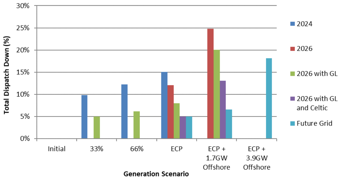
Figure C-61 Total Dispatch Down for Wind Not Priority
