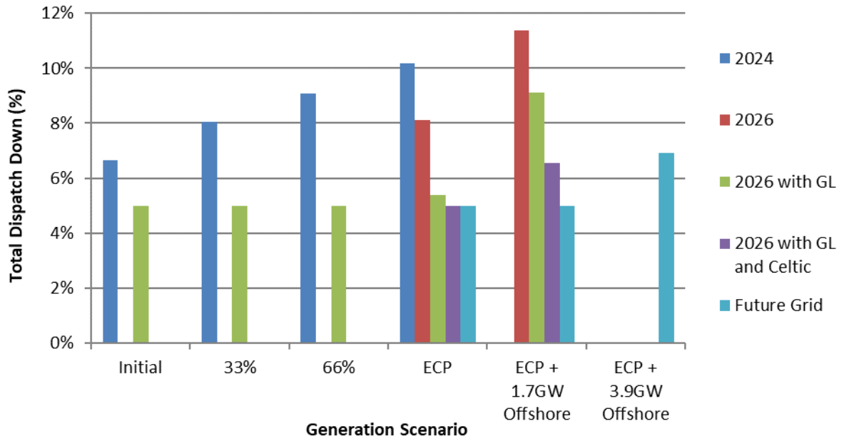
Figure C-22 Total Dispatch Down for Wind Priority
