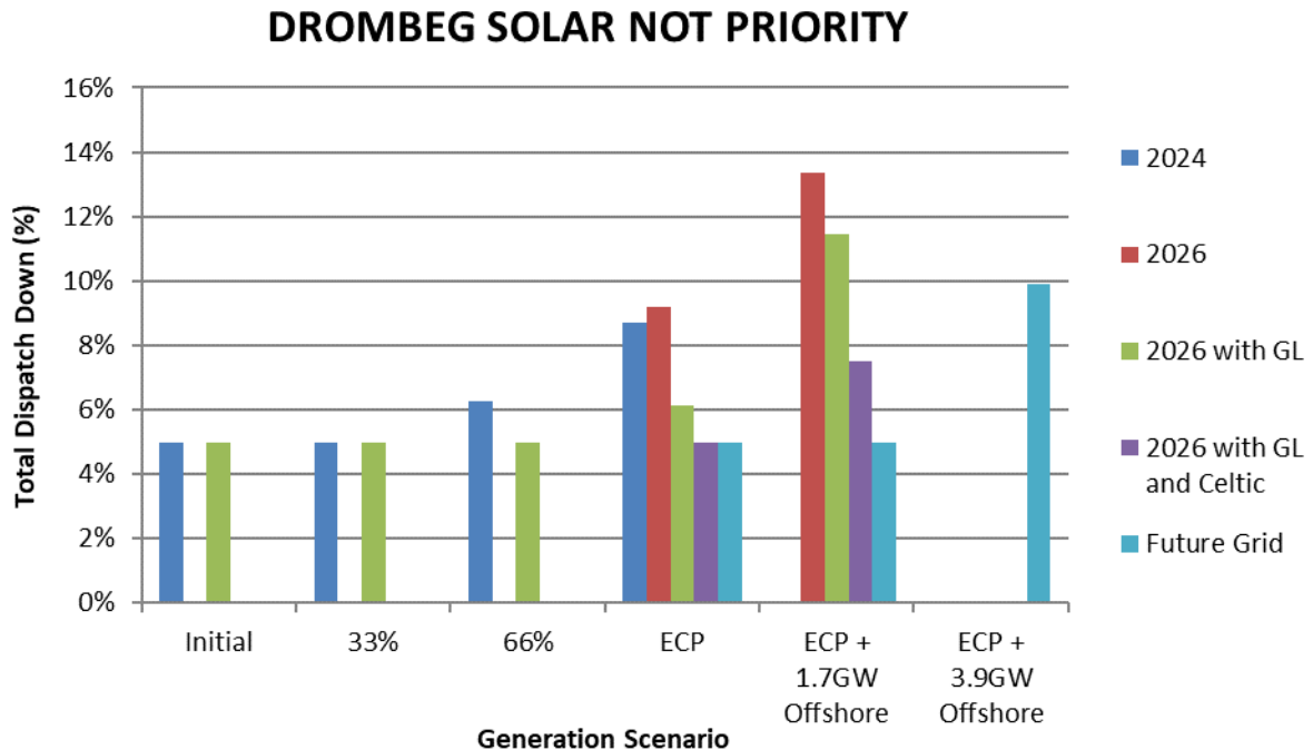
Figure C-30 Total Dispatch Down for Solar Not Priority
