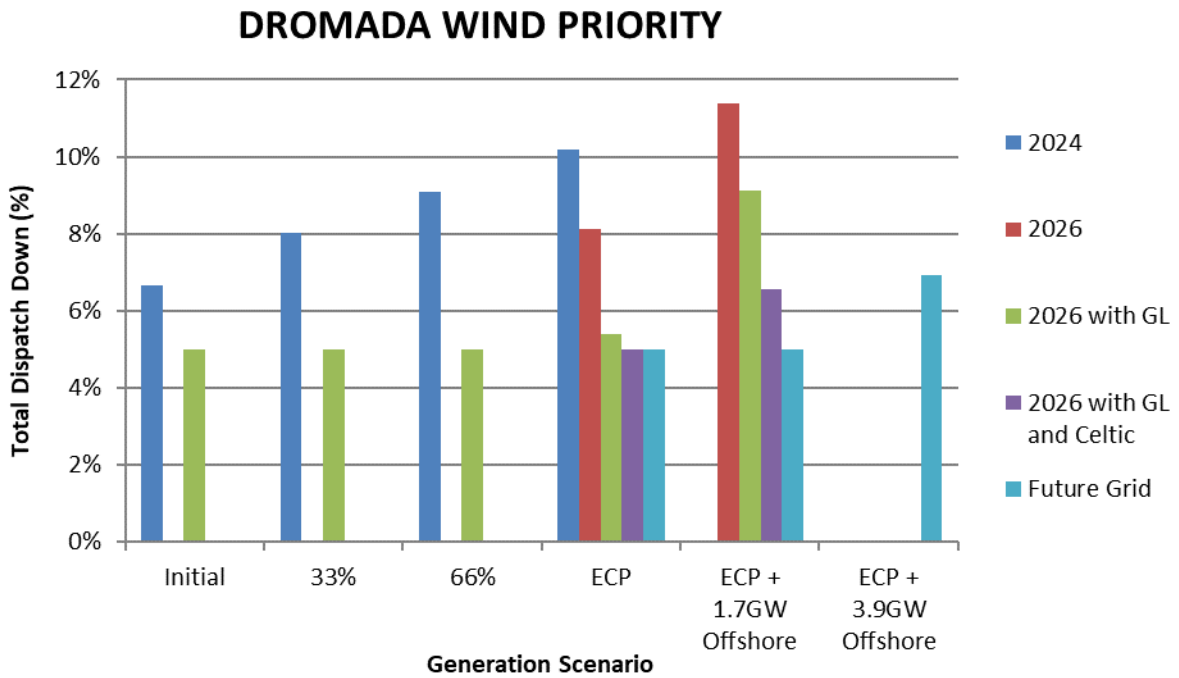
Figure C-28 Total Dispatch Down for Wind Priority
