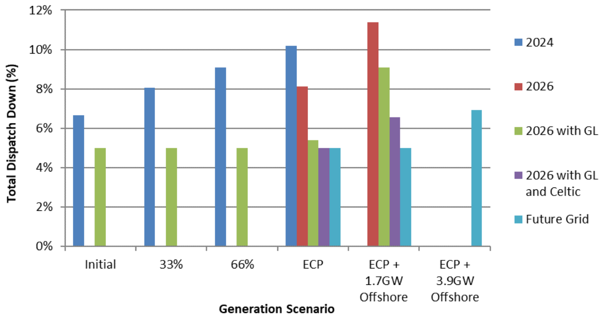
Figure C-24 Total Dispatch Down for Wind Priority
