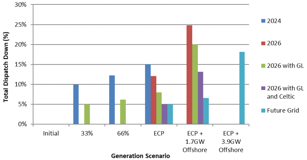
Figure C-50 Total Dispatch Down for Wind Not Priority
