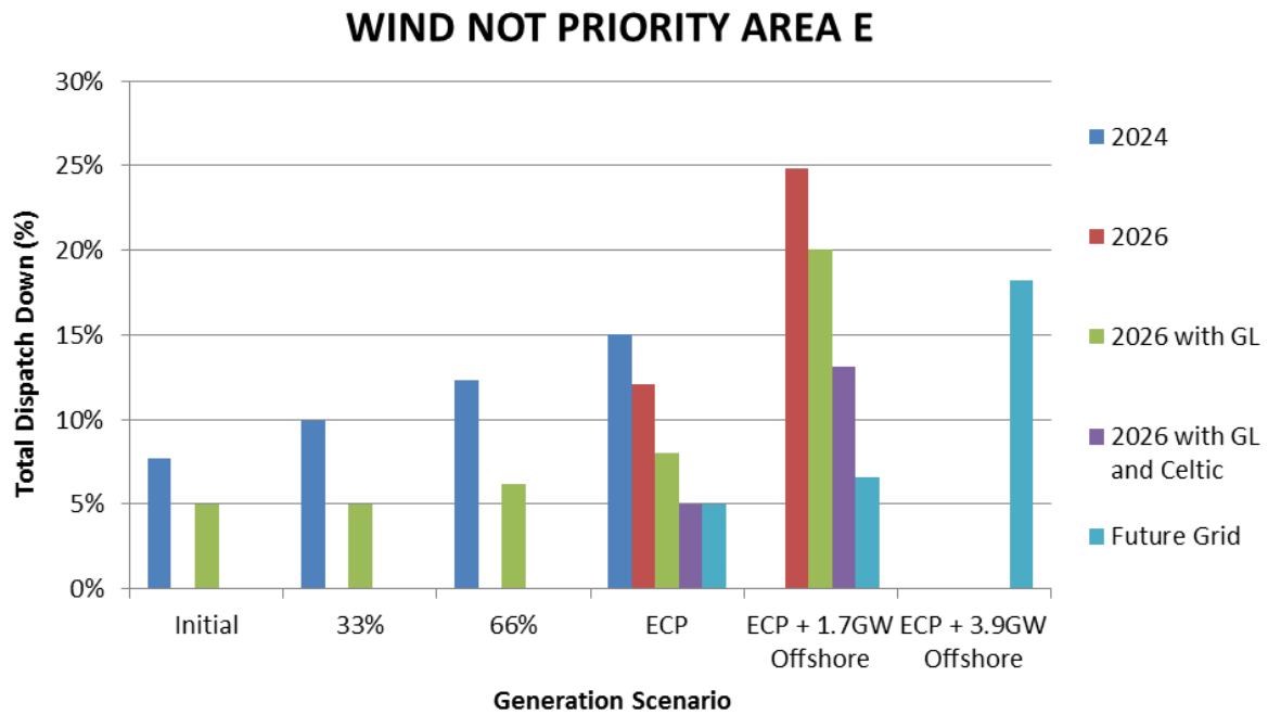
Figure 6-3 Results Wind Not Priority Area E
