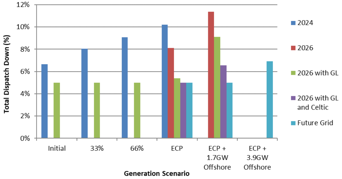
Figure C-11 Total Dispatch Down for Wind Priority
