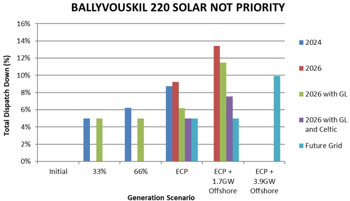
Figure C-7 Total Dispatch Down for Solar Not Priority
