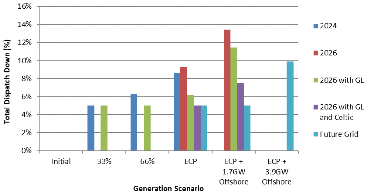
Figure C-67 Total Dispatch Down for Solar Not Priority
