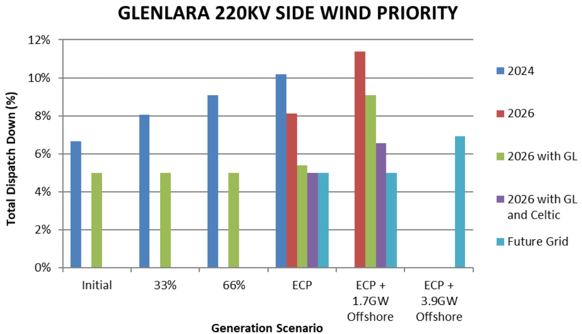
Figure C-39 Total Dispatch Down for Wind Priority
