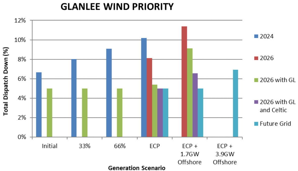
Figure C-34 Total Dispatch Down for Wind Priority
