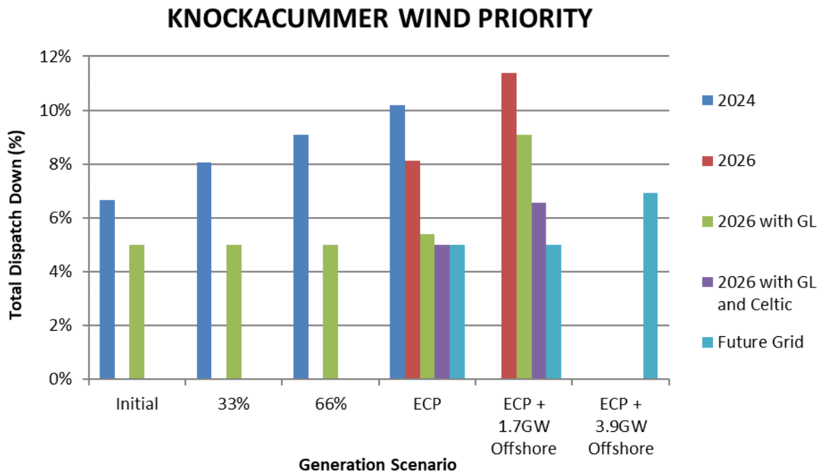
Figure C-44 Total Dispatch Down for Wind Priority
