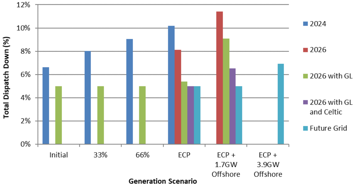
Figure C-57 Total Dispatch Down for Wind Priority
