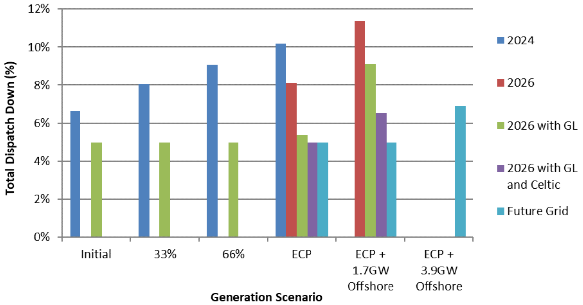
Figure C-17 Total Dispatch Down for Wind Priority
