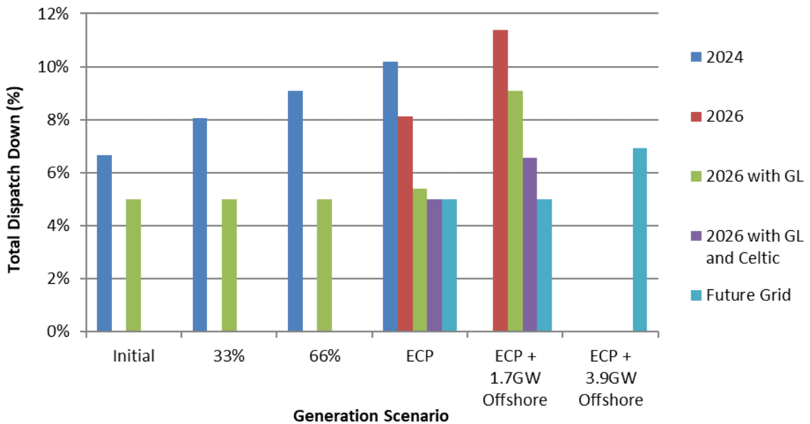
Figure C-59 Total Dispatch Down for Wind Priority
