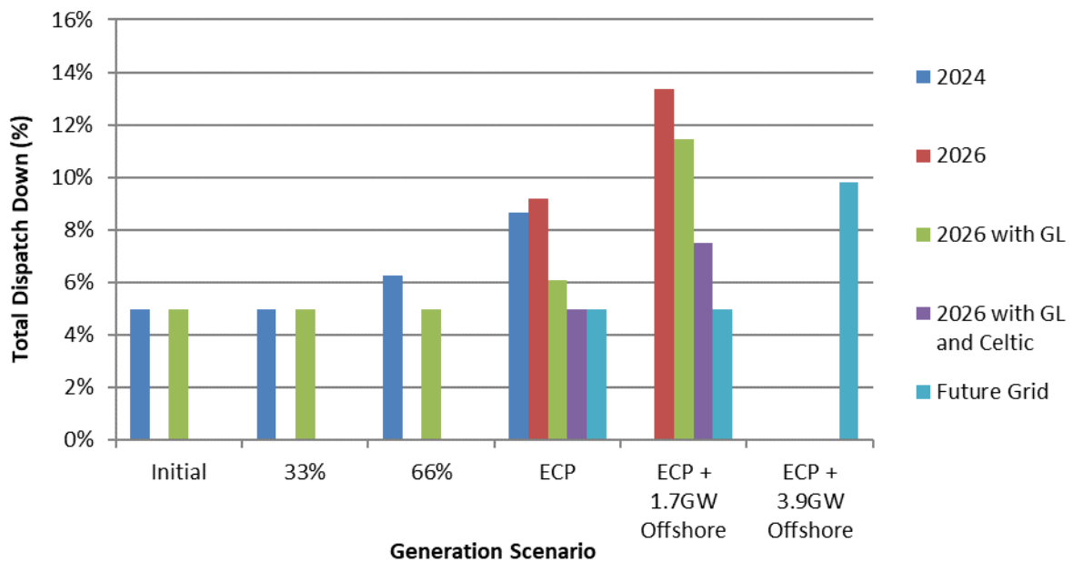
Figure C-36 Total Dispatch Down for Solar Not Priority
