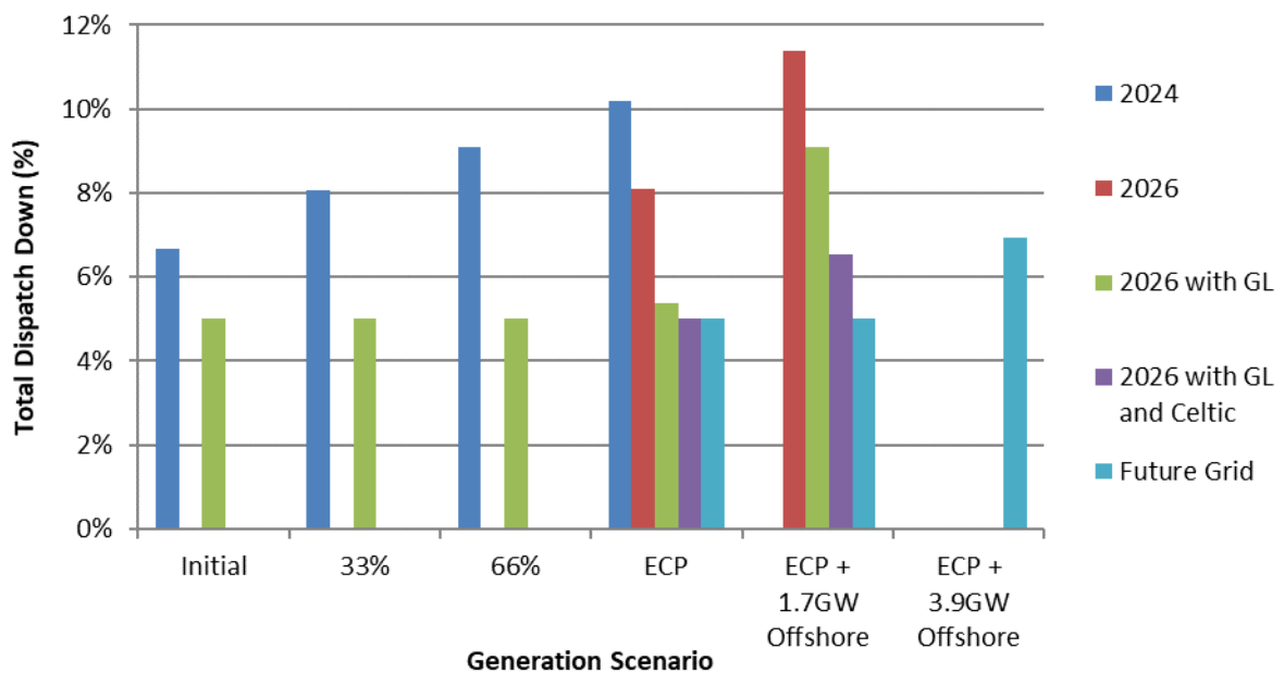
Figure C-3 Total Dispatch Down for Wind Priority
