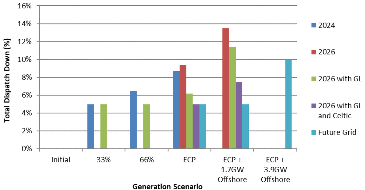
Figure C-56 Total Dispatch Down for Solar Not Priority
