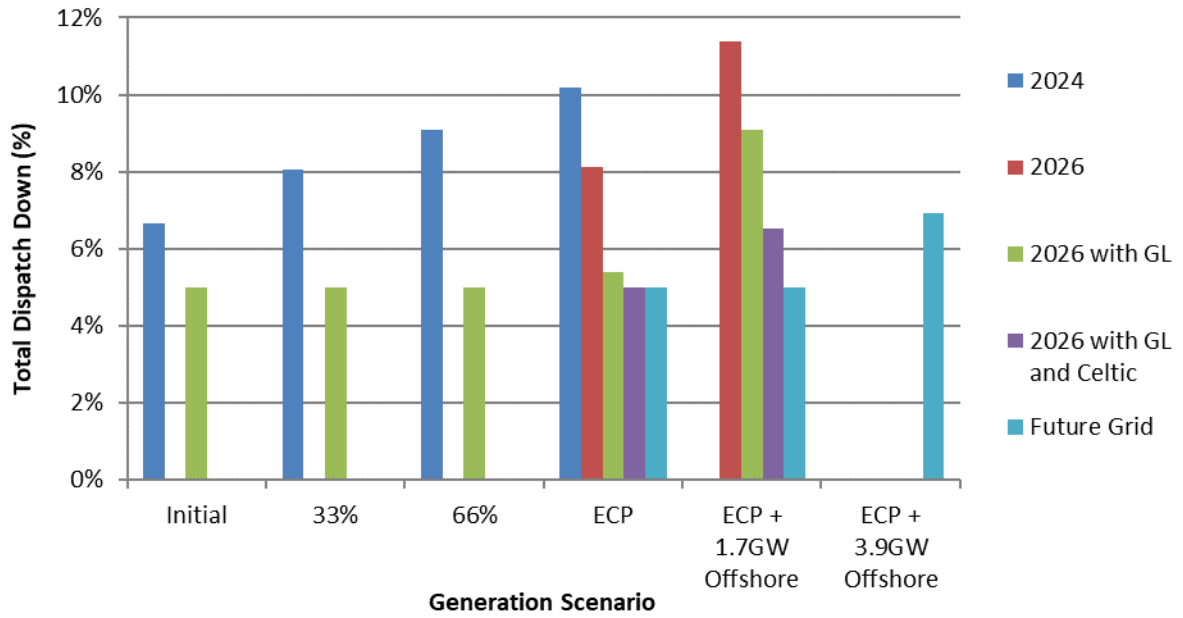
Figure C-37 Total Dispatch Down for Wind Priority
