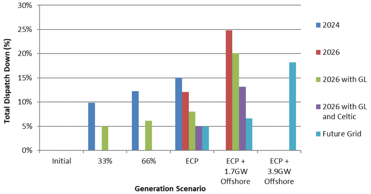
Figure C-8 Total Dispatch Down for Wind Not Priority
