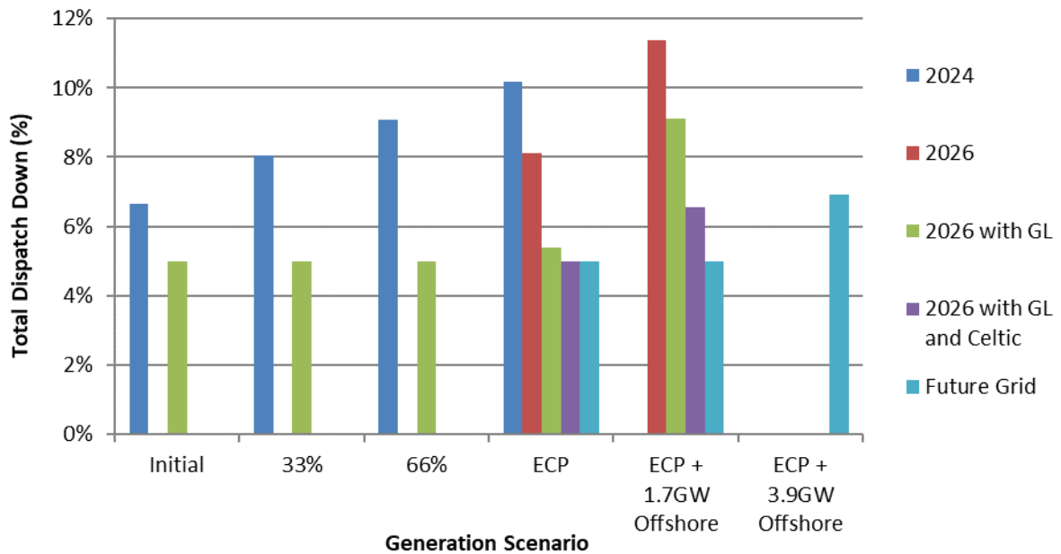
Figure C-19 Total Dispatch Down for Wind Priority
