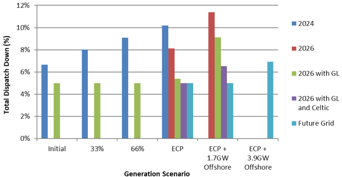
Figure C-54 Total Dispatch Down for Wind Priority
