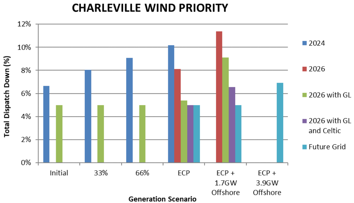
Figure C-14 Total Dispatch Down for Wind Priority
