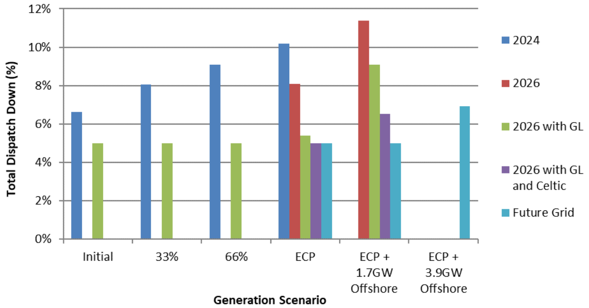
Figure C-65 Total Dispatch Down for Wind Priority
