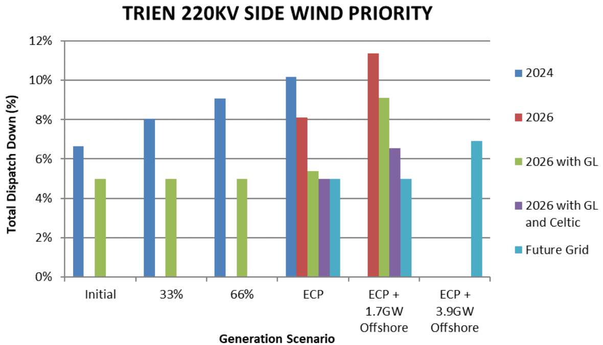
Figure C-70 Total Dispatch Down for Wind Priority
