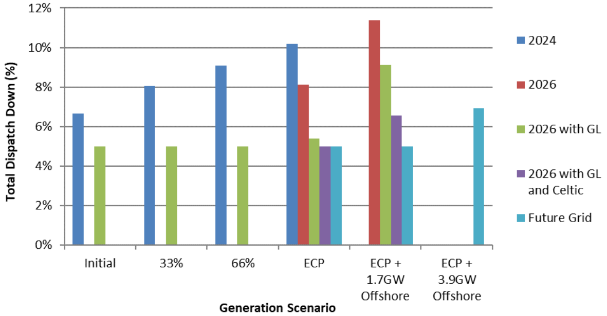
Figure C-42 Total Dispatch Down for Wind Priority
