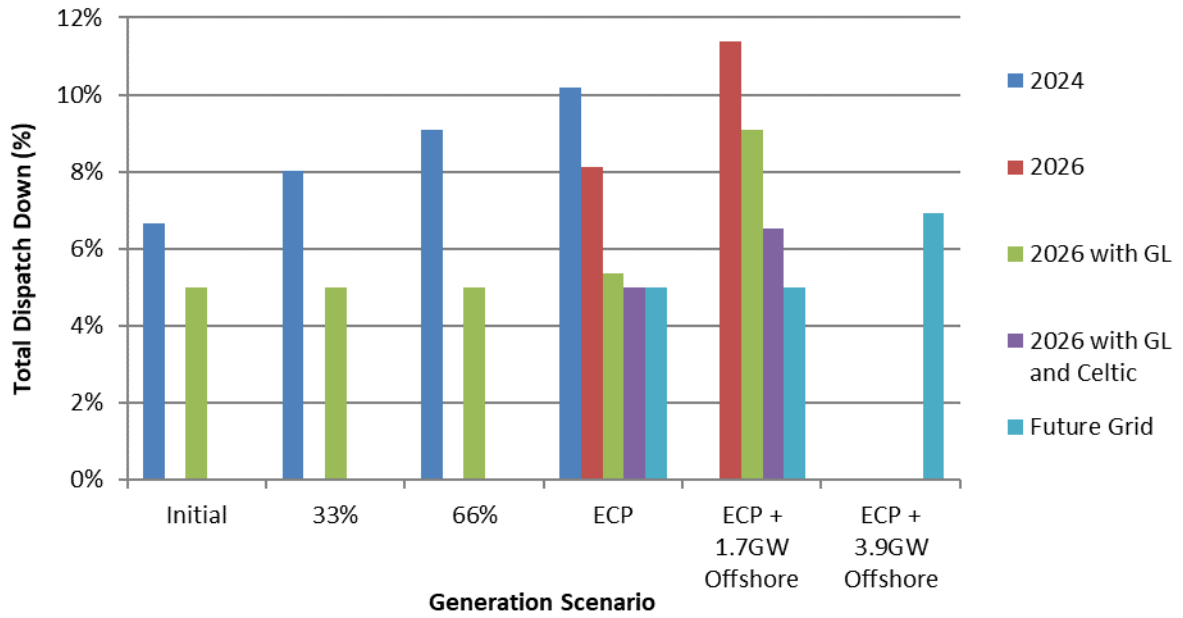
Figure C-47 Total Dispatch Down for Wind Priority
