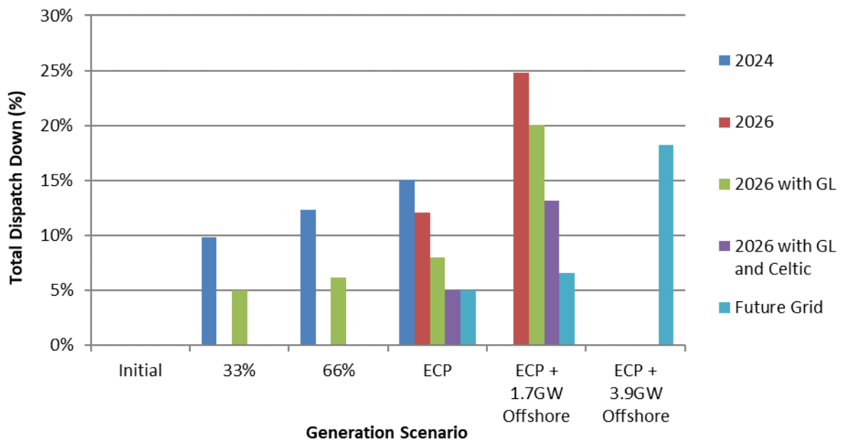
Figure C-41 Total Dispatch Down for Wind Not Priority
