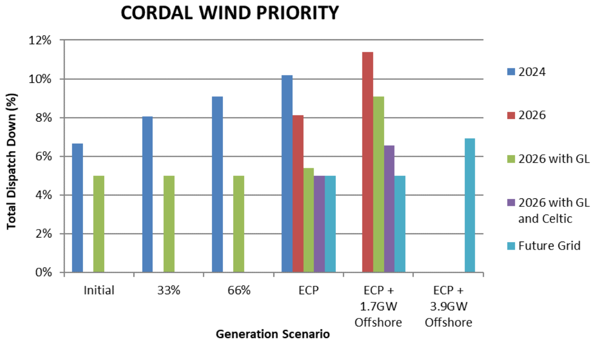
Figure C-26 Total Dispatch Down for Wind Priority
