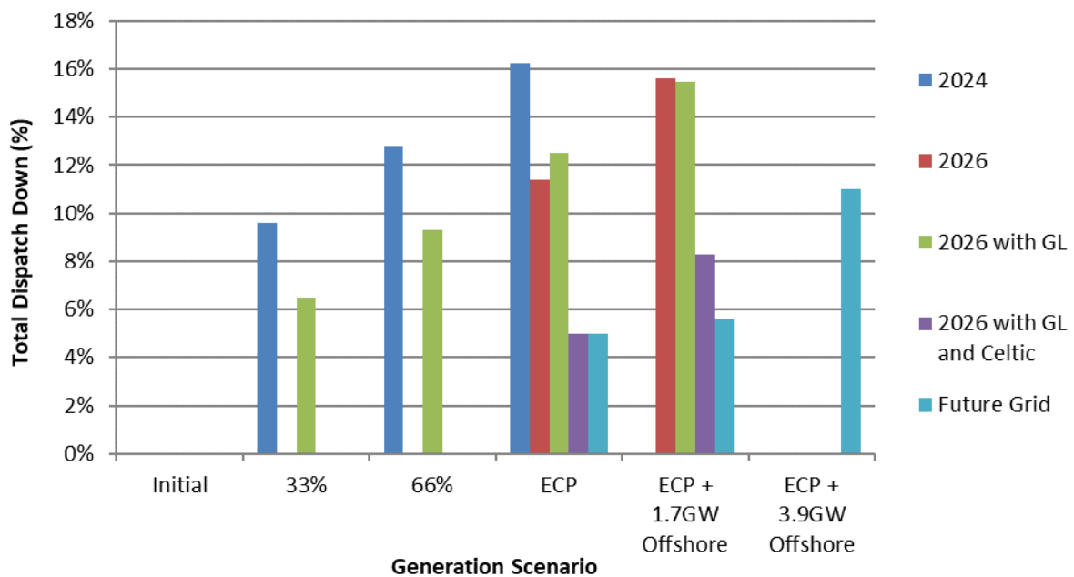
Figure C-33 Total Dispatch Down for Solar Not Priority
