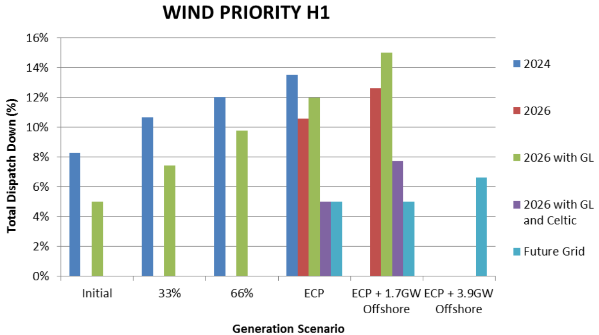
Figure 6-4 Results Wind Priority Area H1
