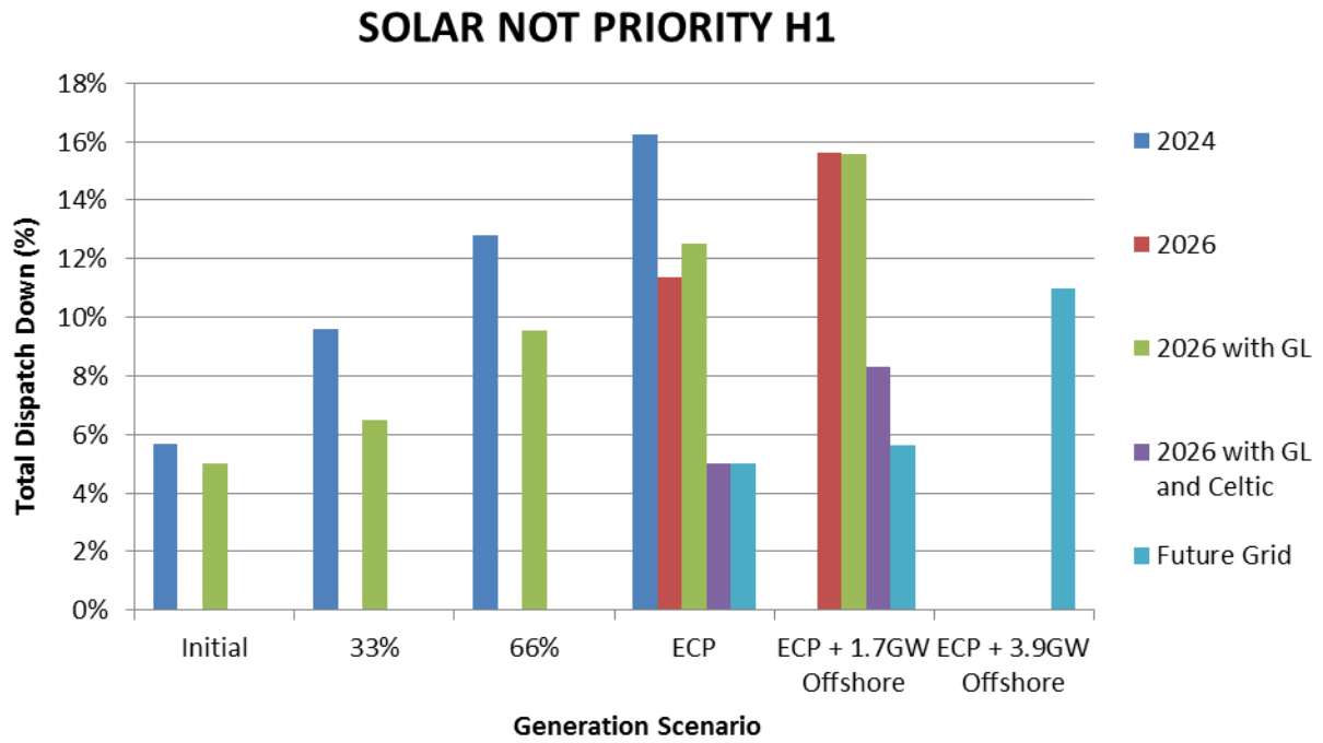
Figure 6-2 Results Solar Not Priority Area H1
