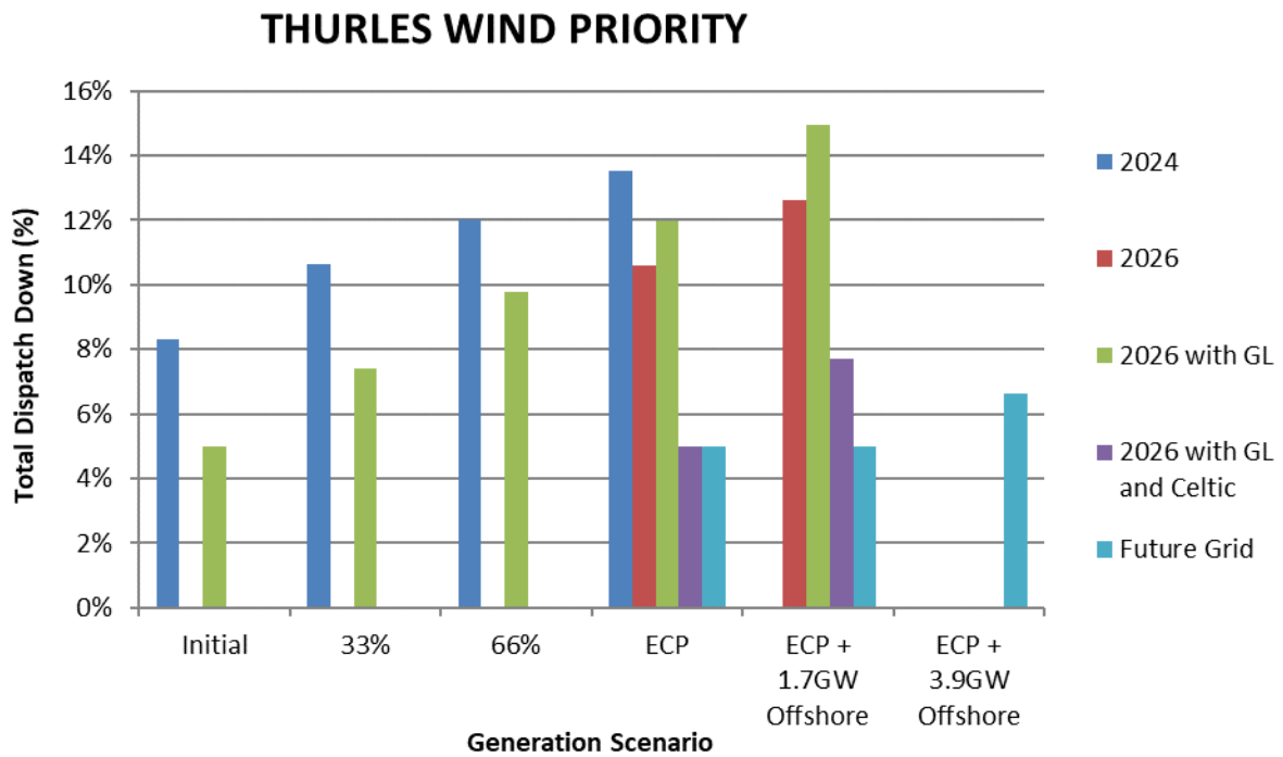
Figure C-29 Total Dispatch Down for Wind Priority
