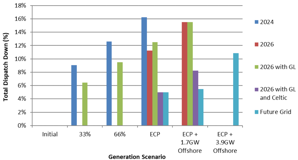
Figure C-31 Total Dispatch Down for Solar Not Priority
