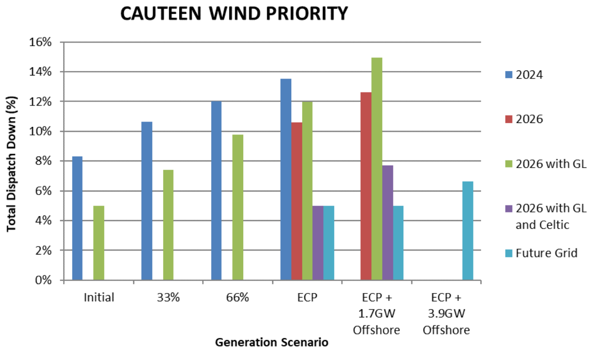
Figure C-12 Total Dispatch Down for Wind Priority
