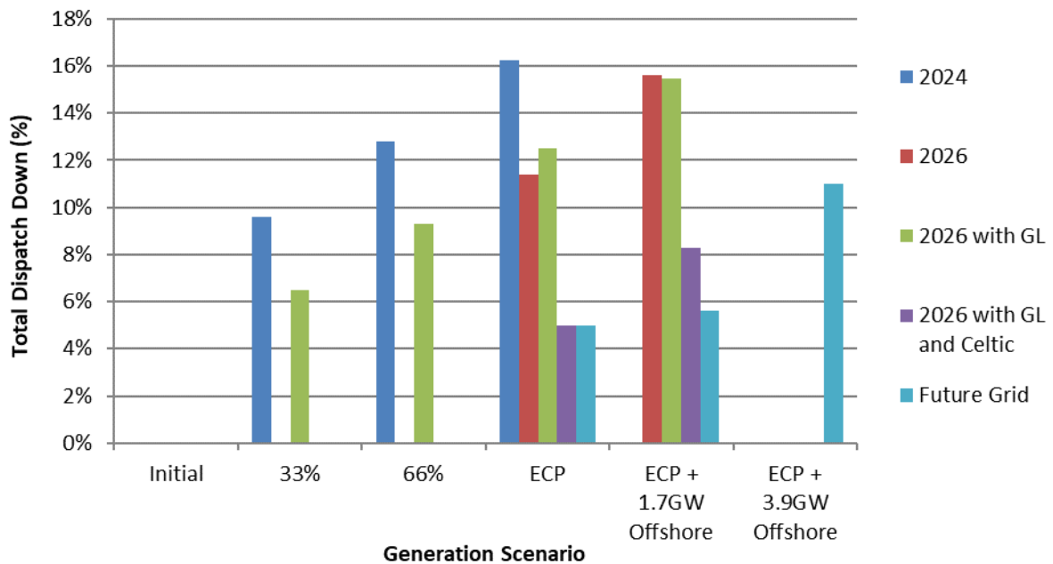
Figure C-27 Total Dispatch Down for Solar Not Priority
