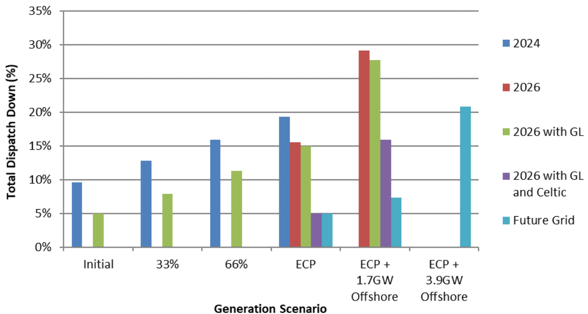
Figure C-20 Total Dispatch Down for Wind Not Priority
