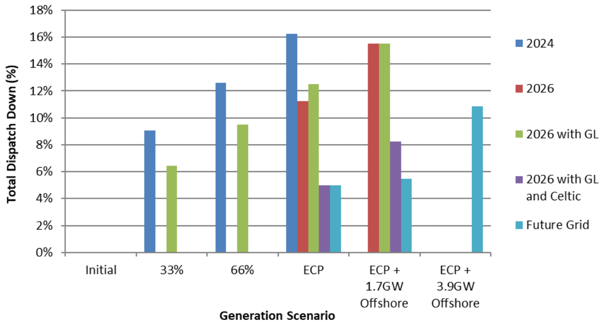
Figure C-25 Total Dispatch Down for Solar Not Priority
