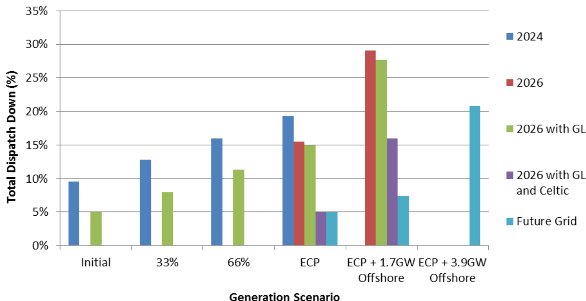
Figure 6-3 Results Wind Not Priority Area H1
