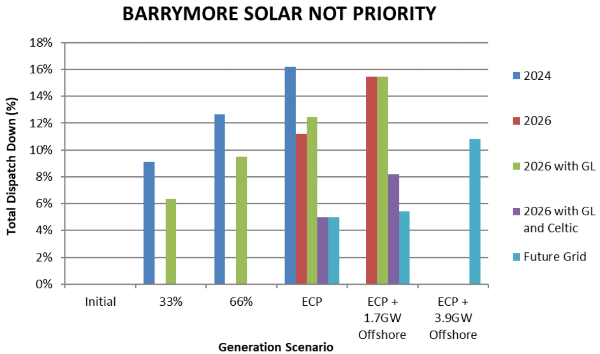
Figure C-7 Total Dispatch Down for Solar Not Priority
