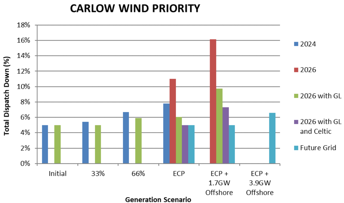
Figure C-19 Total Dispatch Down for Wind Priority
