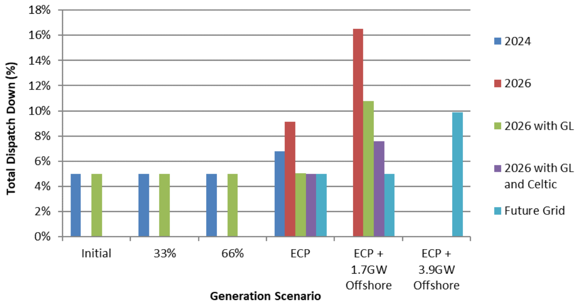
Figure C-37 Total Dispatch Down for Solar Not Priority
