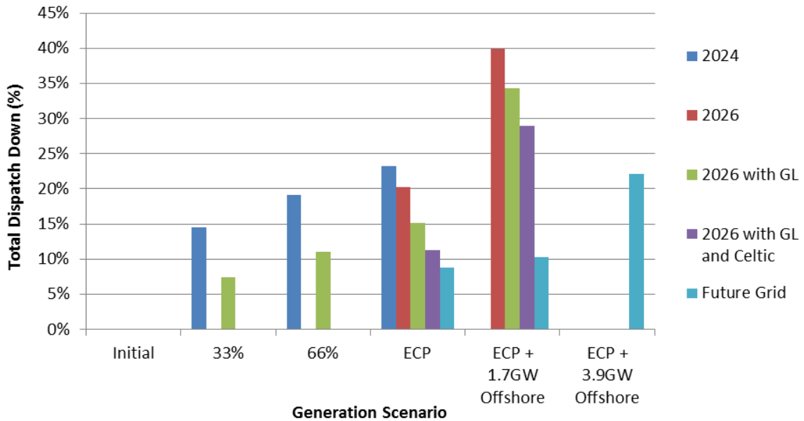
Figure 6-6 Results Wind Not Priority in Ballybeg – Wexford (Area H2)
