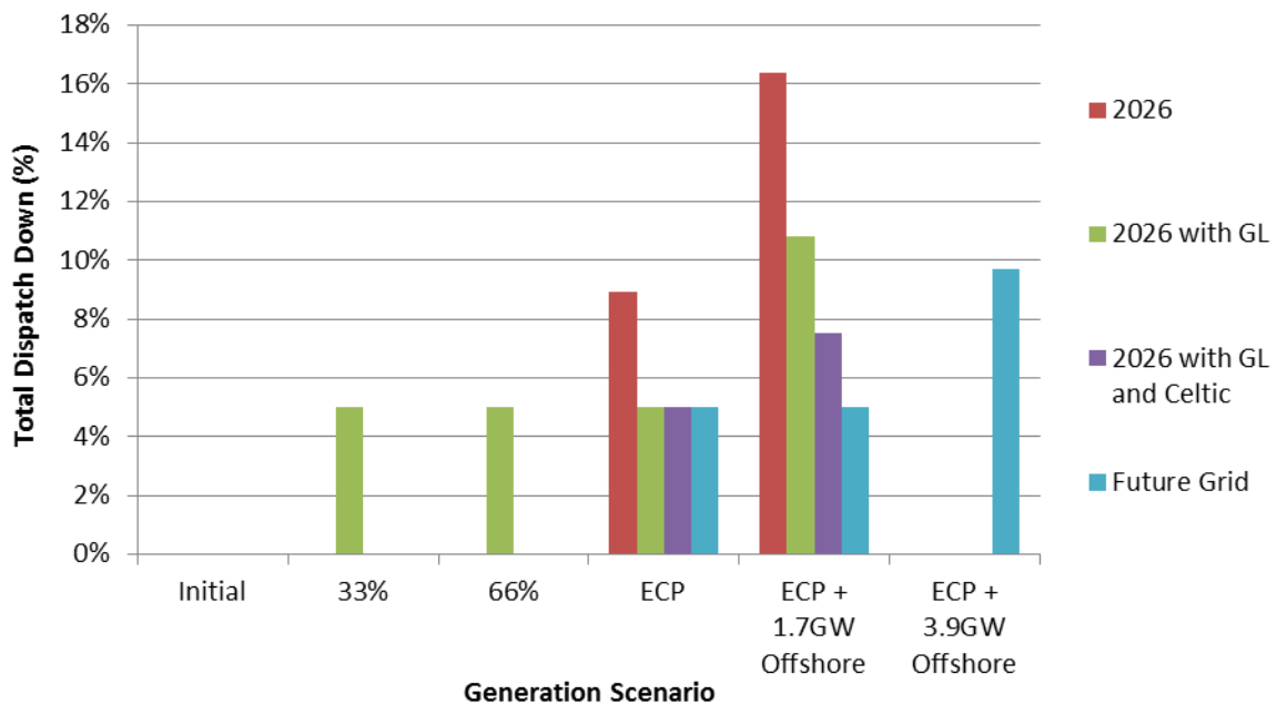
Figure C-9 Total Dispatch Down for Solar Not Priority
