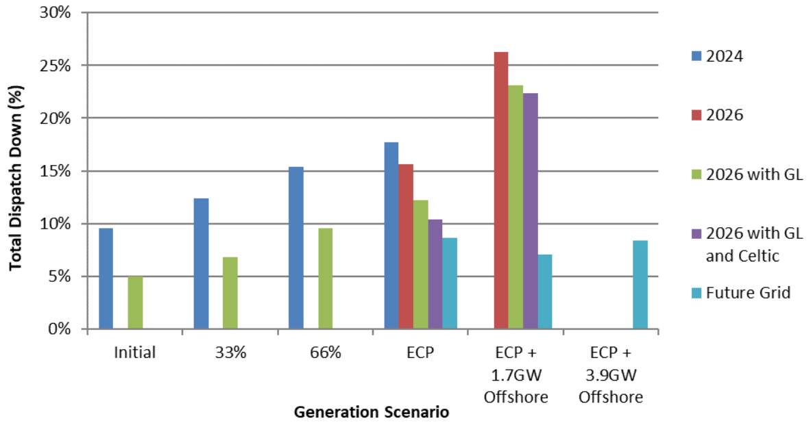
Figure C-41 Total Dispatch Down for Wind Priority
