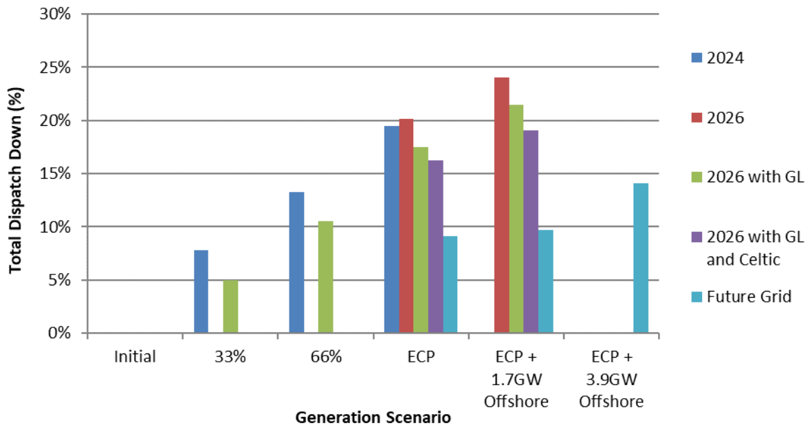
Figure C-26 Total Dispatch Down for Solar Not Priority
