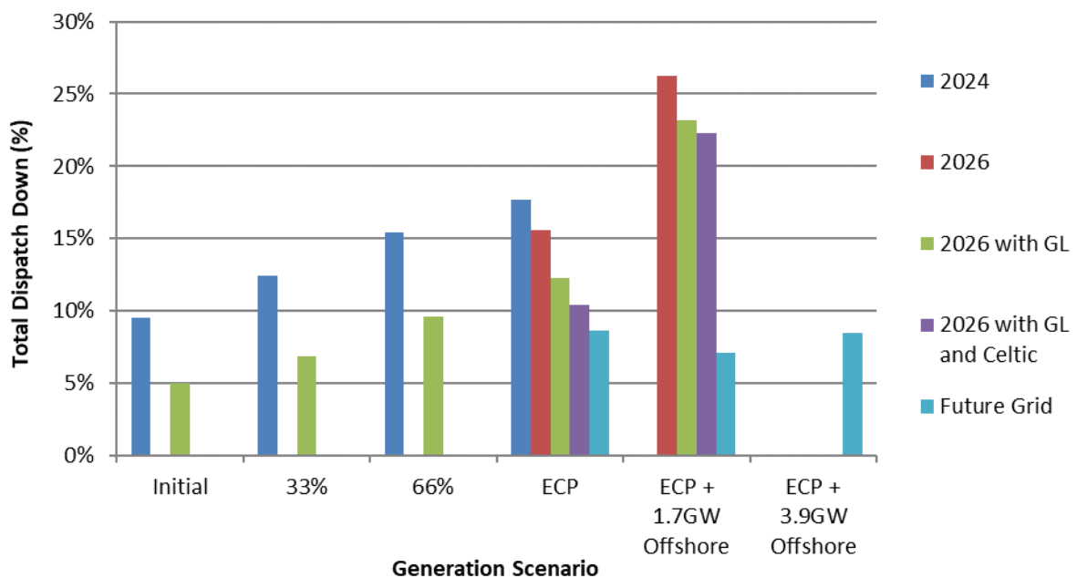
Figure C-5 Total Dispatch Down for Wind Priority
