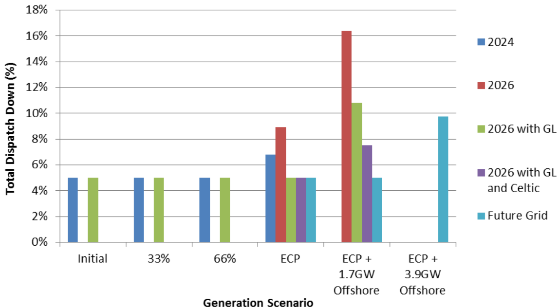
Figure C-29 Total Dispatch Down for Solar Not Priority
