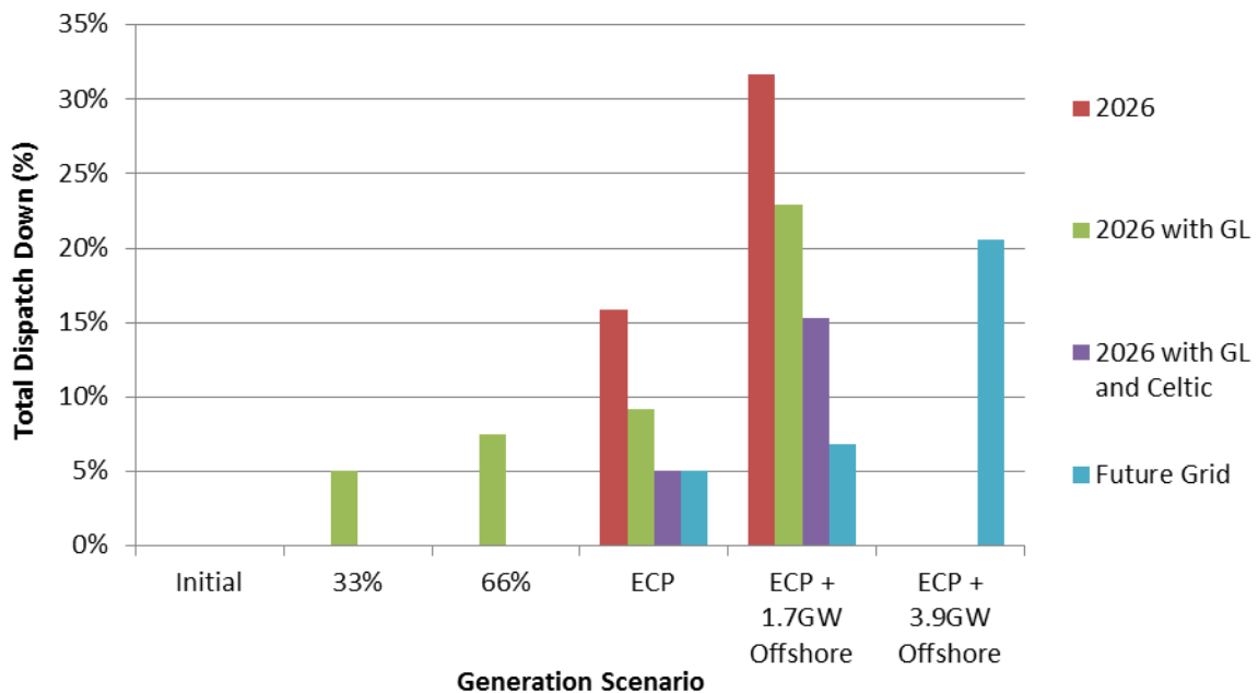
Figure C-10 Total Dispatch Down for Wind Not Priority
