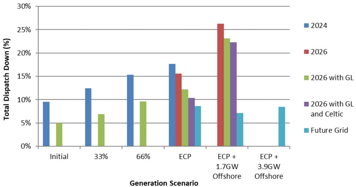
Figure C-21 Total Dispatch Down for Wind Priority
