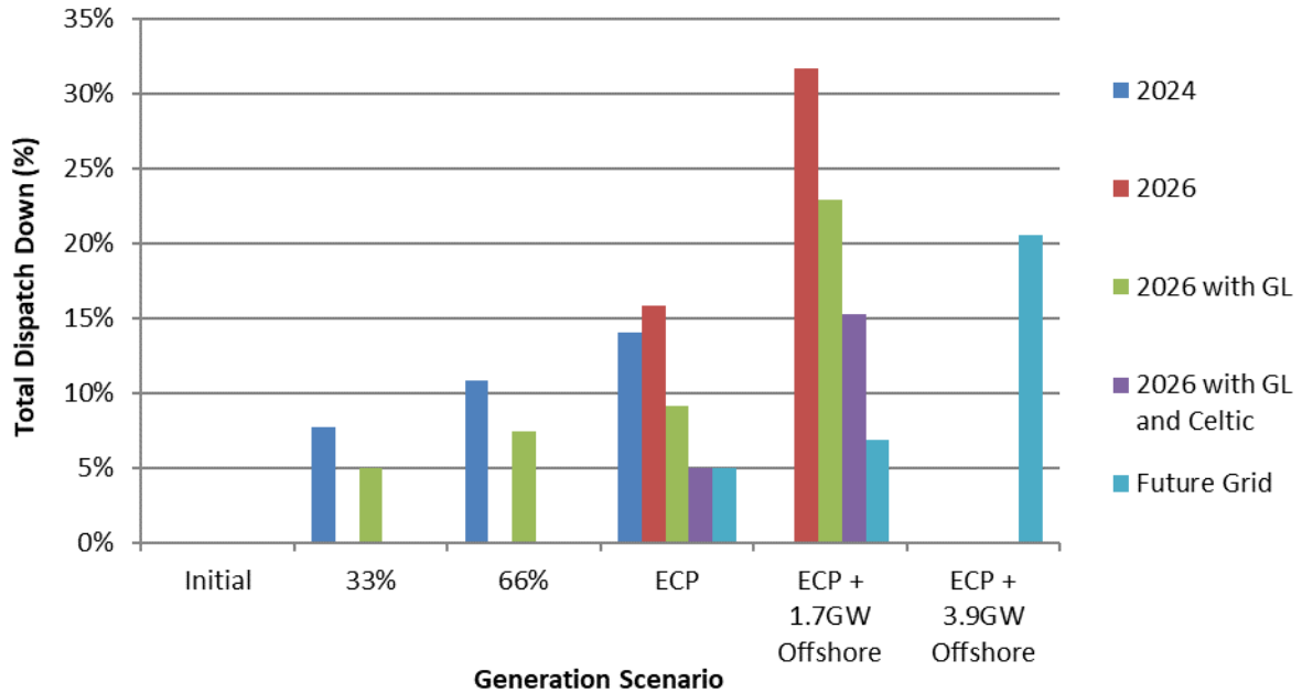
Figure C-18 Total Dispatch Down for Wind Not Priority
