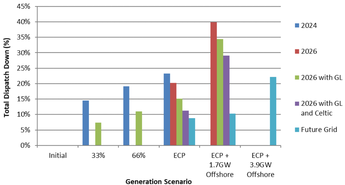
Figure C-4 Total Dispatch Down for Wind Not Priority
