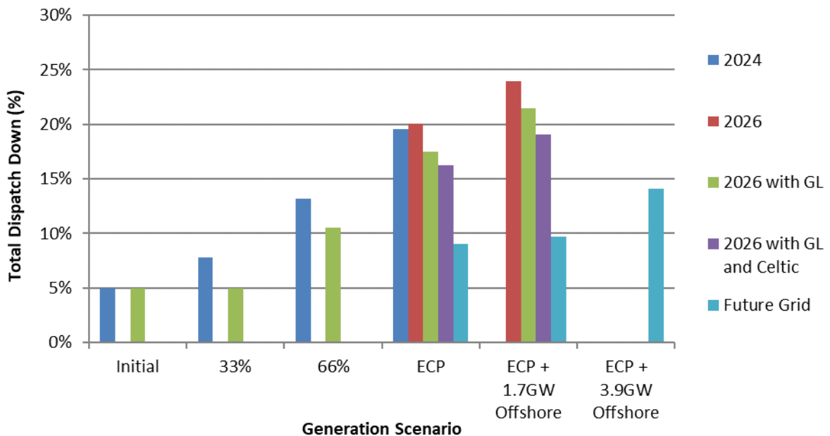
Figure C-23 Total Dispatch Down for Solar Not Priority
