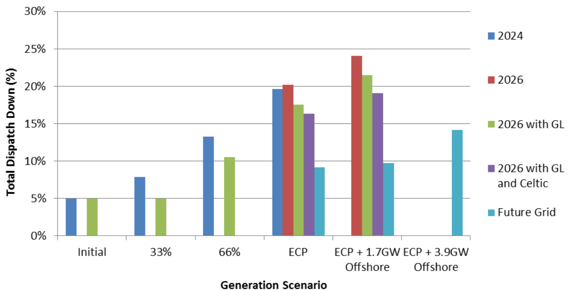
Figure 6-5 Results Solar Not Priority in Ballybeg – Wexford (Area H2)
