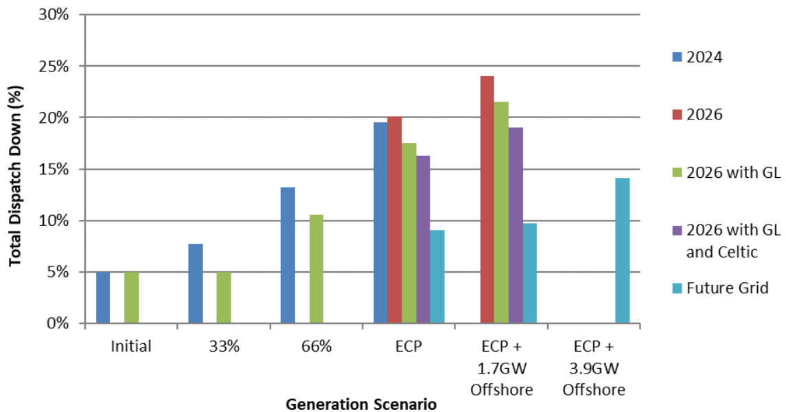
Figure C-40 Total Dispatch Down for Solar Not Priority
