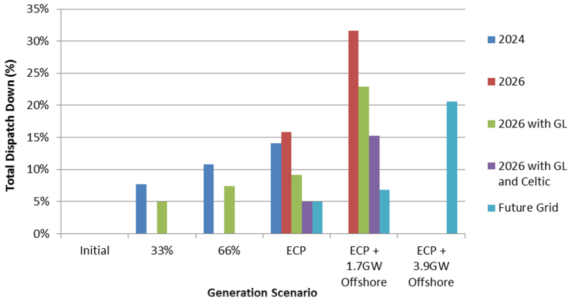
Figure 6-3 Results Wind Not Priority in Carlow – Waterford (Area H2)
