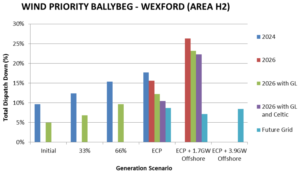
Figure 6-7 Results Wind Priority in Ballybeg – Wexford (Area H2)
