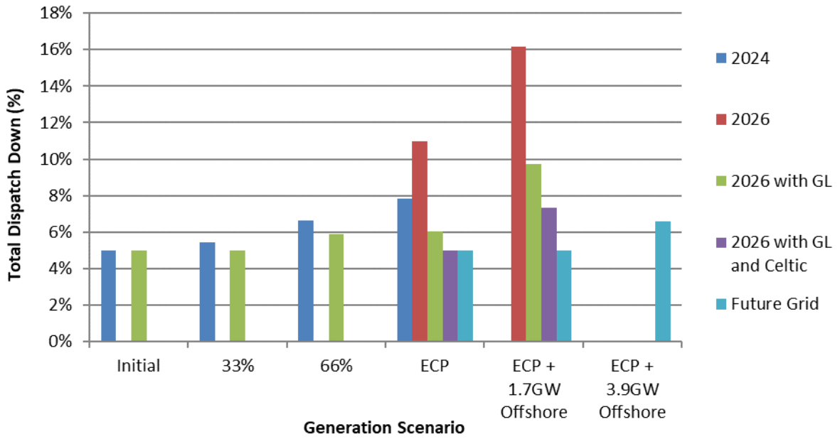
Figure C-38 Total Dispatch Down for Wind Priority
