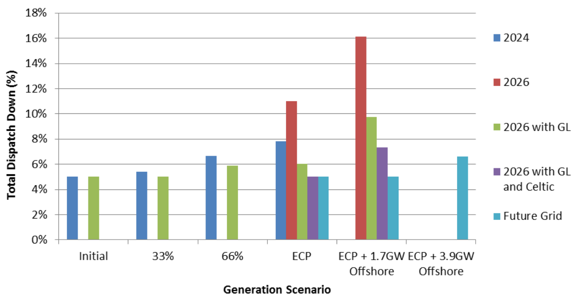
Figure 6-4 Results Wind Priority in Carlow – Waterford (Area H2)
