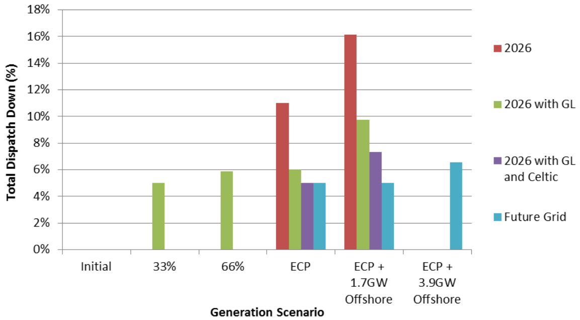
Figure C-11 Total Dispatch Down for Wind Priority
