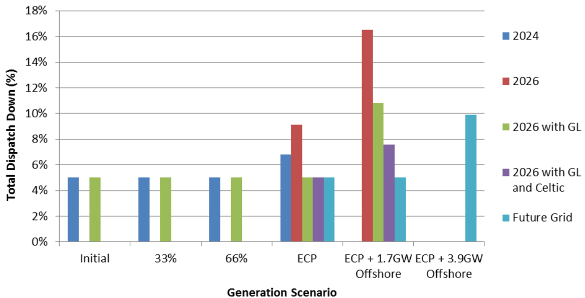
Figure 6-2 Results Solar Not Priority in Carlow – Waterford (Area H2)
