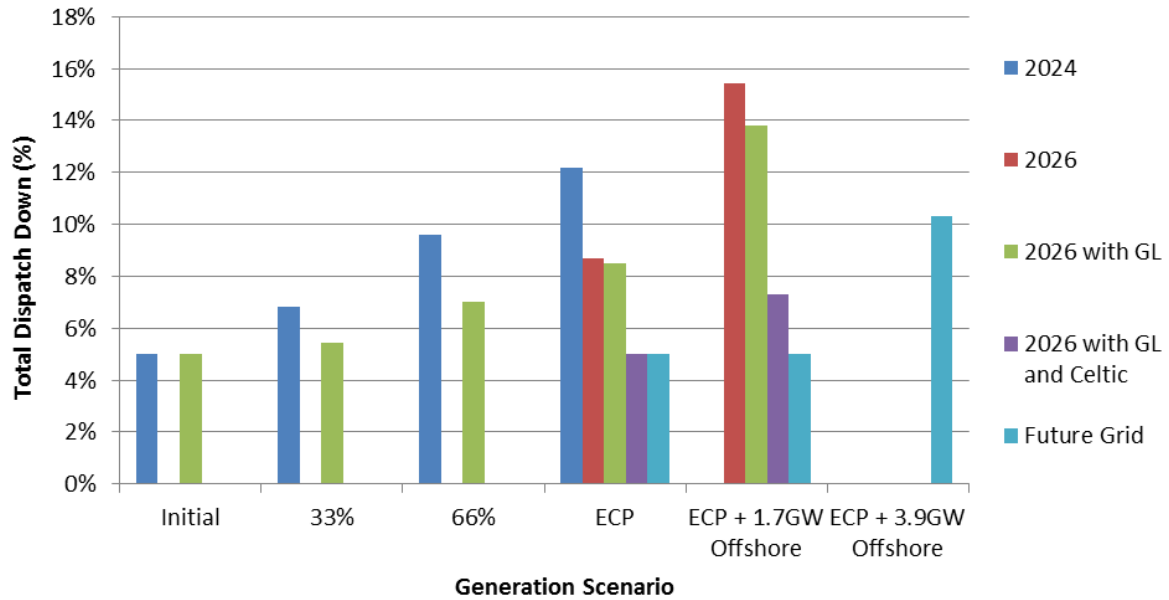
Figure 6-2 Results Solar Not Priority Area I
