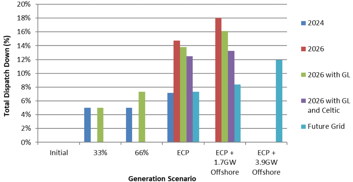
Figure C-62 Total Dispatch Down for Solar Not Priority
