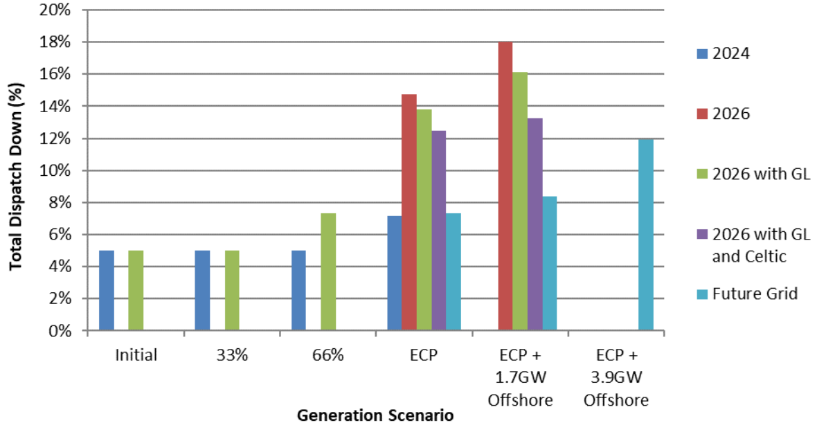
Figure C-60 Total Dispatch Down for Solar Not Priority
