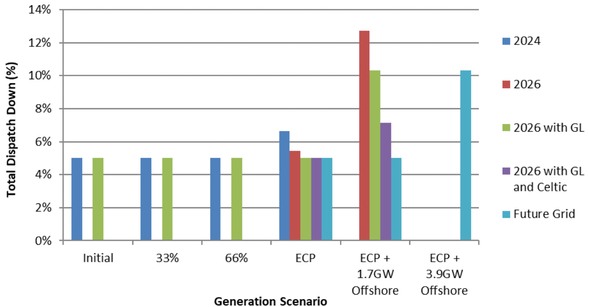
Figure C-55 Total Dispatch Down for Solar Not Priority
