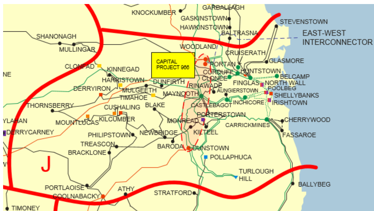
Figure 6-1 Network Map for Area J
