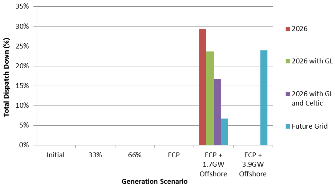
Figure C-5 Total Dispatch Down for Wind Not Priority
