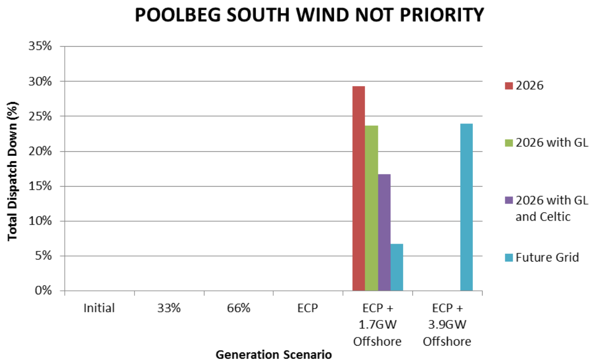
Figure C-49 Total Dispatch Down for Wind Not Priority
