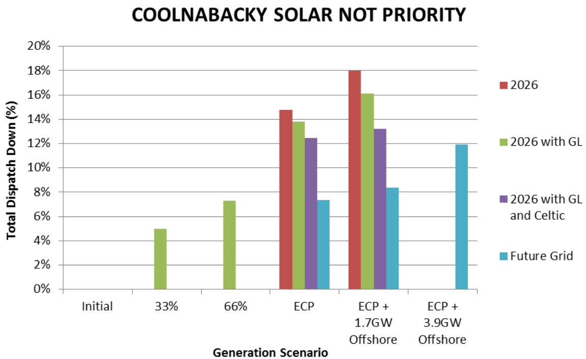
Figure C-15 Total Dispatch Down for Solar Not Priority
