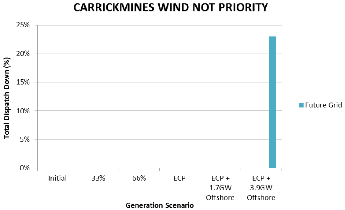
Figure C-11 Total Dispatch Down for Wind Not Priority
