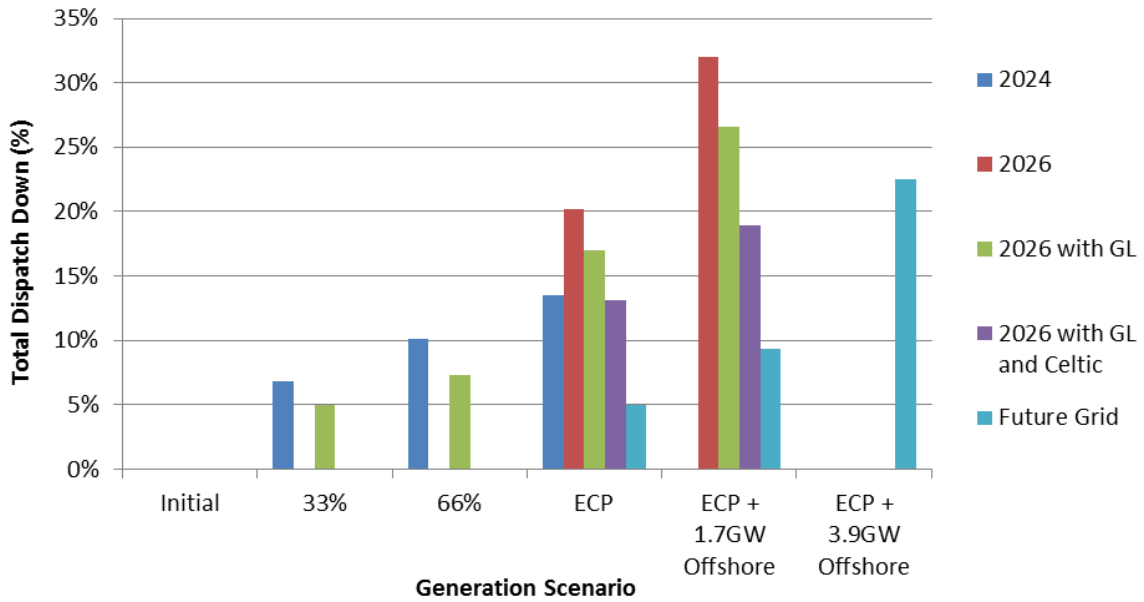
Figure 6-5 Results Wind Not Priority J - Country (Area J)
