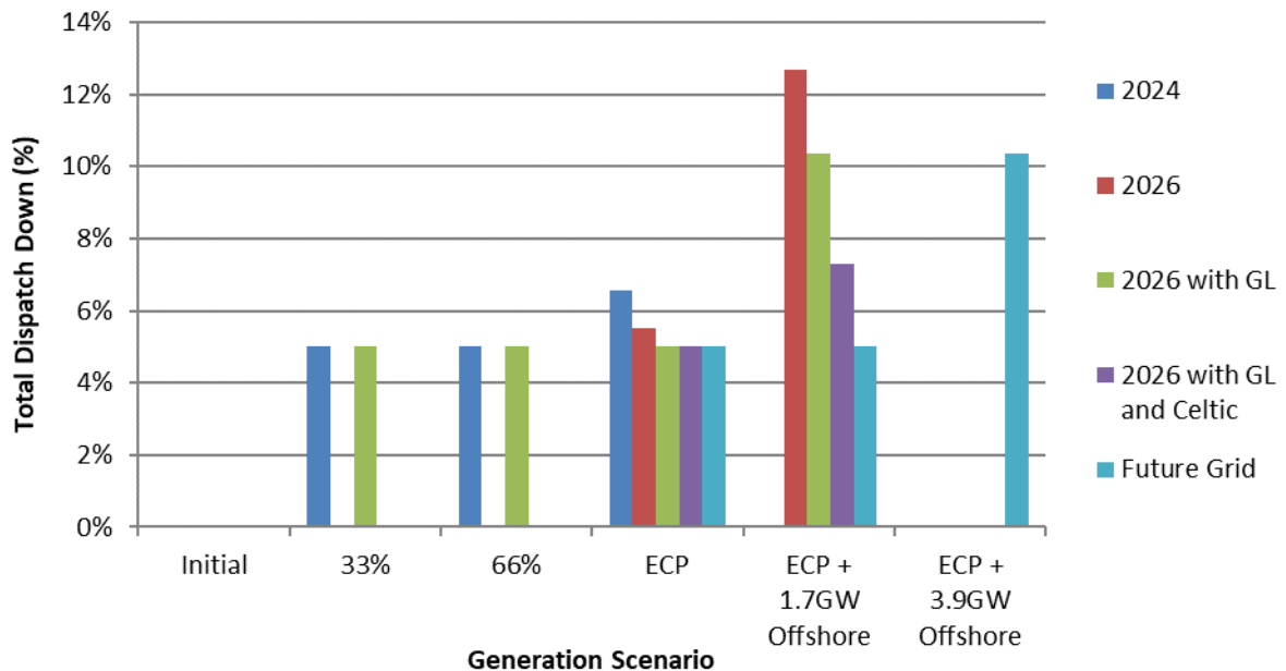
Figure C-24 Total Dispatch Down for Solar Not Priority
