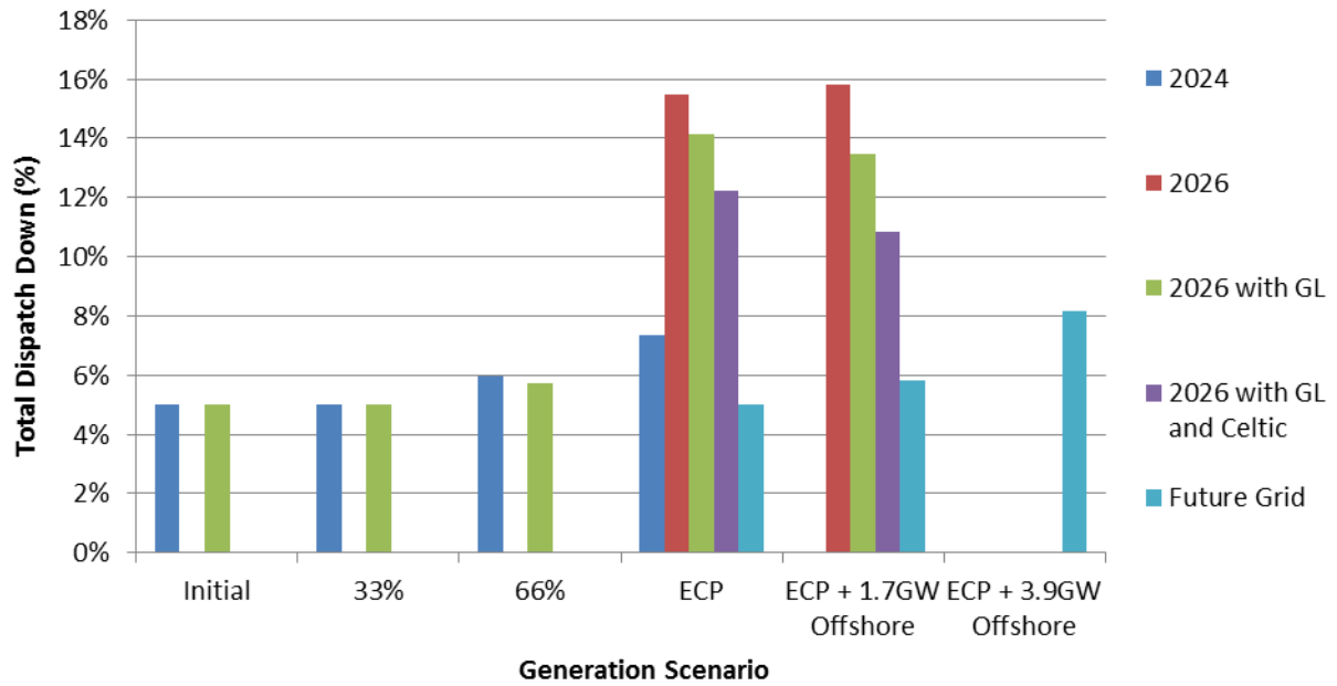
Figure 6-6 Results Wind Priority J - Country (Area J)
