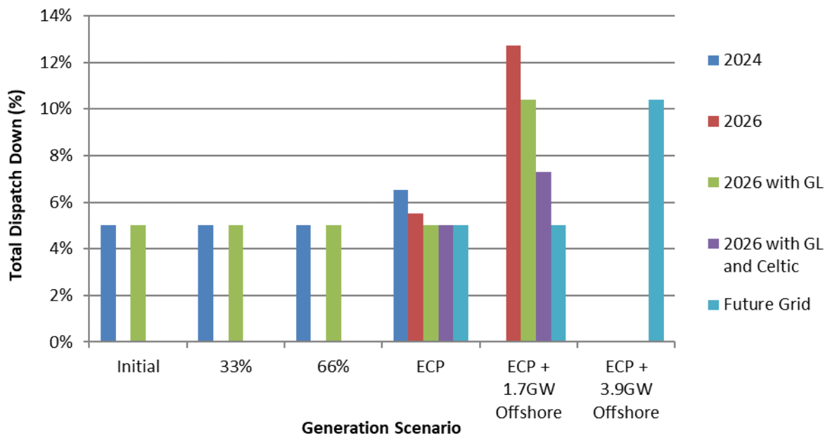
Figure C-30 Total Dispatch Down for Solar Not Priority
