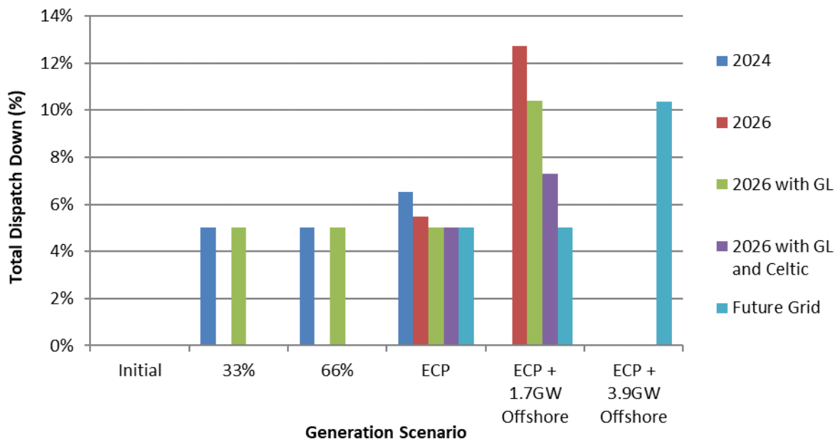
Figure C-28 Total Dispatch Down for Solar Not Priority
