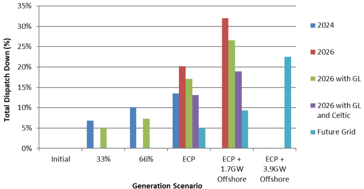
Figure C-45 Total Dispatch Down for Wind Not Priority
