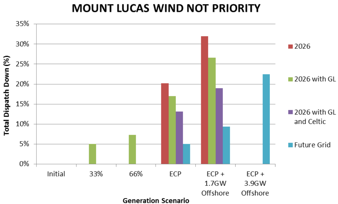
Figure C-38 Total Dispatch Down for Wind Not Priority
