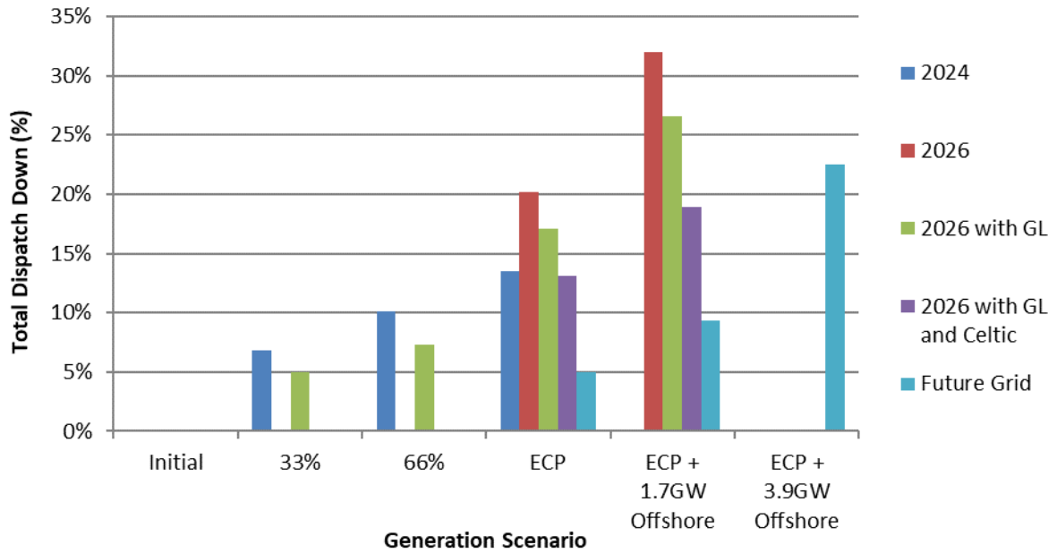
Figure C-52 Total Dispatch Down for Wind Not Priority
