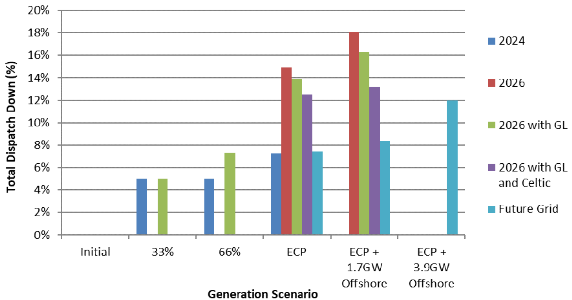
Figure C-51 Total Dispatch Down for Solar Not Priority
