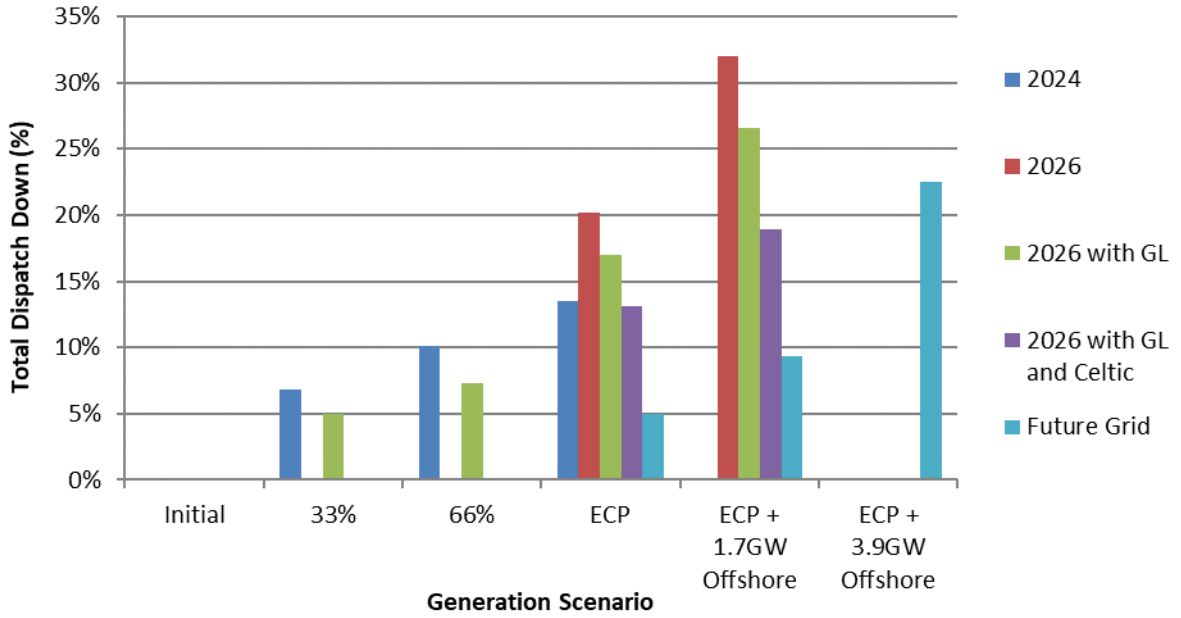
Figure C-58 Total Dispatch Down for Wind Not Priority
