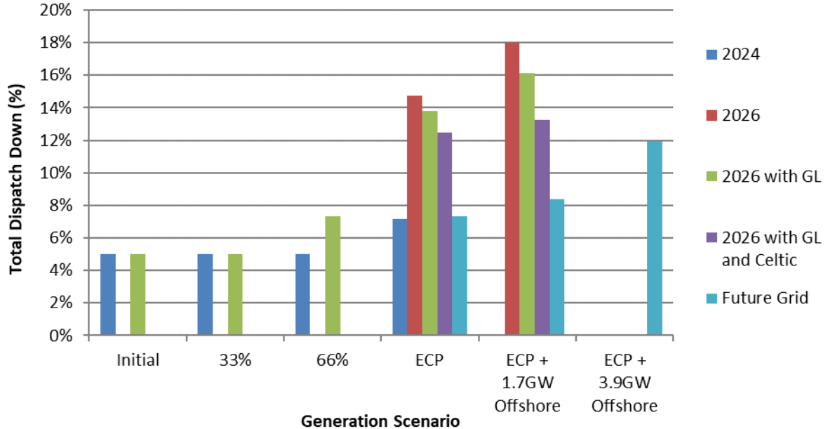
Figure C-32 Total Dispatch Down for Solar Not Priority
