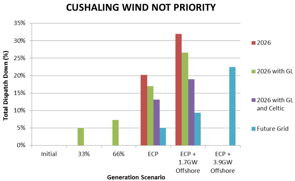
Figure C-17 Total Dispatch Down for Wind Not Priority
