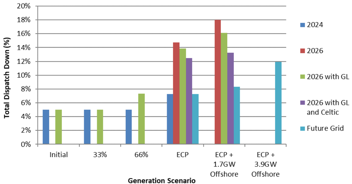
Figure C-57 Total Dispatch Down for Solar Not Priority
