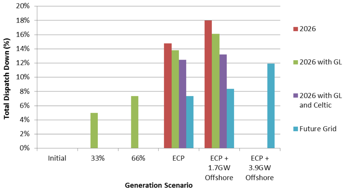
Figure C-13 Total Dispatch Down for Solar Not Priority
