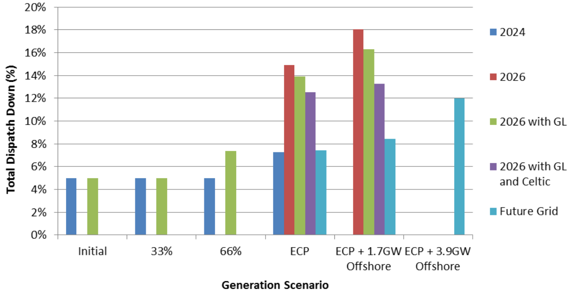
Figure 6-4 Results Solar Not Priority J - Country (Area J)
