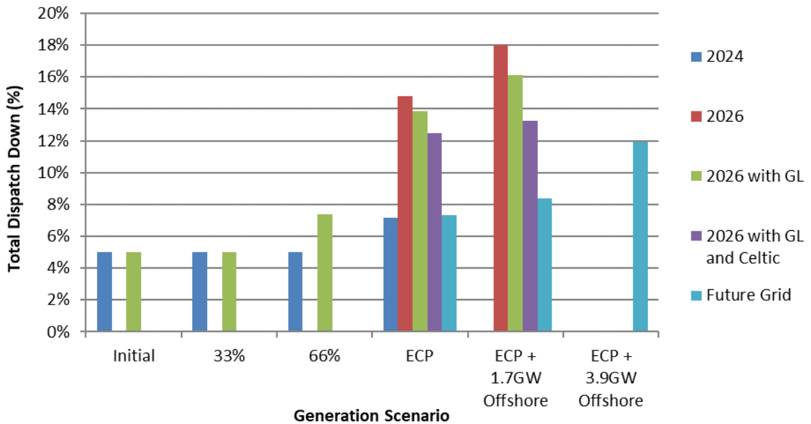
Figure C-34 Total Dispatch Down for Solar Not Priority
