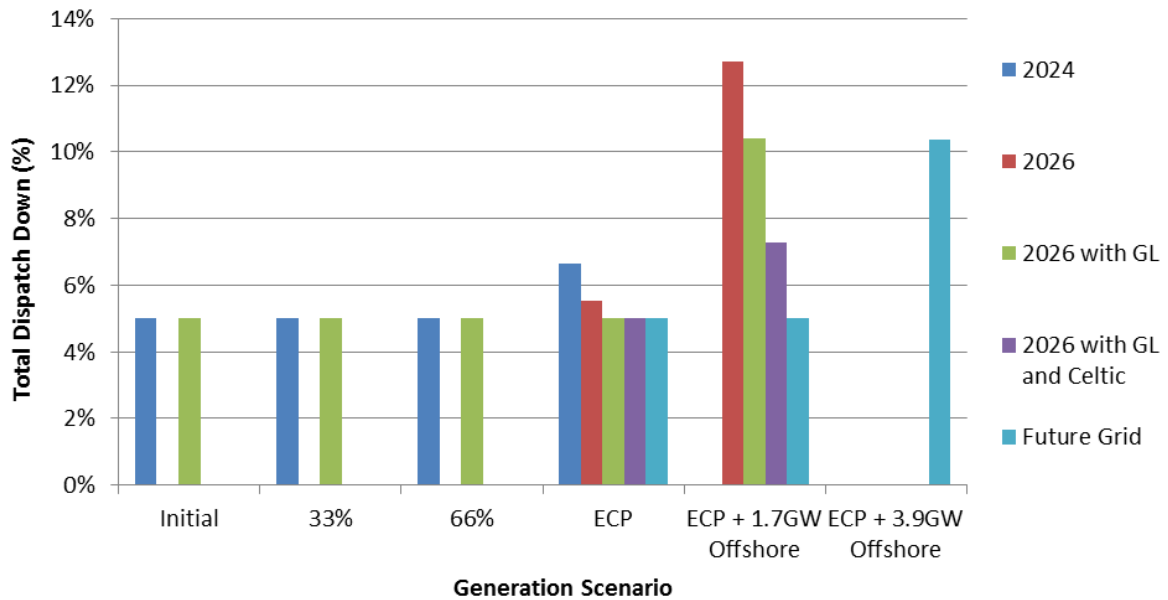
Figure 6-2 Results Solar Not Priority J - Country (Area J)
