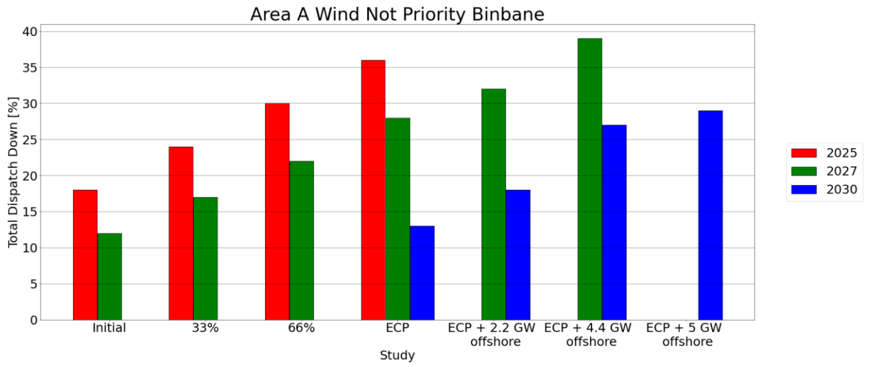
Figure C - 5 Total Dispatch Down for Wind Not Priority
