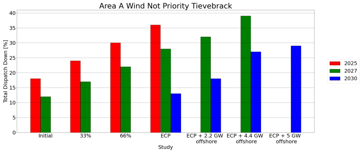
Figure C - 35 Total Dispatch Down for Wind Not Priority
