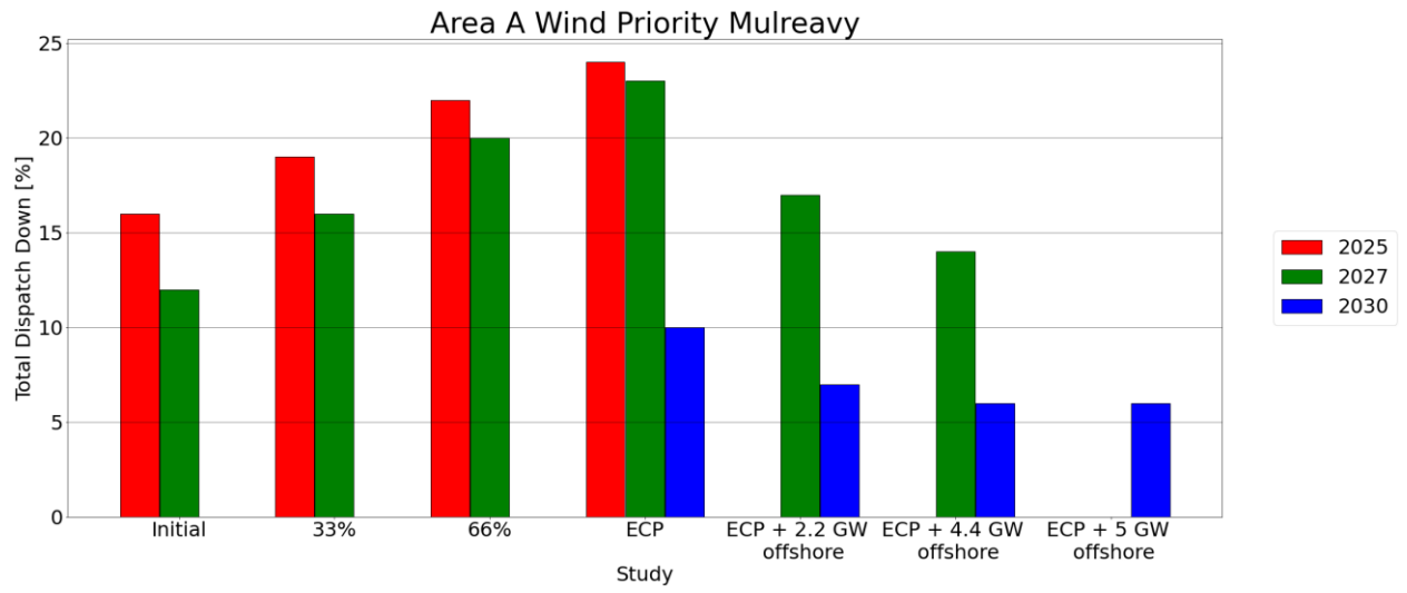
Figure C - 30 Total Dispatch Down for Wind Priority
