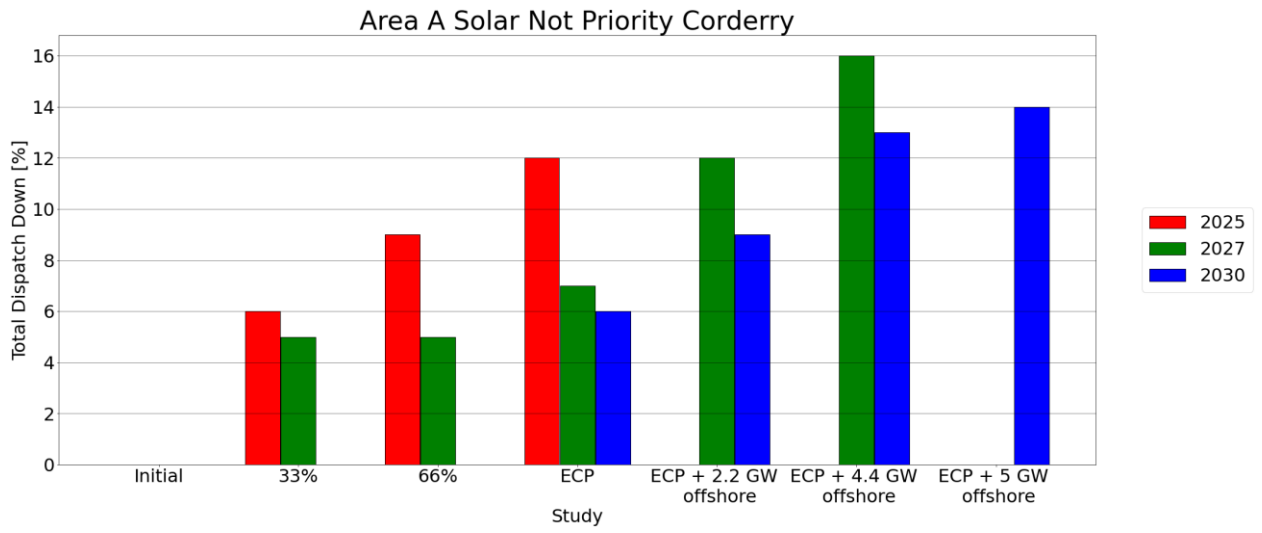
Figure C - 11 Total Dispatch Down for Solar Not Priority
