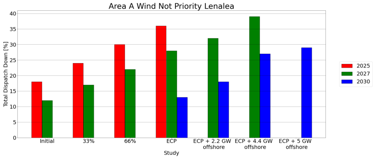
Figure C - 24 Total Dispatch Down for Wind Not Priority
