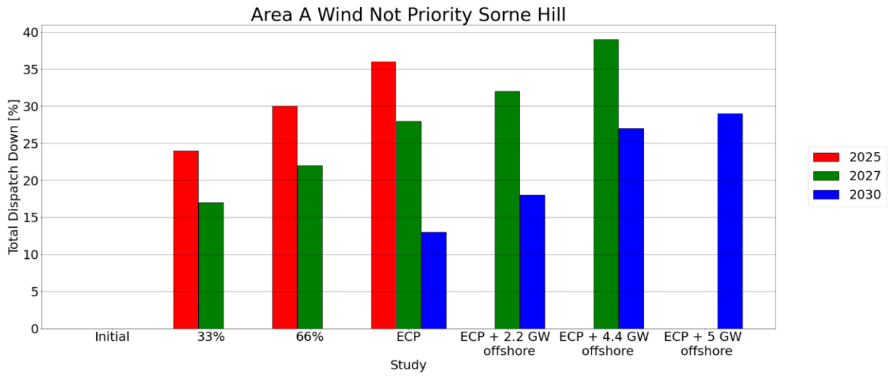
Figure C - 32 Total Dispatch Down for Wind Not Priority
