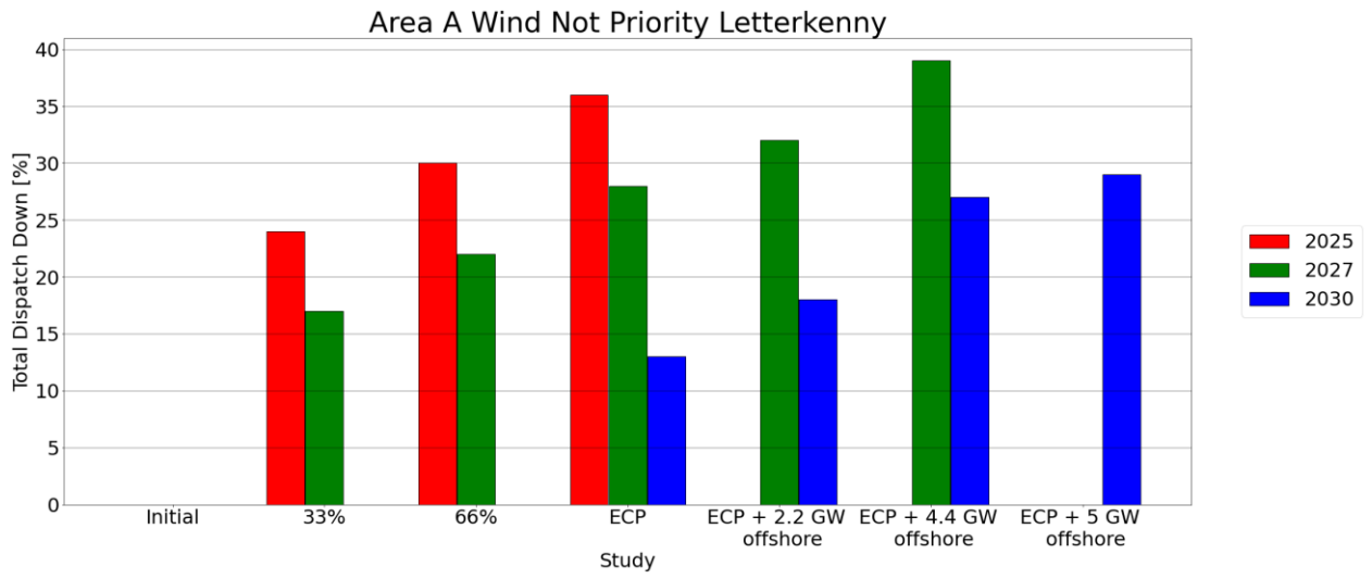
Figure C - 26 Total Dispatch Down for Wind Not Priority
