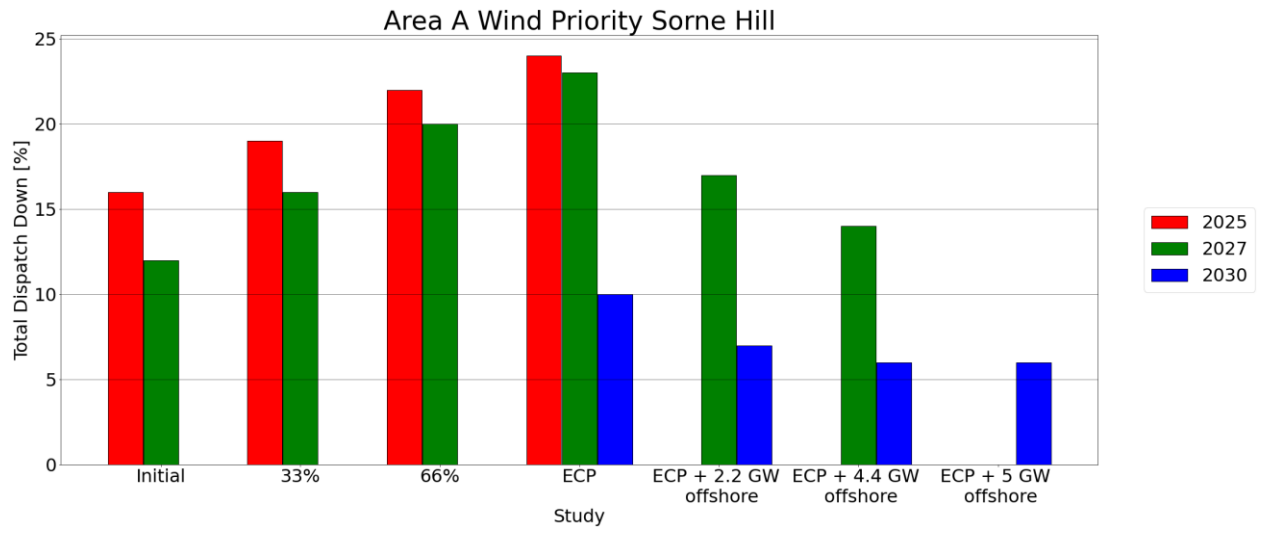
Figure C - 33 Total Dispatch Down for Wind Priority
