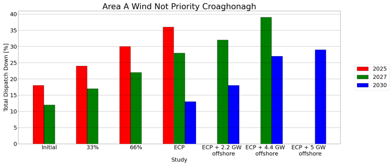
Figure C - 15 Total Dispatch Down for Wind Not Priority
