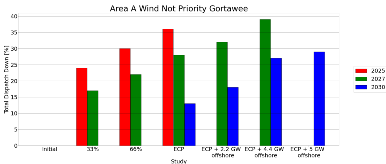
Figure C-22 - Total Dispatch Down for Wind not priority
