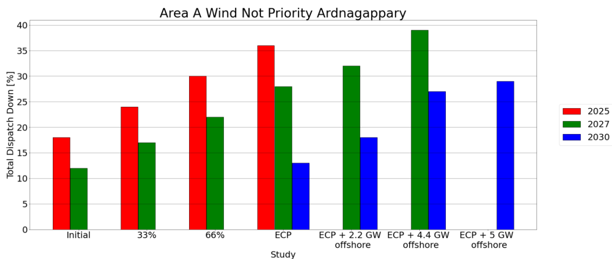
Figure C-3 - Total Dispatch Down for Wind not priority
