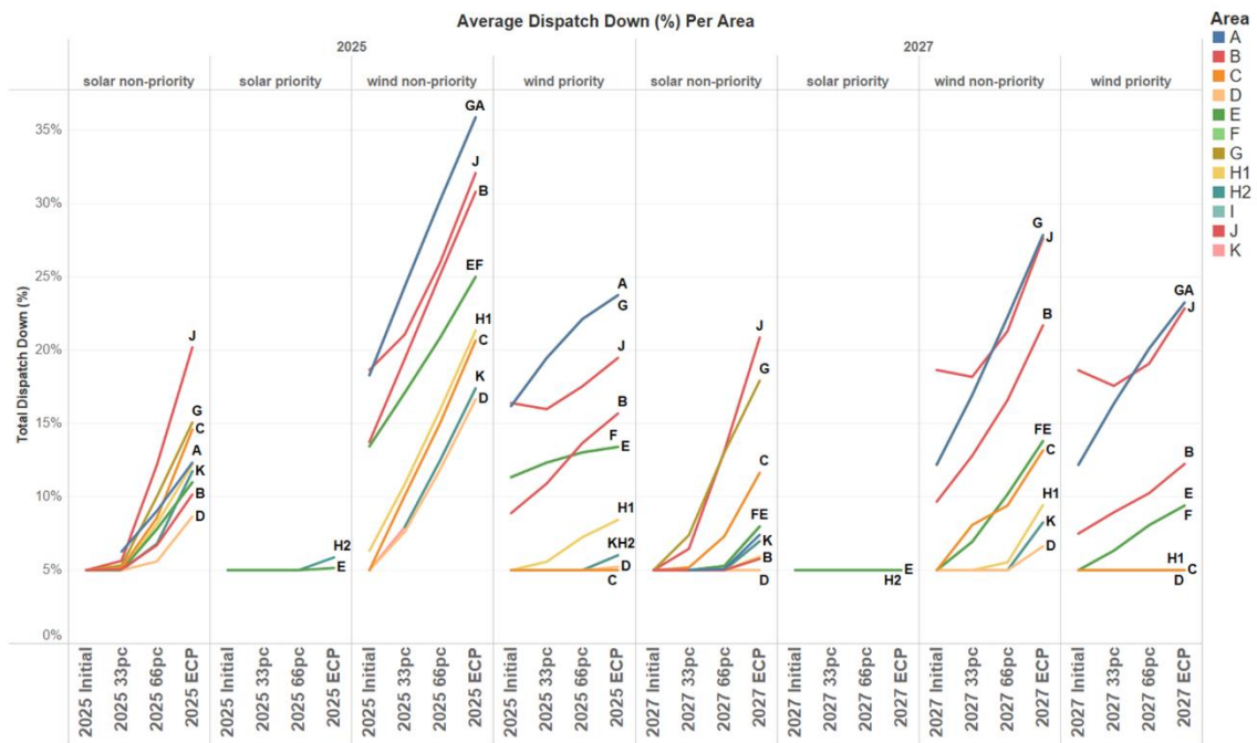
Figure 5-3 Total Dispatch Down % per Area
