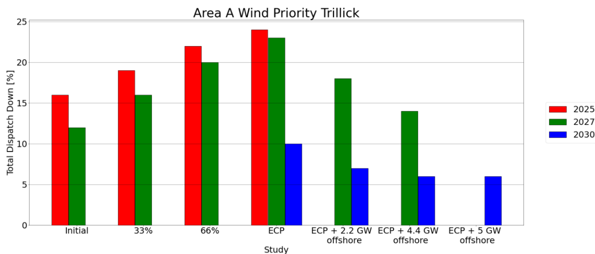
Figure C-37 - Total Dispatch Down for Wind priority
