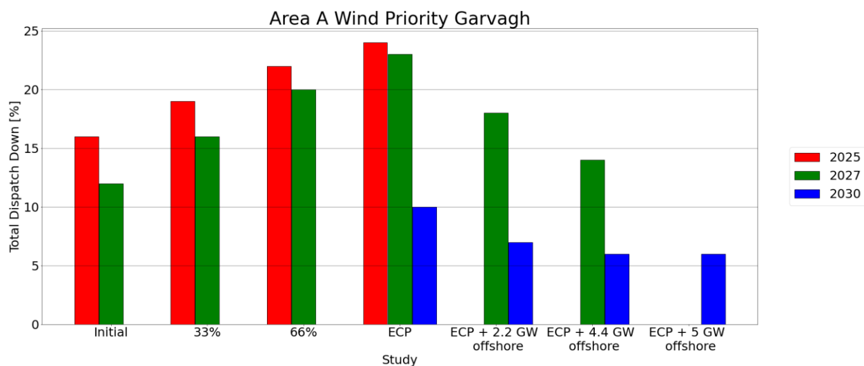
Figure C-18 - Total Dispatch Down for Wind priority
