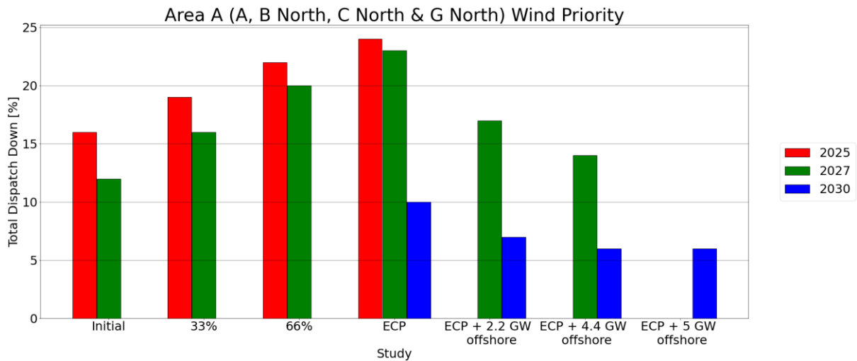
Figure 6-4 Results Wind Priority Area A (A, B North, C North & G North)
