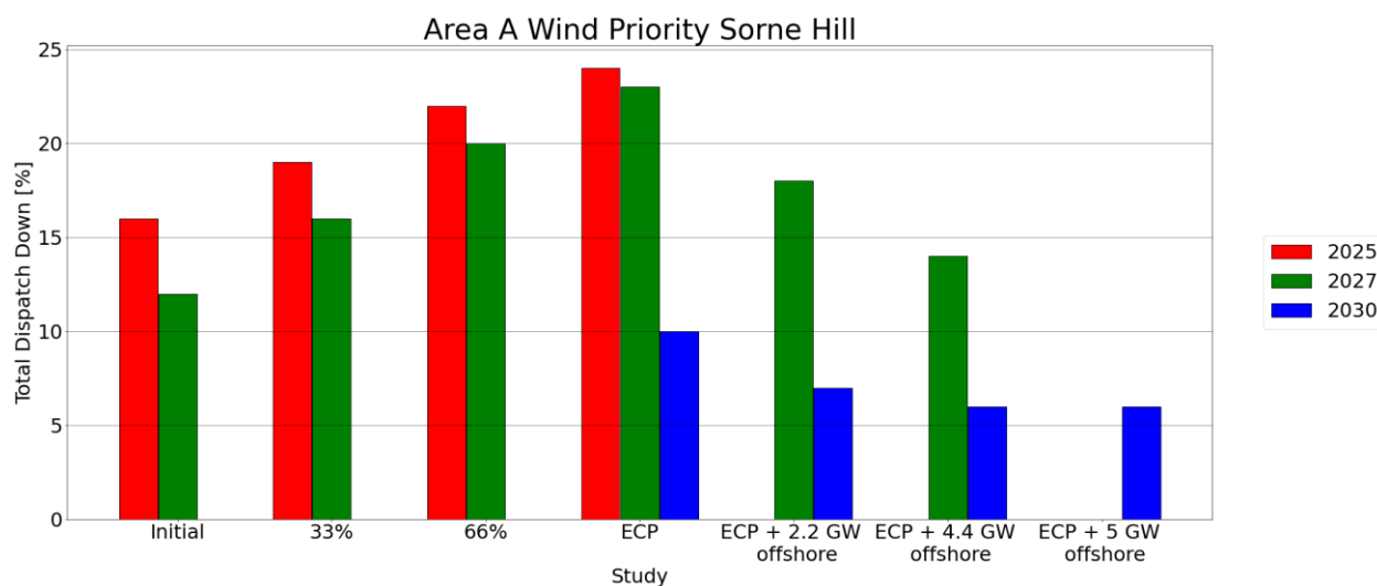
Figure C-33 - Total Dispatch Down for Wind priority
