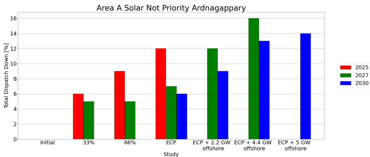
Figure C-2 - Total Dispatch Down for Solar not priority
