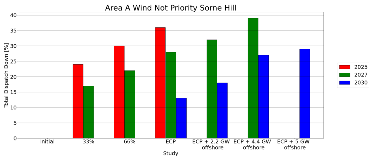
Figure C-32 - Total Dispatch Down for Wind not priority
