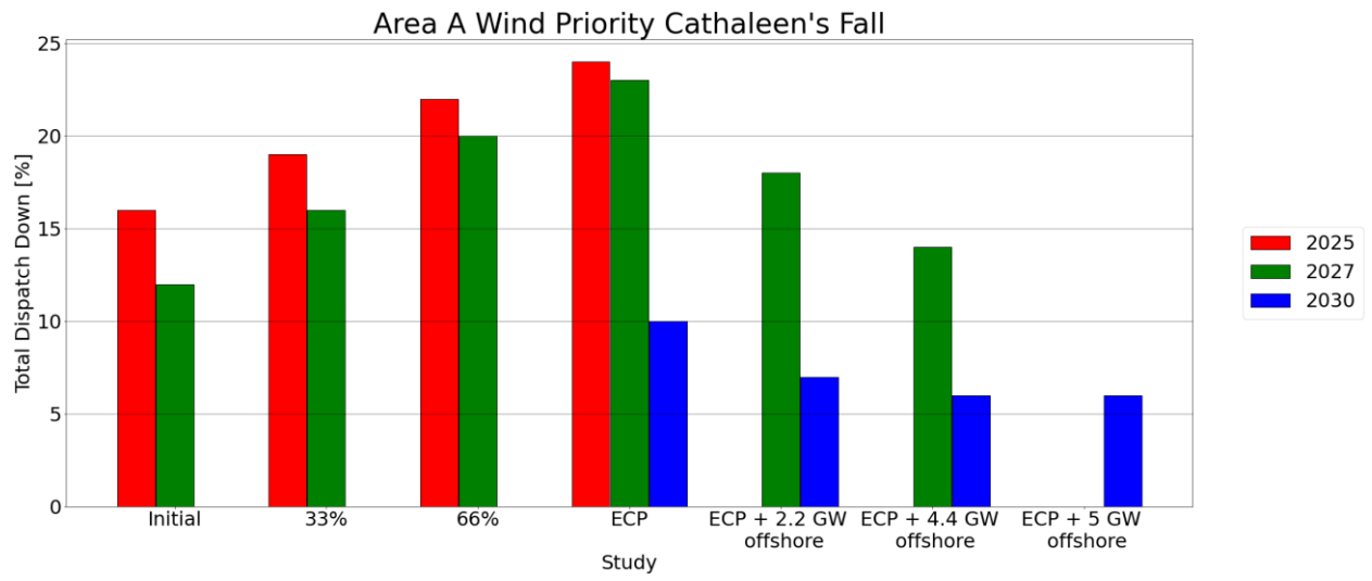
Figure C-9 - Total Dispatch Down for Wind priority
