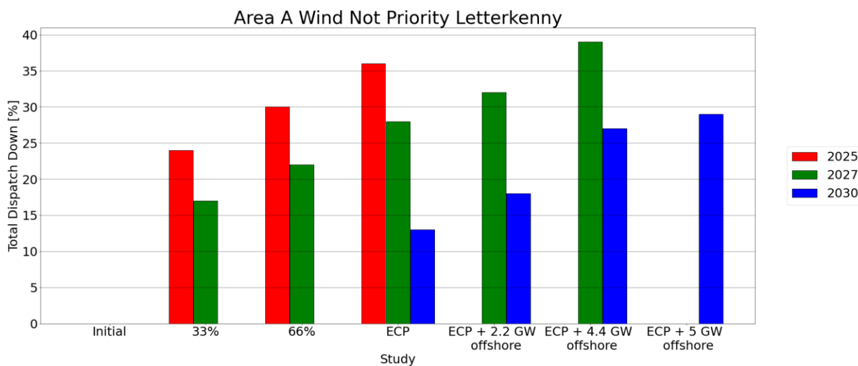
Figure C-26 - Total Dispatch Down for Wind not priority
