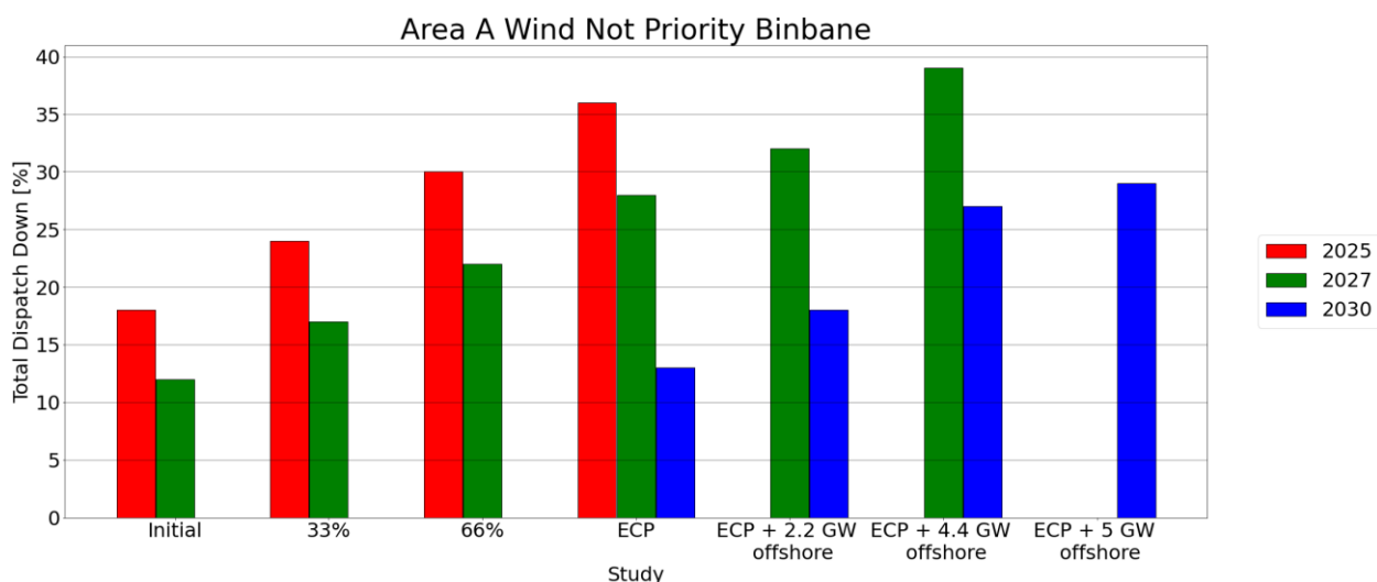
Figure C-5 - Total Dispatch Down for Wind not priority
