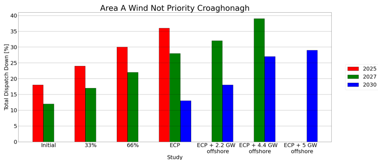
Figure C-15 - Total Dispatch Down for Wind not priority
