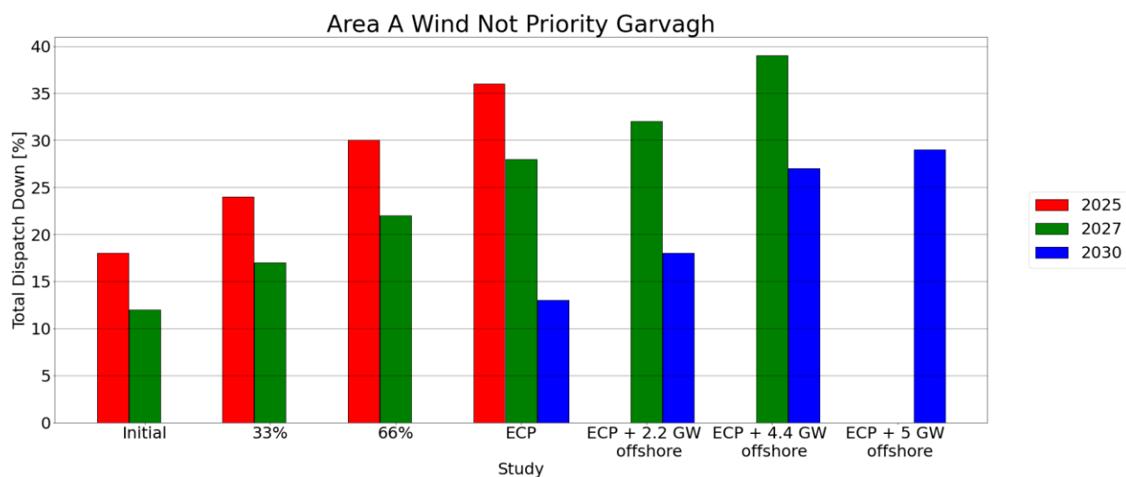
Figure C-17 - Total Dispatch Down for Wind not priority
