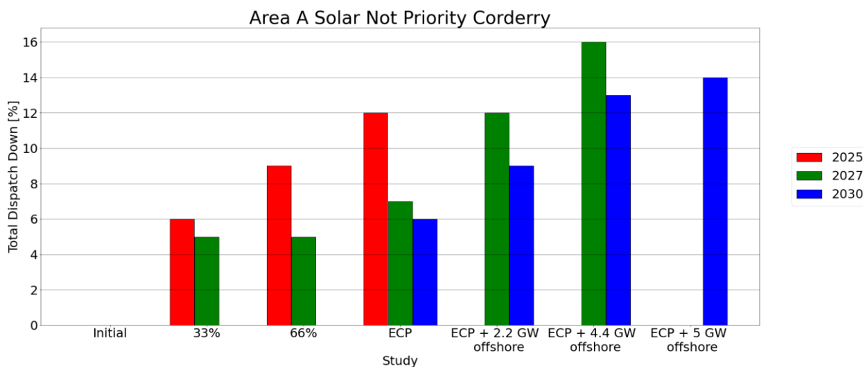
Figure C-11 - Total Dispatch Down for Solar not priority
