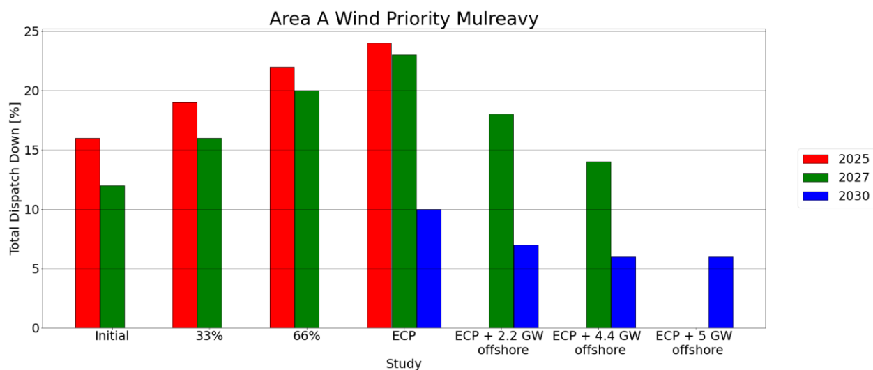
Figure C-30 - Total Dispatch Down for Wind priority
