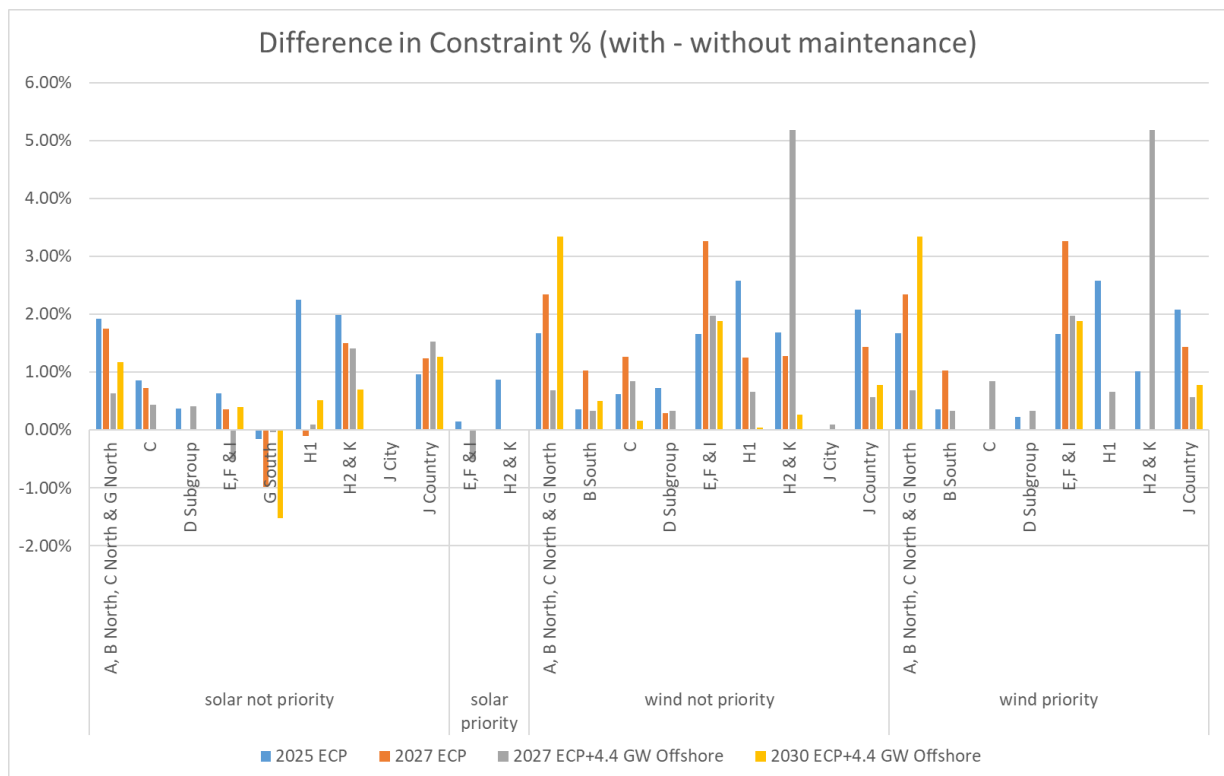
Figure 5-5 Difference in Constraint % (with - without maintenance)
