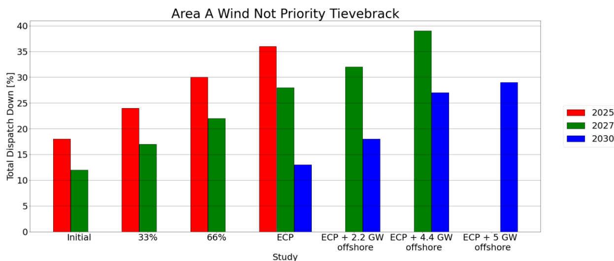
Figure C-35 - Total Dispatch Down for Wind not priority
