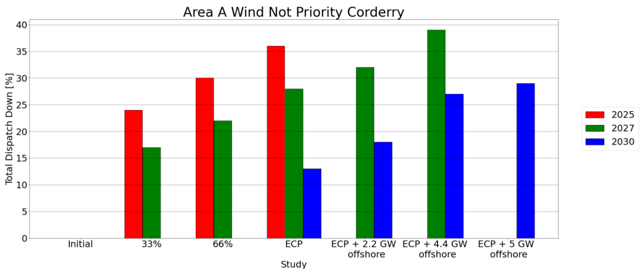
Figure C-12 - Total Dispatch Down for Wind not priority
