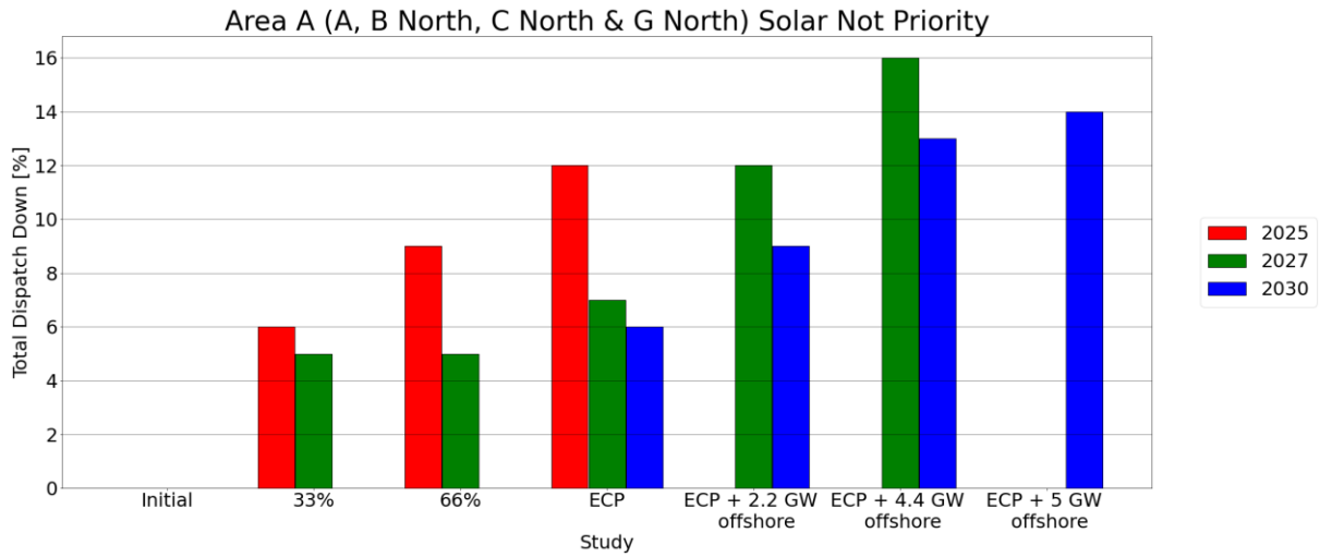
Figure 6-2 Results Solar Non-Priority Area A (A, B North, C North & G North)
