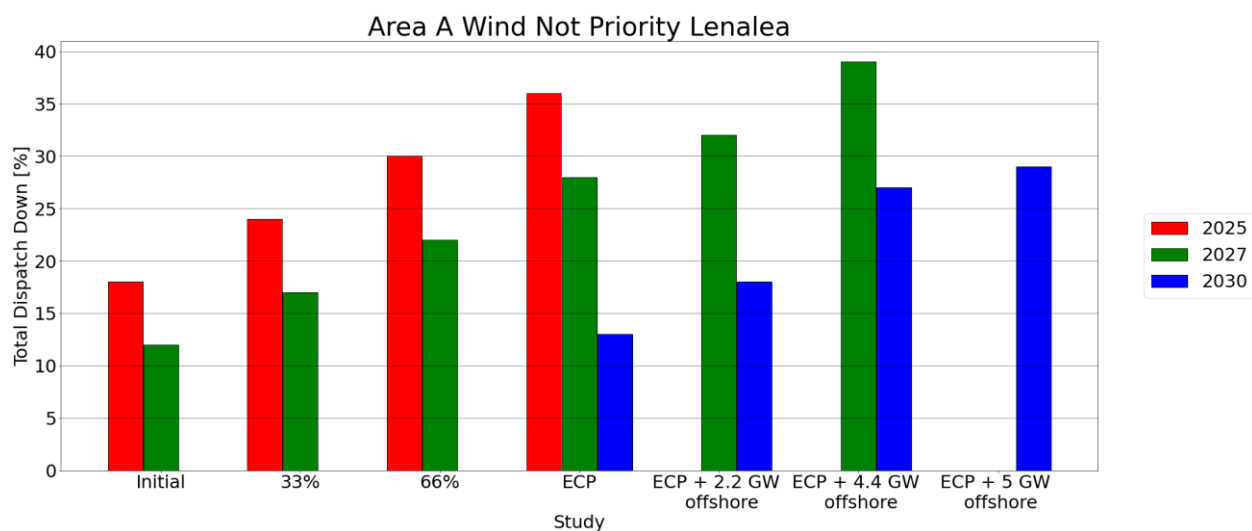
Figure C-24 - Total Dispatch Down for Wind not priority
