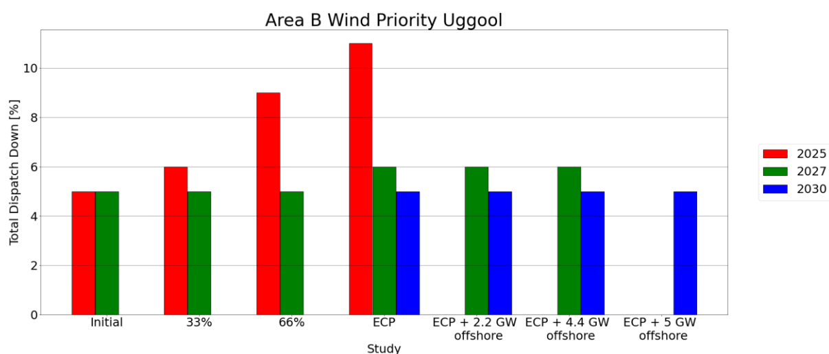
Figure C-39 - Total Dispatch Down for Wind priority
