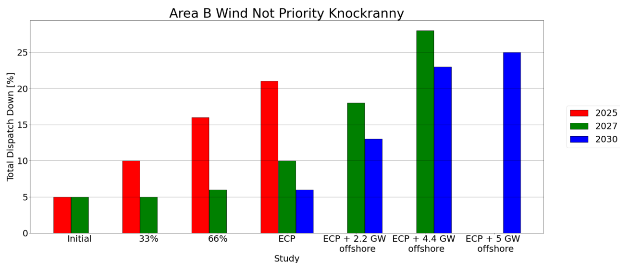
Figure C-23 - Total Dispatch Down for Wind not priority
