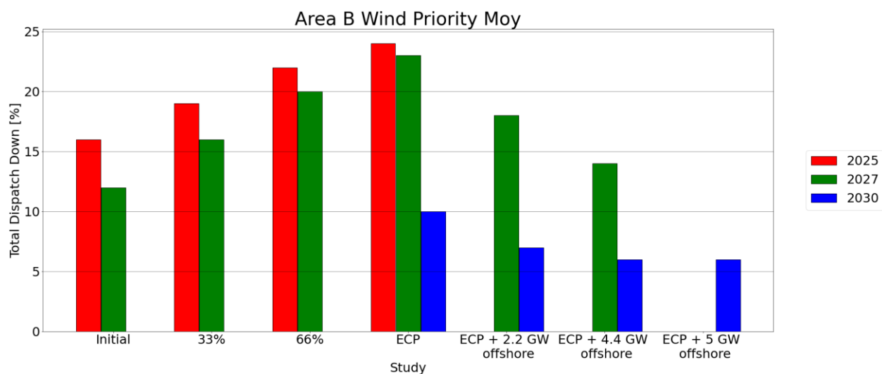
Figure C-26 - Total Dispatch Down for Wind priority
