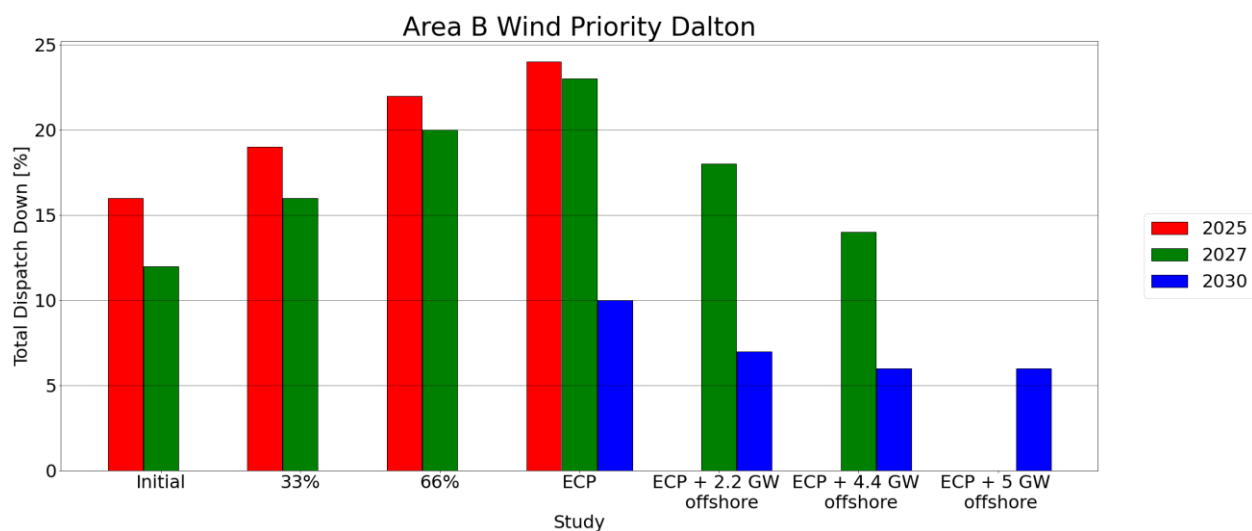
Figure C-16 - Total Dispatch Down for Wind priority
