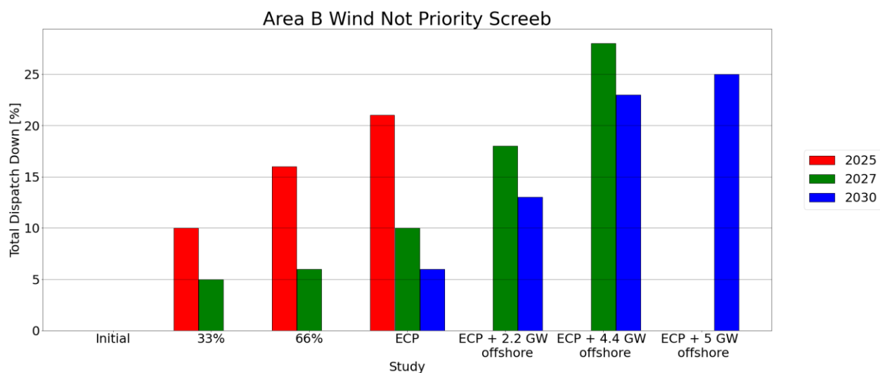
Figure C-30 - Total Dispatch Down for Wind not priority
