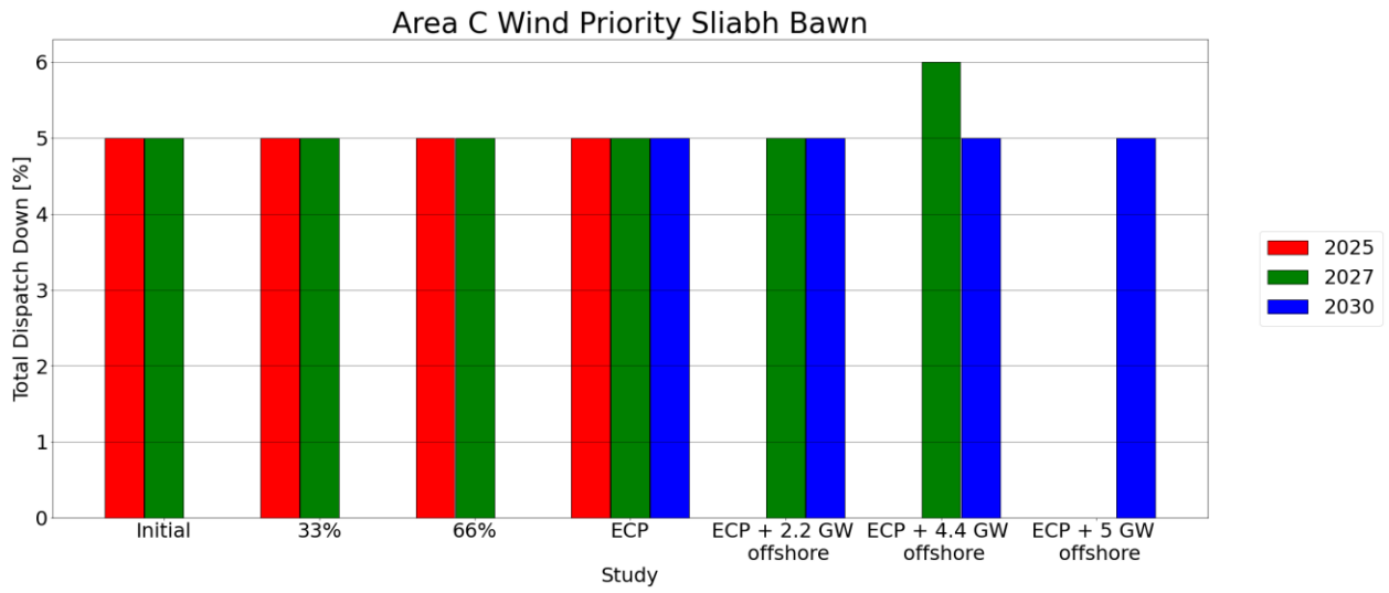
Figure C - 25 Total Dispatch Down for Wind Priority
