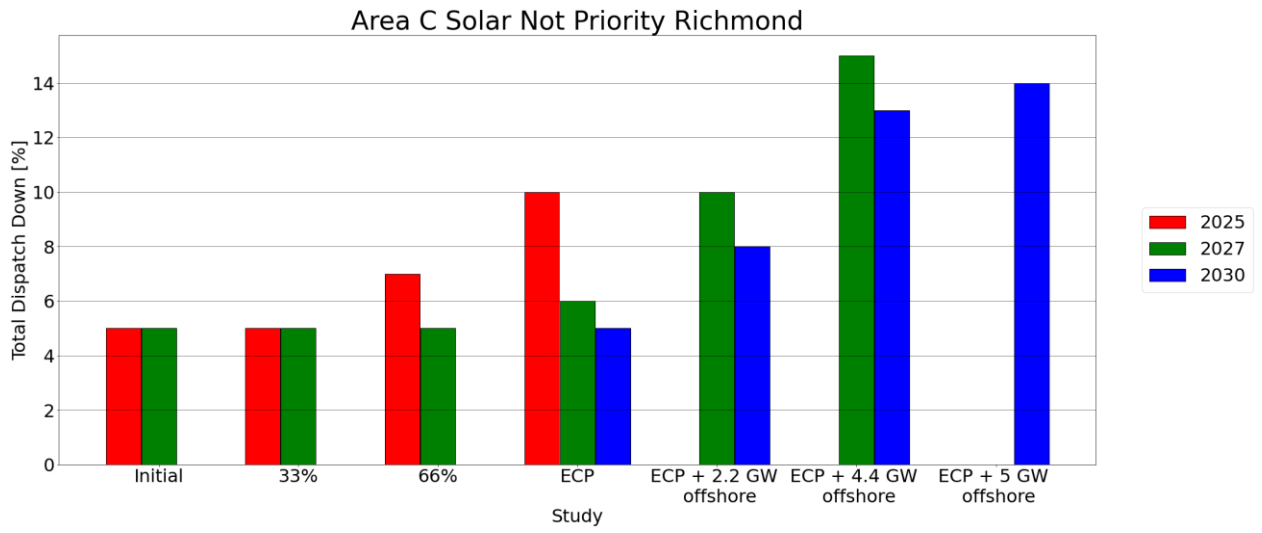
Figure C - 18 Total Dispatch Down for Solar Not Priority
