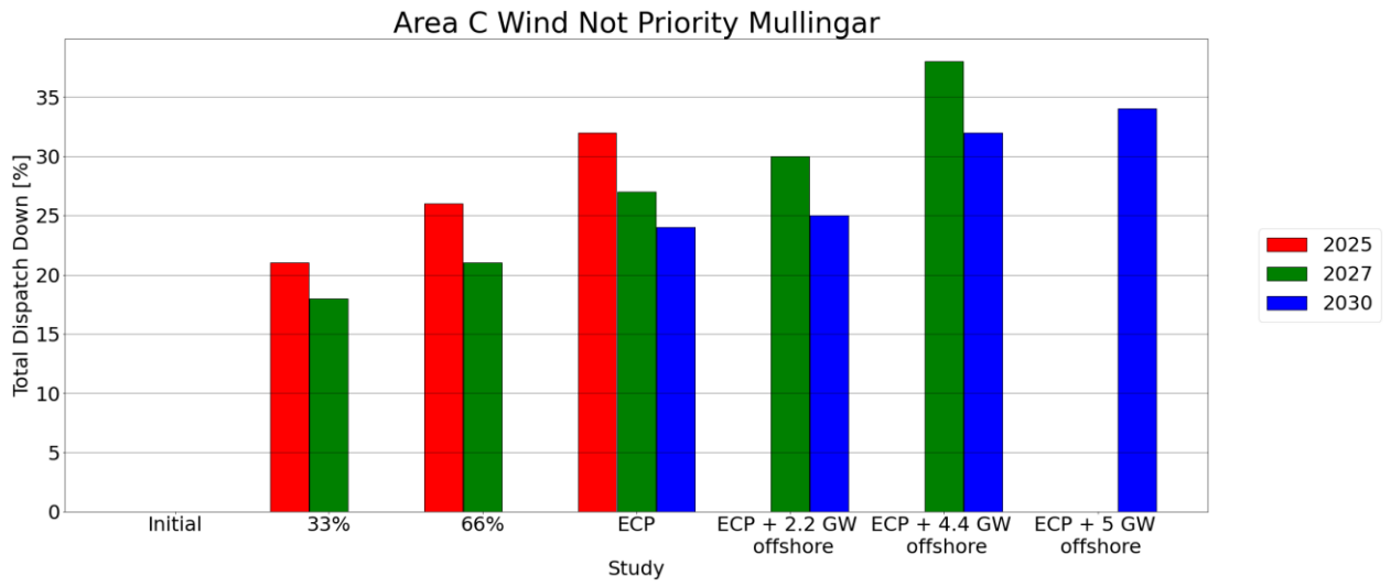
Figure C - 16 Total Dispatch Down for Wind Not Priority
