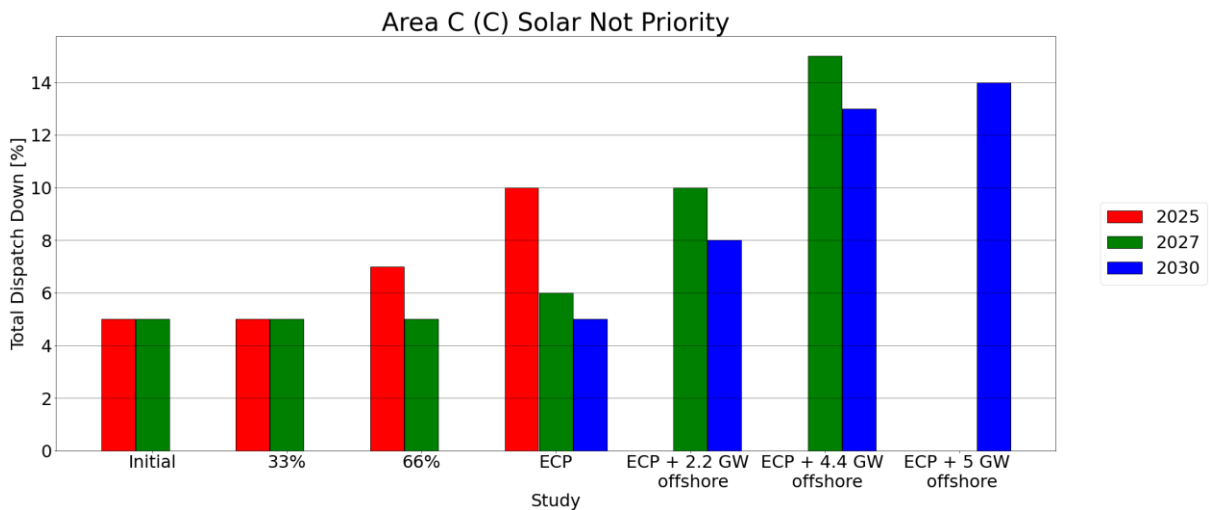
Figure 6-2 Results Solar Not Priority Area C (C South)
