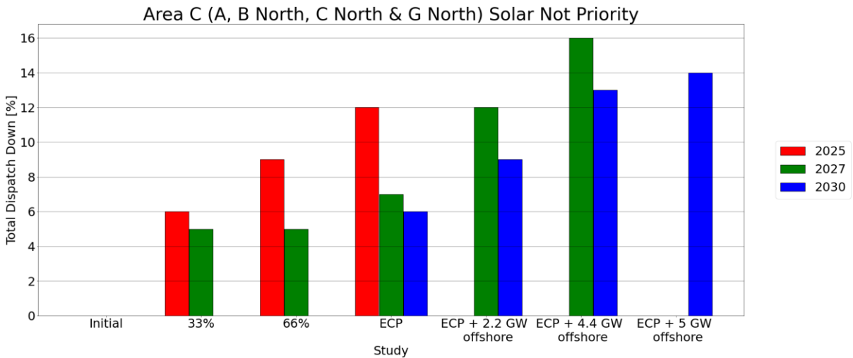
Figure 6-5 Results Solar Not Priority in Area C (A, B North, C North & G North)
