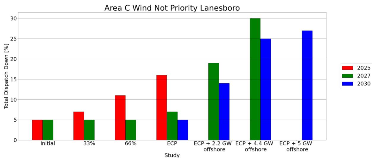
Figure C-13 - Total Dispatch Down for Wind not priority
