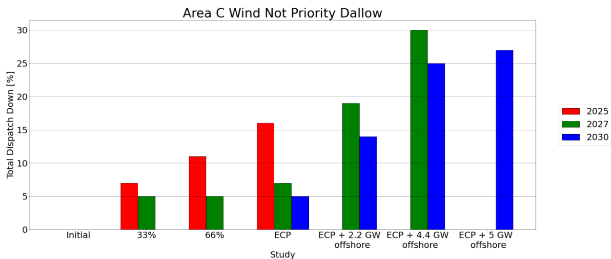
Figure C-7 - Total Dispatch Down for Wind not priority
