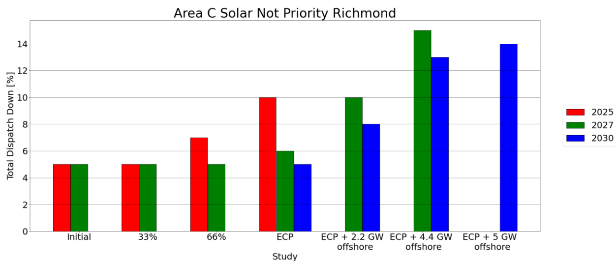
Figure C-18 - Total Dispatch Down for Solar not priority
