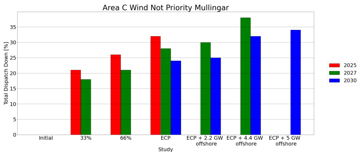
Figure C-16 - Total Dispatch Down for Wind not priority
