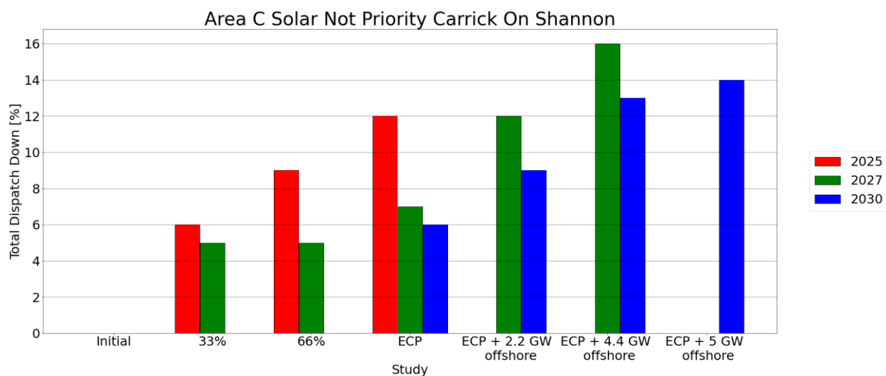
Figure C-5 - Total Dispatch Down for Solar not priority
