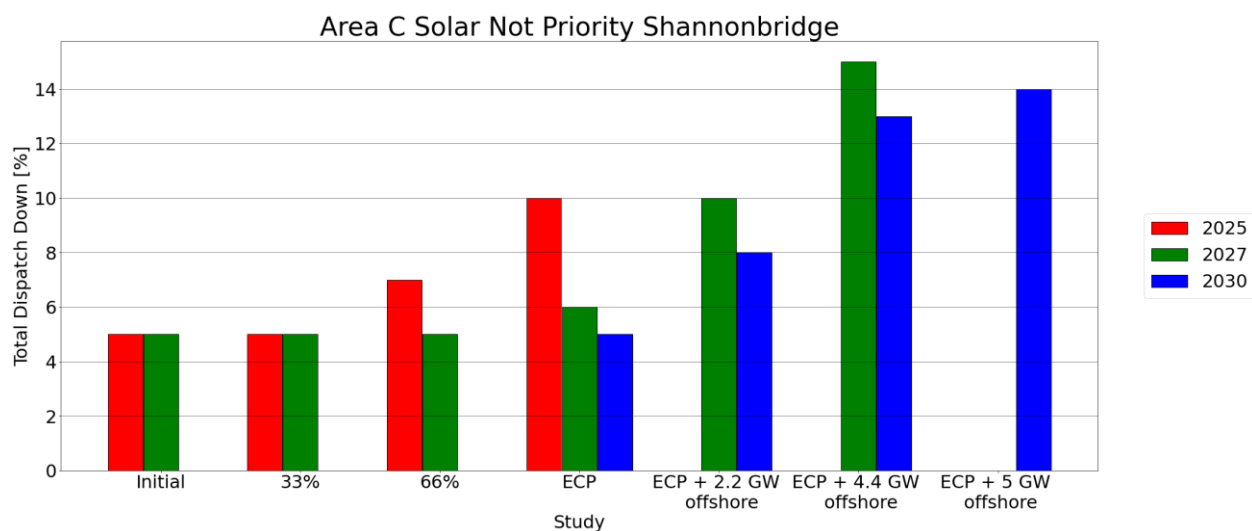
Figure C-21 - Total Dispatch Down for Solar not priority
