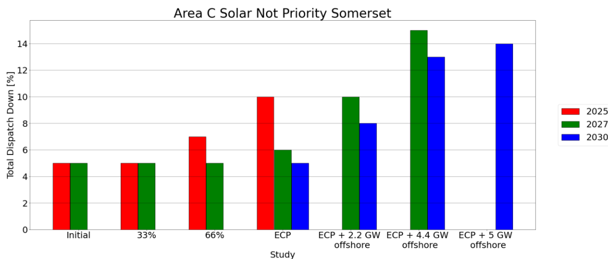
Figure C-27 - Total Dispatch Down for Solar not priority
