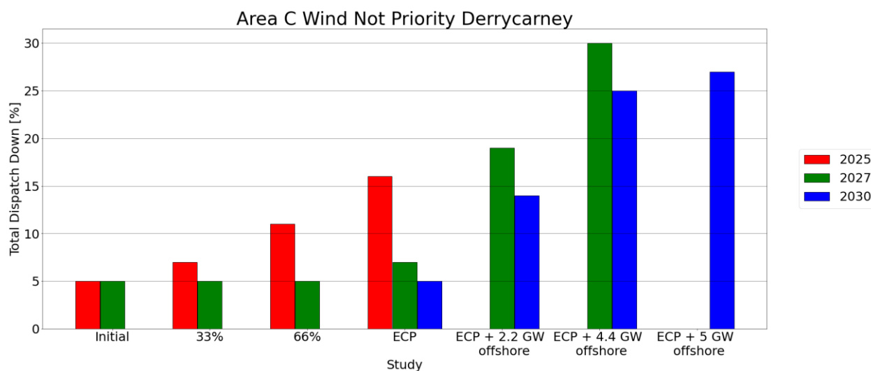
Figure C-10 - Total Dispatch Down for Wind not priority
