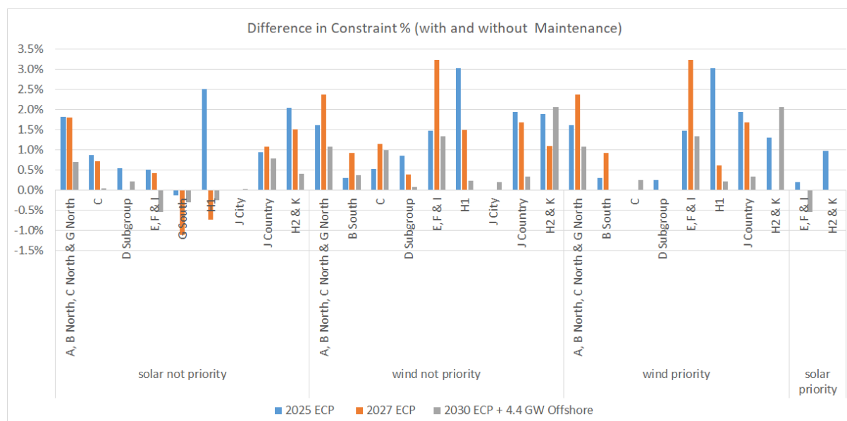
Figure 5-5 Difference in Constraint % (with - without maintenance)
