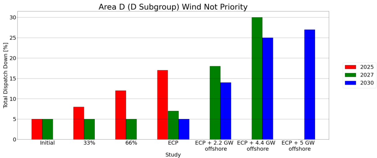
Figure 6-3 Results Wind Not Priority in Area D
