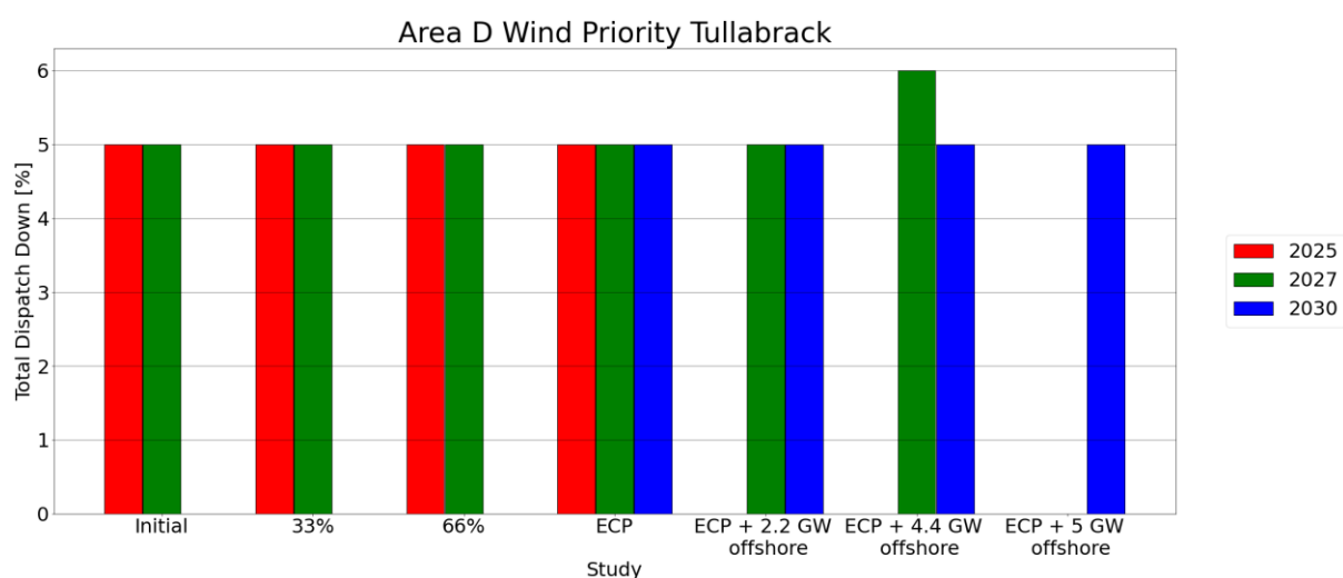
Figure C-17 - Total Dispatch Down for Wind priority
