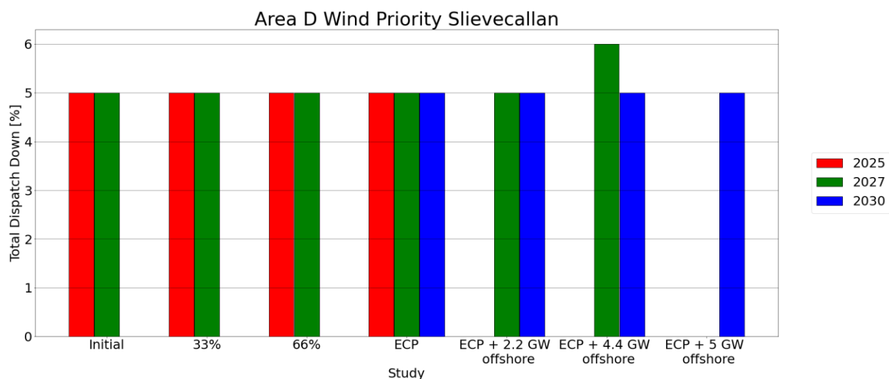
Figure C-14 - Total Dispatch Down for Wind priority
