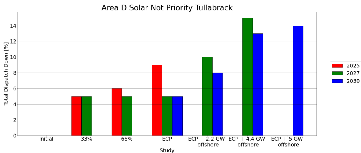
Figure C-16 - Total Dispatch Down for Solar not priority
