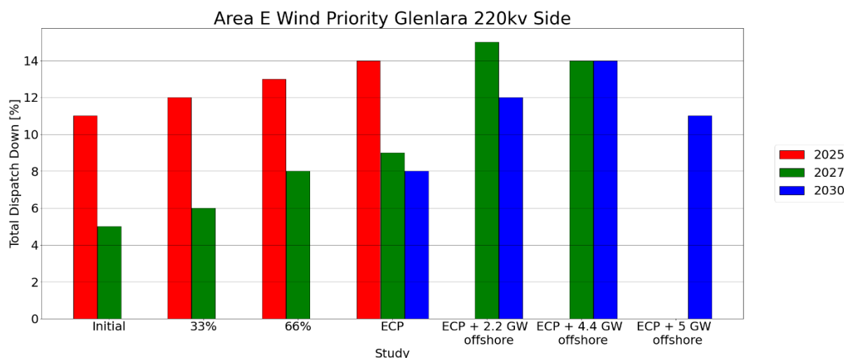
Figure C - 41 Total Dispatch Down for Wind Priority
