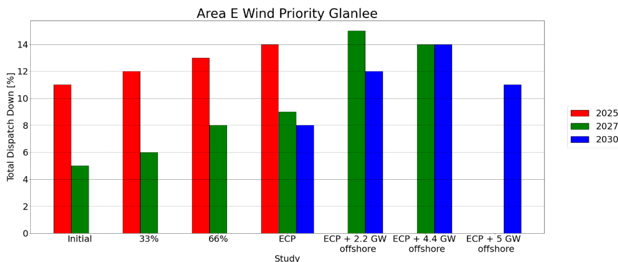
Figure C - 35 Total Dispatch Down for Wind Priority
