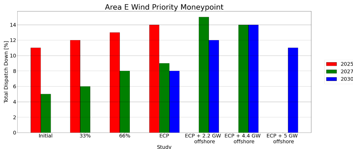
Figure C - 56 Total Dispatch Down for Wind Priority
