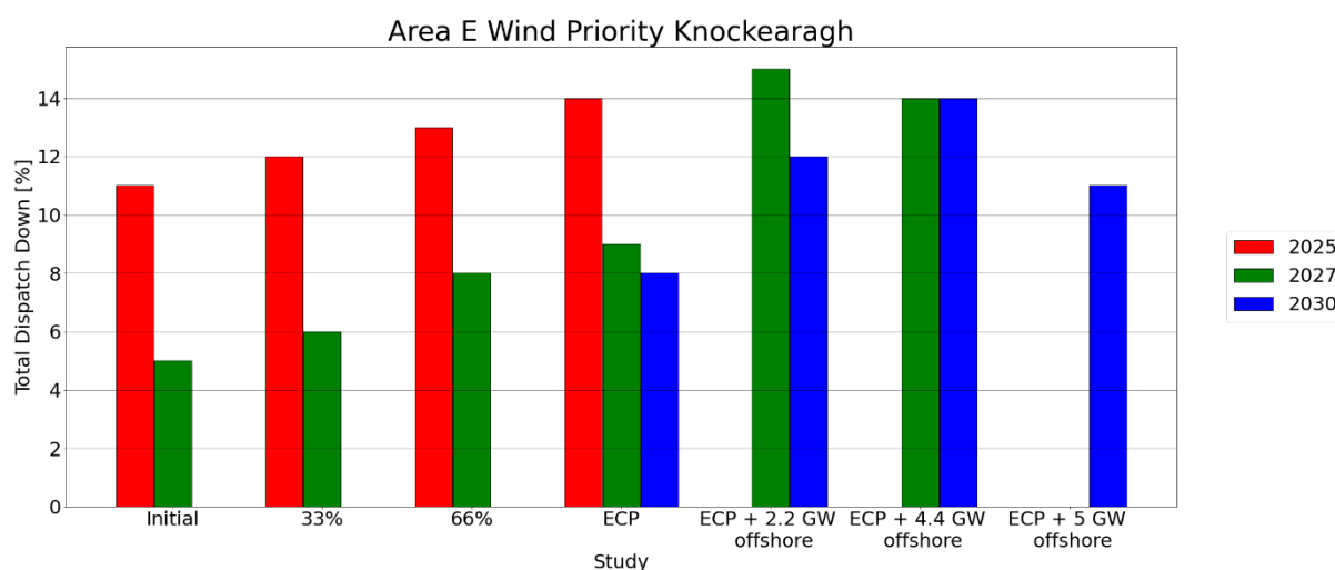
Figure C - 48 Total Dispatch Down for Wind Priority
