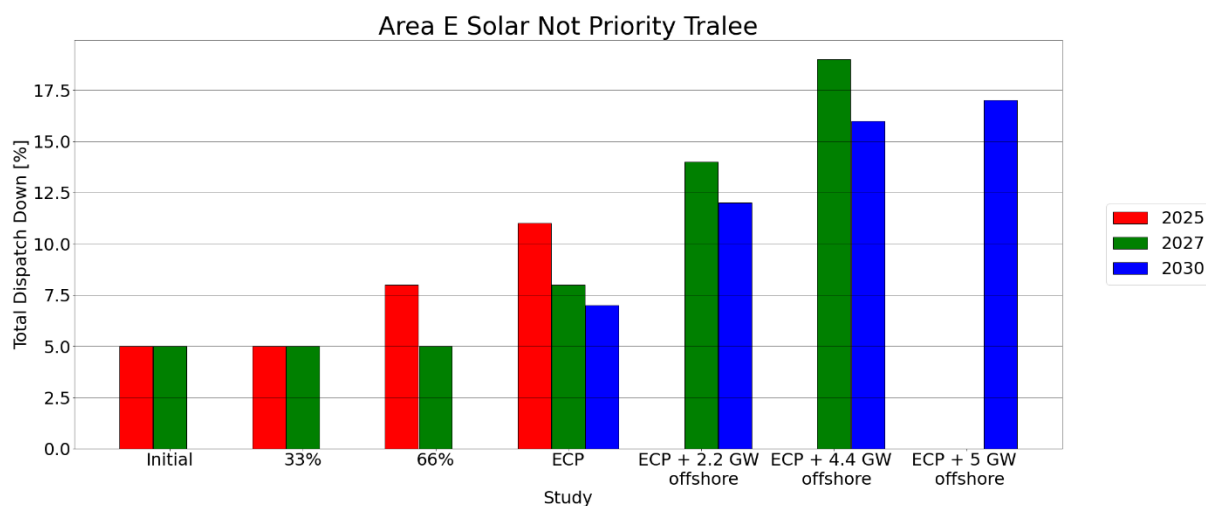
Figure C - 69 Total Dispatch Down for Solar Not Priority
