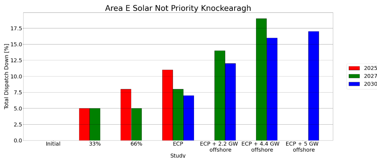
Figure C - 47 Total Dispatch Down for Solar Not Priority
