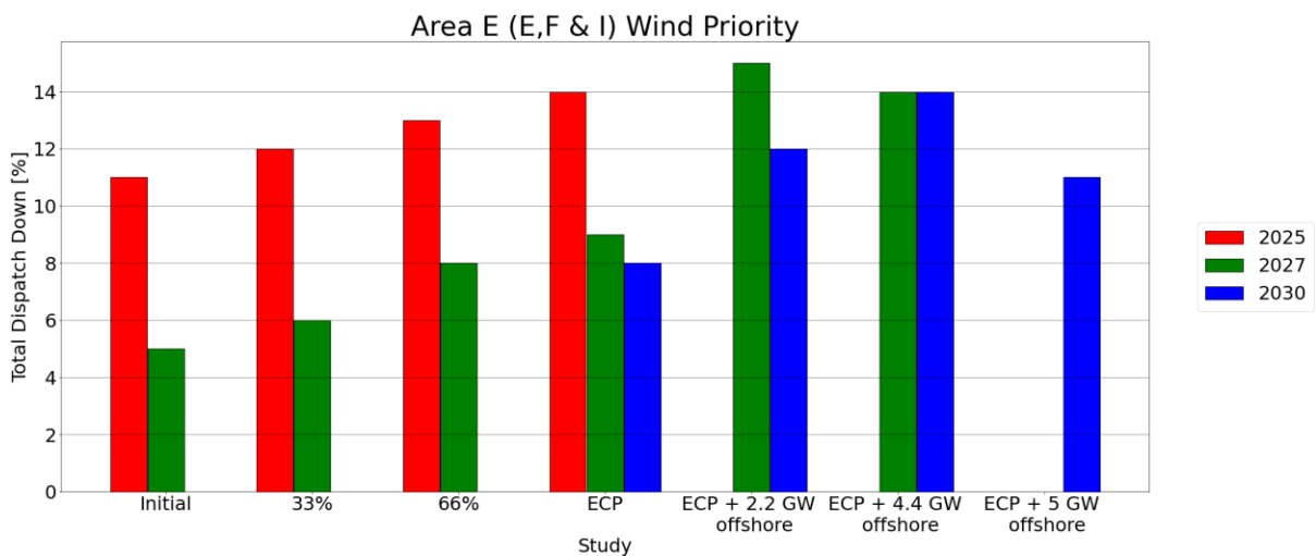
Figure 6-5 Results Wind Priority Area E (E F & I)
