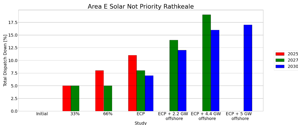
Figure C - 63 Total Dispatch Down for Solar Not Priority
