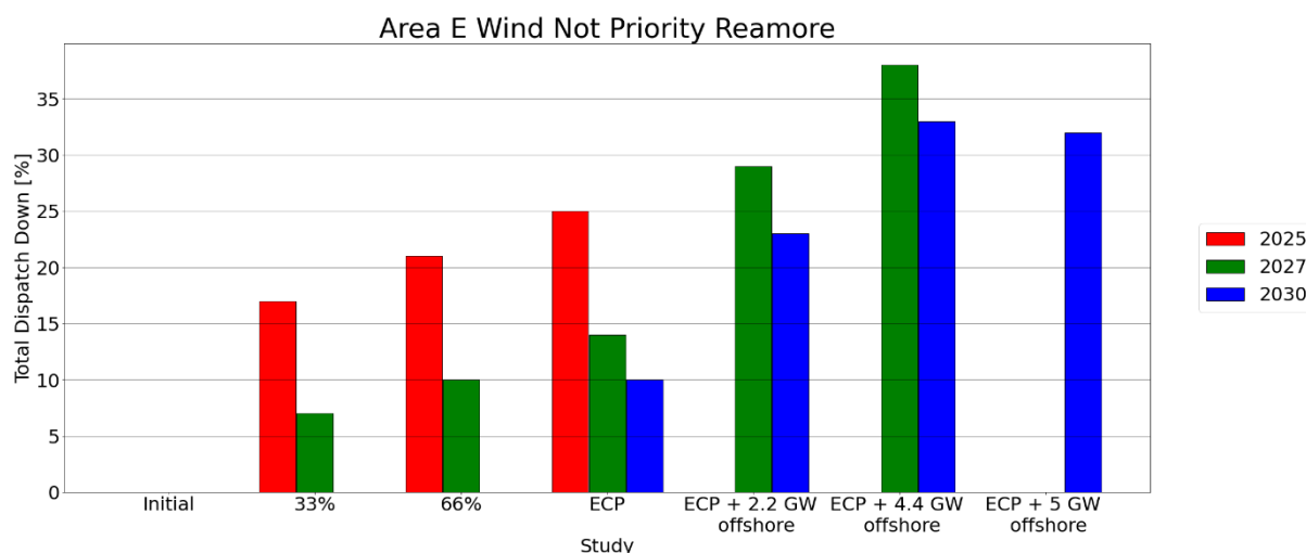
Figure C - 66 Total Dispatch Down for Wind Not Priority
