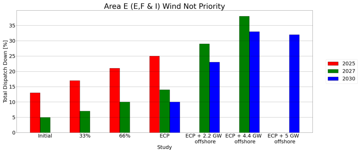
Figure 6-3 Results Wind Not Priority in Area E (E F & I)
