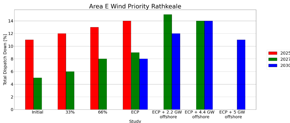
Figure C - 64 Total Dispatch Down for Wind Priority
