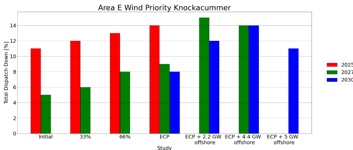
Figure C - 45 Total Dispatch Down for Wind Priority
