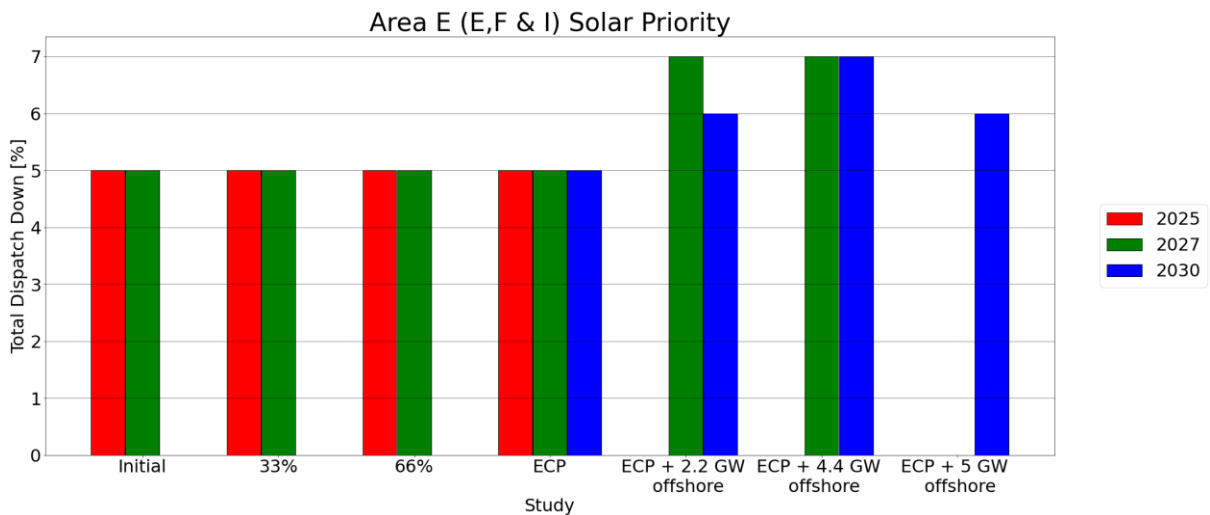
Figure 6-4 Results Solar Priority Area E (E F & I)
