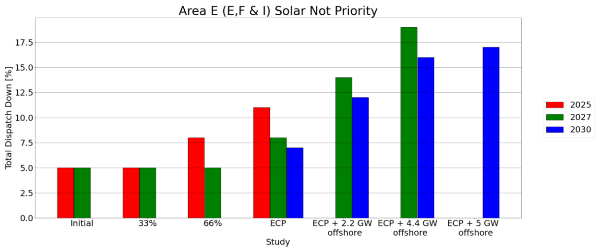
Figure 6-2 Results Solar Not Priority Area E (E F & I)
