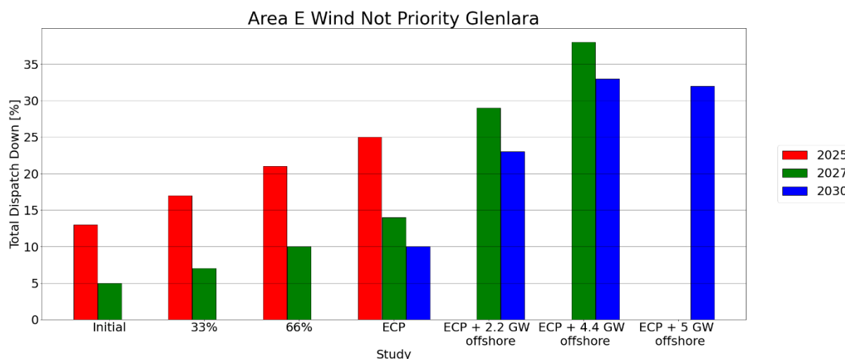
Figure C - 38 Total Dispatch Down for Wind Not Priority
