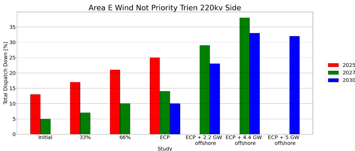
Figure C - 75 Total Dispatch Down for Wind Not Priority
