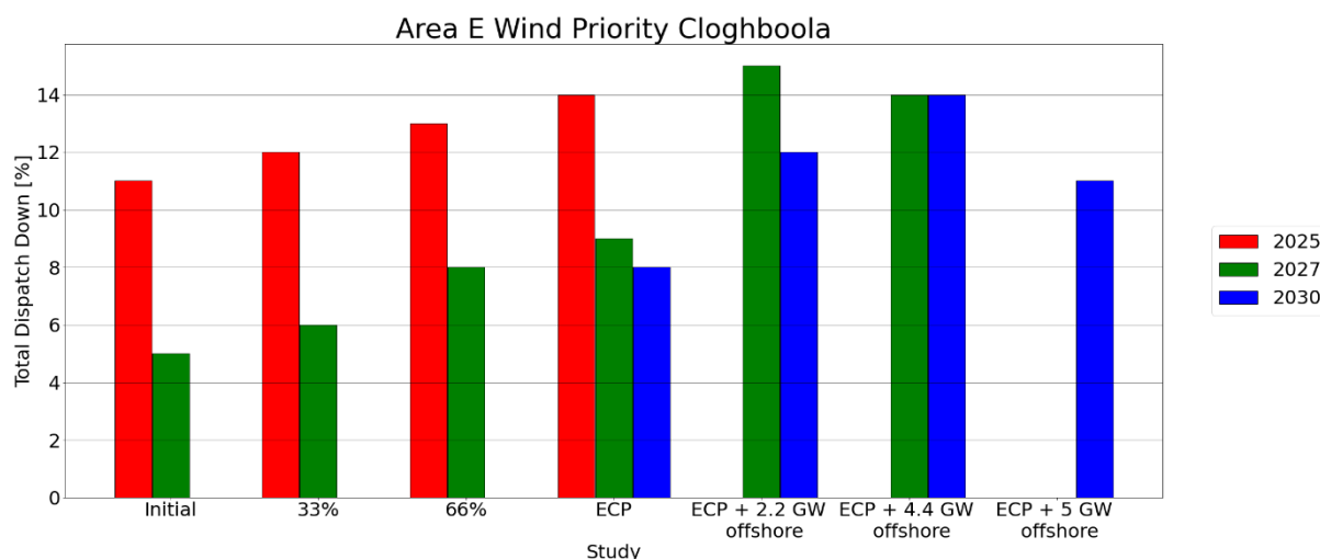
Figure C - 19 Total Dispatch Down for Wind Priority
