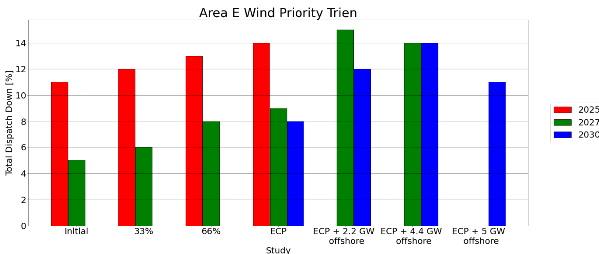
Figure C - 73 Total Dispatch Down for Wind Priority
