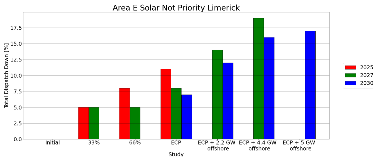
Figure C - 50 Total Dispatch Down for Solar Not Priority
