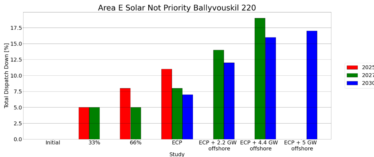
Figure C - 7 Total Dispatch Down for Solar Not Priority
