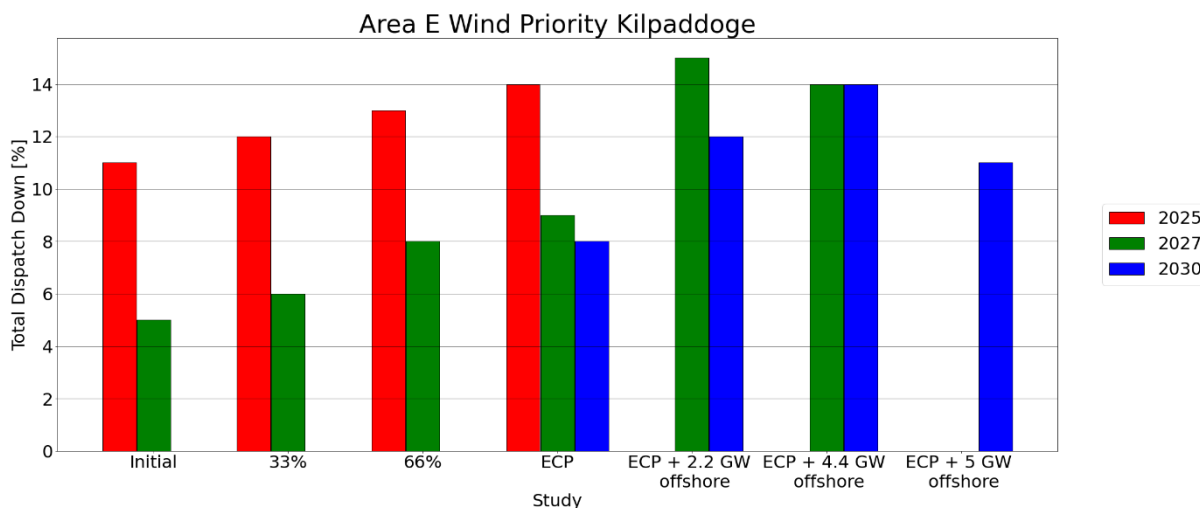
Figure C - 43 Total Dispatch Down for Wind Priority
