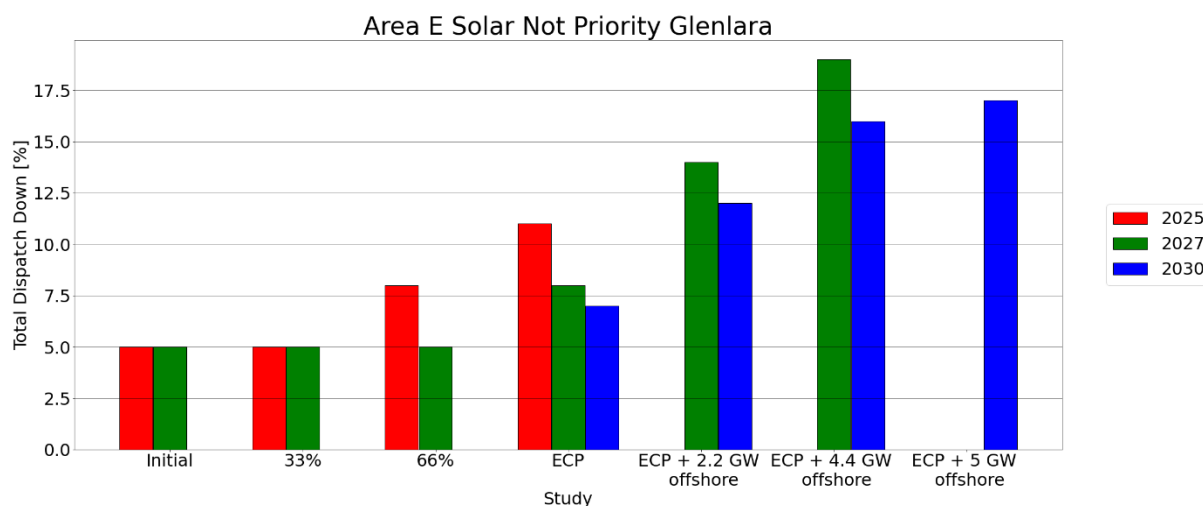
Figure C - 37 Total Dispatch Down for Solar Not Priority
