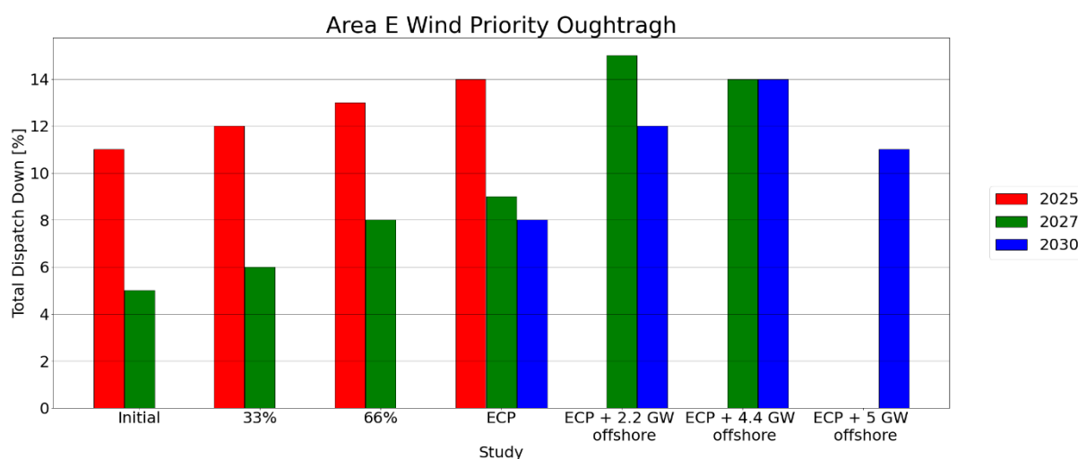
Figure C - 61 Total Dispatch Down for Wind Priority
