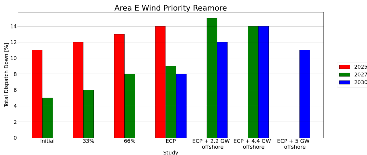
Figure C - 67 Total Dispatch Down for Wind Priority
