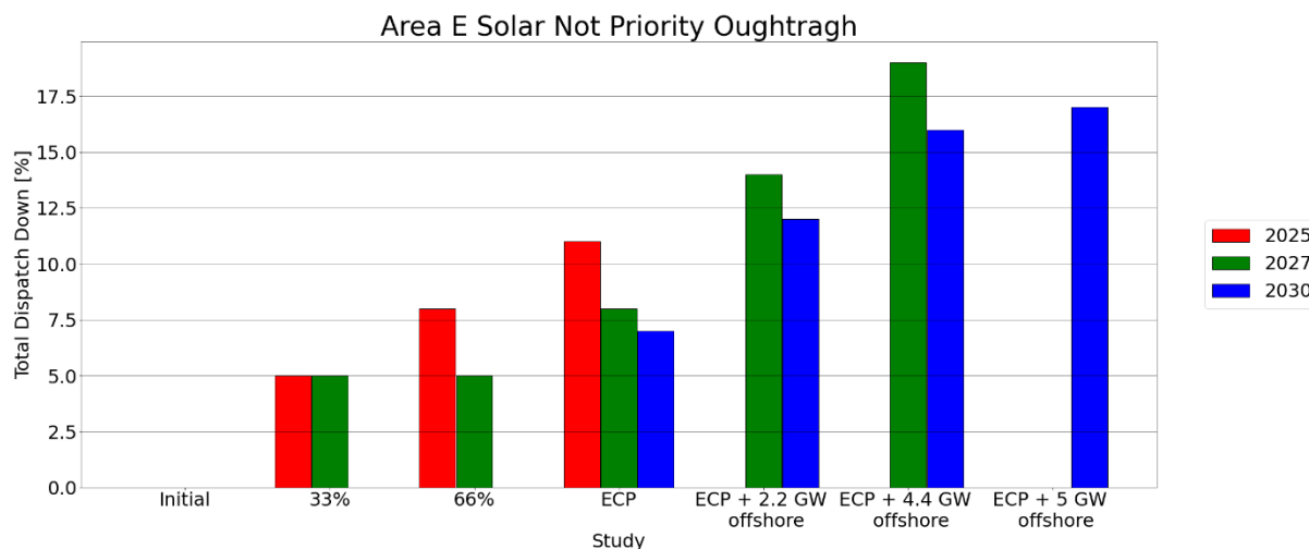
Figure C - 60 Total Dispatch Down for Solar Not Priority
