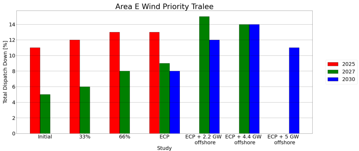
Figure C-70 - Total Dispatch Down for Wind priority
