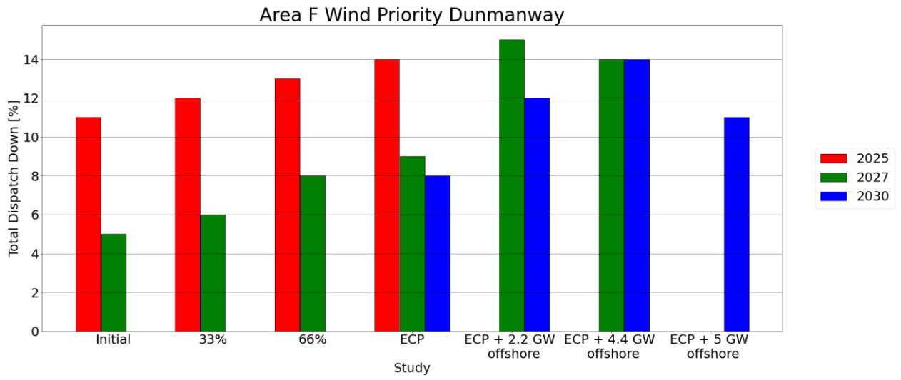
Figure C - 10 Total Dispatch Down for Wind Priority
