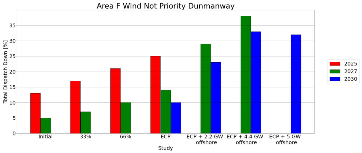
Figure C - 9 Total Dispatch Down for Wind Not Priority
