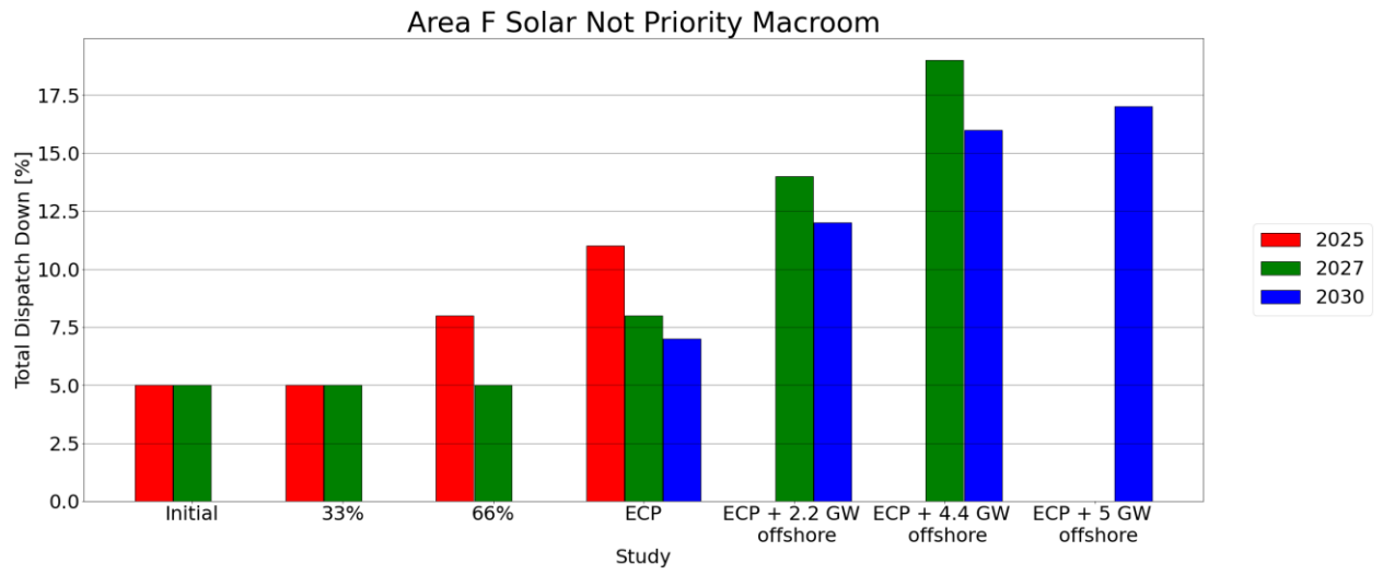
Figure C - 12 Total Dispatch Down for Solar Not Priority
