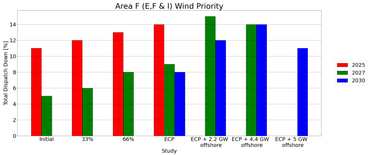
Figure 6-4 Results Wind Priority Area F (E F & I)
