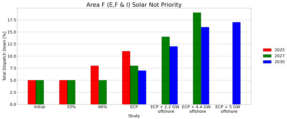
Figure 6-2 Results Solar Not Priority Area F (E F & I)
