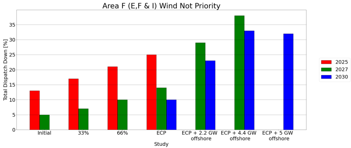
Figure 6-3 Results Wind Not Priority in Area F (E F & I)
