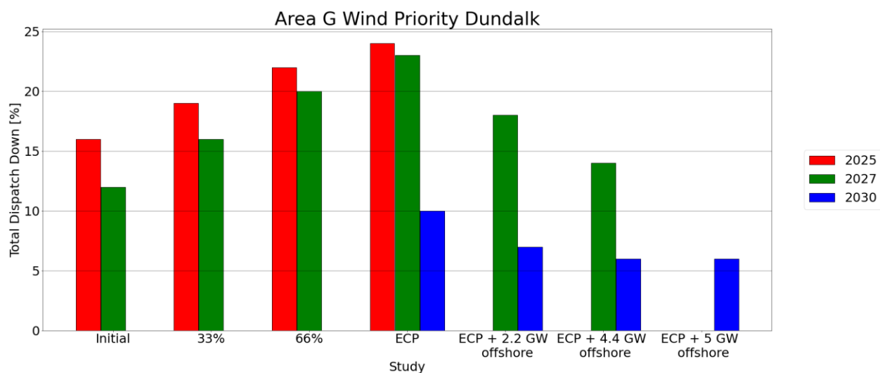
Figure C-7 - Total Dispatch Down for Wind priority
