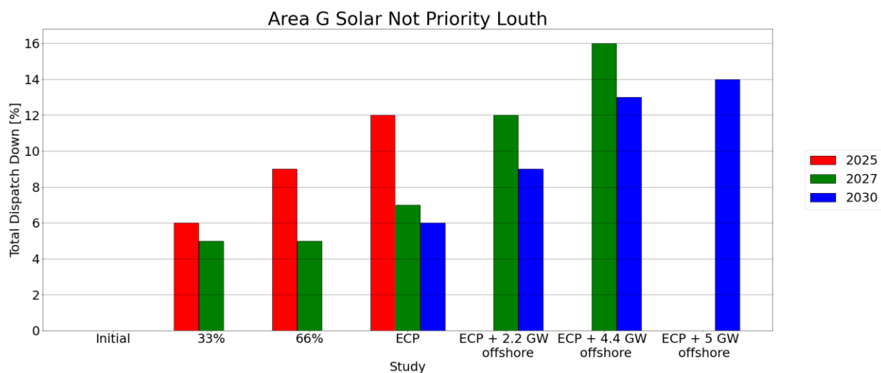
Figure C-19 - Total Dispatch Down for Solar not priority
