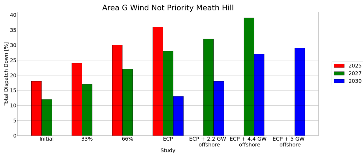
Figure C-21 - Total Dispatch Down for Wind not priority
