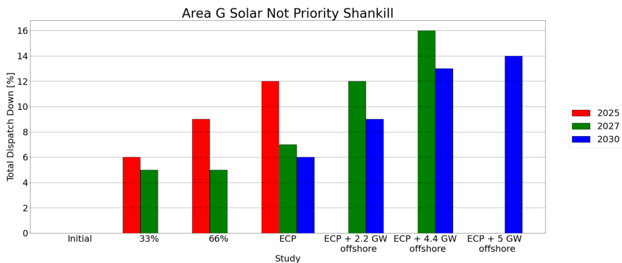
Figure C-30 - Total Dispatch Down for Solar not priority
