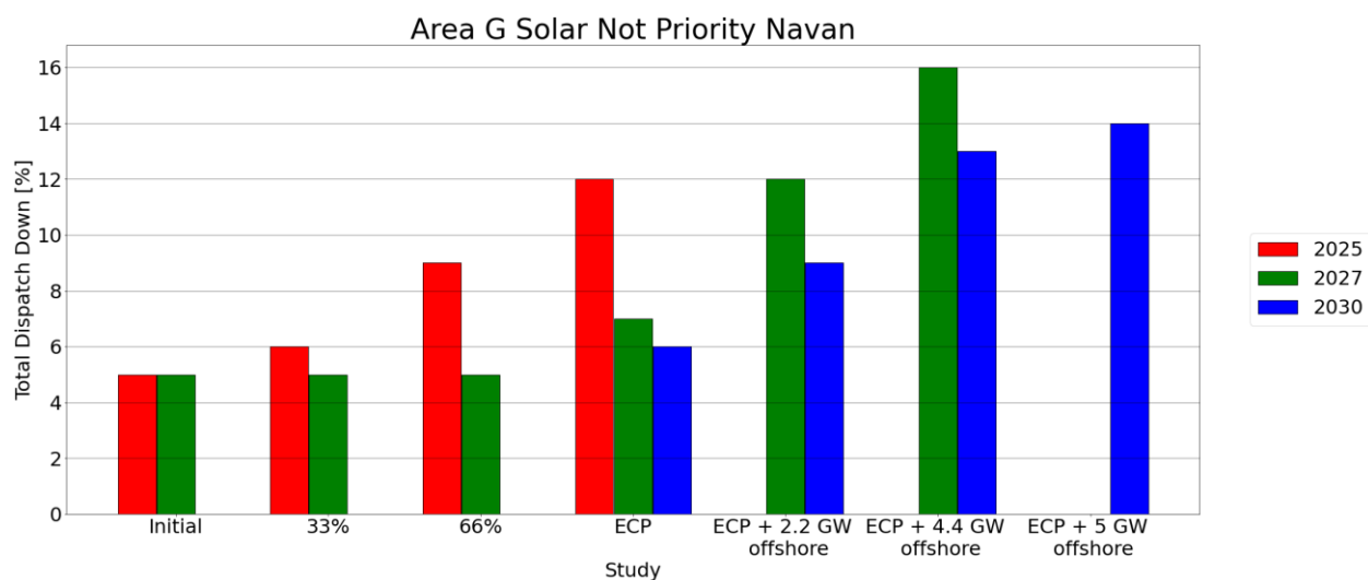
Figure C-24 - Total Dispatch Down for Solar not priority
