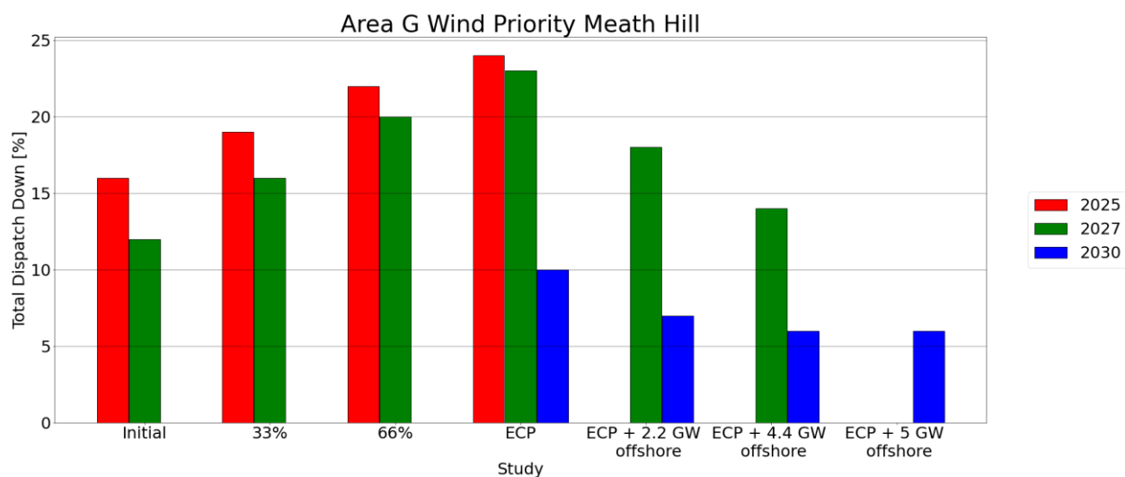
Figure C-22 - Total Dispatch Down for Wind priority
