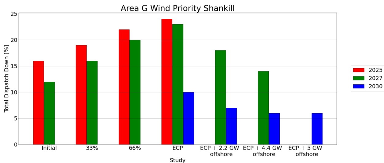
Figure C-31 - Total Dispatch Down for Wind priority
