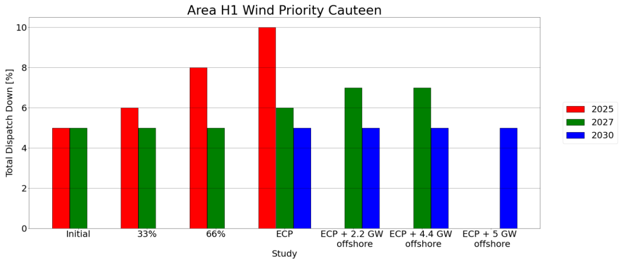
Figure C - 11 Total Dispatch Down for Wind Priority
