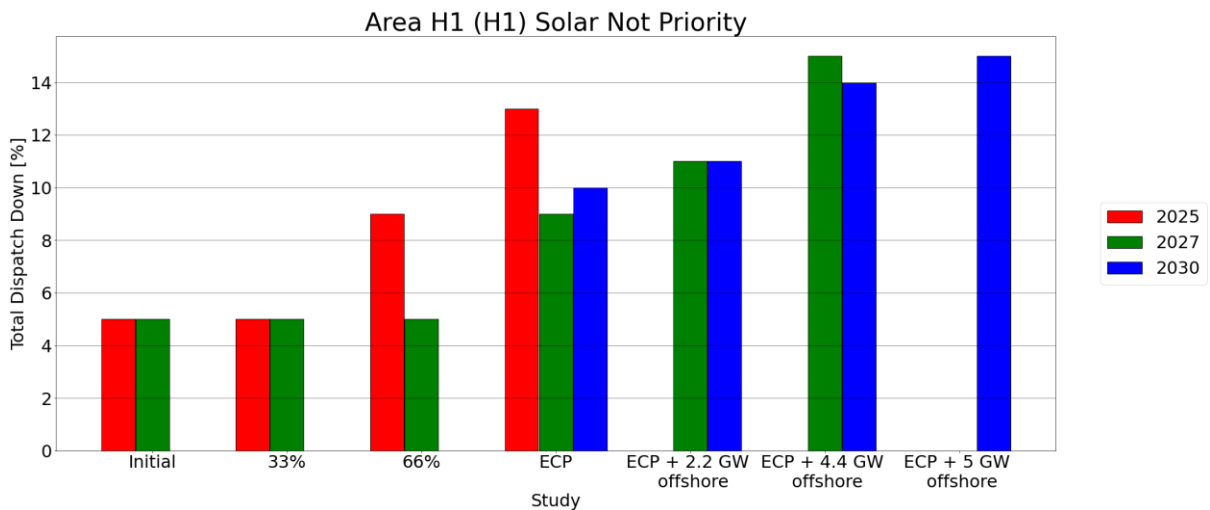
Figure 6-2 Results Solar Not Priority Area H1 (H1)
