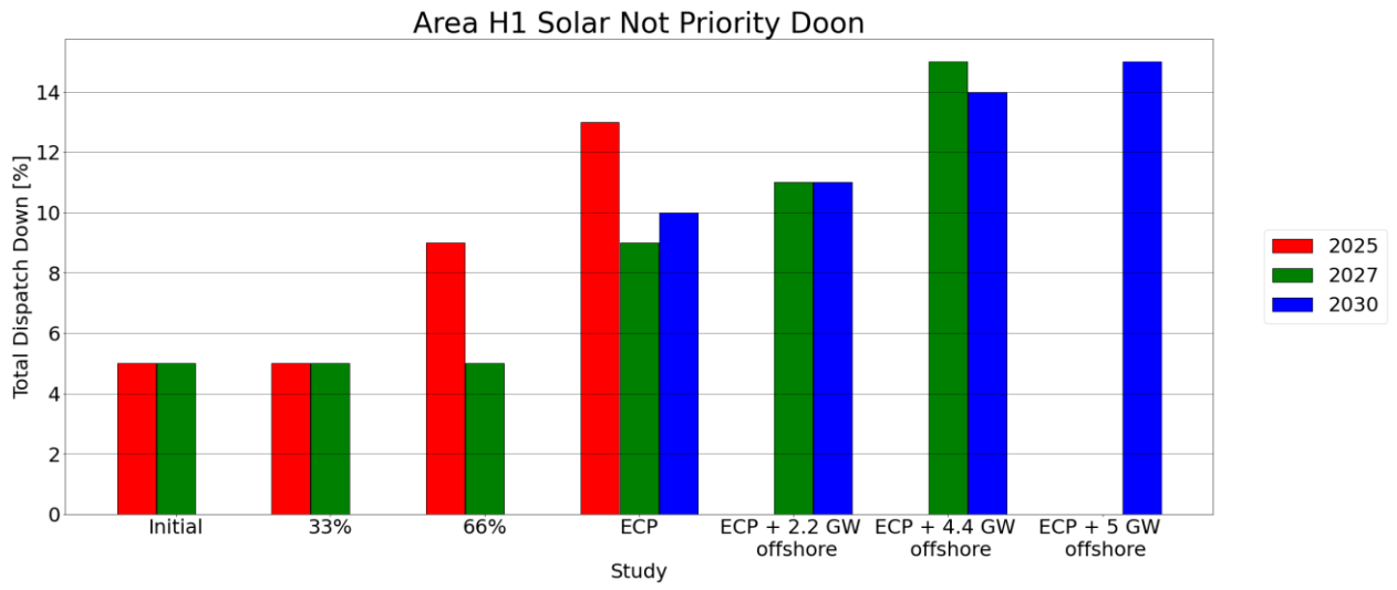
Figure C - 13 Total Dispatch Down for Solar Not Priority
