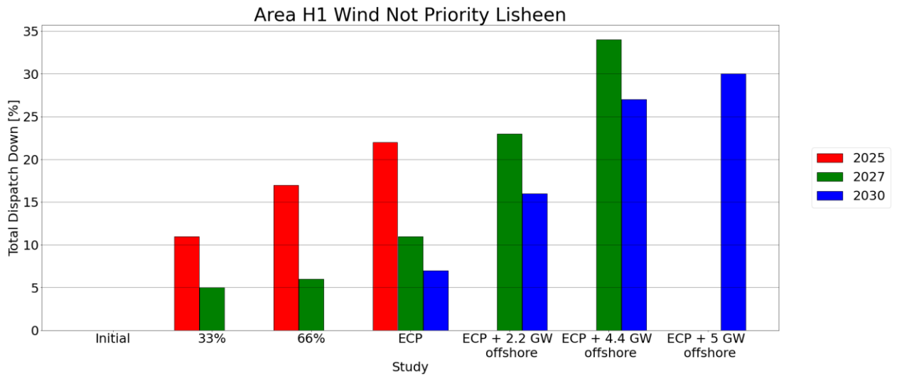
Figure C - 22 Total Dispatch Down for Wind Not Priority
