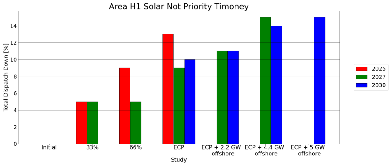
Figure C - 33 Total Dispatch Down for Solar Not Priority
