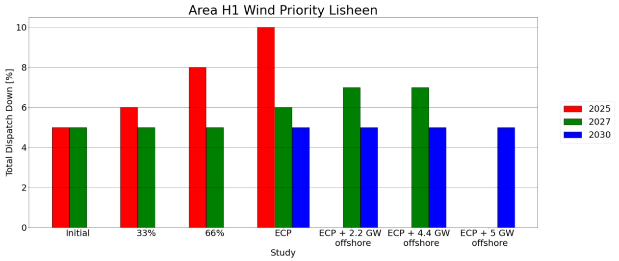
Figure C - 23 Total Dispatch Down for Wind Priority
