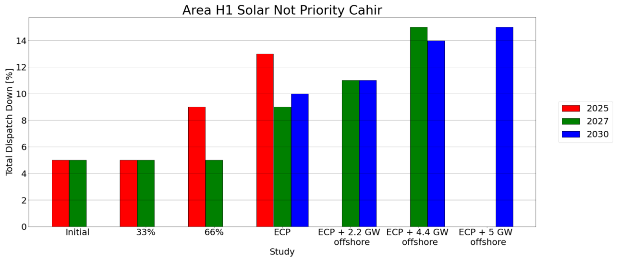
Figure C - 9 Total Dispatch Down for Solar Not Priority
