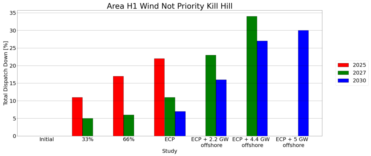
Figure C - 17 Total Dispatch Down for Wind Not Priority
