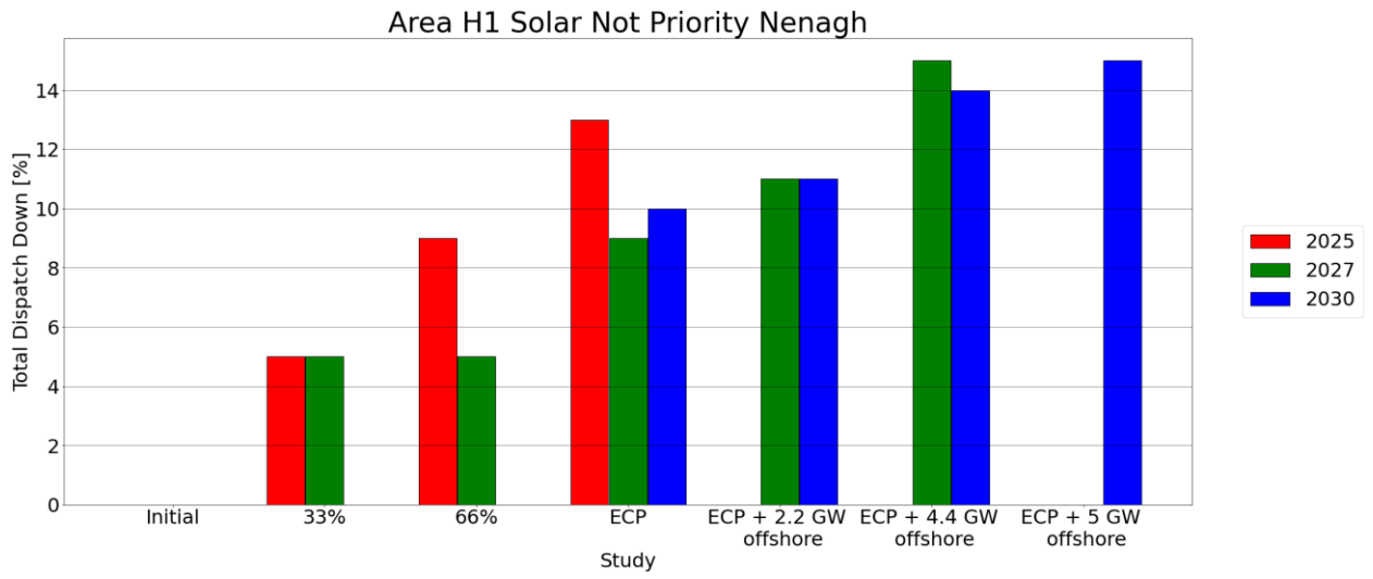
Figure C - 27 Total Dispatch Down for Solar Not Priority
