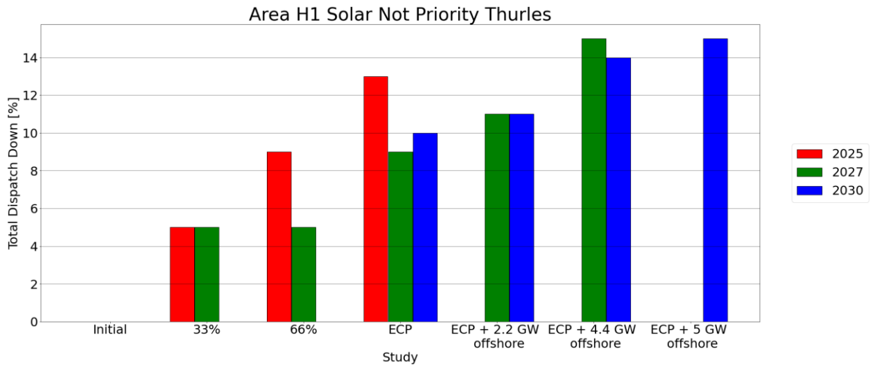
Figure C - 29 Total Dispatch Down for Solar Not Priority
