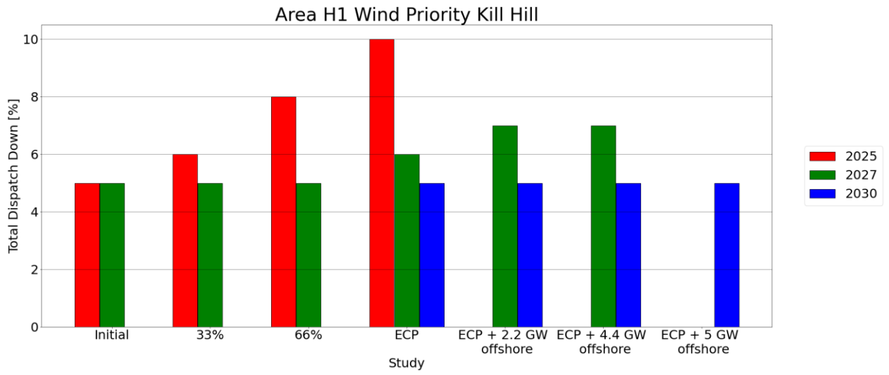
Figure C - 18 Total Dispatch Down for Wind Priority
