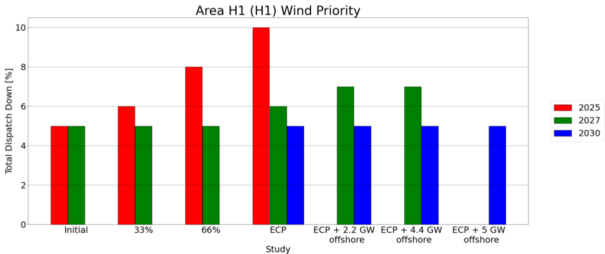
Figure 6-4 Results Wind Priority in Area H1 (H1)
