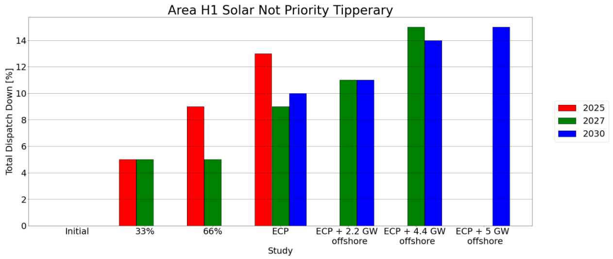
Figure C - 35 Total Dispatch Down for Solar Not Priority
