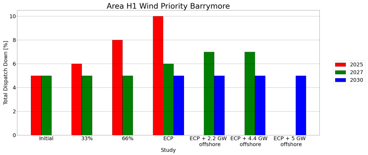
Figure C - 7 Total Dispatch Down for Wind Priority
