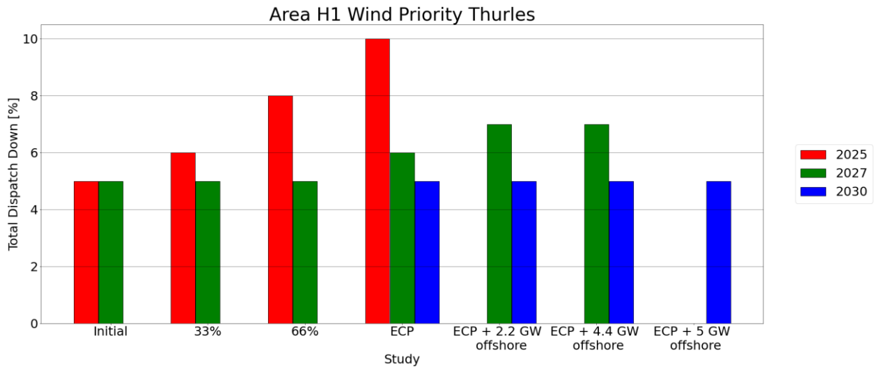
Figure C - 31 Total Dispatch Down for Wind Priority
