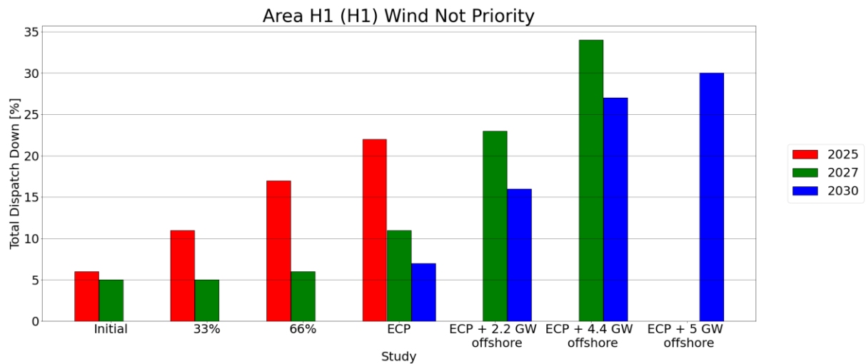
Figure 6-3 Results Wind Not Priority in Area H1 (H1)
