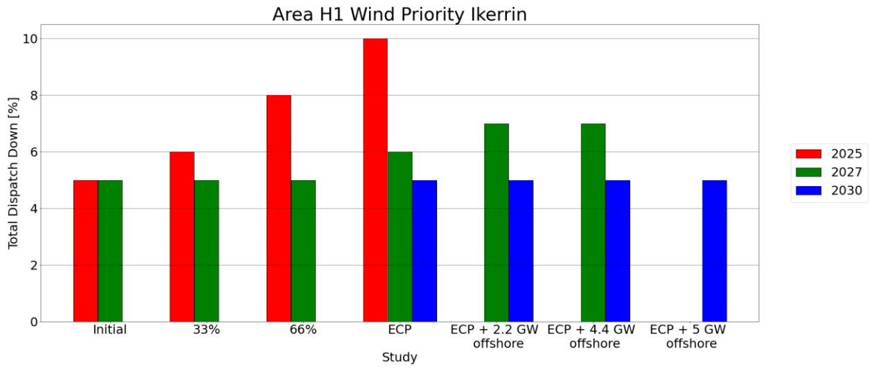
Figure C - 15 Total Dispatch Down for Wind Priority
