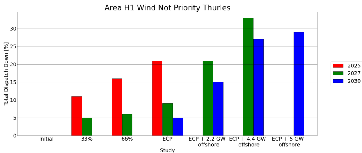
Figure C-29 - Total Dispatch Down for Wind not priority
