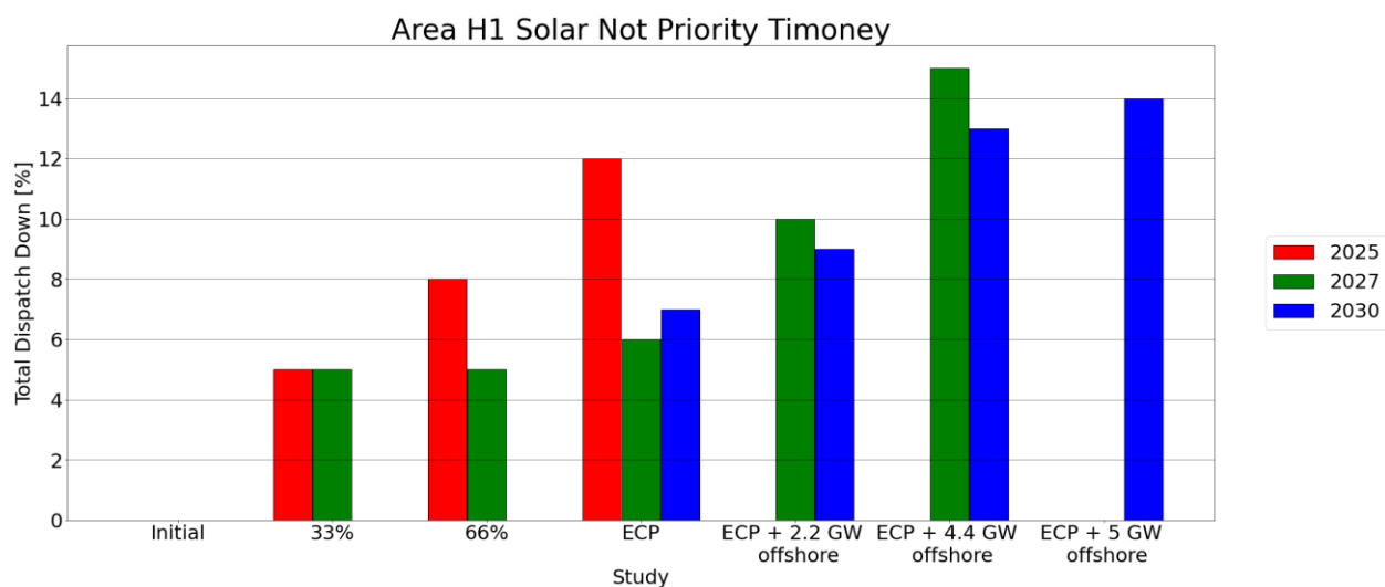
Figure C-32 - Total Dispatch Down for Solar not priority
