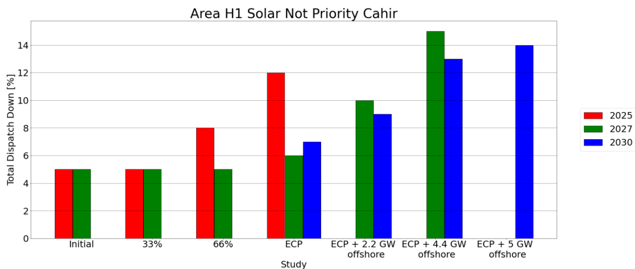
Figure C-9 - Total Dispatch Down for Solar not priority
