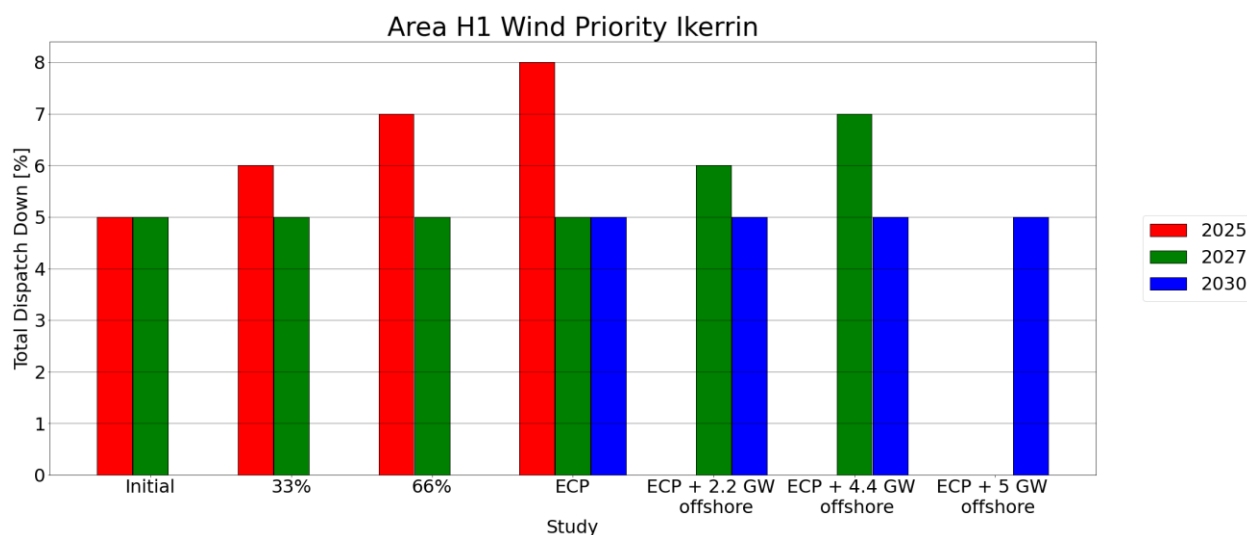
Figure C-15 - Total Dispatch Down for Wind priority
