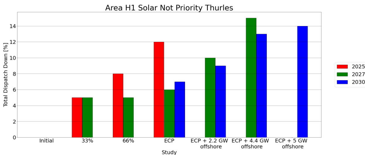
Figure C-28 - Total Dispatch Down for Solar not priority
