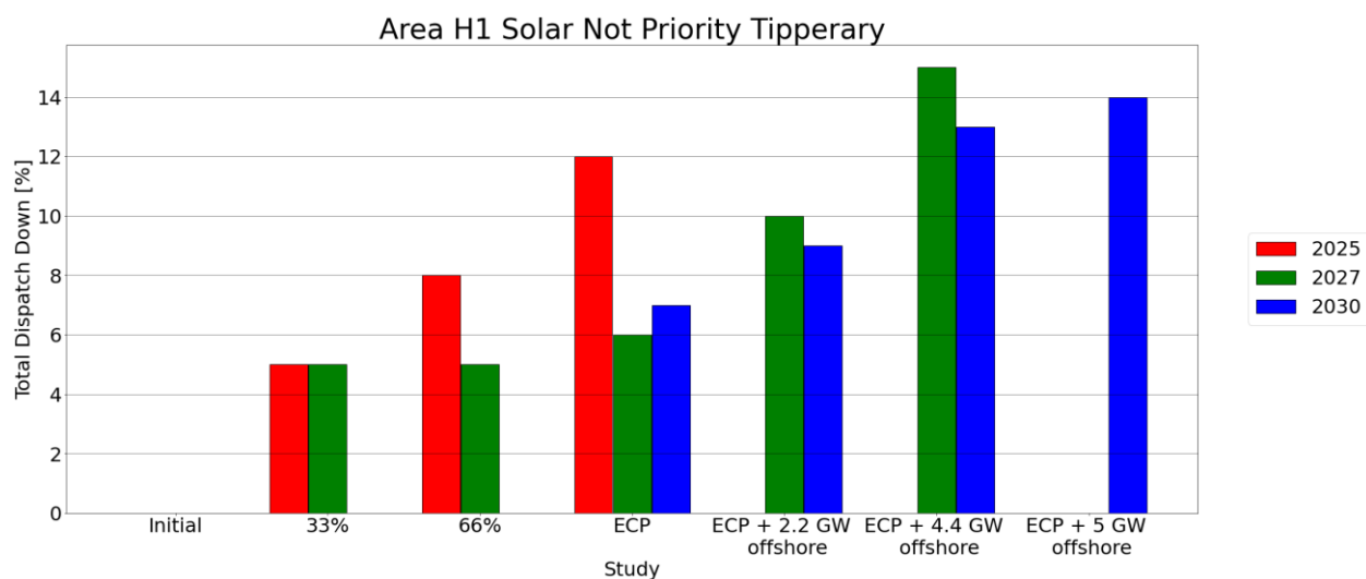
Figure C-34 - Total Dispatch Down for Solar not priority
