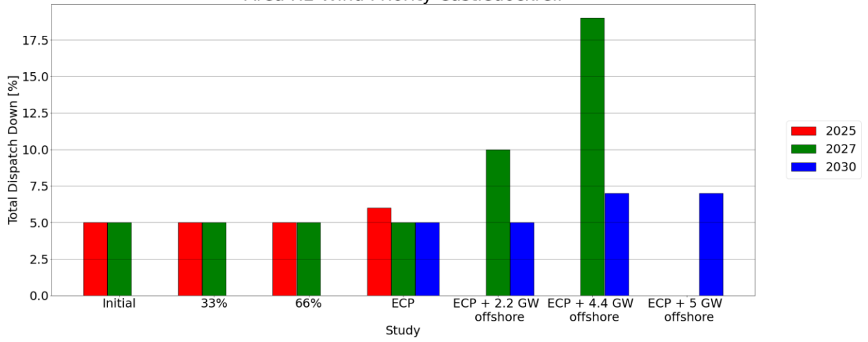
Figure C - 21 Total Dispatch Down for Wind Priority
