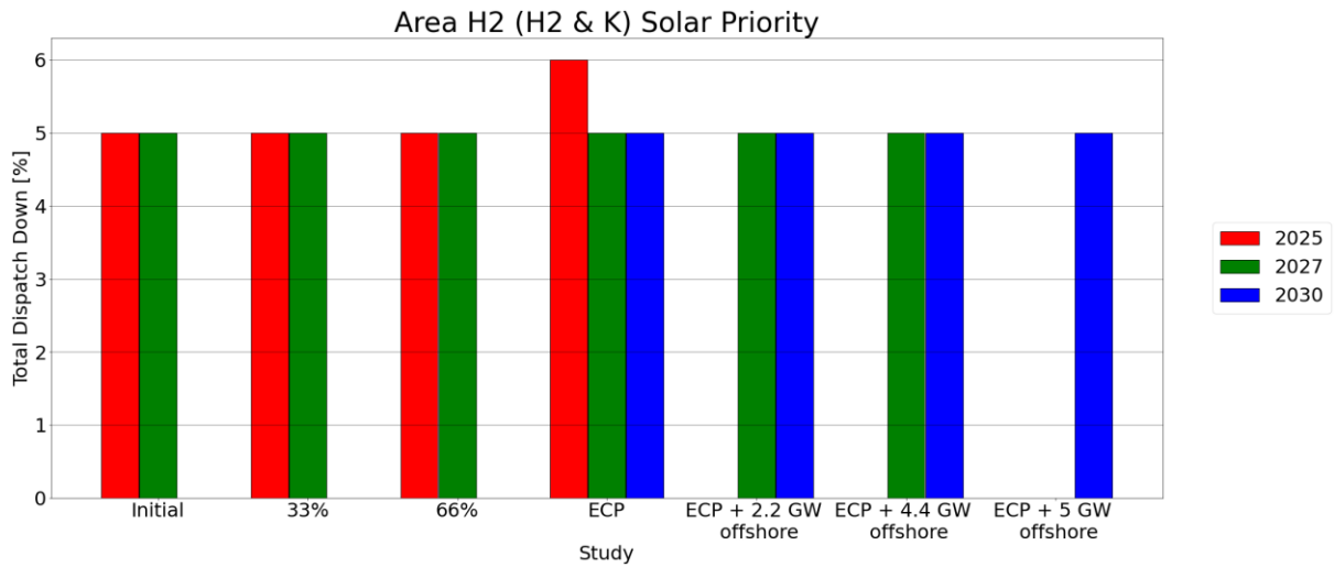
Figure 6-4 Results Solar Priority in Area H2 (H2 & K)
