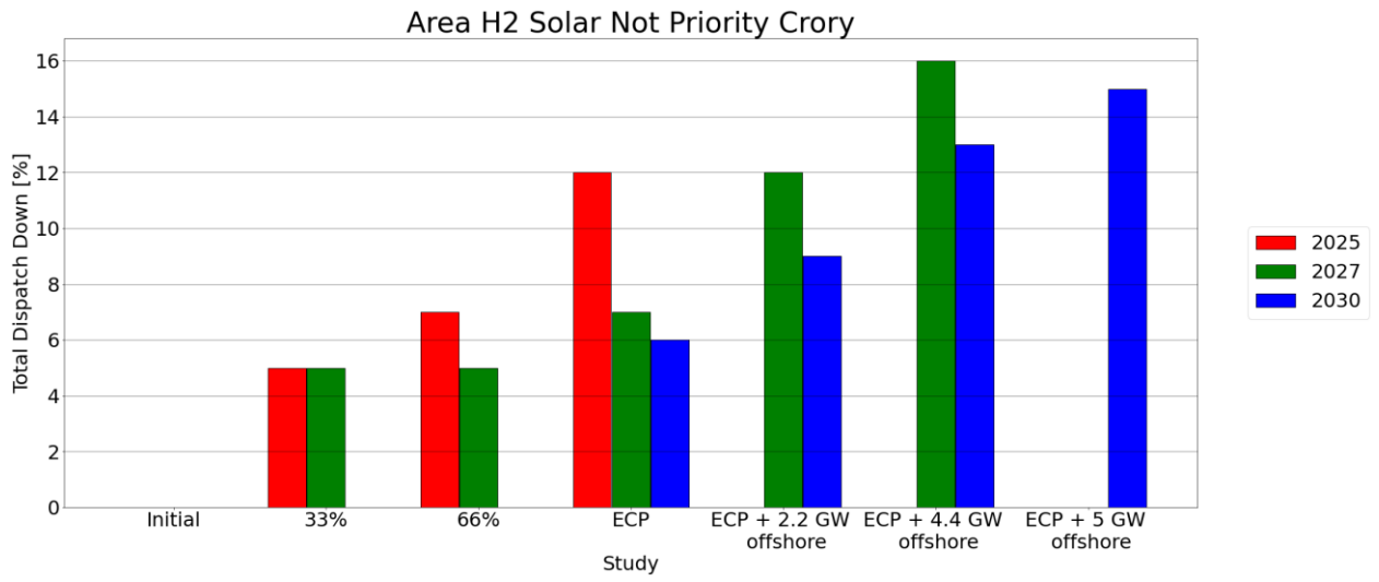
Figure C - 26 Total Dispatch Down for Solar Not Priority
