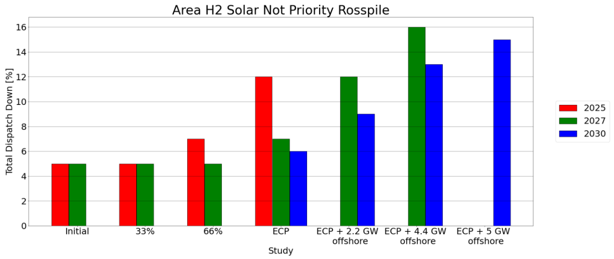
Figure C - 139 Total Dispatch Down for Solar Not Priority
