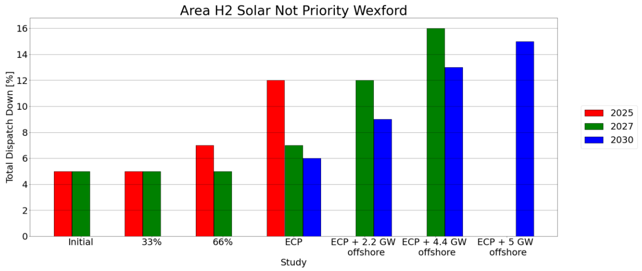
Figure C - 46 Total Dispatch Down for Solar Not Priority
