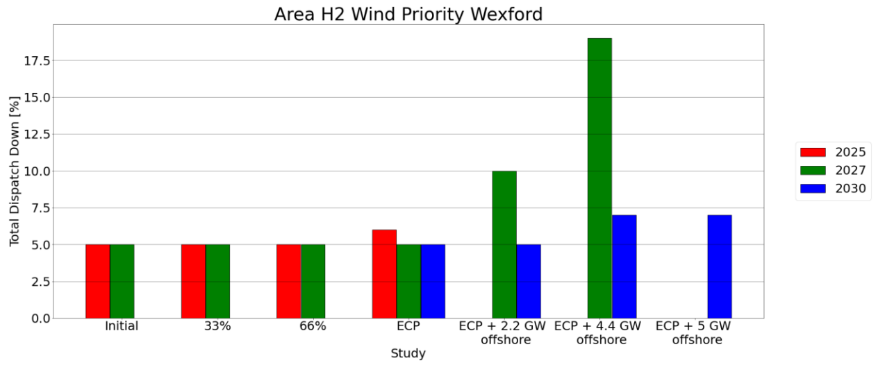
Figure C - 158 Total Dispatch Down for Wind Priority
