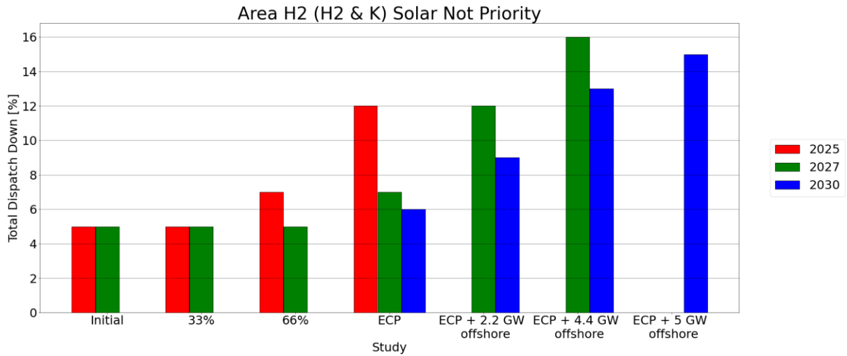
Figure 6-2 Results Solar Not Priority Area H2 (H2 & K)
