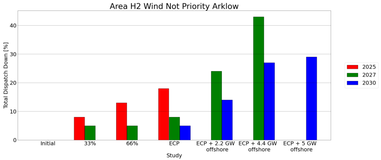
Figure C - 3 Total Dispatch Down for Wind Not Priority
