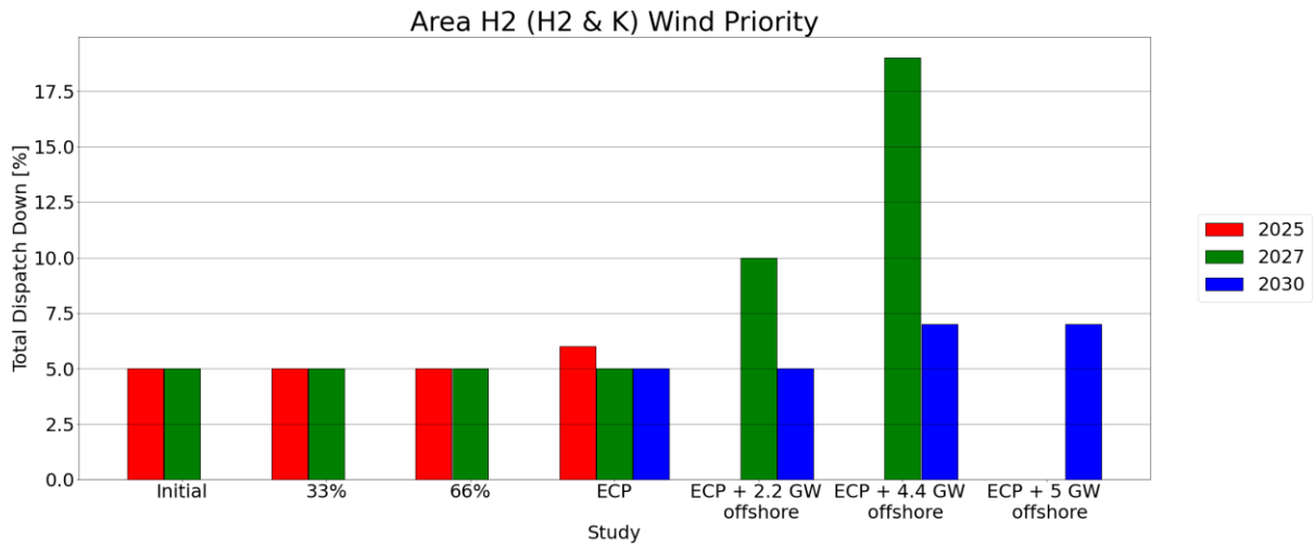
Figure 6-5 Results Wind Not Priority in Area H2 (H2 & K)
