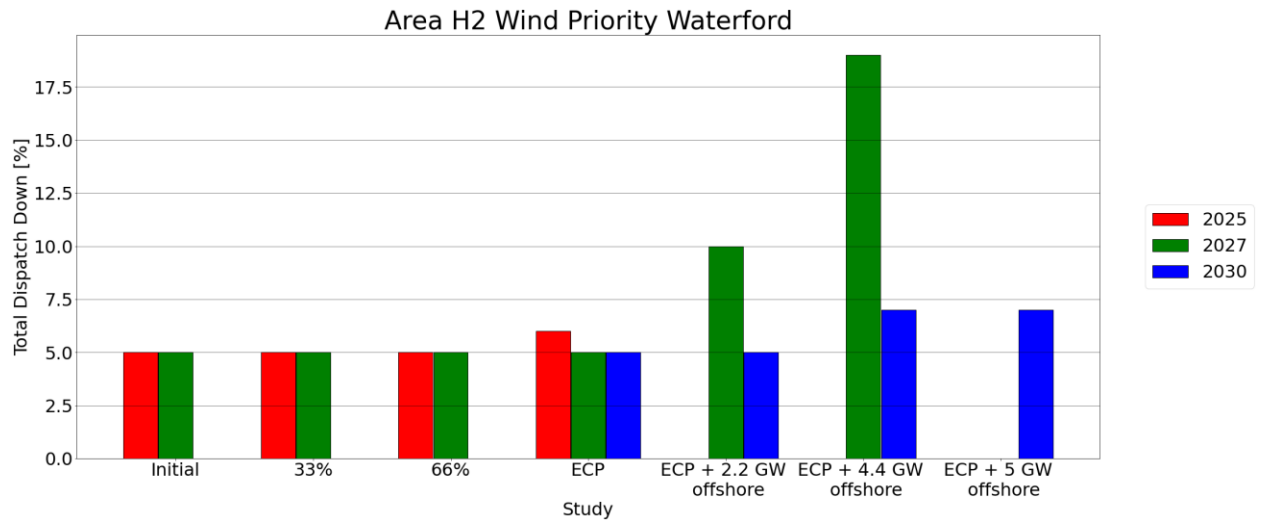
Figure C - 44 Total Dispatch Down for Wind Priority
