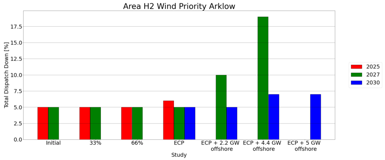
Figure C - 4 Total Dispatch Down for Wind Priority
