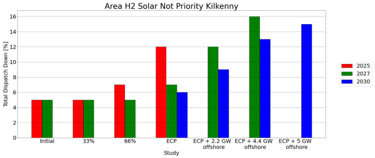
Figure C - 105 Total Dispatch Down for Solar Not Priority
