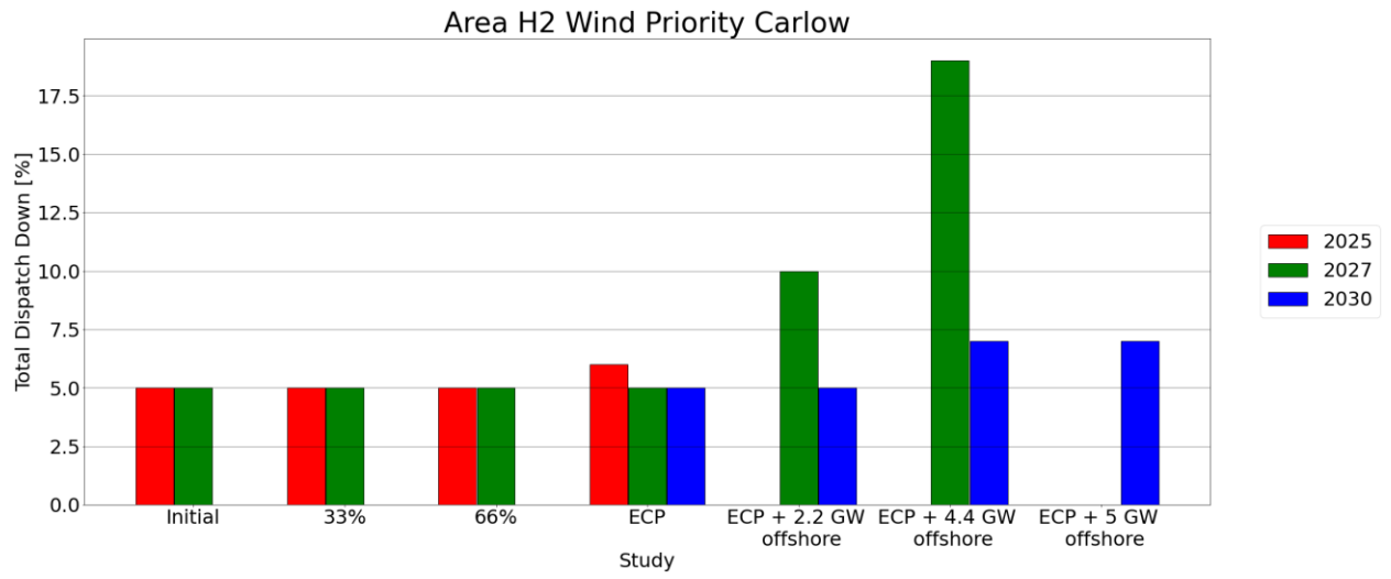
Figure C - 6 Total Dispatch Down for Wind Priority
