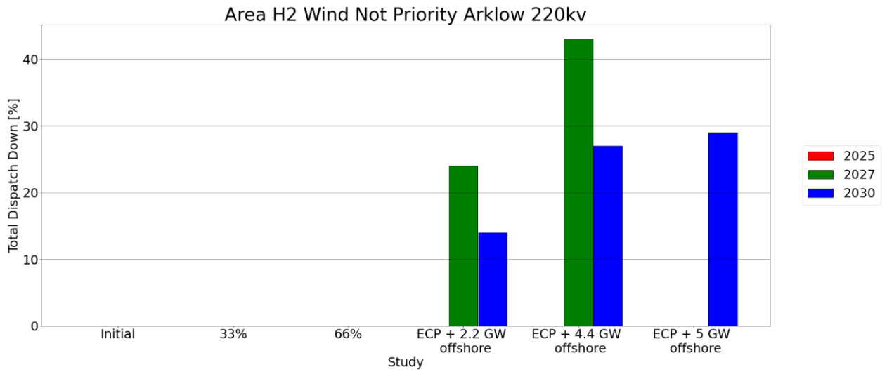
Figure C - 6 Total Dispatch Down for Wind Not Priority
