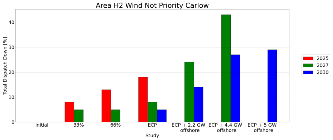
Figure C - 18 Total Dispatch Down for Wind Not Priority
