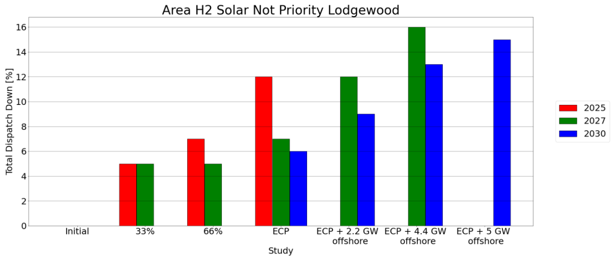
Figure C - 127 Total Dispatch Down for Solar Not Priority
