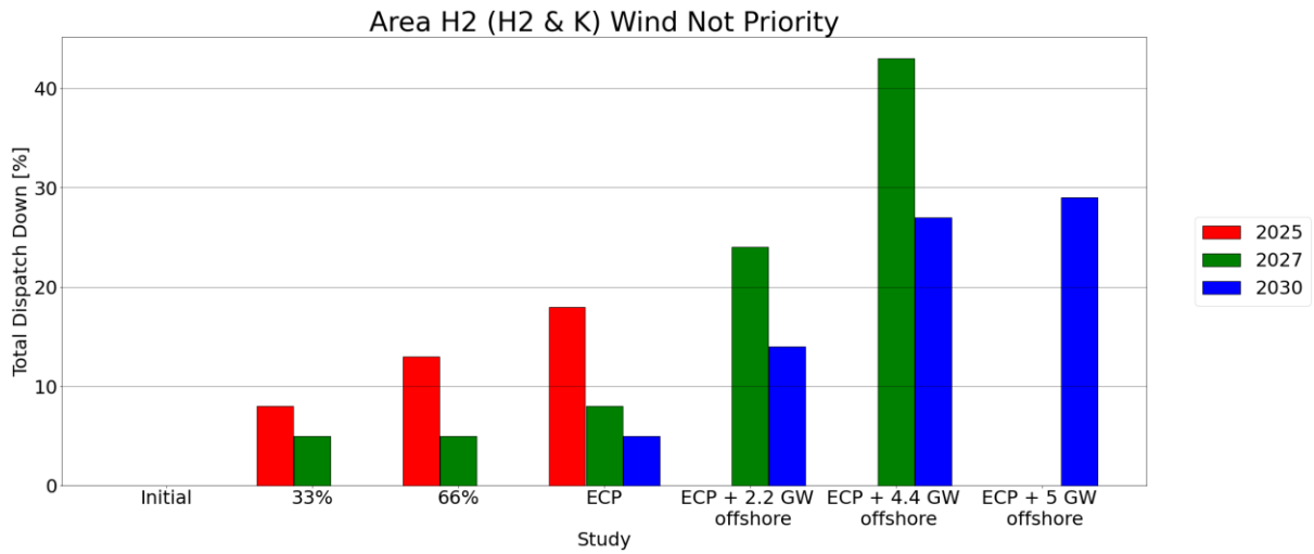
Figure 6-3 Results Wind Not Priority in Area H2 (H2 & K)
