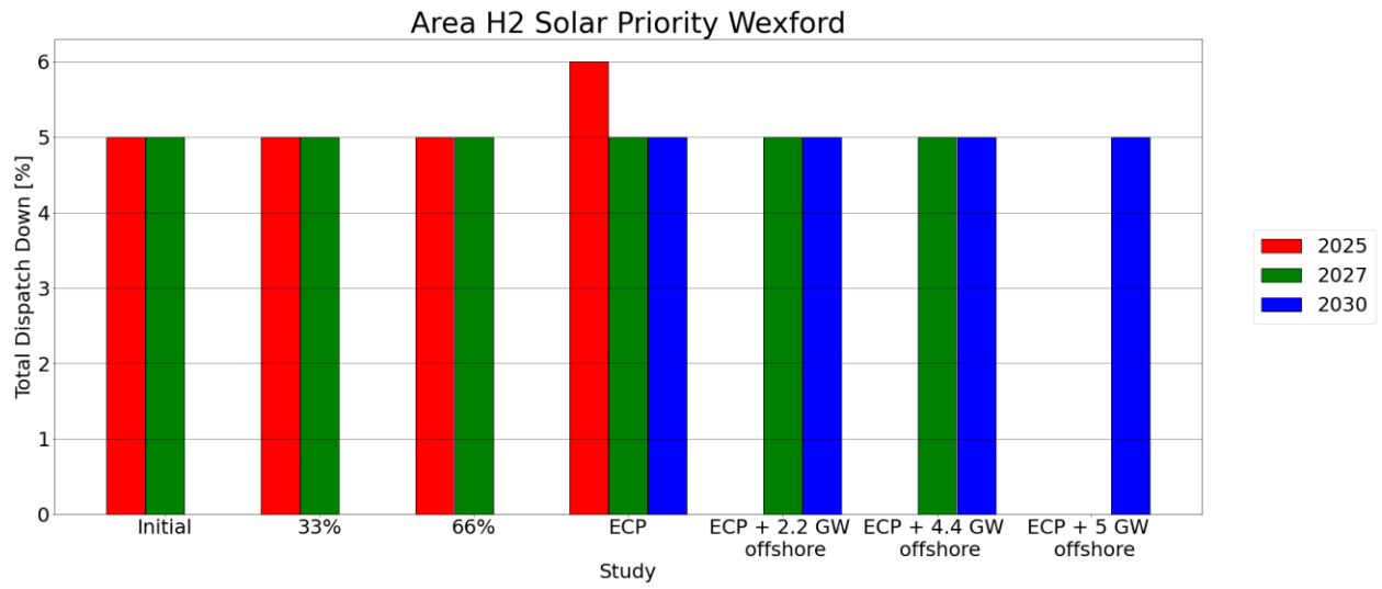
Figure C - 47 Total Dispatch Down for Solar Priority
