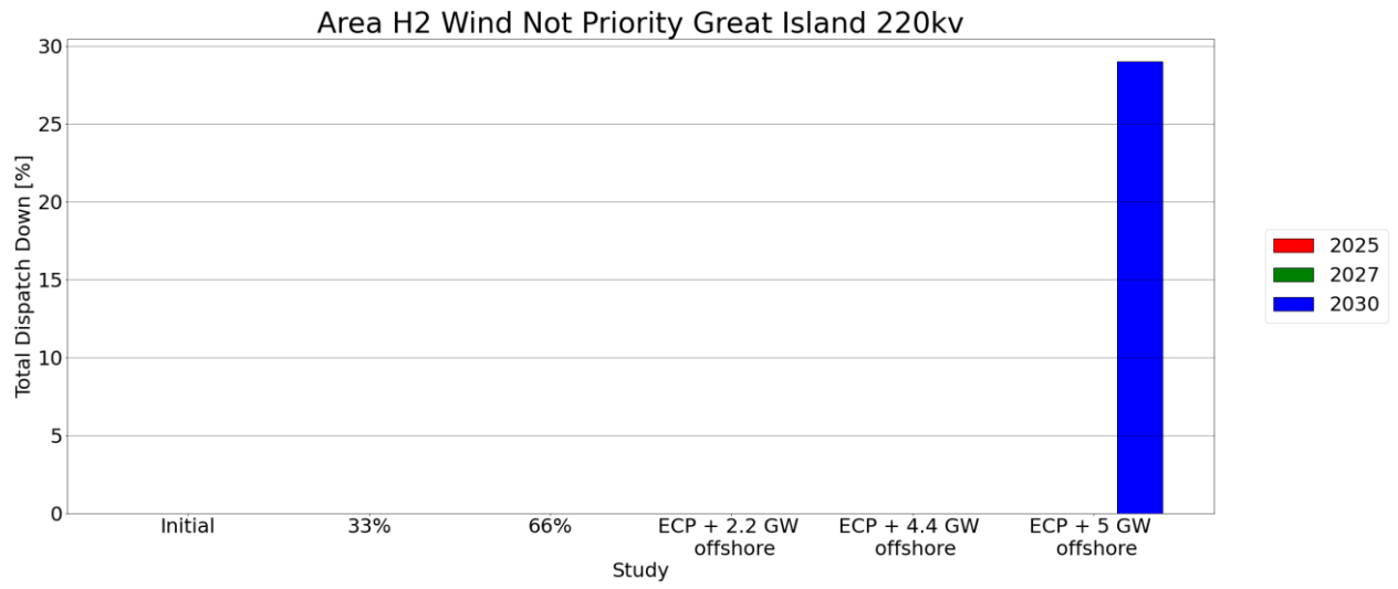
Figure C - 319 Total Dispatch Down for Wind Not Priority
