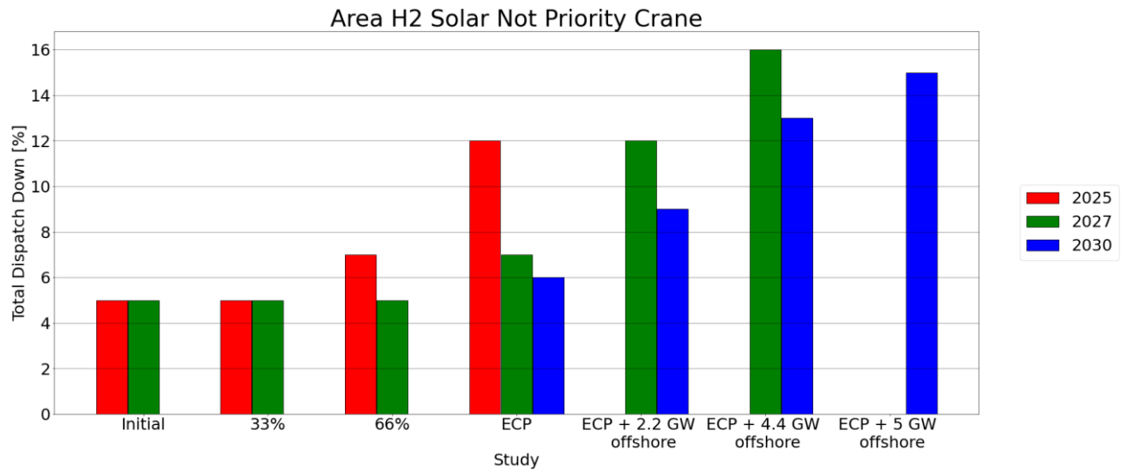
Figure C - 23 Total Dispatch Down for Solar Not Priority
