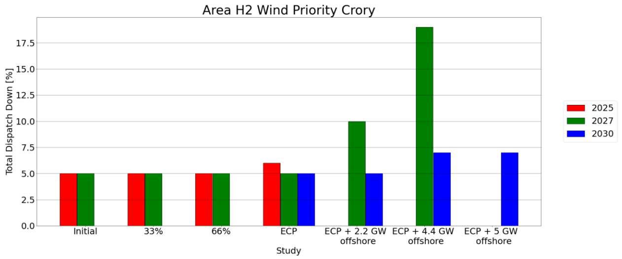
Figure C - 27 Total Dispatch Down for Wind Priority
