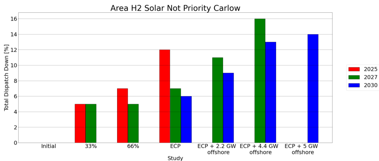
Figure C-17 - Total Dispatch Down for Solar not priority
