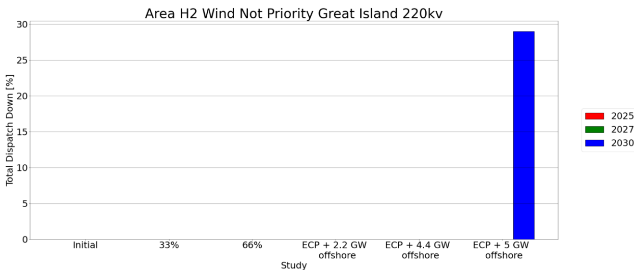
Figure C-31 - Total Dispatch Down for Wind not priority
