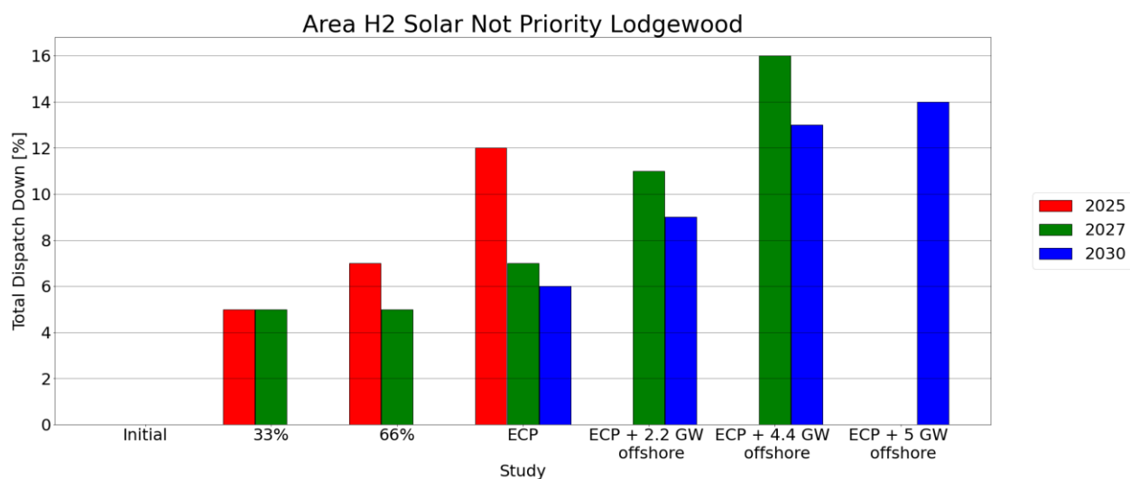
Figure C-37 - Total Dispatch Down for Solar not priority
