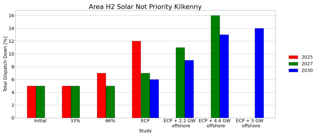
Figure C-35 - Total Dispatch Down for Solar not priority
