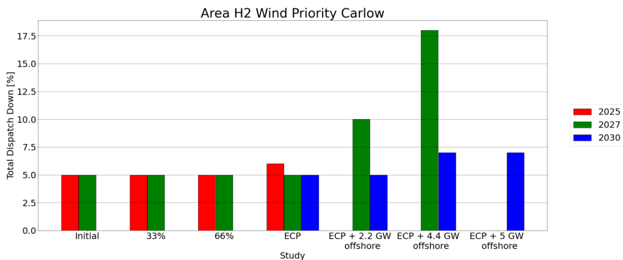
Figure C-19 - Total Dispatch Down for Wind priority
