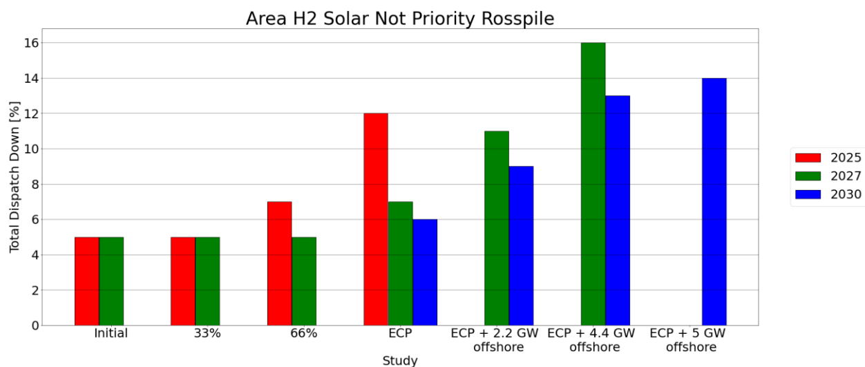
Figure C-39 - Total Dispatch Down for Solar not priority
