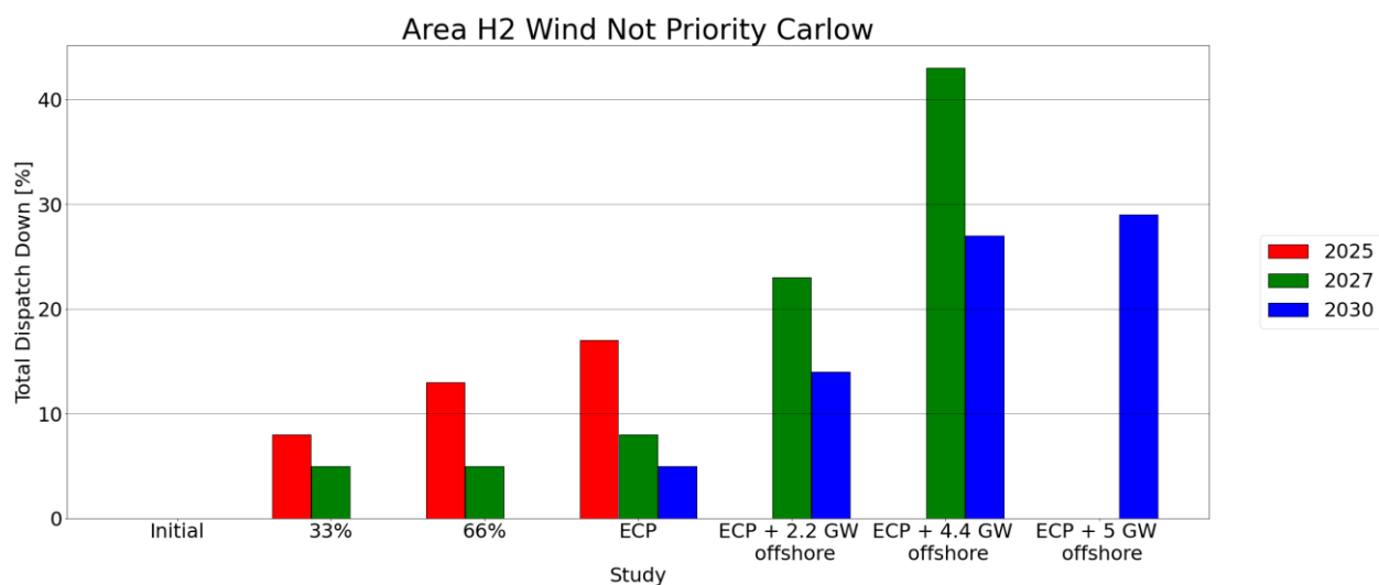
Figure C-18 - Total Dispatch Down for Wind not priority
