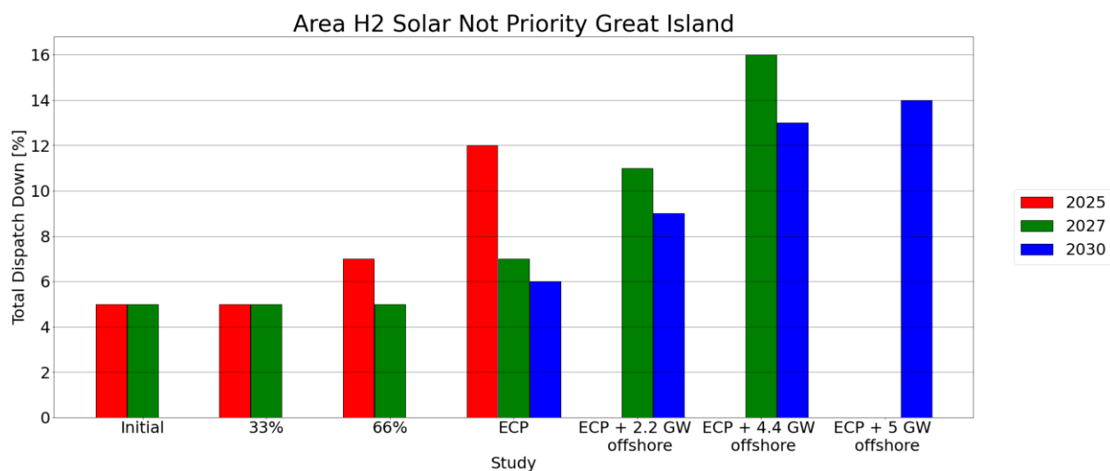
Figure C-29 - Total Dispatch Down for Solar not priority
