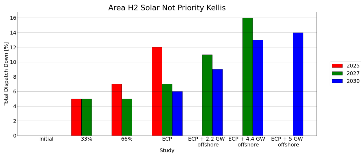
Figure C-33 - Total Dispatch Down for Solar not priority
