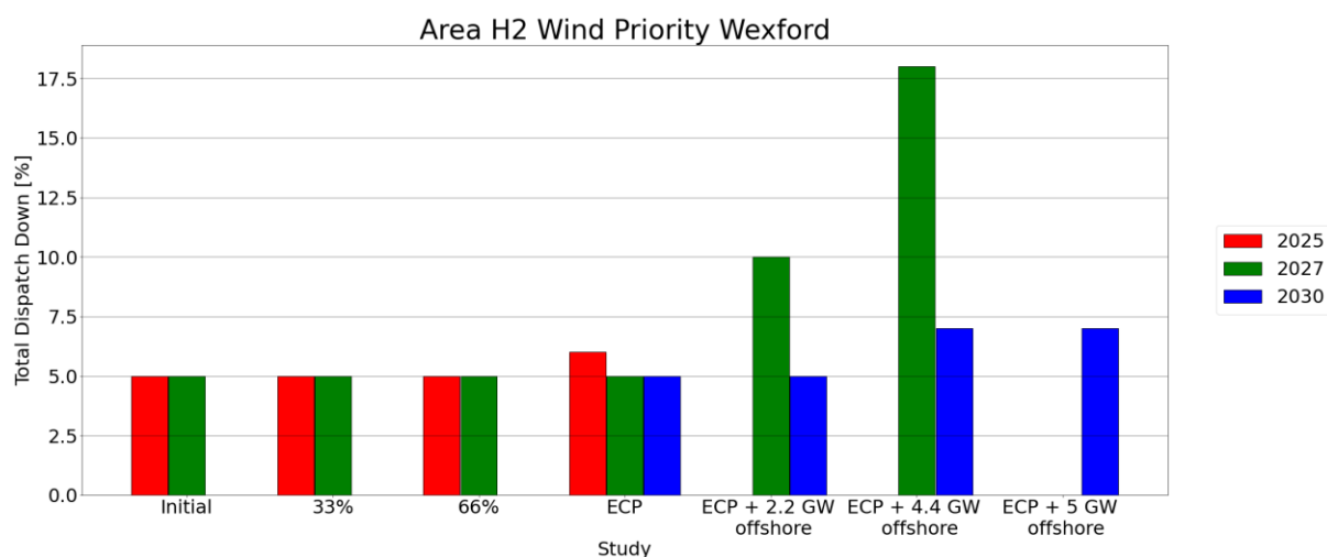
Figure C-47 - Total Dispatch Down for Wind priority
