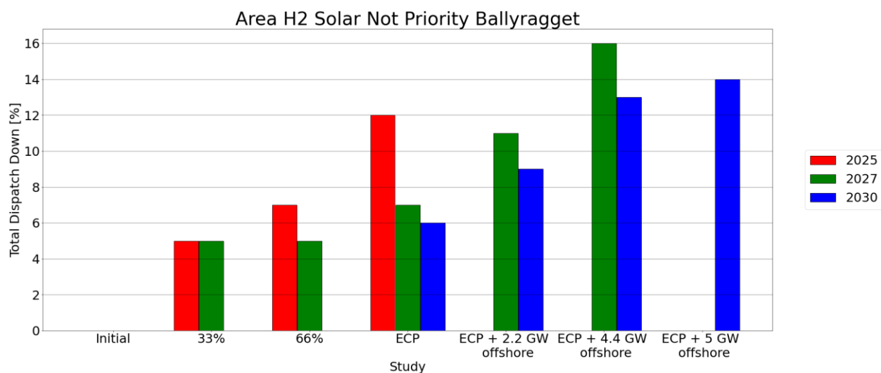
Figure C-10 - Total Dispatch Down for Solar not priority
