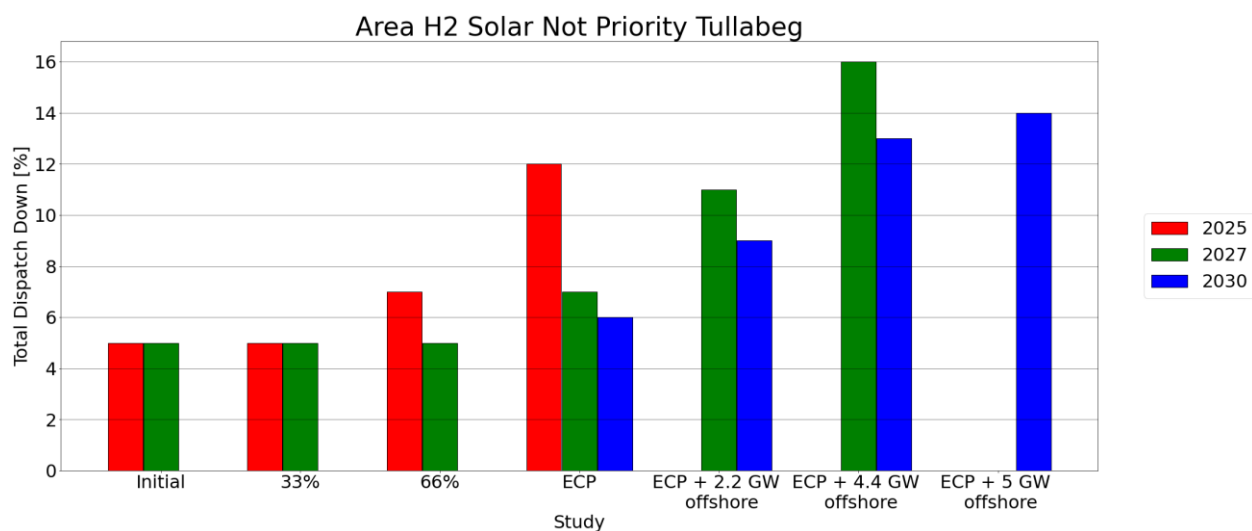
Figure C-41 - Total Dispatch Down for Solar not priority
