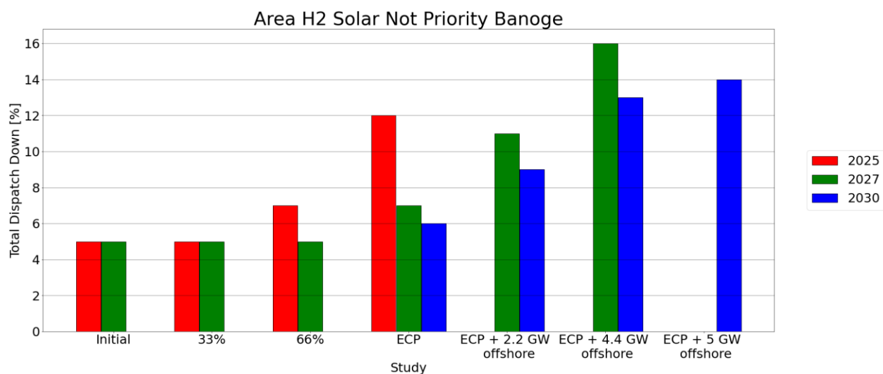
Figure C-15 - Total Dispatch Down for Solar not priority
