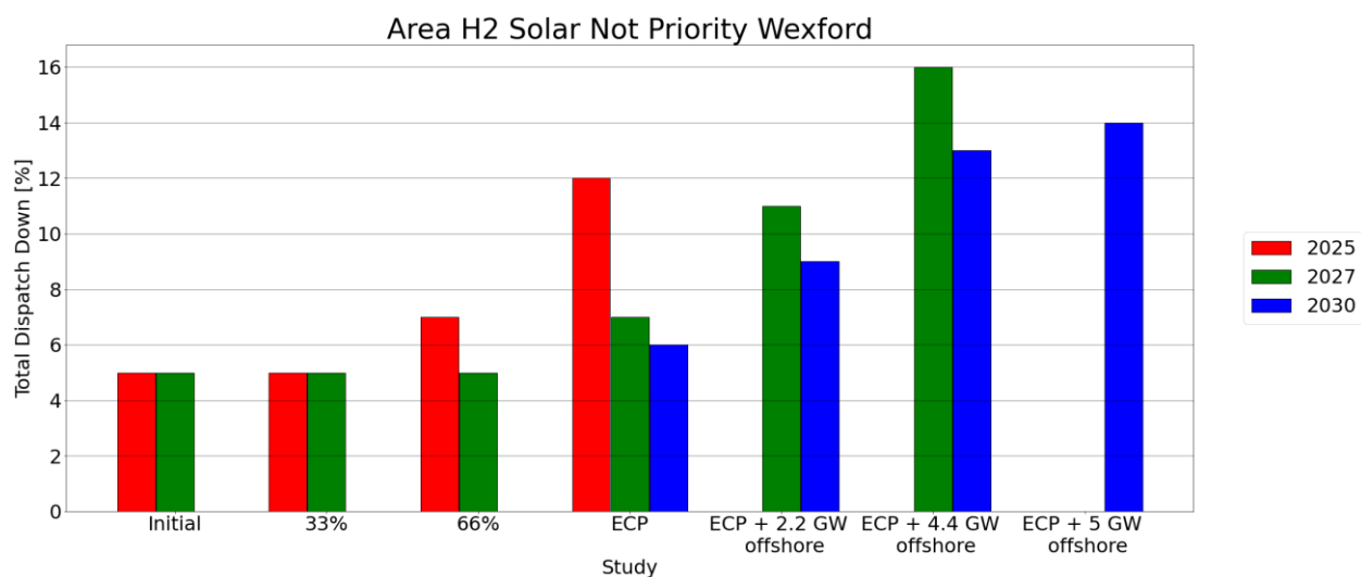
Figure C-46 - Total Dispatch Down for Solar not priority
