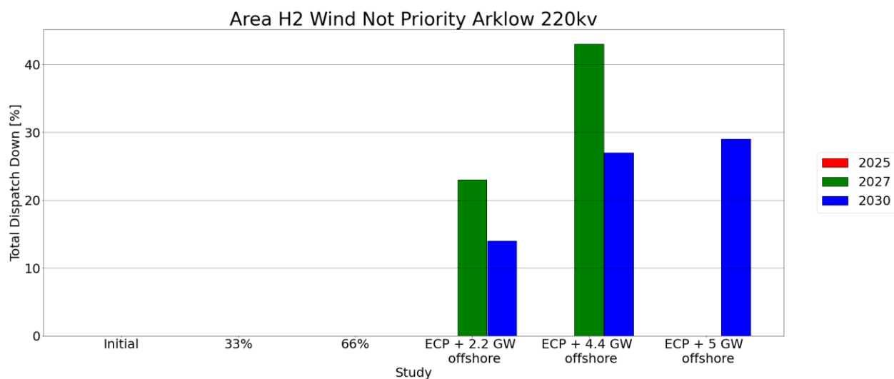
Figure C-6 - Total Dispatch Down for Wind not priority
