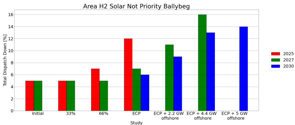
Figure C-8 - Total Dispatch Down for Solar not priority
