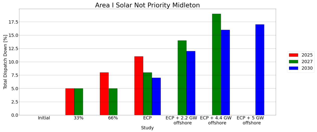
Figure C - 16 Total Dispatch Down for Solar Not Priority
