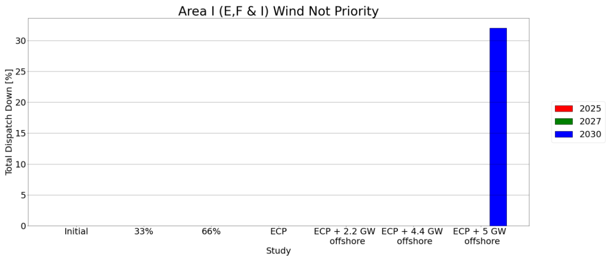
Figure 6-3 Results Wind Not Priority in Area I (E F & I)
