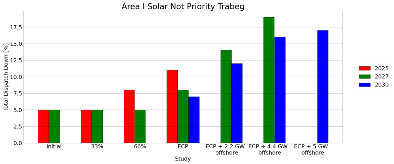
Figure C - 20 Total Dispatch Down for Solar Not Priority
