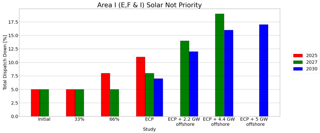
Figure 6-2 Results Solar Not Priority Area I (E F & I)
