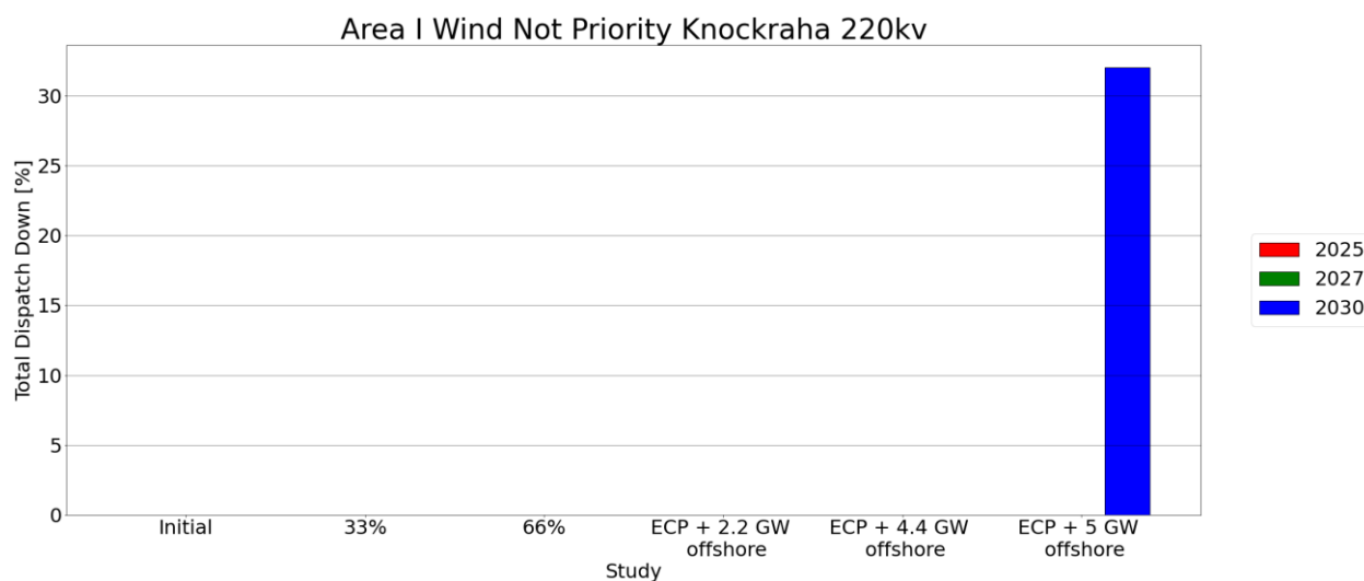
Figure C-12 - Total Dispatch Down for Wind not priority
