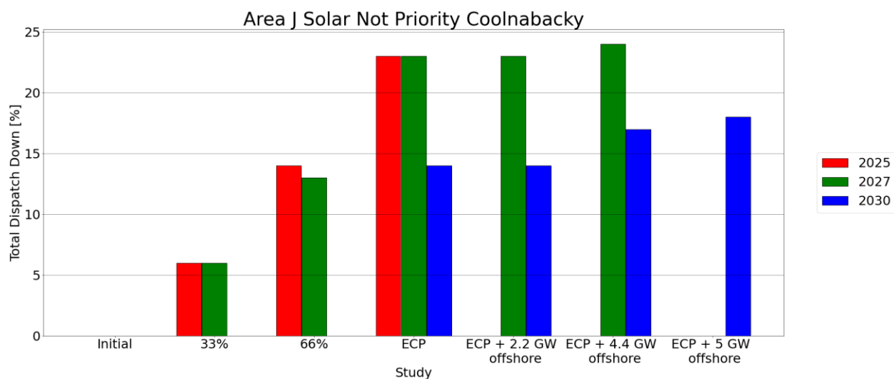
Figure C-14 - Total Dispatch Down for Solar not priority
