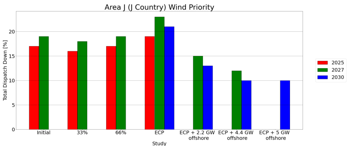
Figure 6-4 Results Wind Priority in Area J (J Country)
