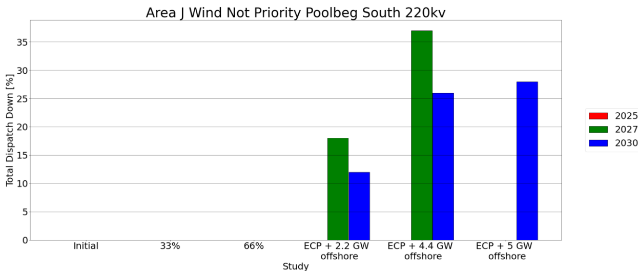
Figure C-48 - Total Dispatch Down for Wind not priority
