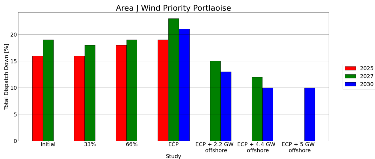
Figure C-52 - Total Dispatch Down for Wind priority
