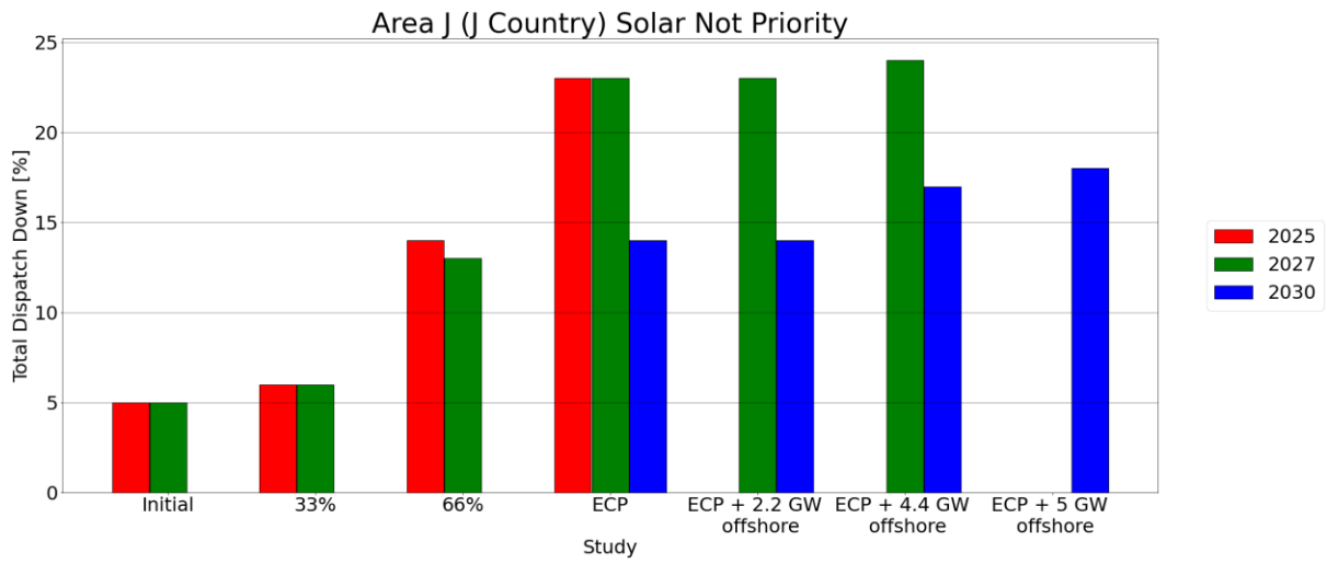
Figure 6-2 Results Solar Not Priority in Area J (J Country)
