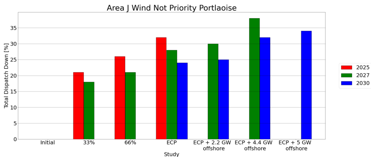
Figure C-51 - Total Dispatch Down for Wind not priority
