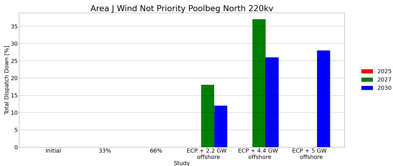
Figure C-46 - Total Dispatch Down for Wind not priority
