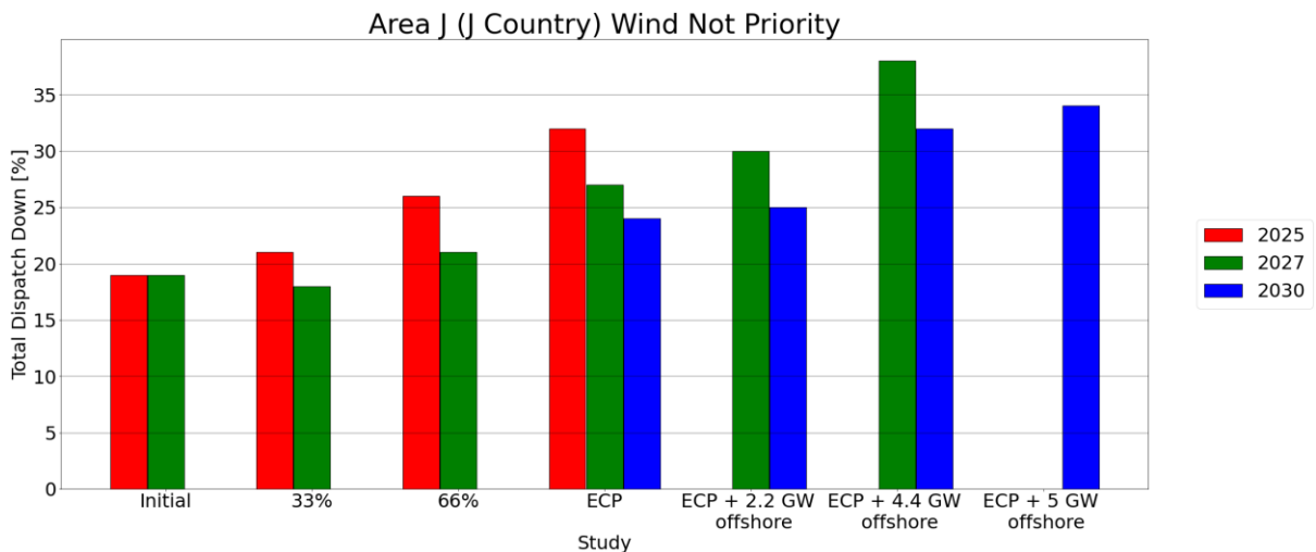
Figure 6-3 Results Wind Not Priority in Area J (J Country)
