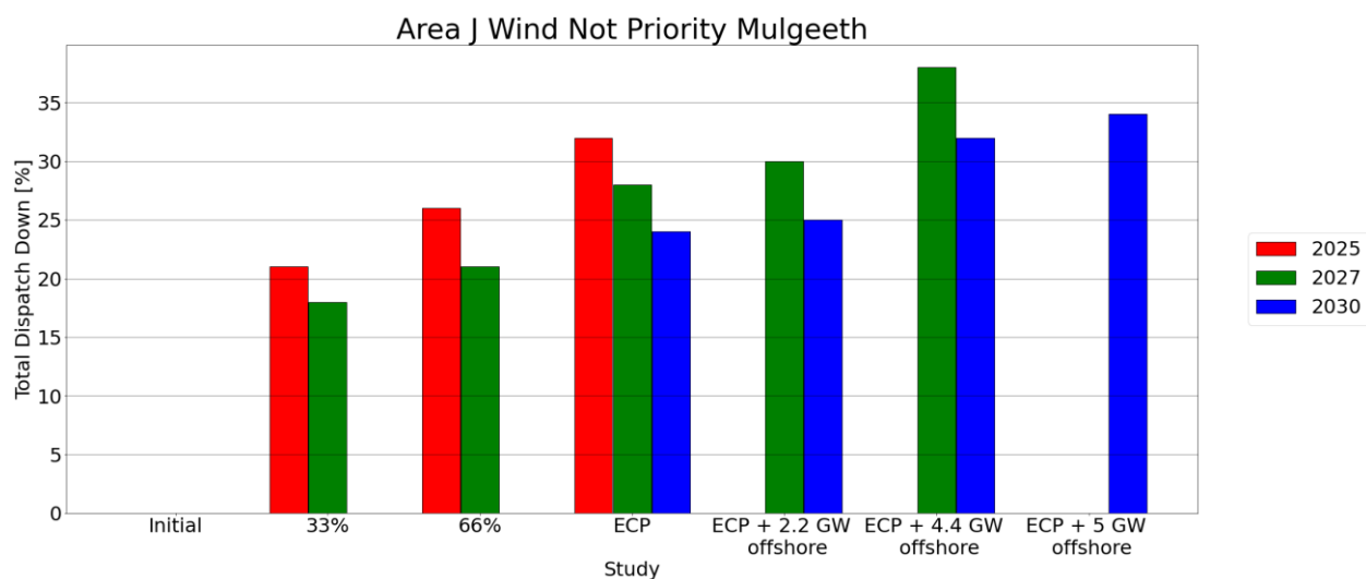
Figure C-40 - Total Dispatch Down for Wind not priority
