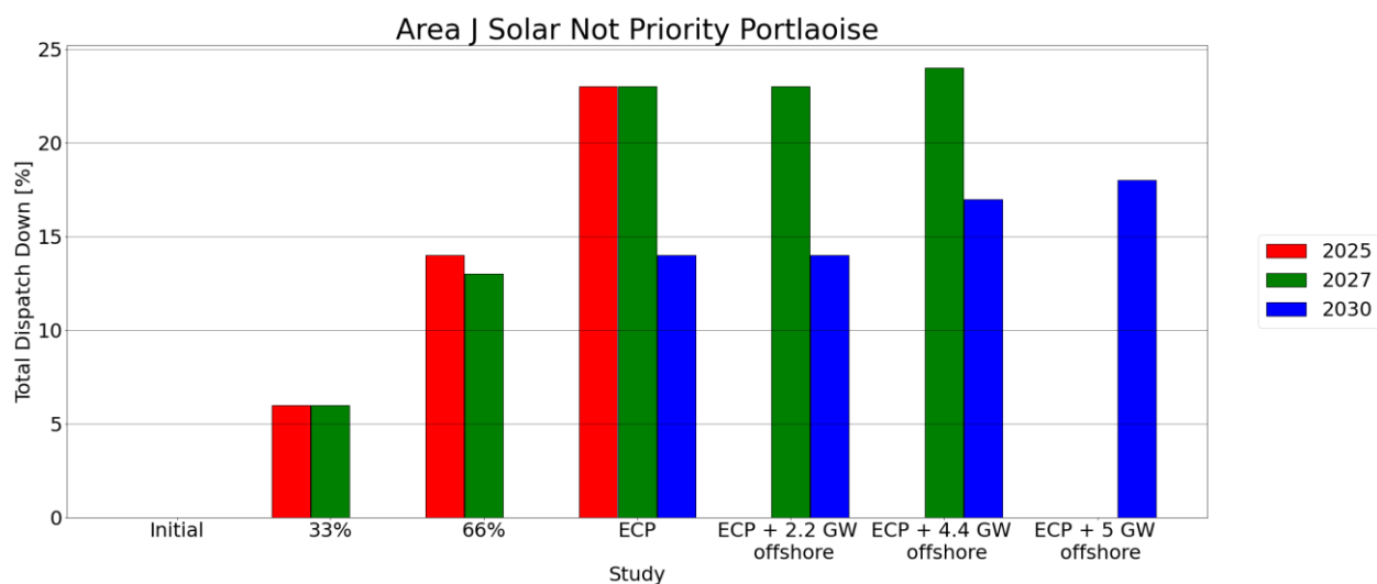
Figure C-50 - Total Dispatch Down for Solar not priority
