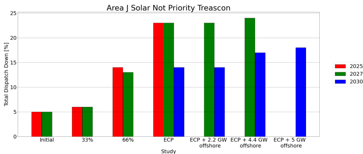
Figure C-61 - Total Dispatch Down for Solar not priority
