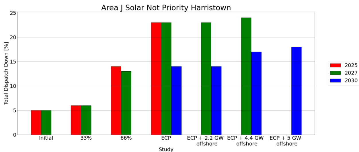
Figure C-31 - Total Dispatch Down for Solar not priority
