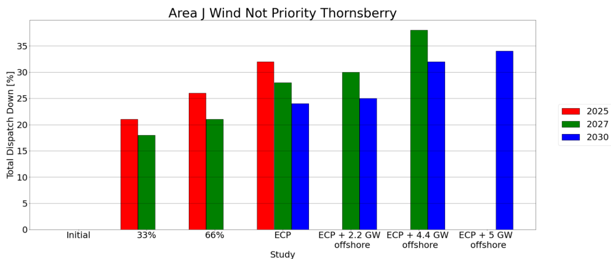
Figure C-57 - Total Dispatch Down for Wind not priority
