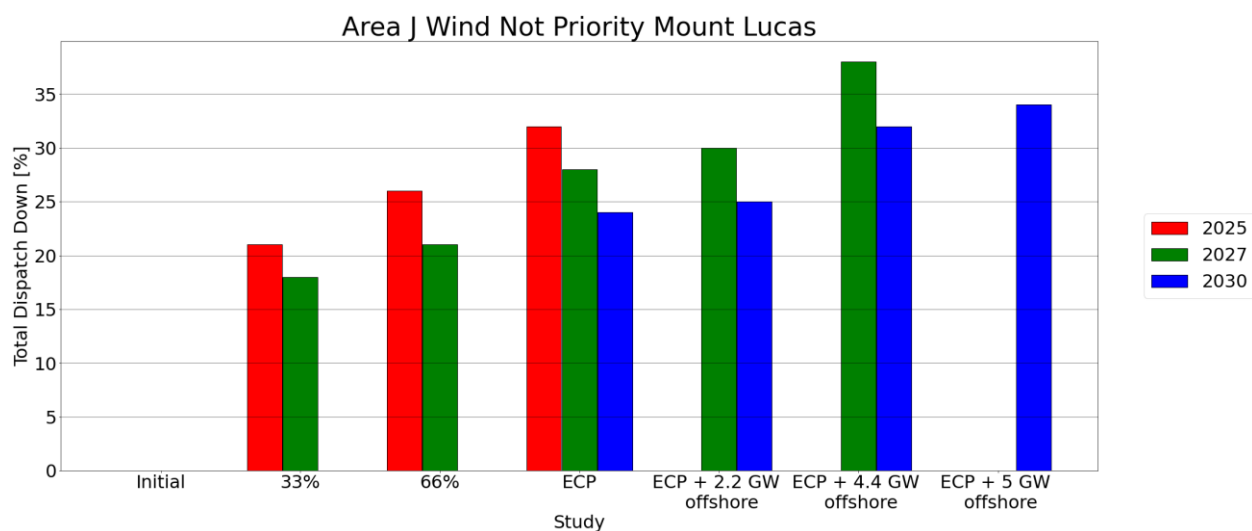
Figure C-37 - Total Dispatch Down for Wind not priority
