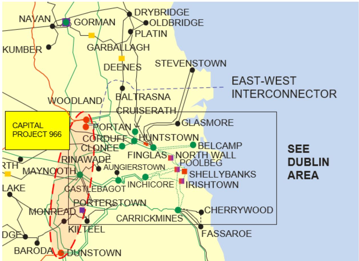
Figure C-26 - Location of node Glasmore
