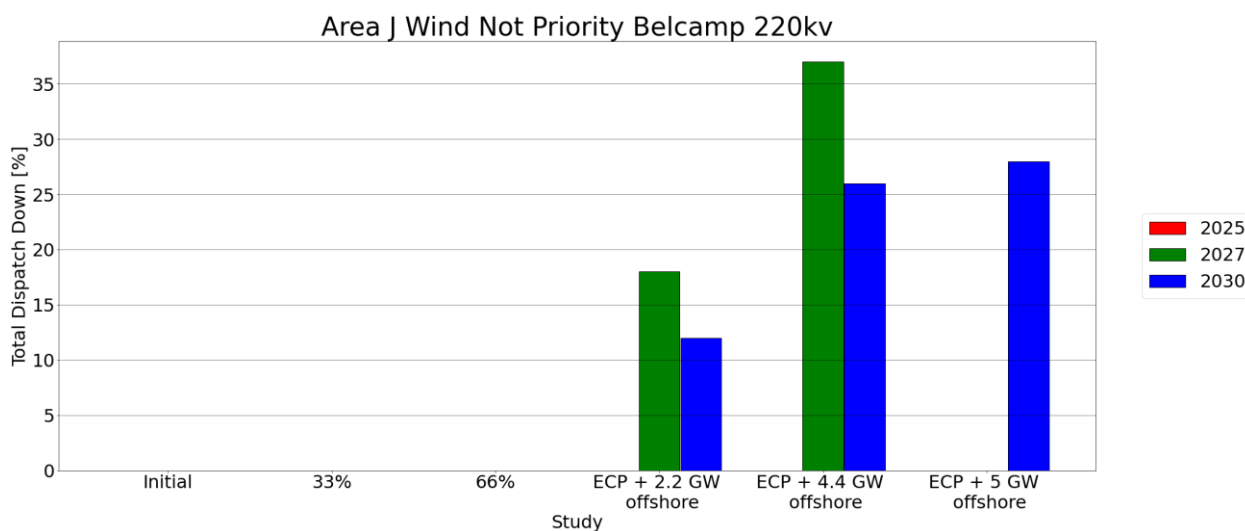
Figure C-4 - Total Dispatch Down for Wind not priority
