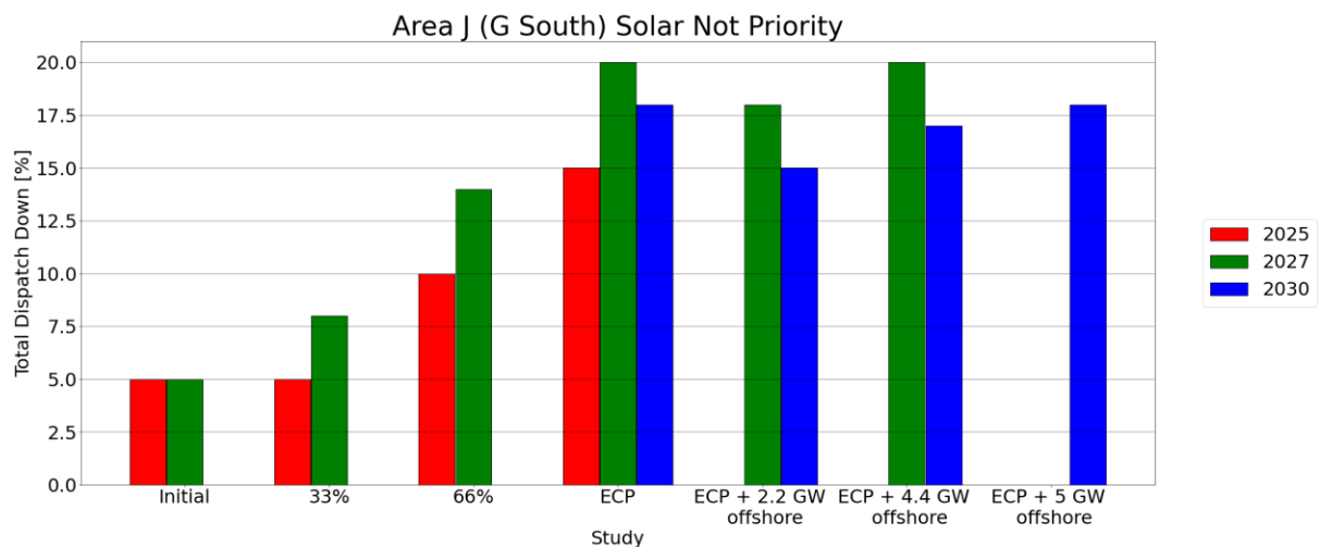
Figure 6-5 Results Solar Not Priority in Area J (G South)
