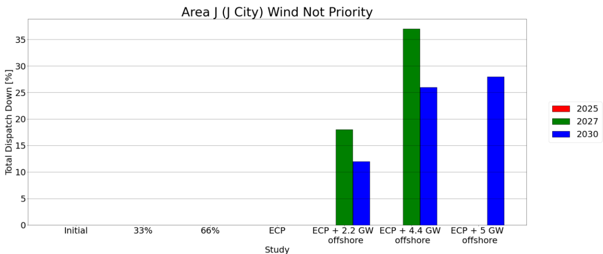
Figure 6-7 Results Wind Not Priority in Area J (J City)
