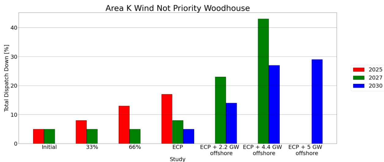
Figure C-8 - Total Dispatch Down for Wind not priority
