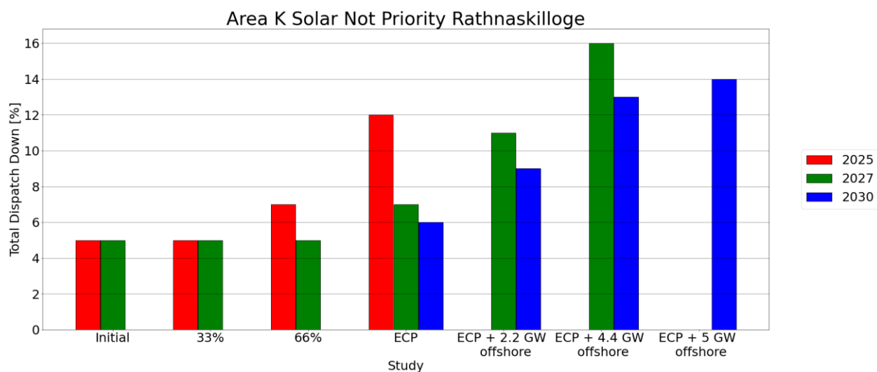
Figure C-6 - Total Dispatch Down for Solar not priority
