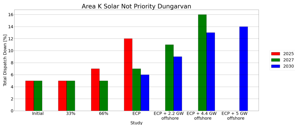
Figure C-4 - Total Dispatch Down for Solar not priority
