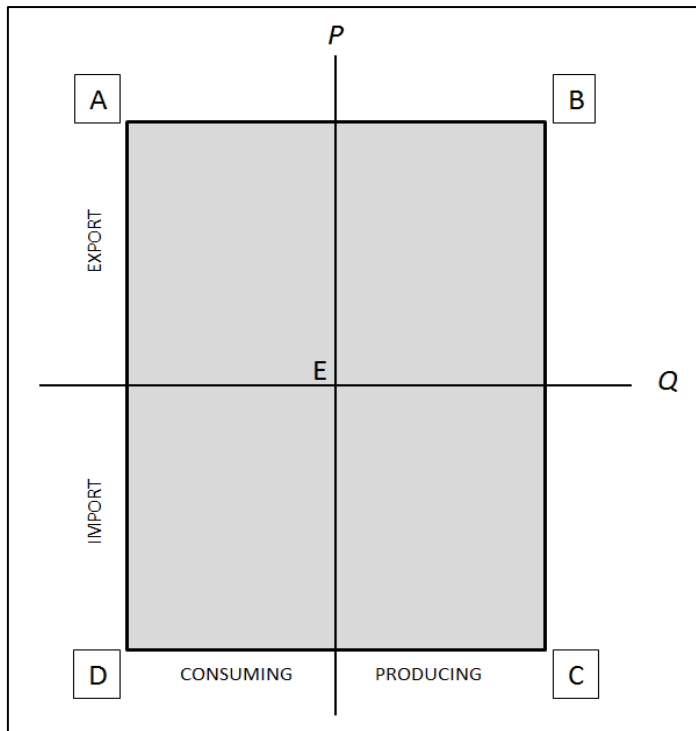
Figure PPM 1.6.3.1.b: Minimum Reactive Power Capability of Controllable PPMs consisting of ESPs
