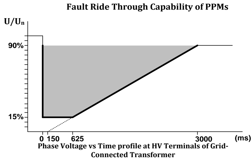
Figure 1.4.1- Fault Ride-Through Capability of Controllable PPMs
