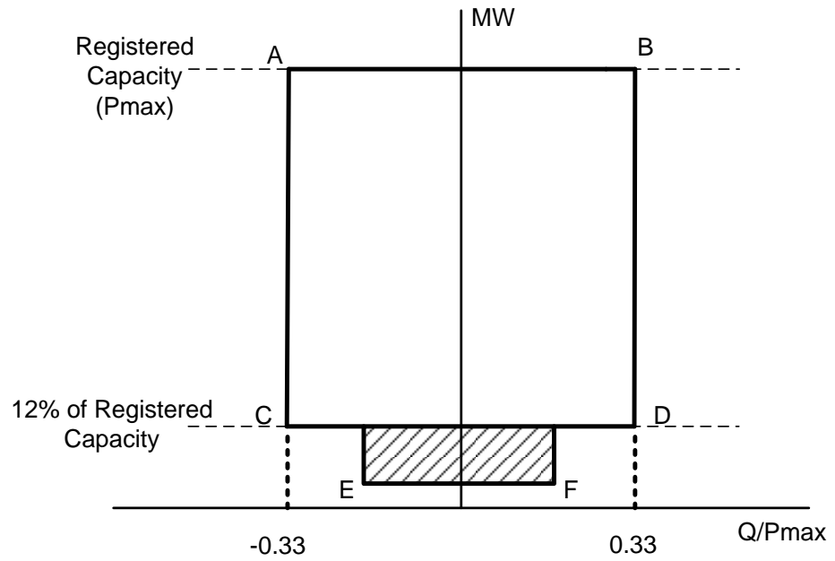
Figure PPM1.4 Figure PPM 1.6.3.1.a – Minimum Reactive Power Capability of Controllable PPM
