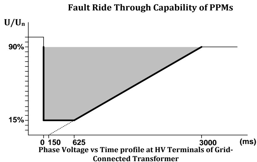
Figure PPM-1.1 1.4.1- Fault Ride-Through Capability of Controllable PPMs
