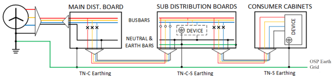
Figure 1 – Earthing Concept
