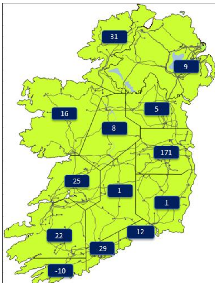
Figure 5 - Total regional MW dispatch change from 2020/21 to 2021/22
